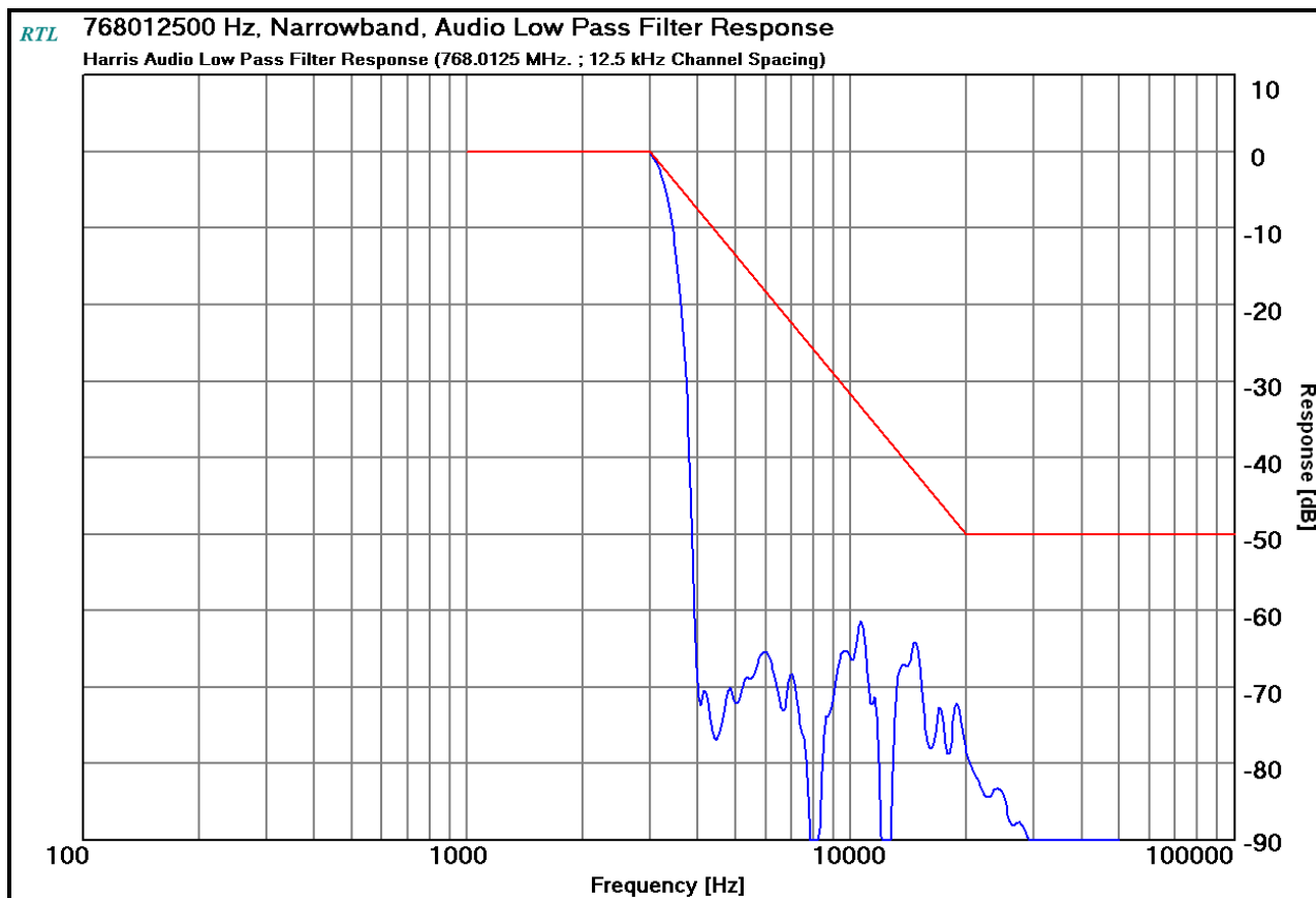
Plot 10-22: Modulation Characteristics – Audio Low Pass Filter – 768.0125 MHz
