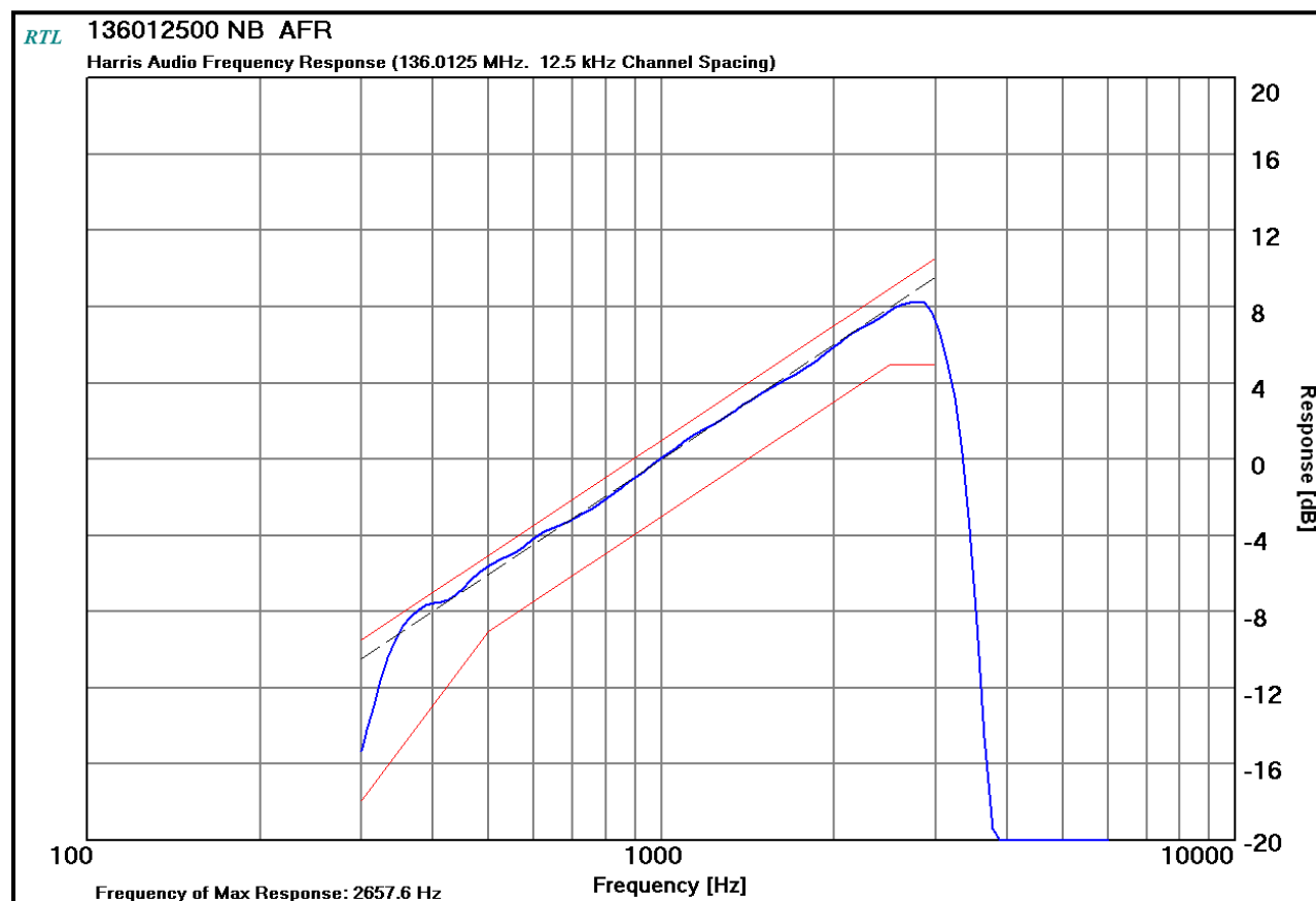
Plot 10-1: Modulation Characteristics - Audio Frequency Response – 136.0125 MHz
