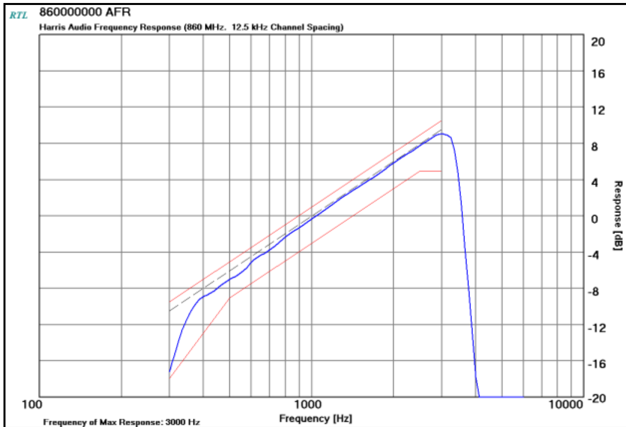
Plot 10-14: Modulation Characteristics - Audio Frequency Response – 860.0000 MHz
