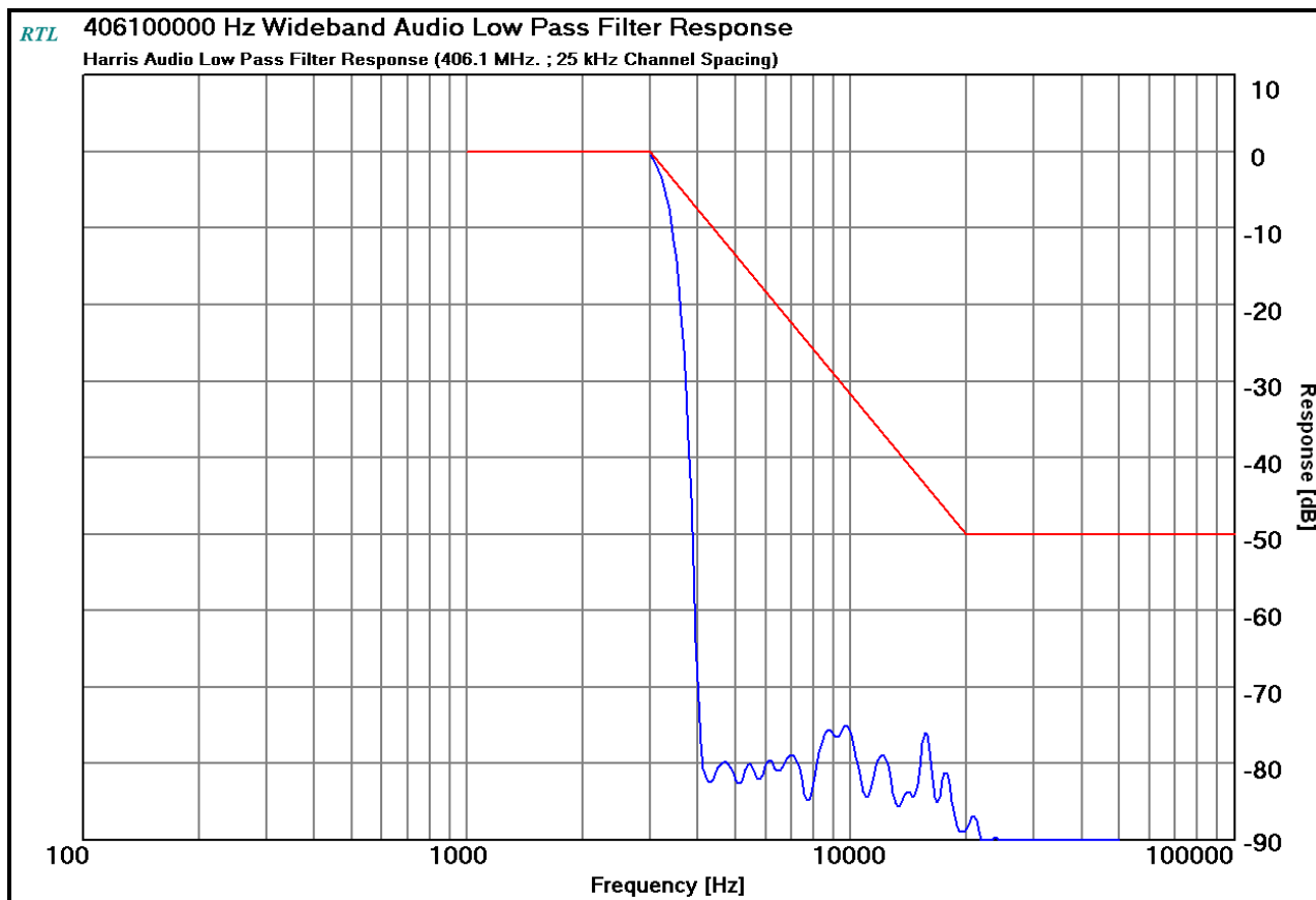
Plot 10-19: Modulation Characteristics – Audio Low Pass Filter – 406.1000 MHz (WB)
