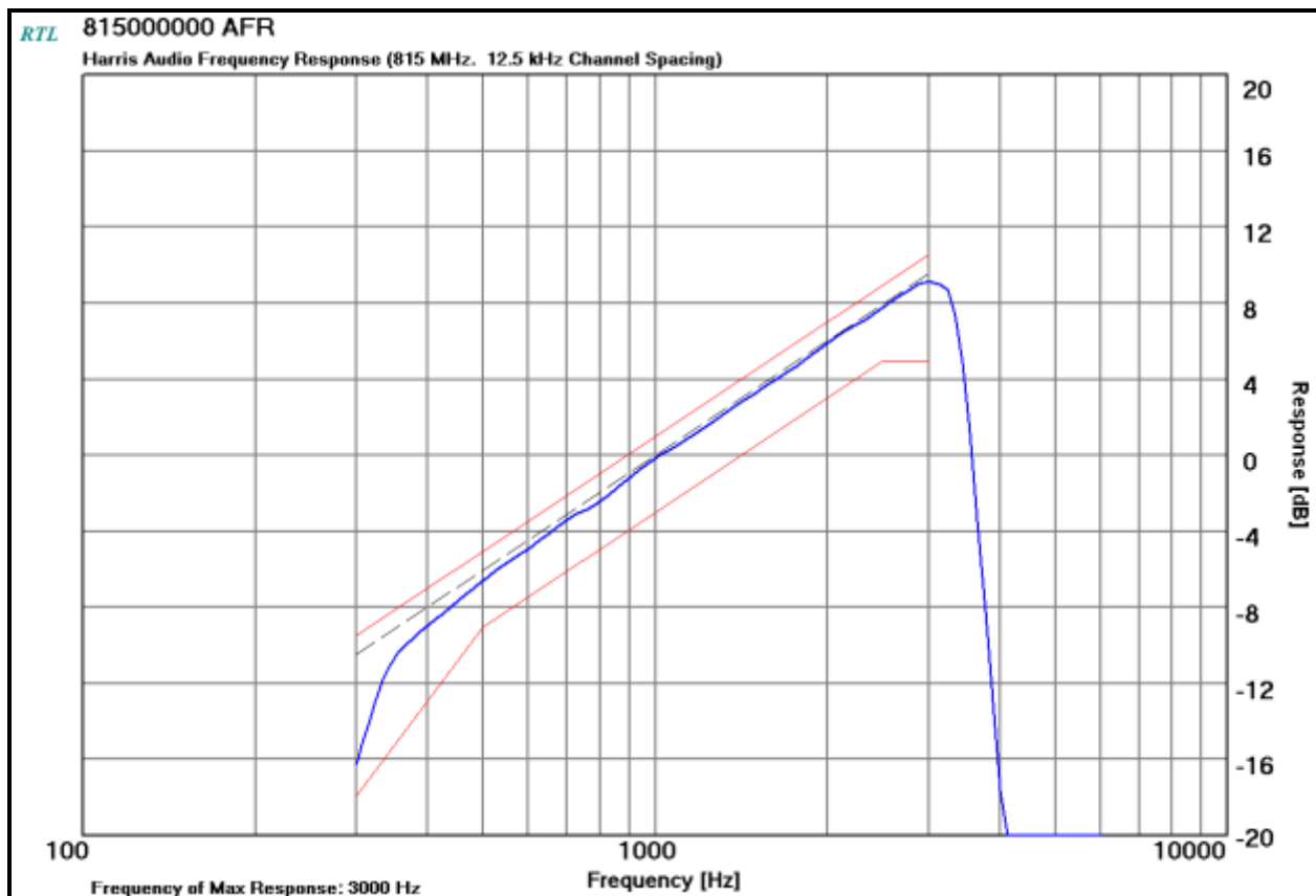
Plot 10-11: Modulation Characteristics - Audio Frequency Response – 815.0000 MHz
