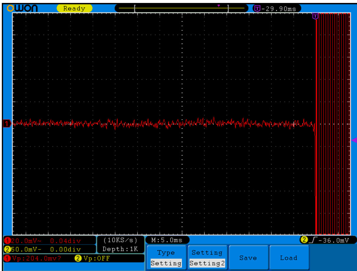
Plot 11-2: Transient Frequency Behavior – 162 MHz; High Power; Narrowband; Carrier OFF Time
