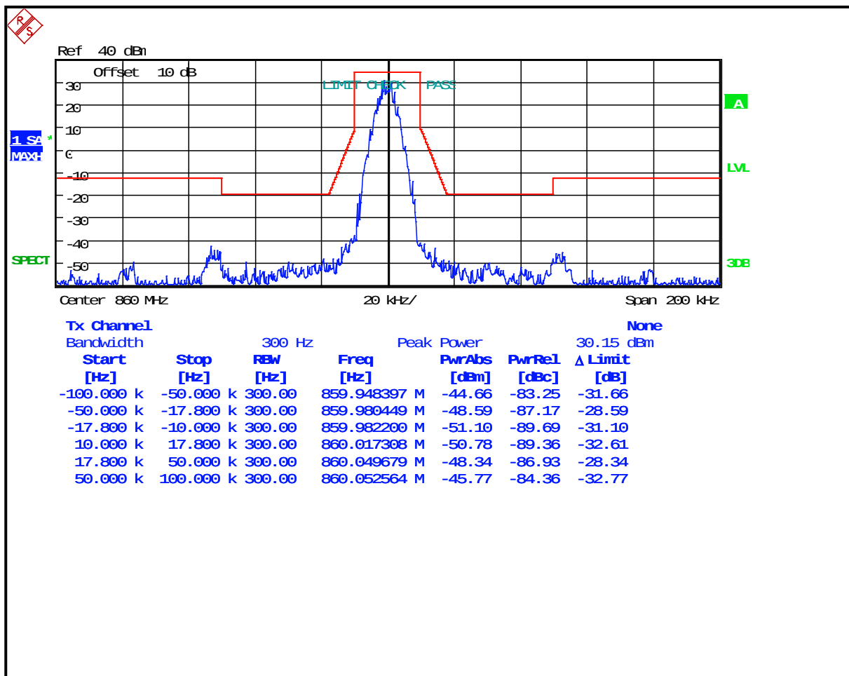
Plot 8-91: Occupied Bandwidth – 860 MHz; P25 RND; Mask G
