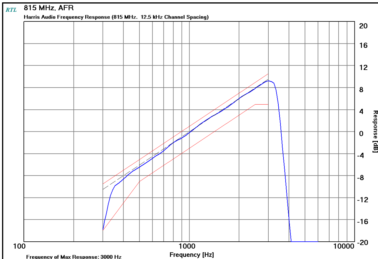
Plot 10-6: Modulation Characteristics - Audio Frequency Response - 815 MHz
