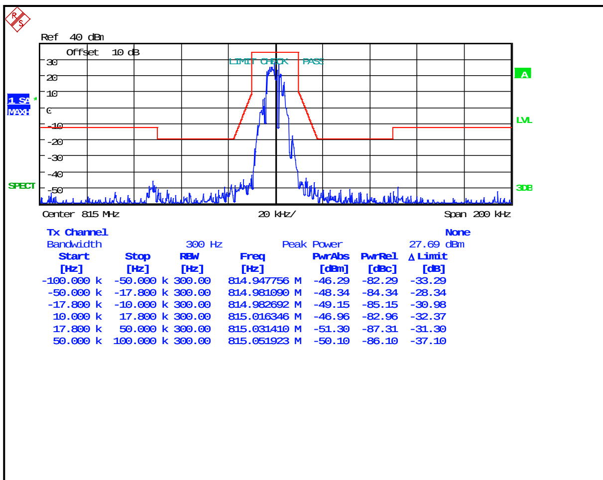
Plot 8-93: Occupied Bandwidth – 815 MHz; CPM TDMA; Mask G
