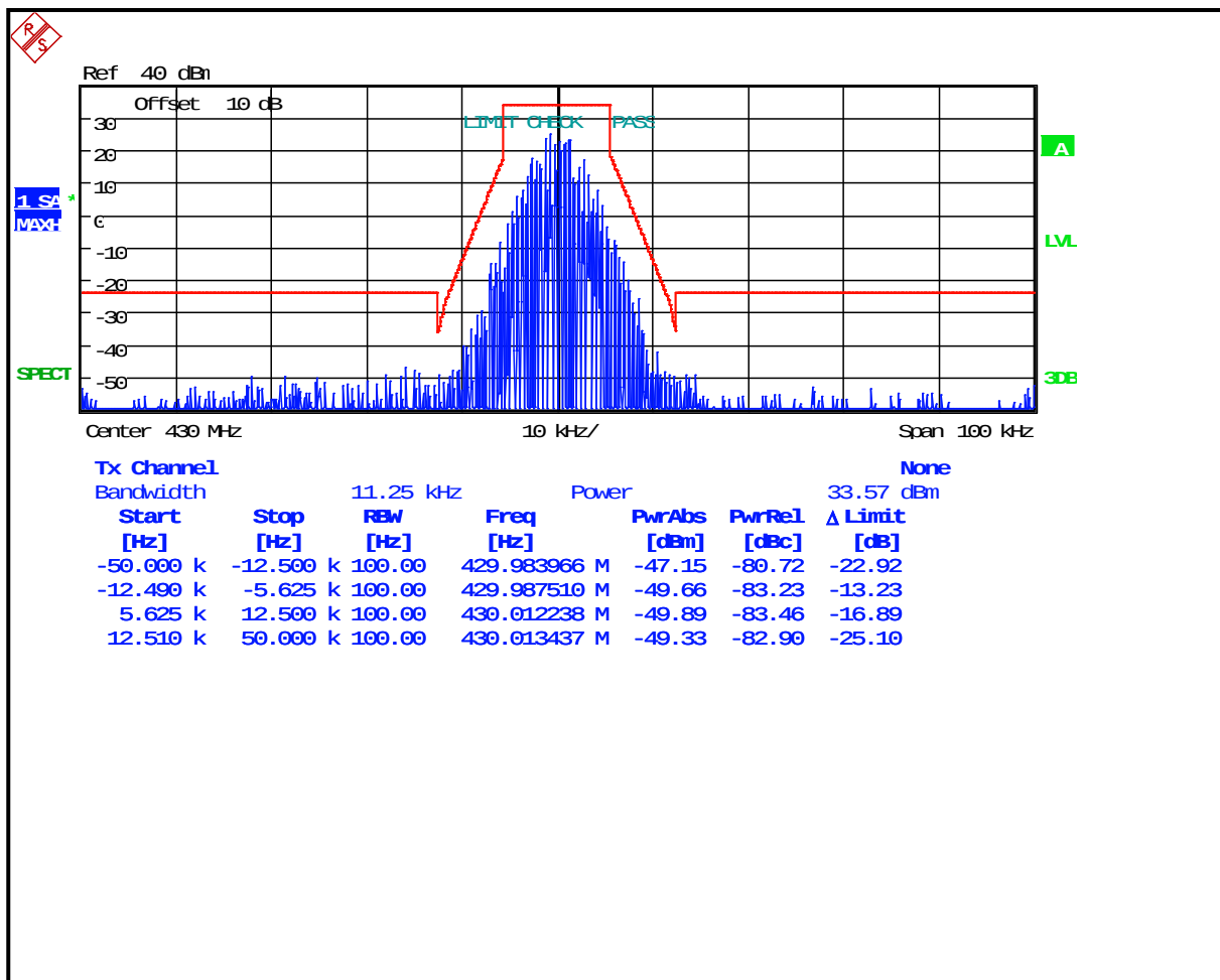
Plot 8-50: Occupied Bandwidth – 430 MHz; CPM TDMA; Mask D
