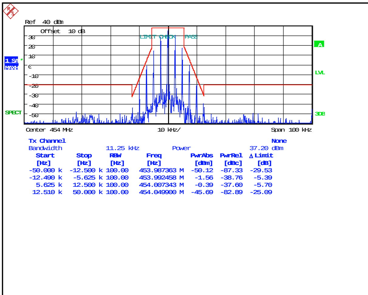
Plot 8-38: Occupied Bandwidth – 454 MHz; Narrowband Analog; Mask D
