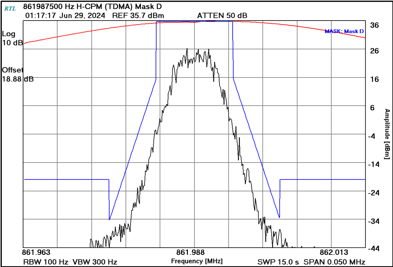
Plot 4-18: Occupied Bandwidth – 861.9875 MHz; H-CPM (TDMA); Mask D
