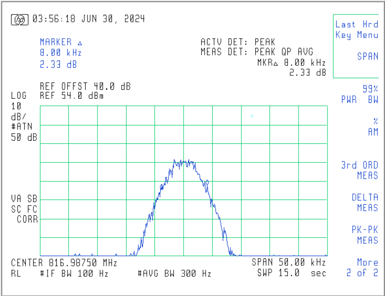
Plot 4-36: OBW 99%, 816.9875 MHz, C4FM
