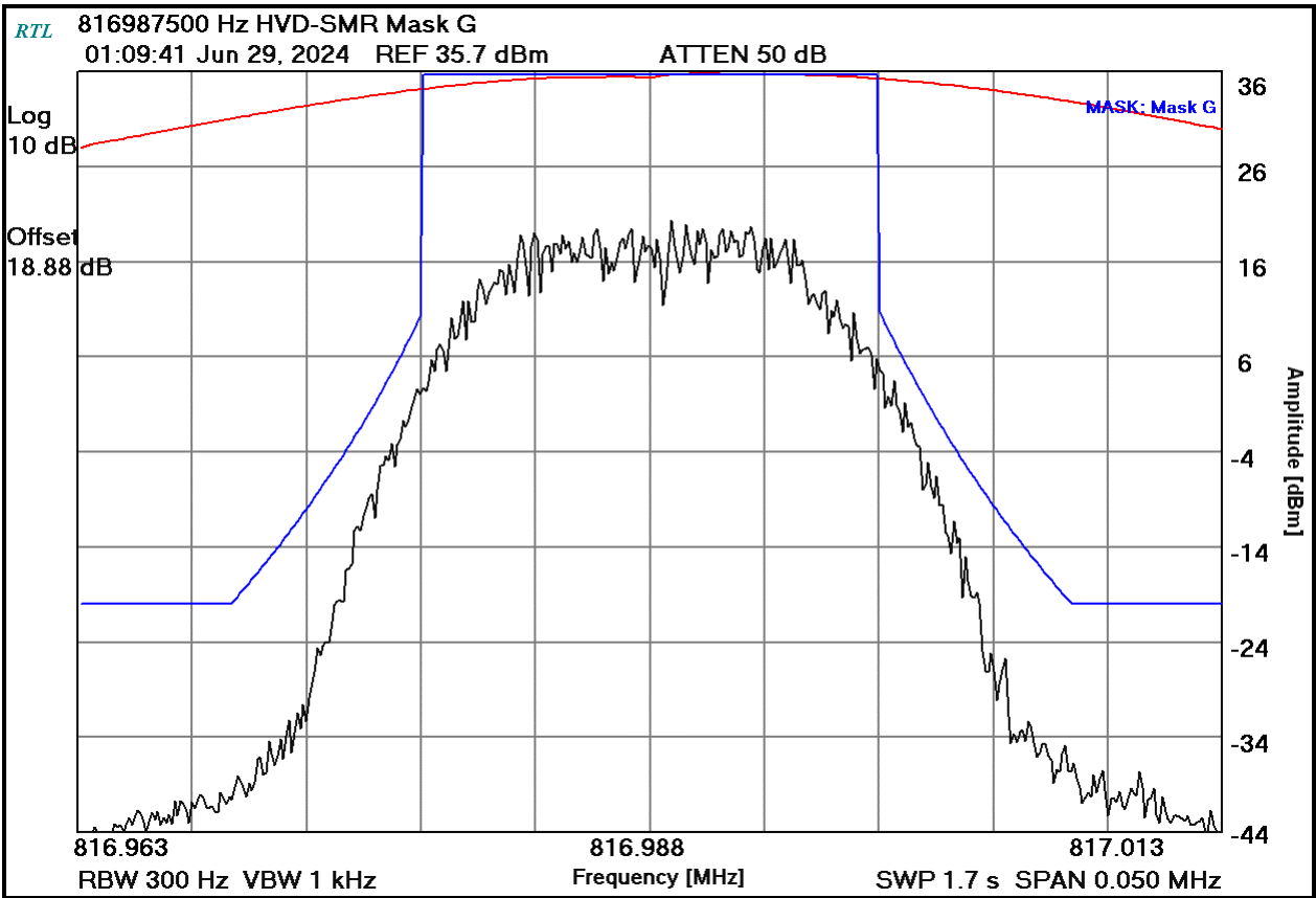
Plot 4-19: Occupied Bandwidth – 816.9875 MHz; HVD-SMR; Mask G
