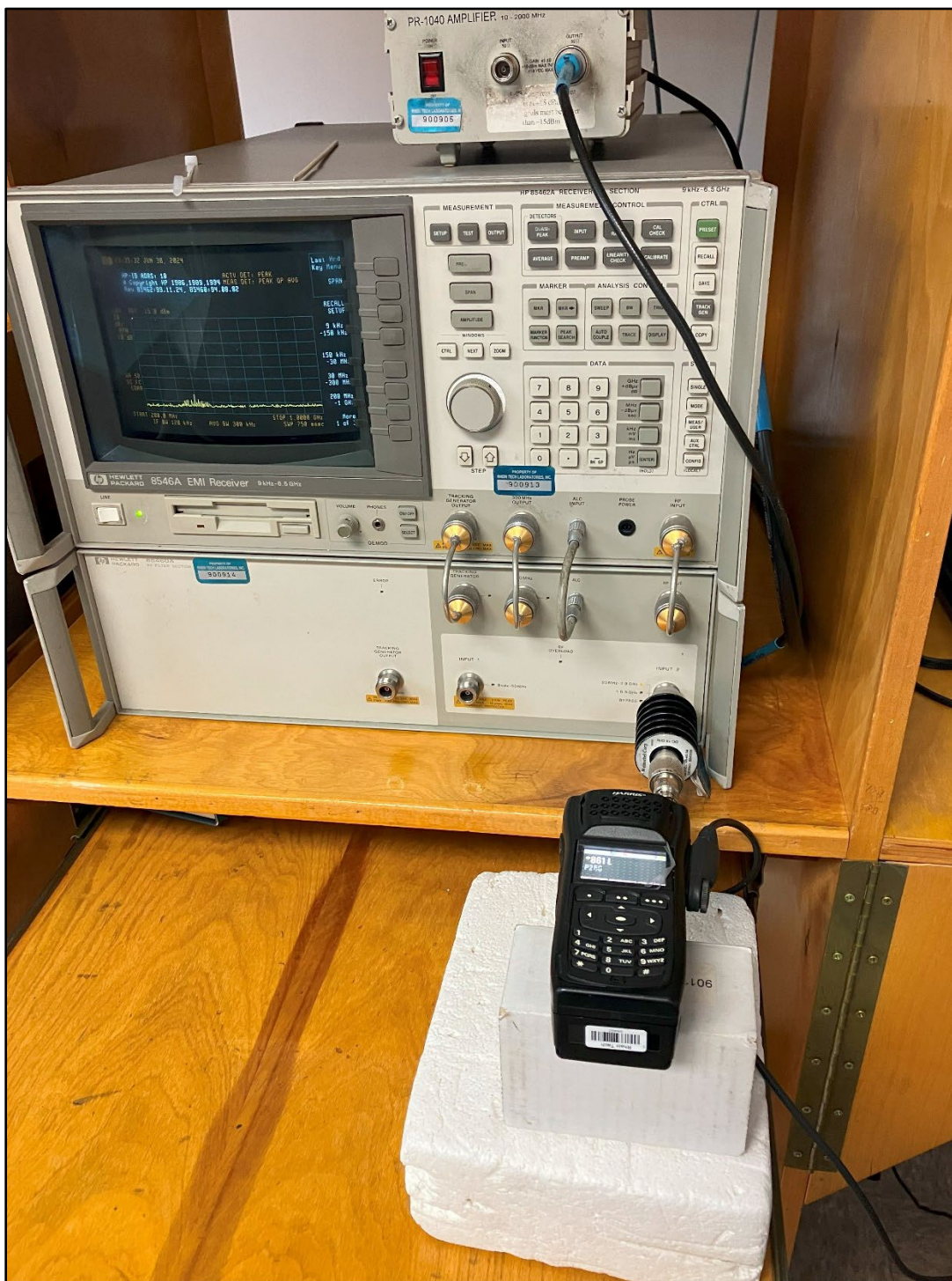
Photograph 5: Conducted Antenna Port Emissions
