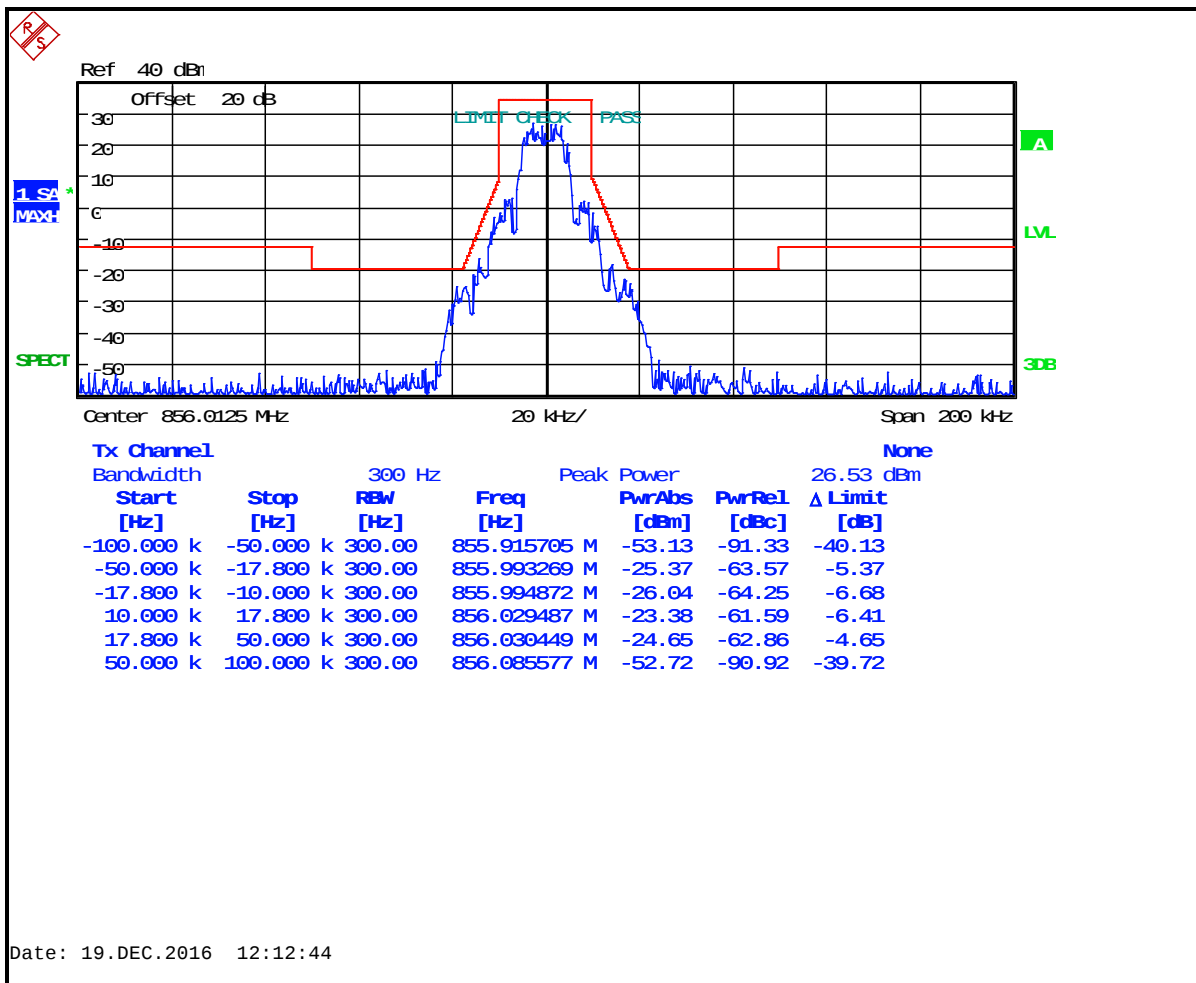
Plot 8-63: Occupied Bandwidth – 856.0125 MHz; WB 2-Level FSK 9600; Mask G
