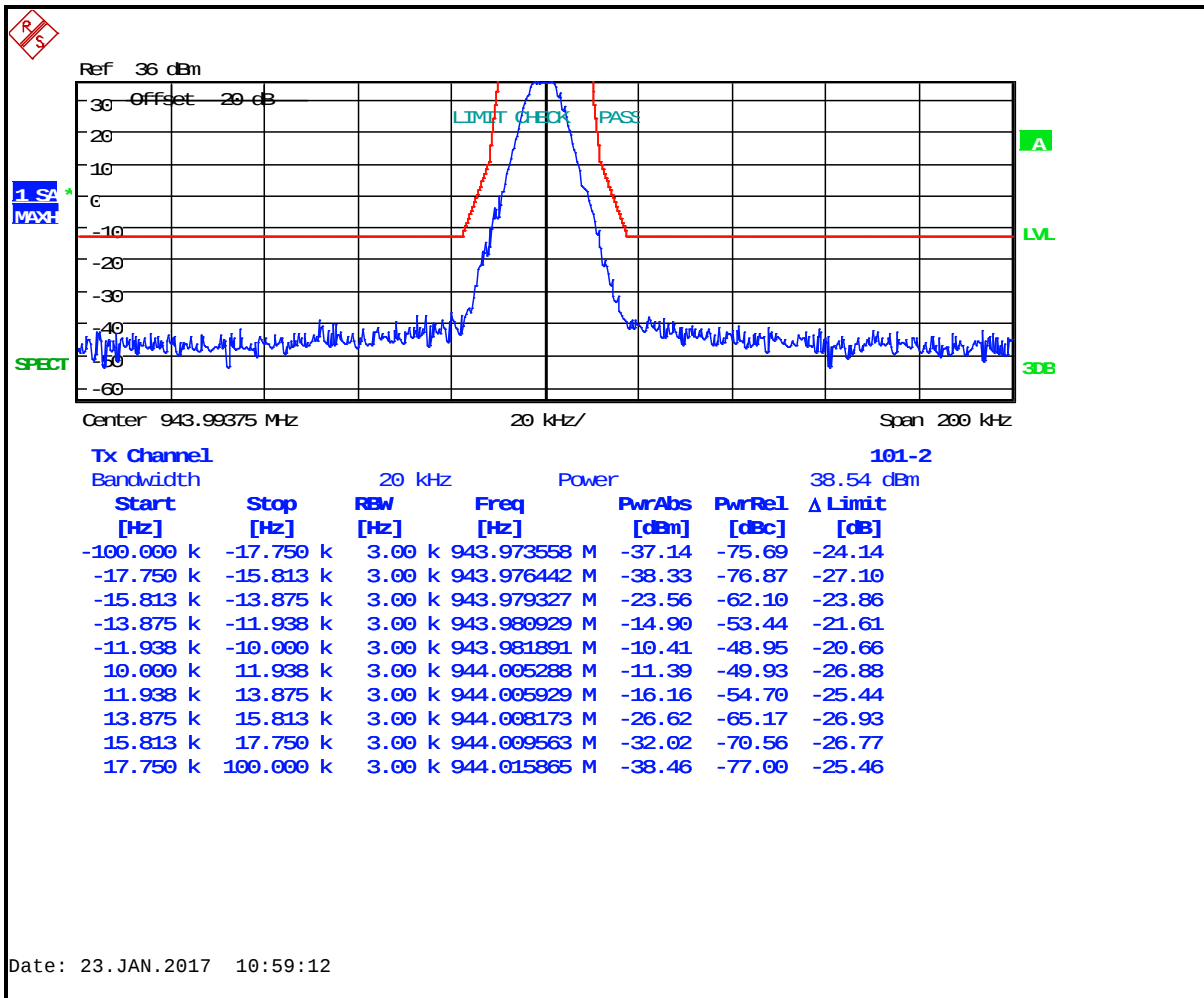
Plot 8-112: Occupied Bandwidth – 943.99375 MHz; 2-Level FSK 9600 NB; Mask 101.111(2)
