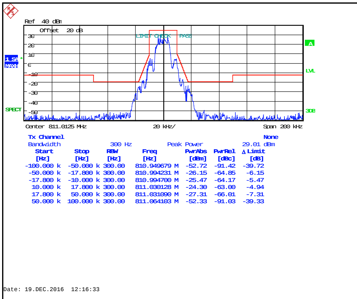
Plot 8-60: Occupied Bandwidth – 811.0125 MHz; WB 2-Level FSK 9600; Mask G
