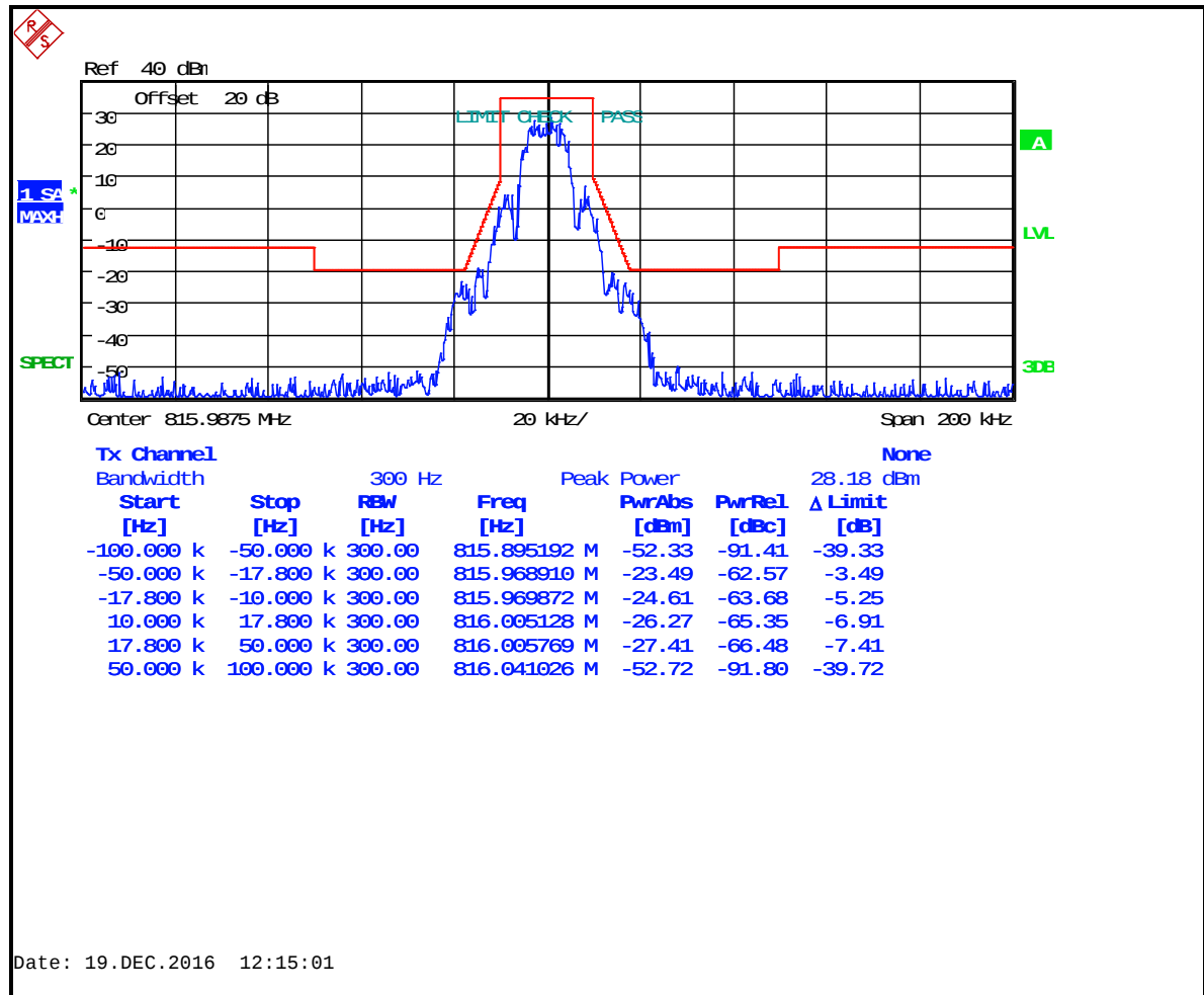
Plot 8-61: Occupied Bandwidth – 815.9875 MHz; WB 2-Level FSK 9600; Mask G
