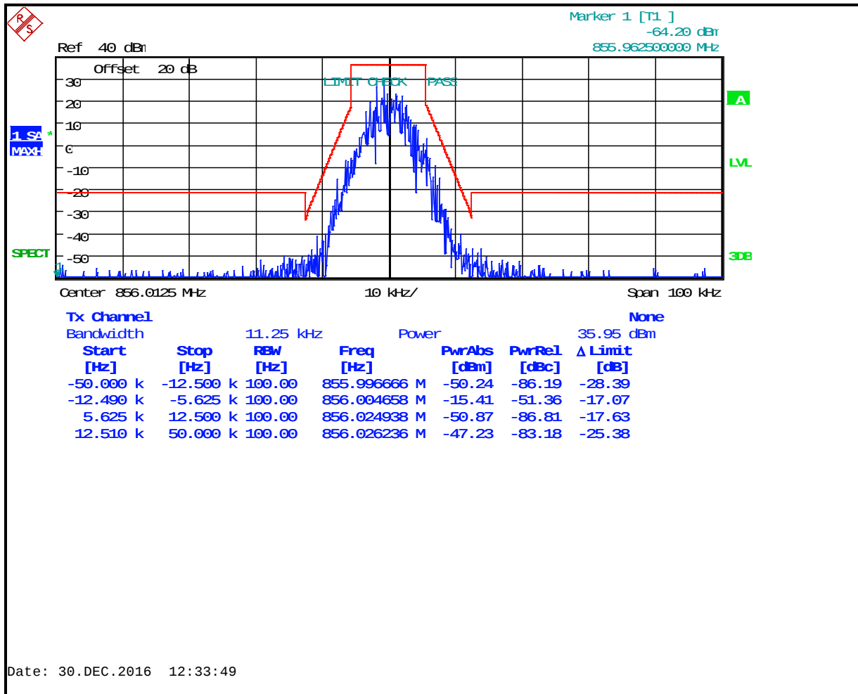
Plot 8-75: Occupied Bandwidth – 856.0125 MHz; P25; Mask D
