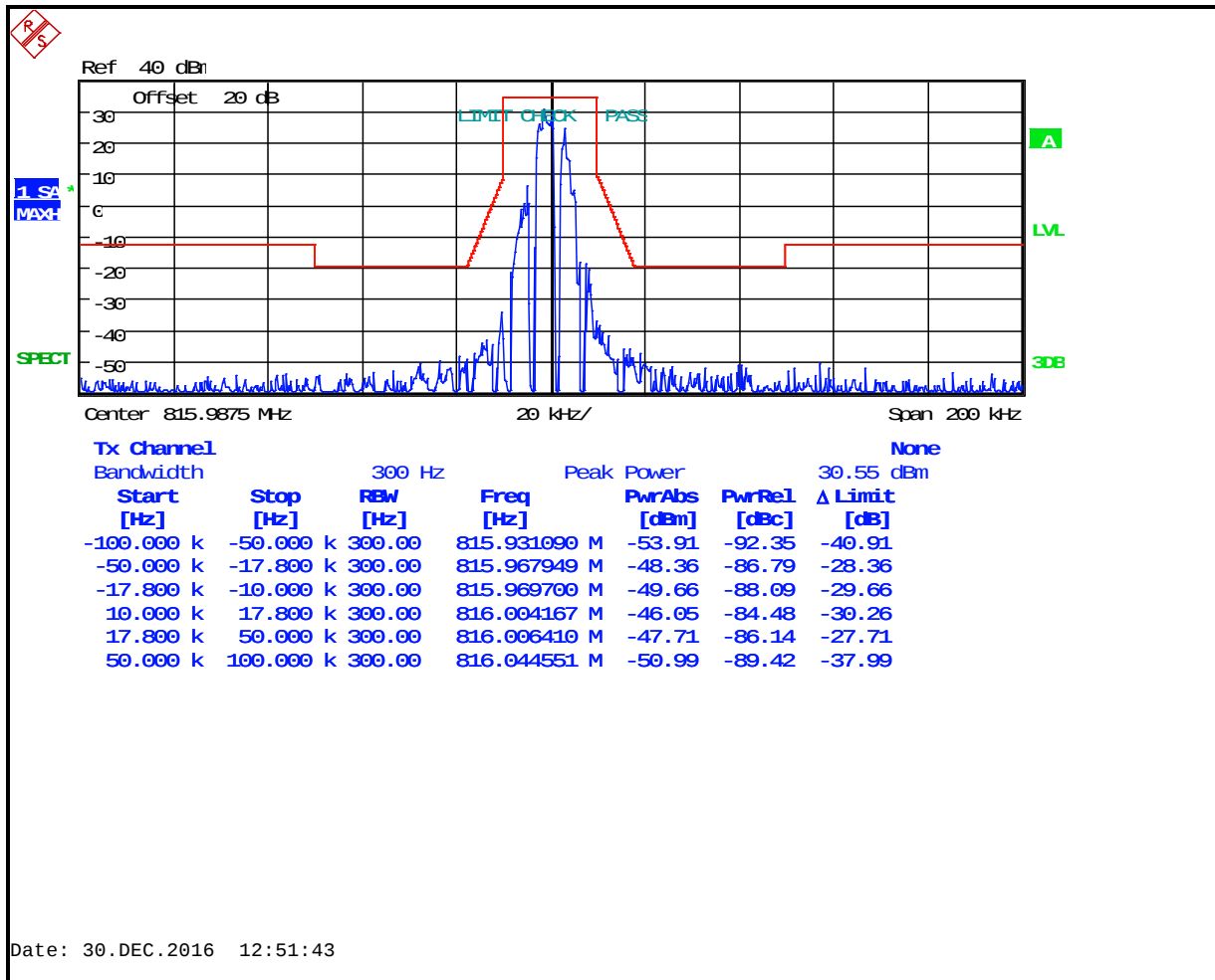
Plot 8-79: Occupied Bandwidth – 815.9875 MHz; P25 Phase 2; Mask G
