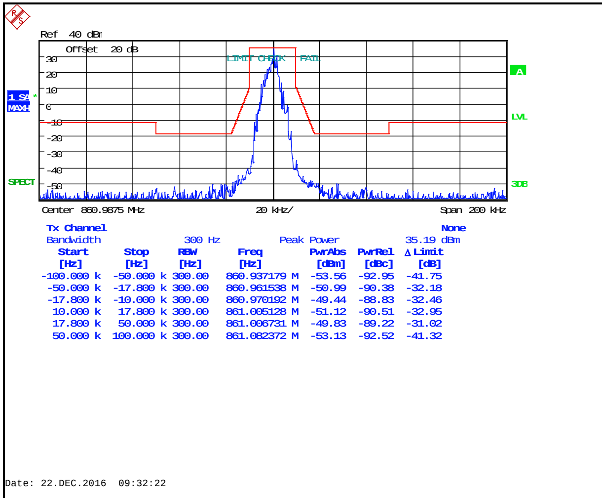
Plot 8-70: Occupied Bandwidth – 860.9875 MHz; P25; Mask G
