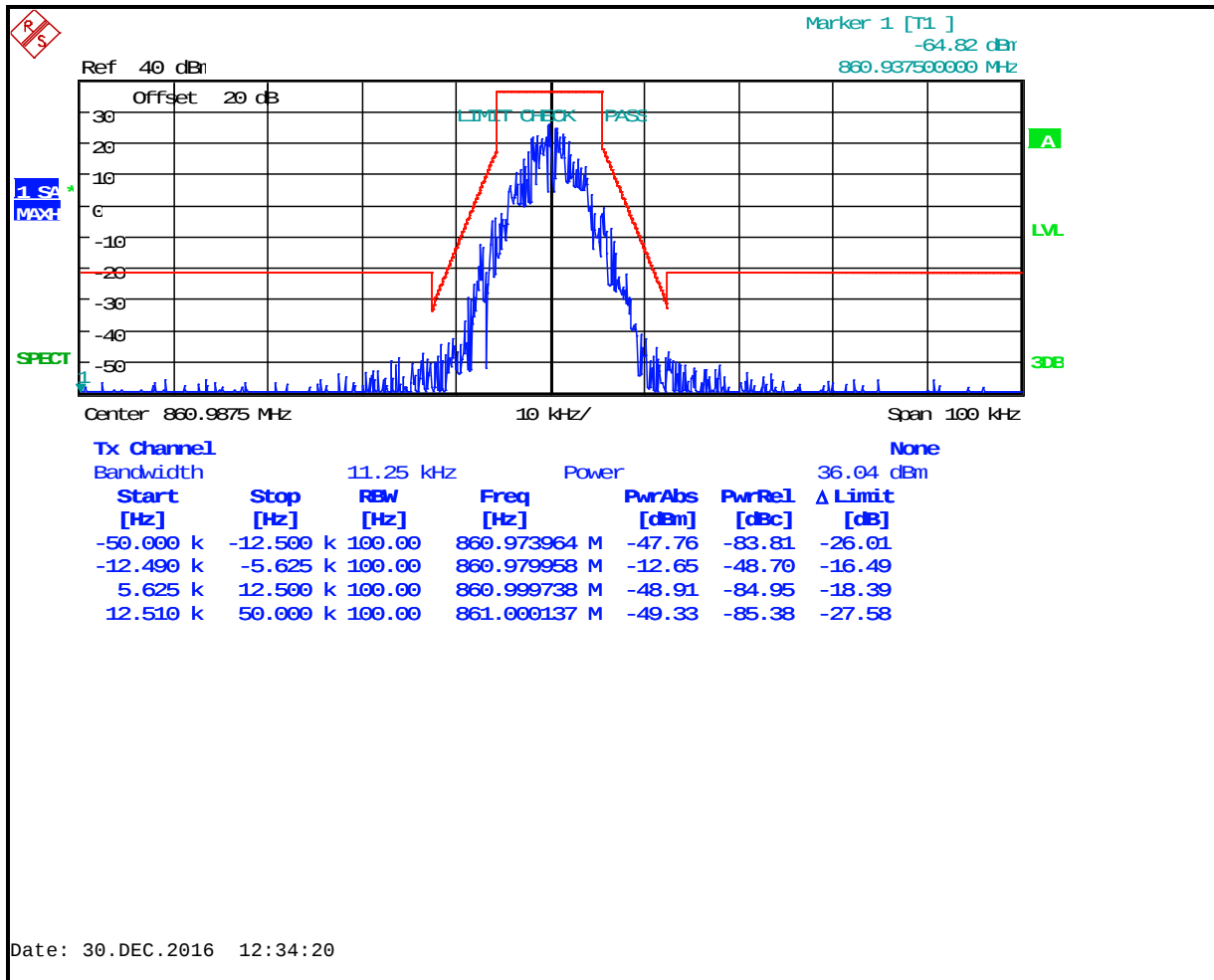
Plot 8-76: Occupied Bandwidth – 860.9875 MHz; P25; Mask D
