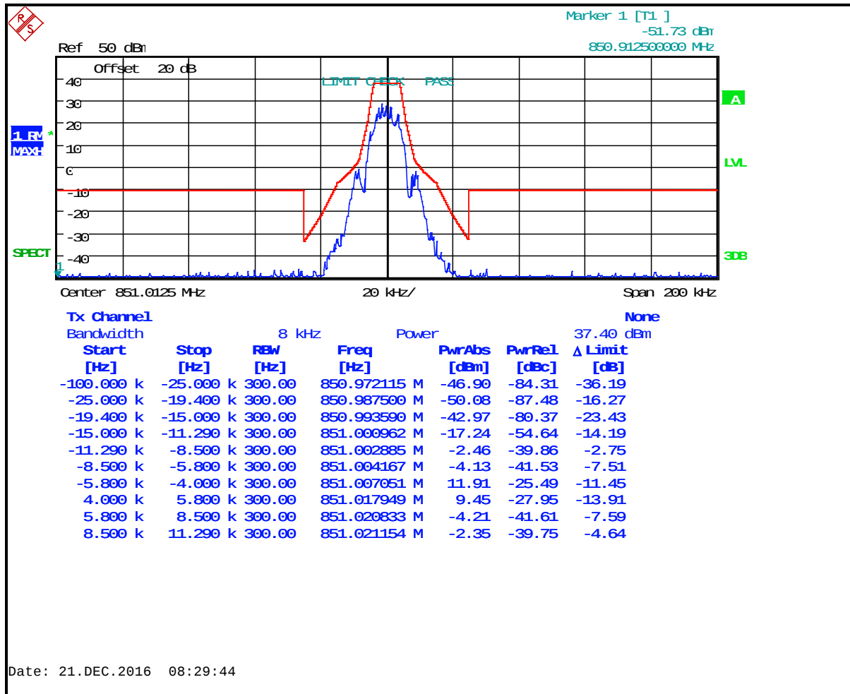
Plot 8-56: Occupied Bandwidth – 851.0125 MHz; 2-Level FSK 9600 NPSPAC; Mask H
