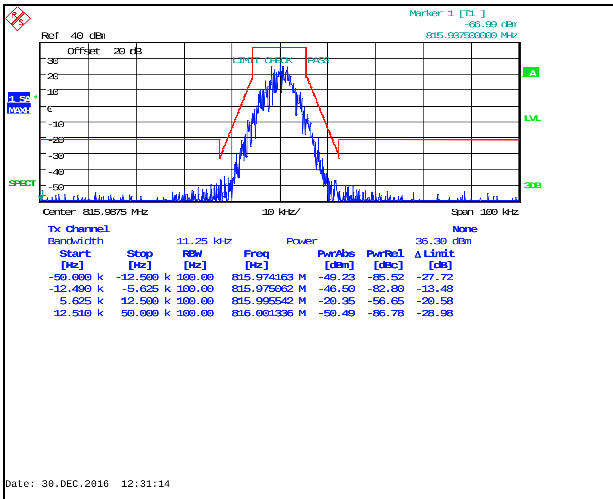
Plot 8-73: Occupied Bandwidth – 815.9875 MHz; P25; Mask D
