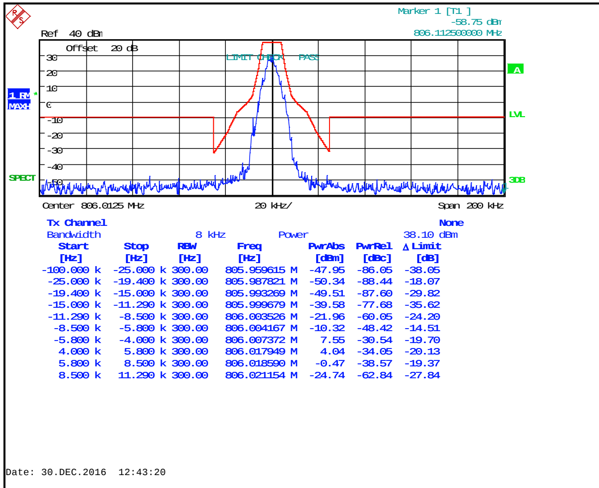
Plot 8-65: Occupied Bandwidth – 806.0125 MHz; P25; Mask H
