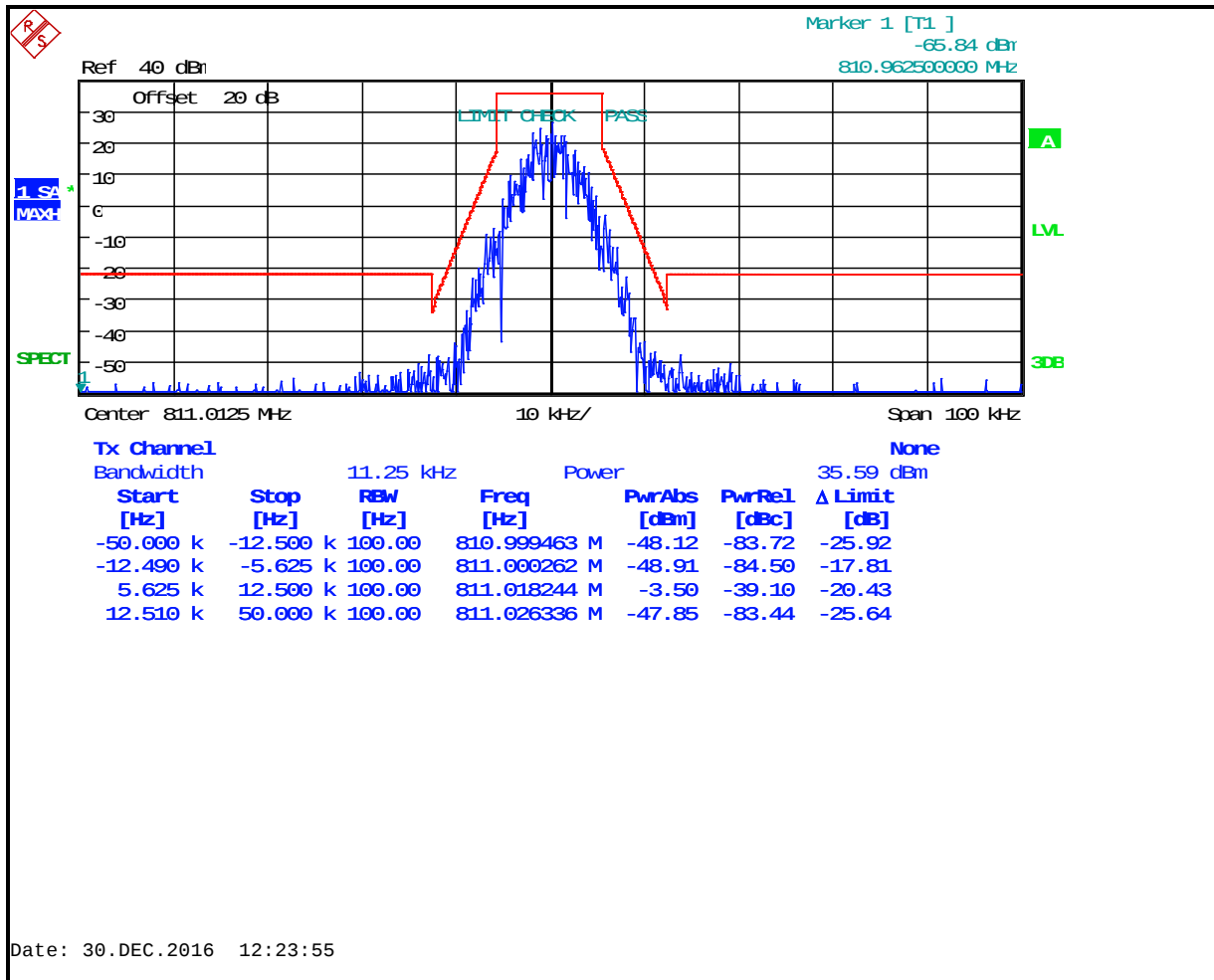
Plot 8-72: Occupied Bandwidth – 811.0125 MHz; P25; Mask D
