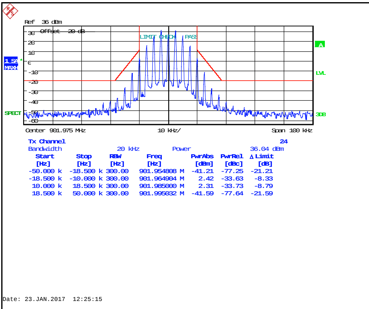
Plot 8-96: Occupied Bandwidth – 901.9750 MHz; WB Analog; Mask 24.133(1)
