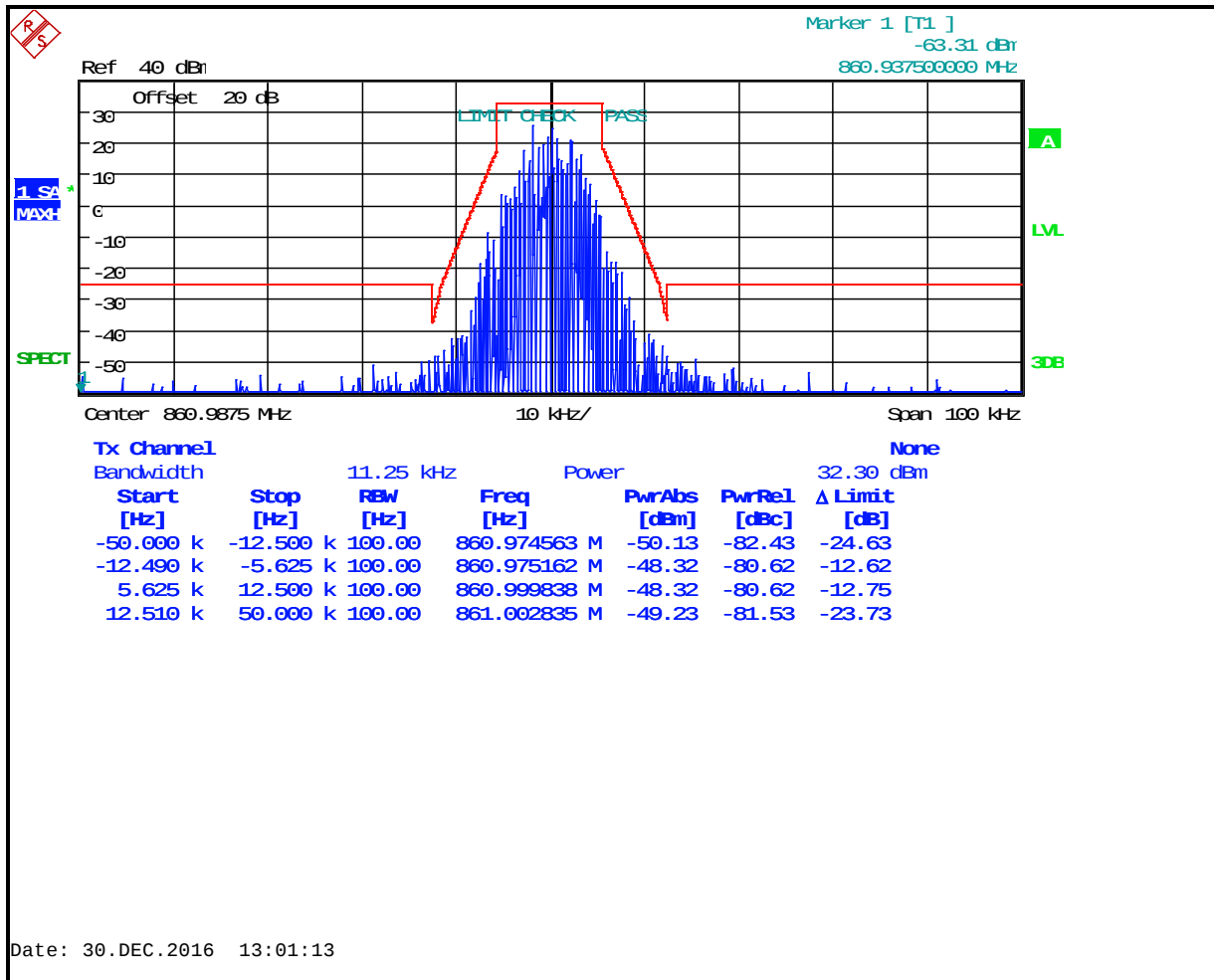
Plot 8-88: Occupied Bandwidth – 860.9875 MHz; P25 Phase 2; Mask D
