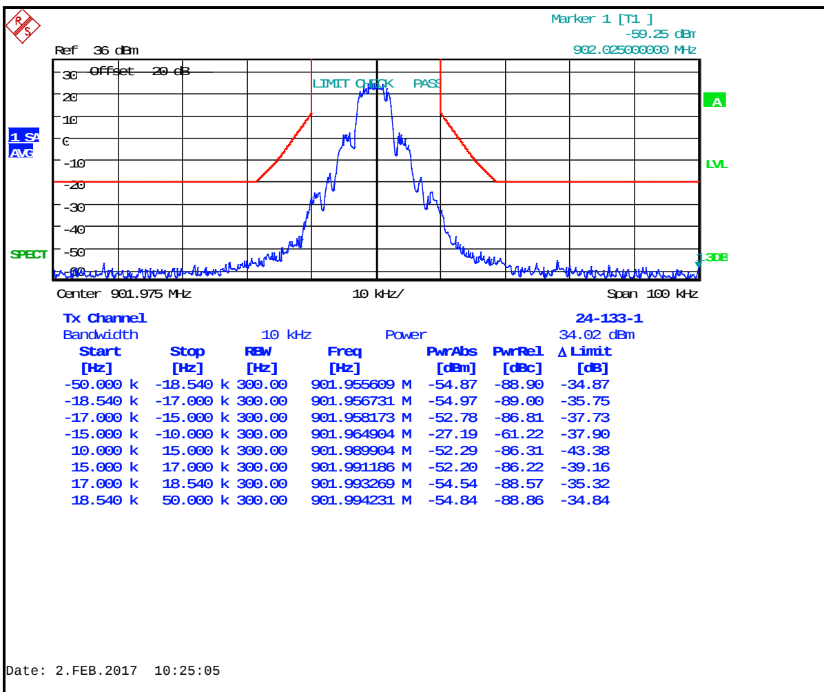
Plot 8-99: Occupied Bandwidth – 901.9750 MHz; 2-Level FSK 4800 XNB; Mask 24.133(1)
