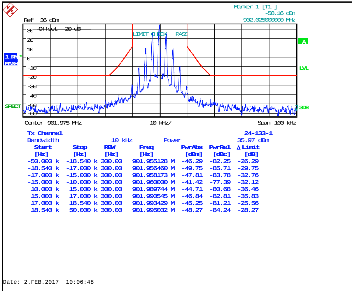
Plot 8-95: Occupied Bandwidth – 901.9750 MHz; NB Analog; Mask 24.133(1)
