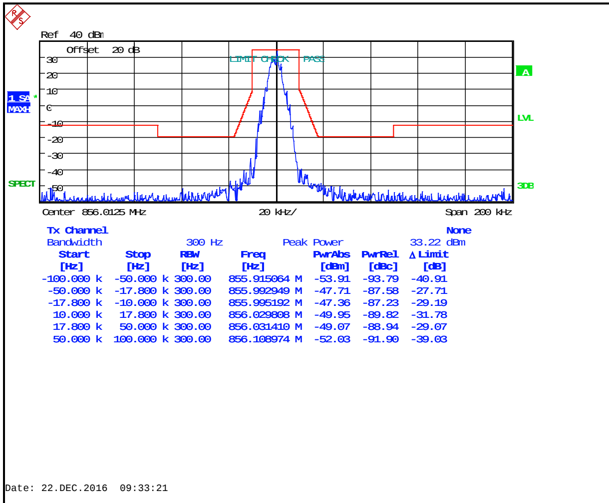
Plot 8-69: Occupied Bandwidth – 856.0125 MHz; P25; Mask G
