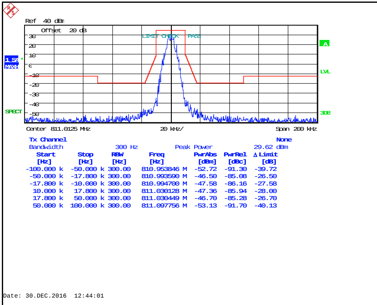
Plot 8-66: Occupied Bandwidth – 811.0125 MHz; P25; Mask G
