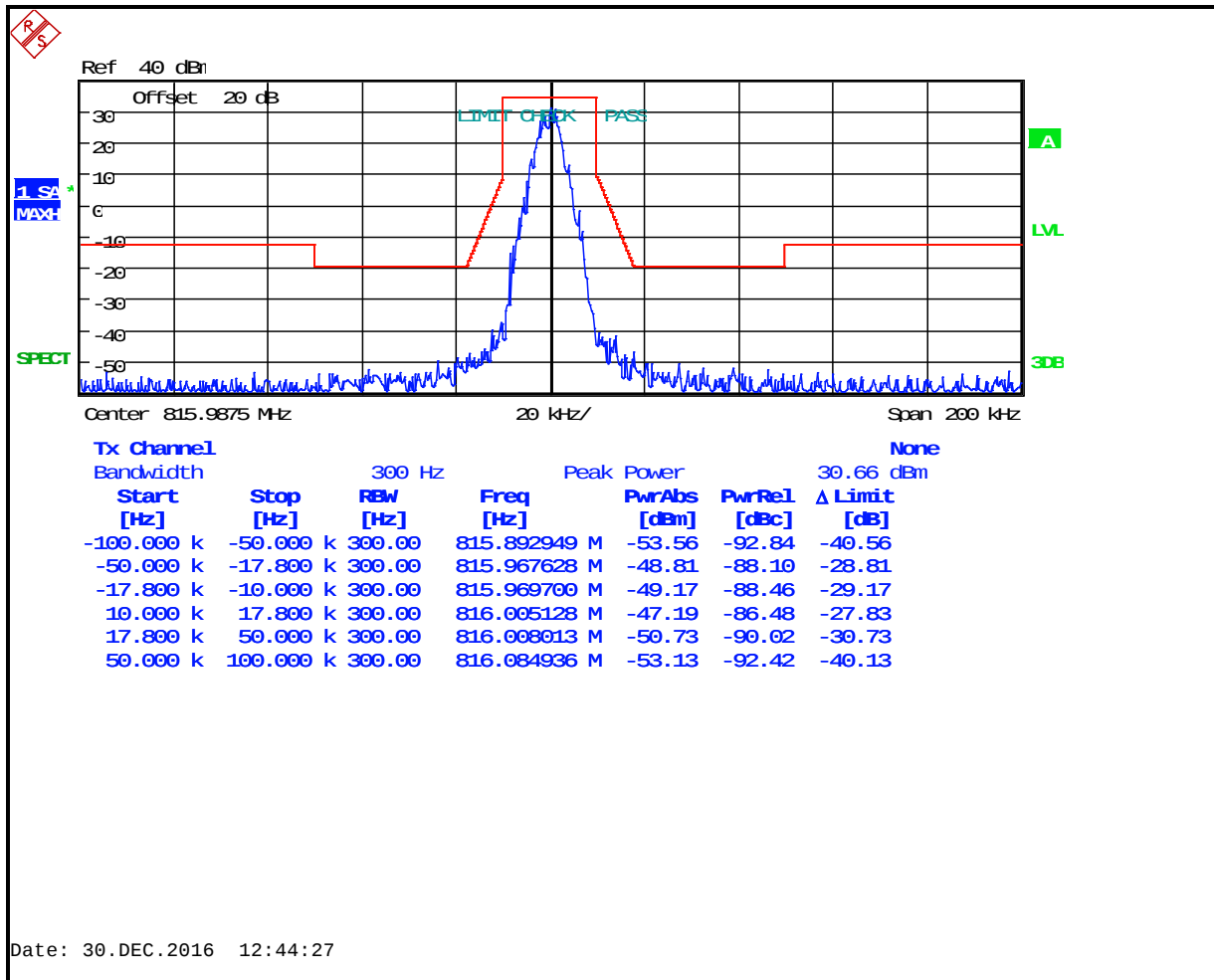
Plot 8-67: Occupied Bandwidth – 815.9875 MHz; P25; Mask G
