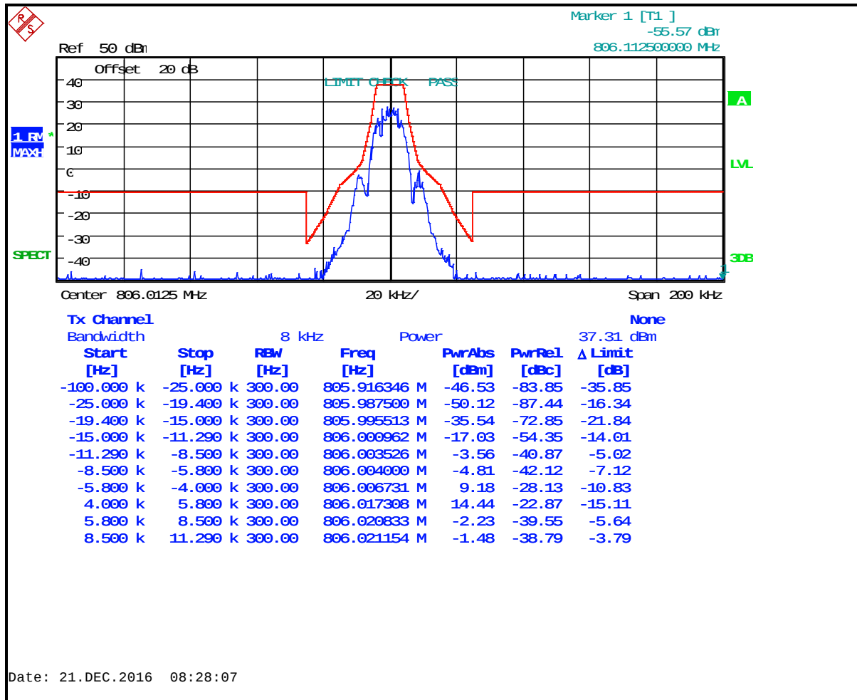
Plot 8-55: Occupied Bandwidth – 806.0125 MHz; 2-Level FSK 9600 NPSPAC; Mask H
