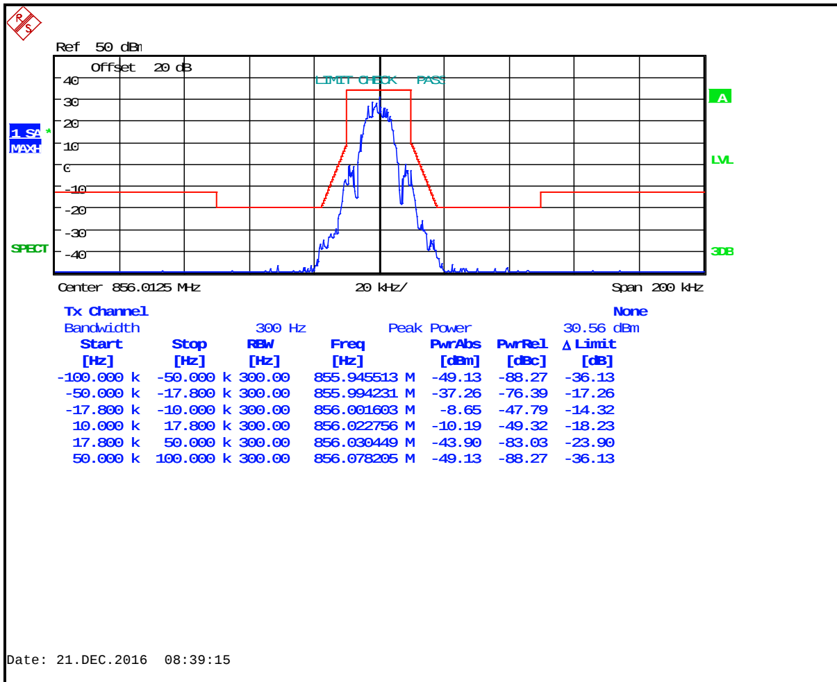
Plot 8-57: Occupied Bandwidth – 856.0125 MHz; 2-Level FSK 9600 NPSPAC; Mask G
