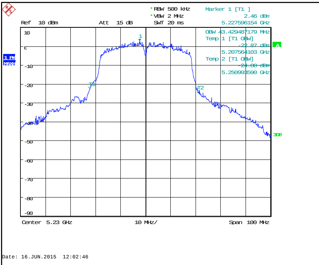
Plot 8-29: 26 dB Bandwidth (Frequency 5230 MHz) - 802.11a (40 MHz BW, 36 Mbps)
