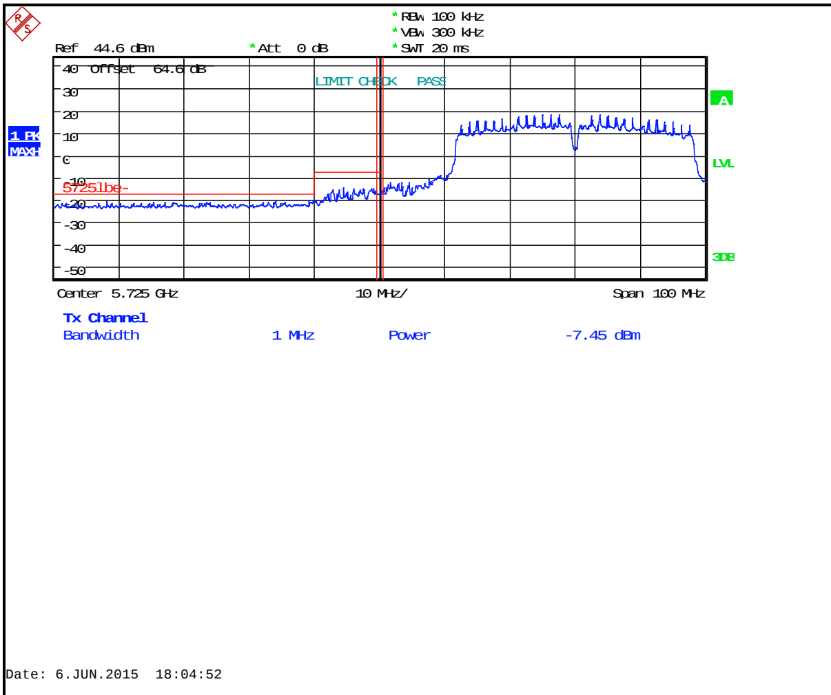
Plot 6-37: Lower Band Edge: Measurement Channel 149 (5745 MHz, 40 MHz BW, 802.11a, Peak)
