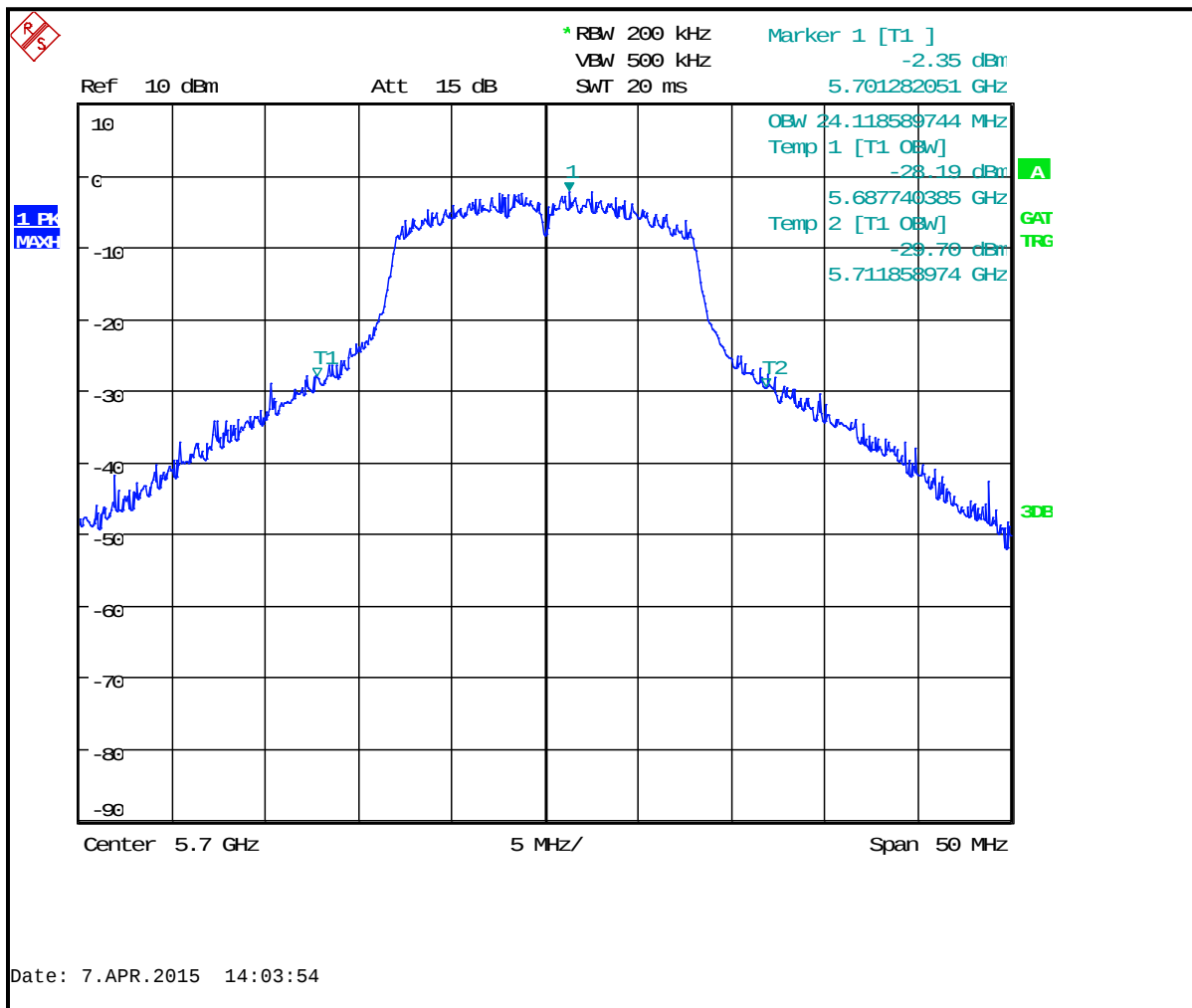
Plot 8-23: 26 dB Bandwidth Channel 140 (TX Frequency 5700 MHz) - 802.11n
