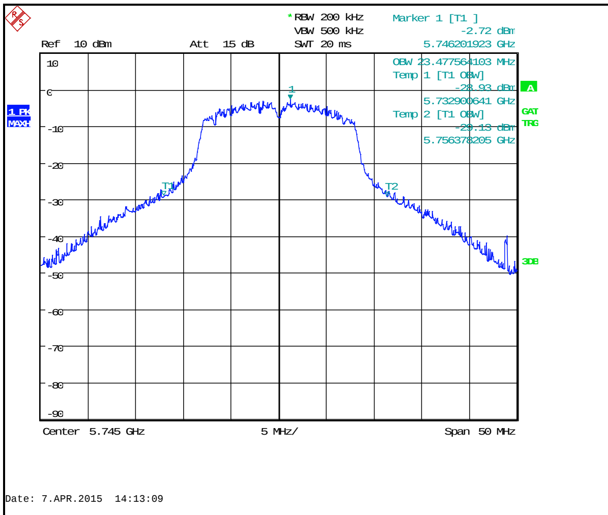
Plot 8-24: 26 dB Bandwidth Channel 149 (TX Frequency 5745 MHz) - 802.11n
