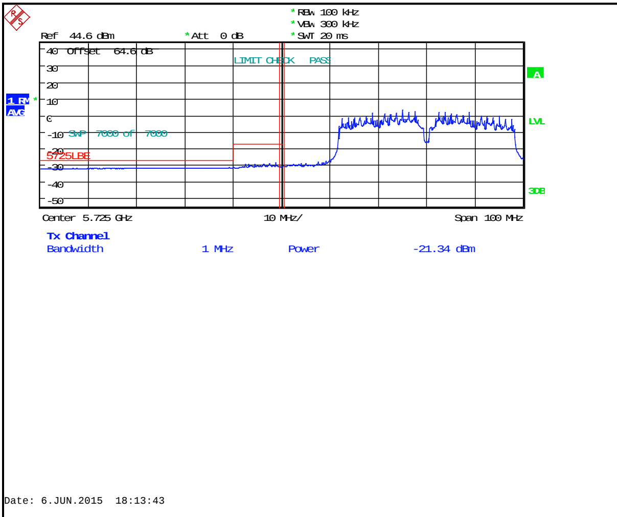
Plot 6-40: Lower Band Edge: Measurement Channel 149 (5745 MHz, 40 MHz BW, 802.11n, Average)
