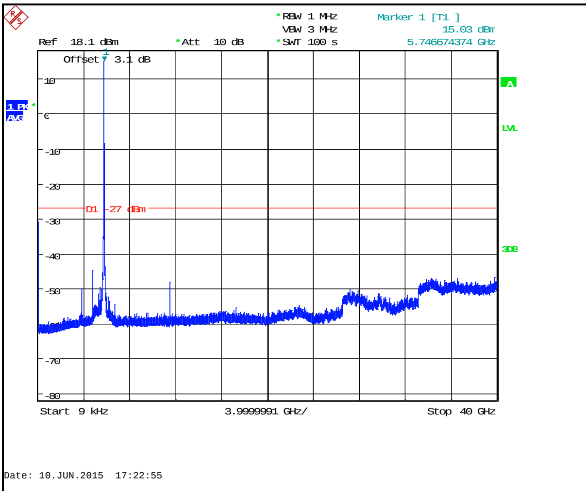
Plot 7-13: Undesirable Emissions Channel 149 (5745 MHz)
