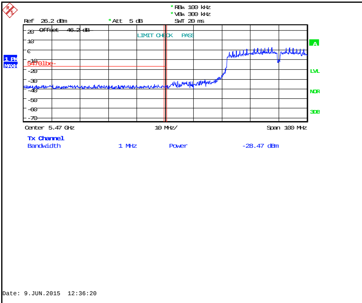
Plot 6-23: Lower Band Edge: Measurement Channel 100 (5500 MHz, 40 MHz BW, 802.11n, Peak)
