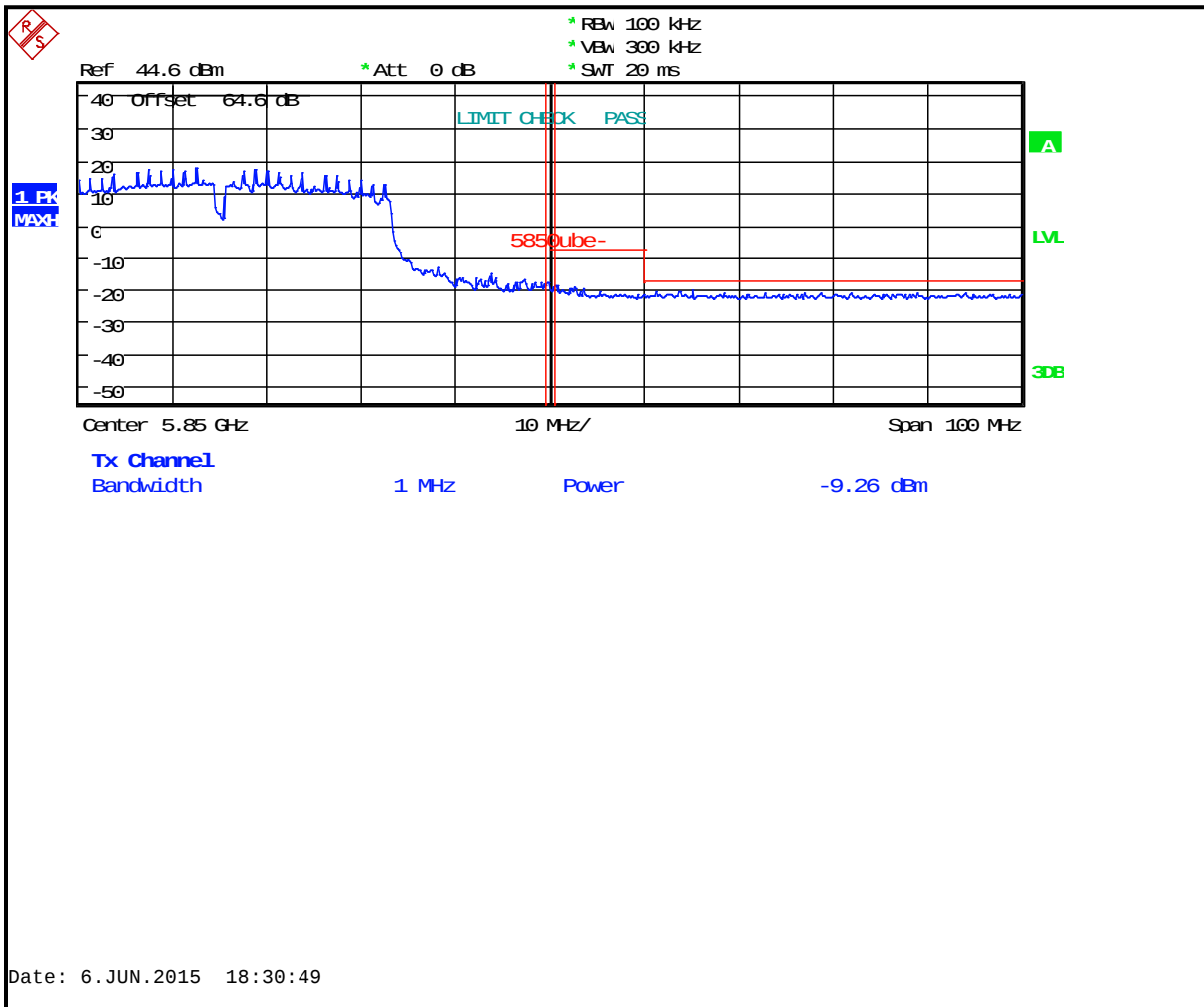
Plot 6-47: Upper Band Edge: Measurement Channel 165 (5825 MHz, 40 MHz BW, 802.11n, Peak)
