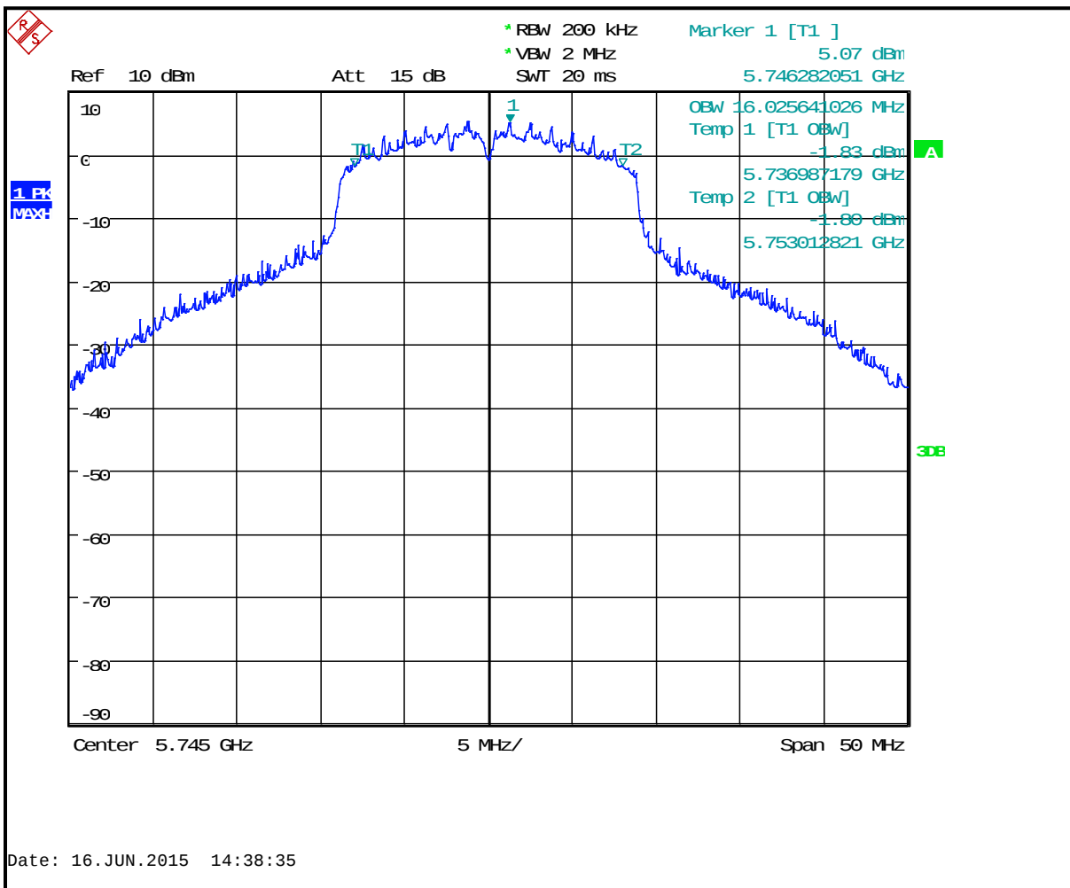
Plot 8-53: 6 dB Bandwidth Channel 149 (TX Frequency 5745 MHz) - 802.11a
