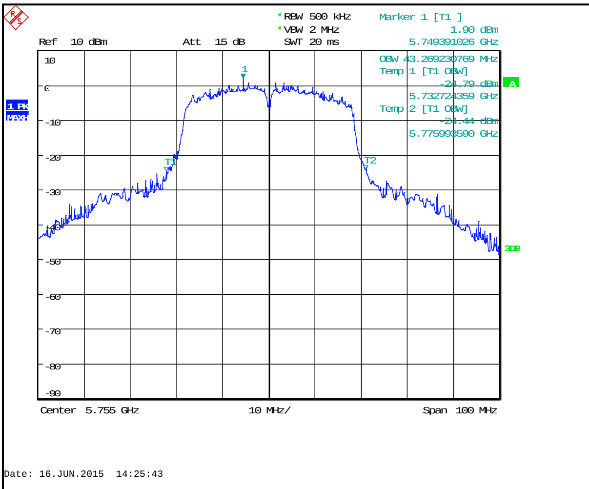
Plot 8-50: 26 dB Bandwidth (Frequency 5755 MHz) - 802.11n (40 MHz BW)
