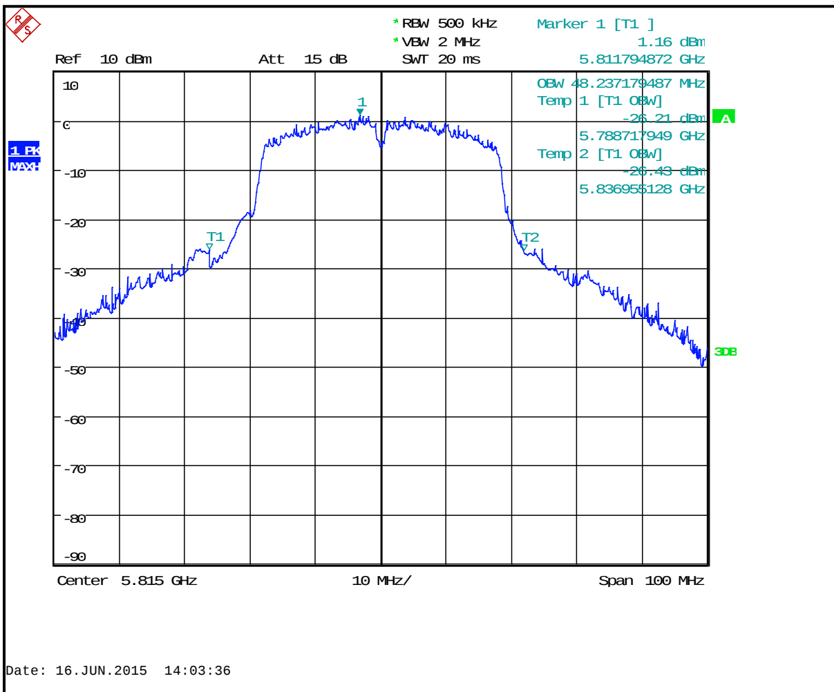
Plot 8-39: 26 dB Bandwidth (Frequency 5815 MHz) - 802.11a (40 MHz BW, 36 Mbps)
