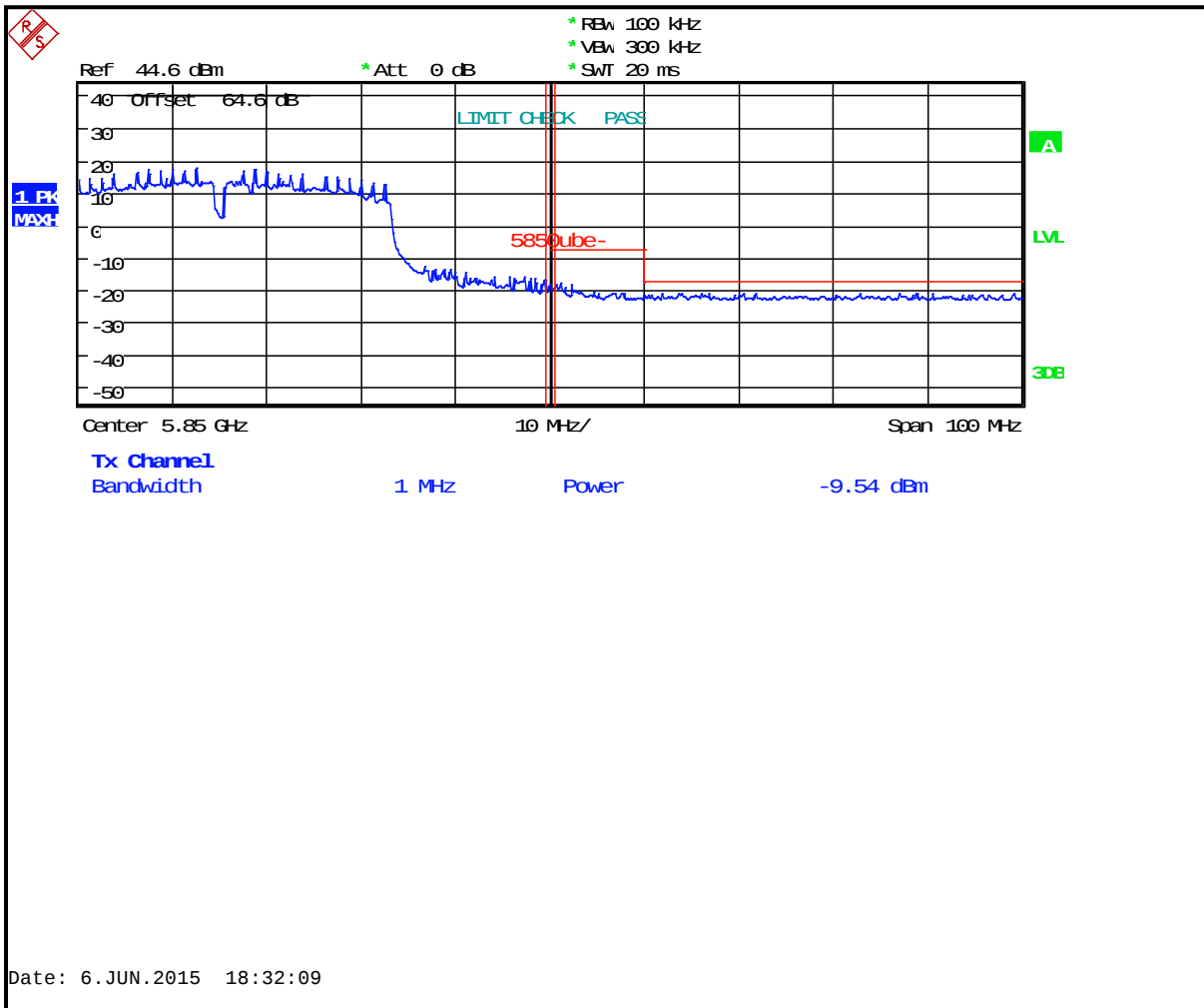
Plot 6-45: Upper Band Edge: Measurement Channel 165 (5825 MHz, 40 MHz BW, 802.11a, Peak)
