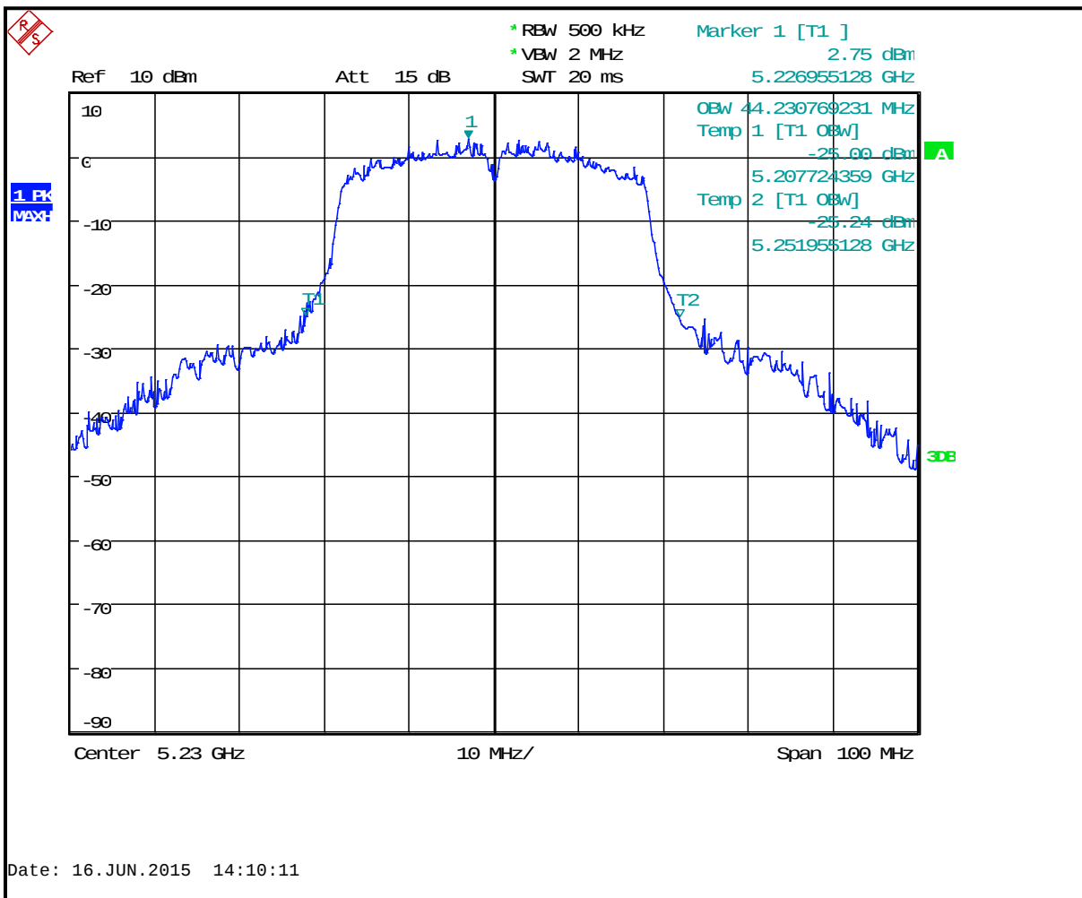
Plot 8-42: 26 dB Bandwidth (Frequency 5230 MHz) - 802.11n (40 MHz BW)
