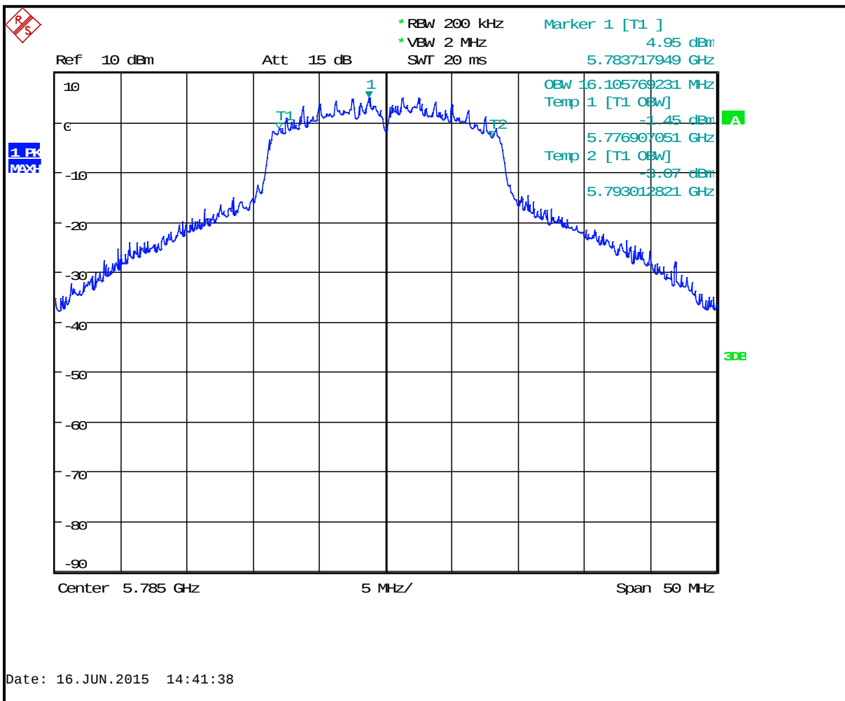
Plot 8-54: 6 dB Bandwidth Channel 157 (TX Frequency 5785 MHz) - 802.11a
