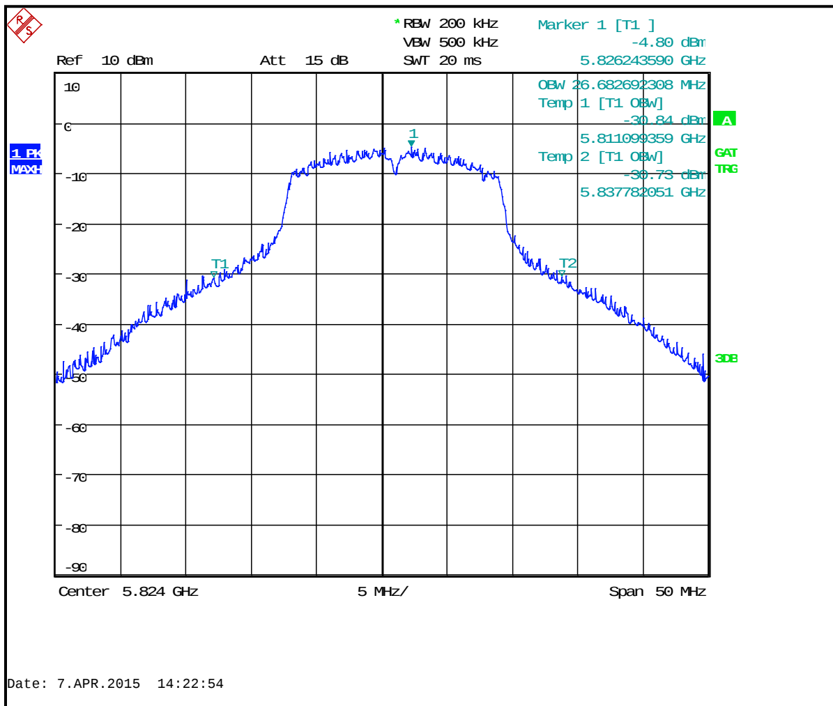
Plot 8-26: 26 dB Bandwidth Channel 165 (TX Frequency 5825 MHz) - 802.11n
