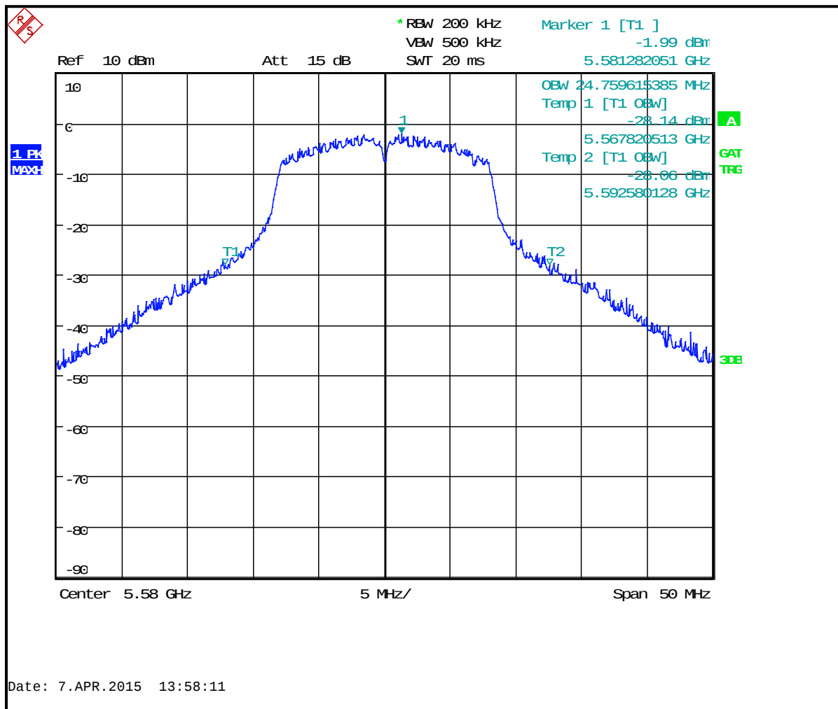
Plot 8-22: 26 dB Bandwidth Channel 116 (TX Frequency 5580 MHz) - 802.11n
