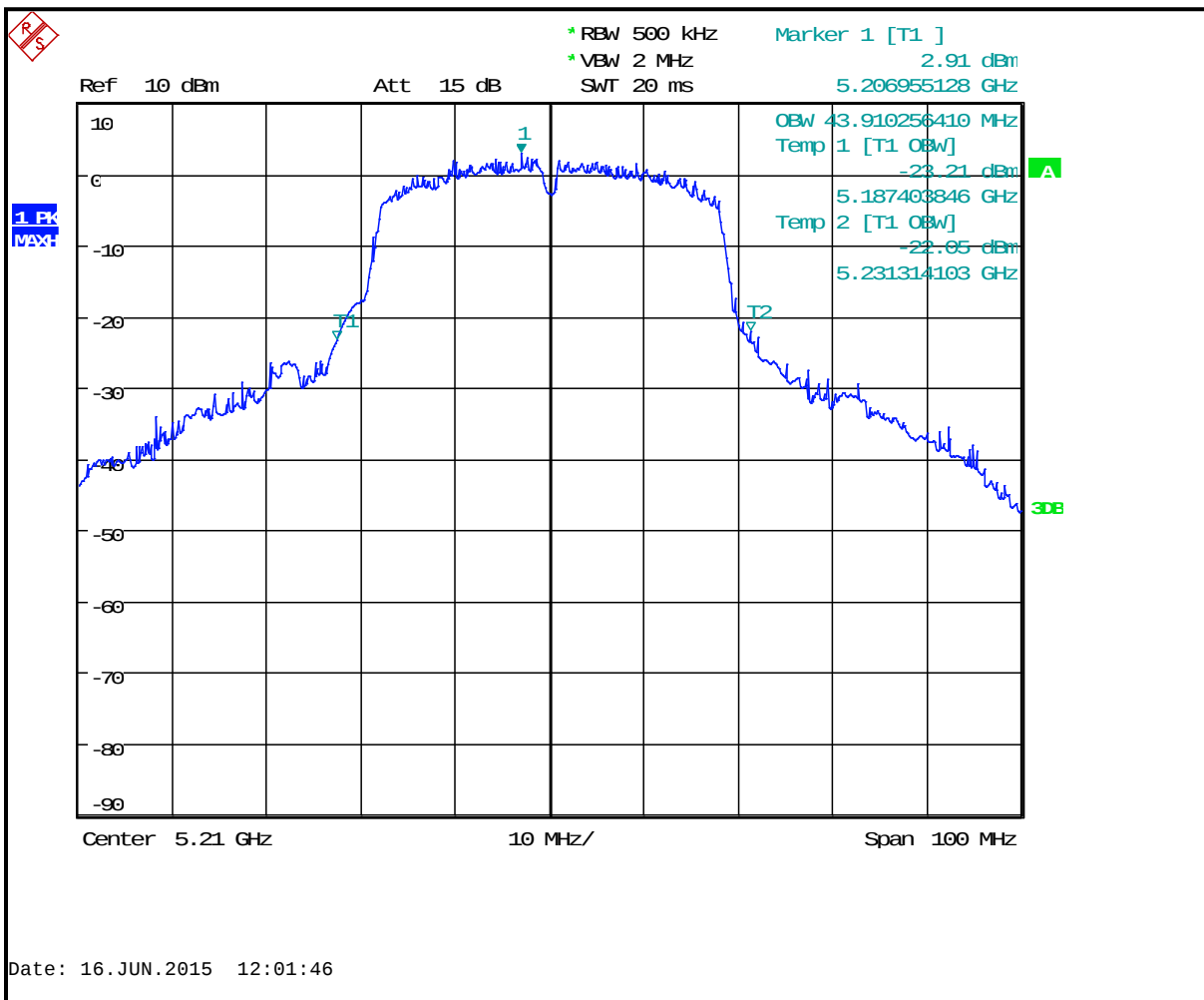
Plot 8-28: 26 dB Bandwidth (Frequency 5210 MHz) - 802.11a (40 MHz BW, 36 Mbps)
