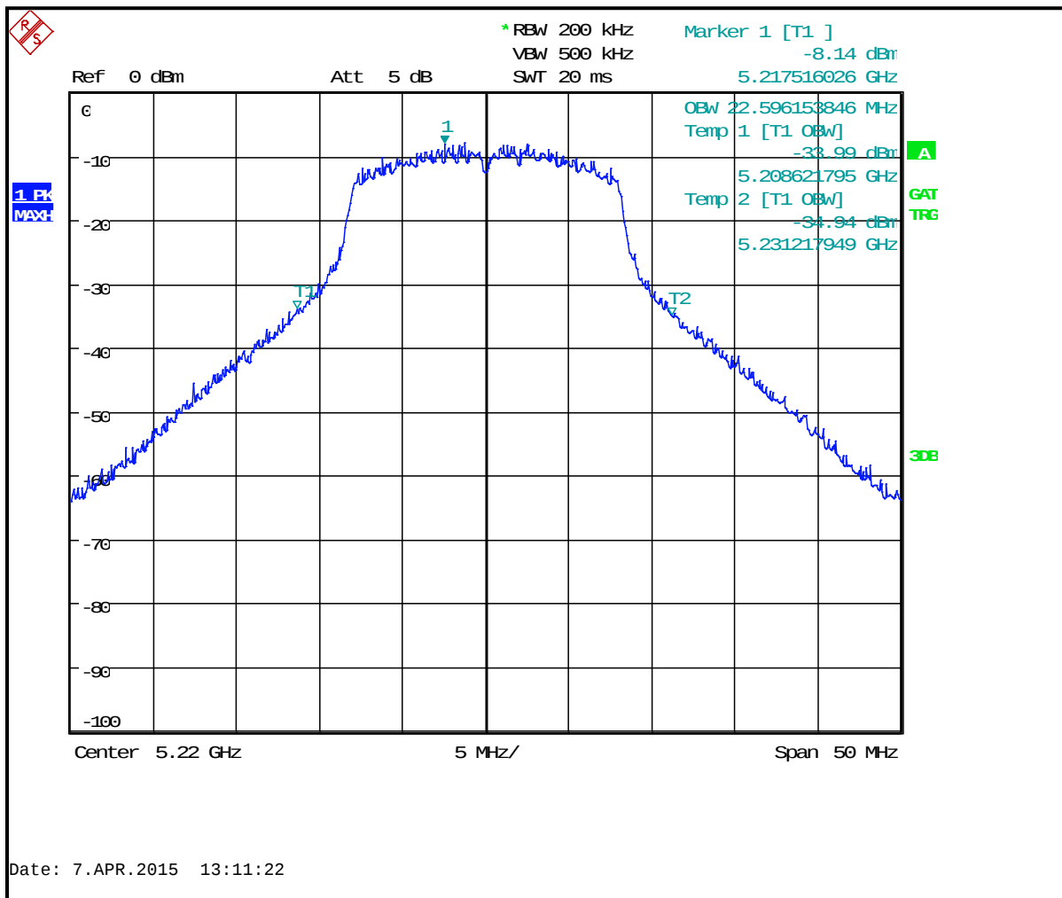
Plot 8-16: 26 dB Bandwidth Channel 44 (TX Frequency 5220 MHz) - 802.11n
