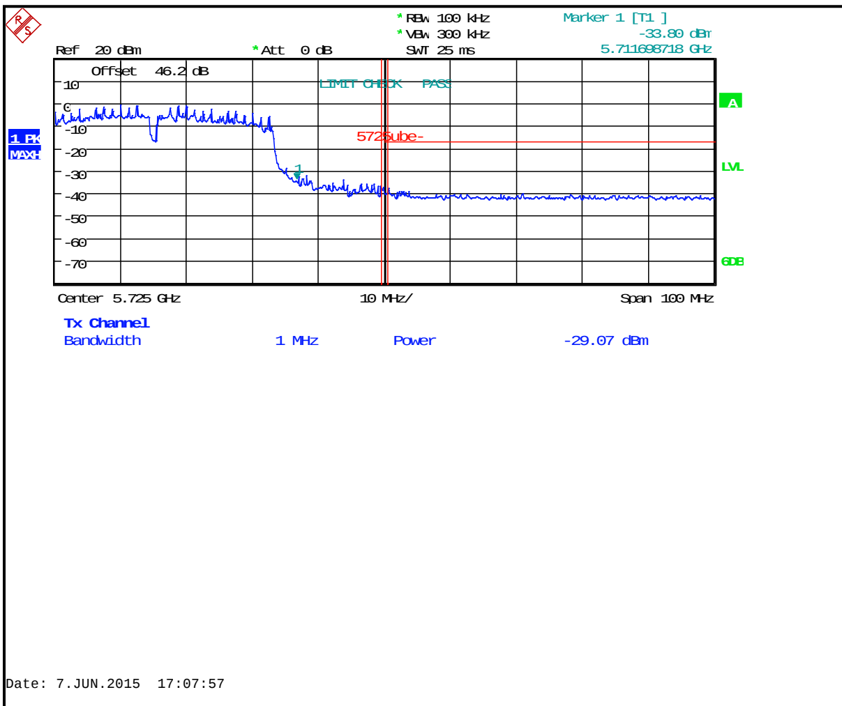
Plot 6-31: Upper Band Edge: Measurement Channel 140 (5700 MHz, 40 MHz BW, 802.11n, Peak)
