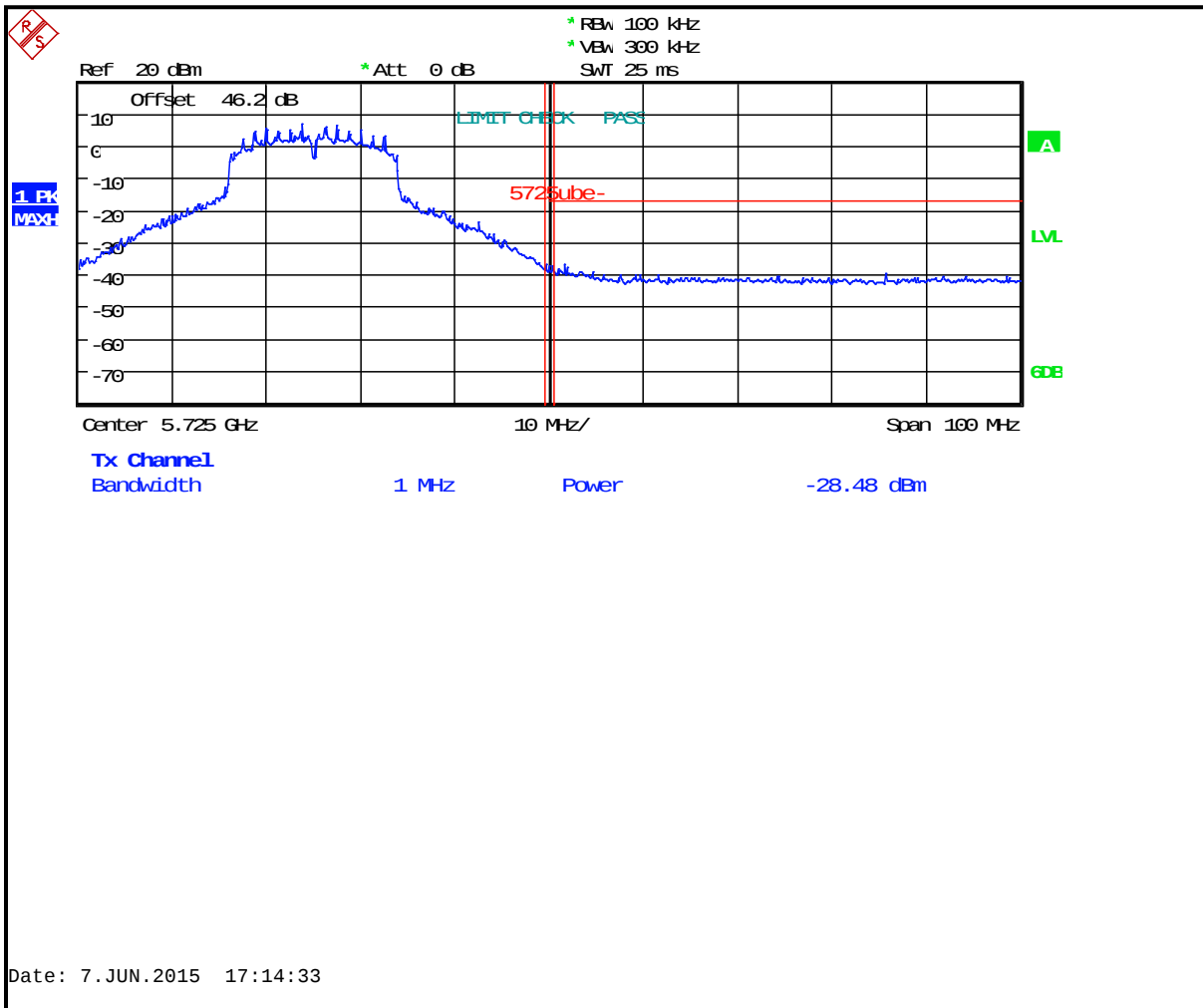
Plot 6-27: Upper Band Edge: Measurement Channel 140 (5700 MHz, 802.11n, Peak)
