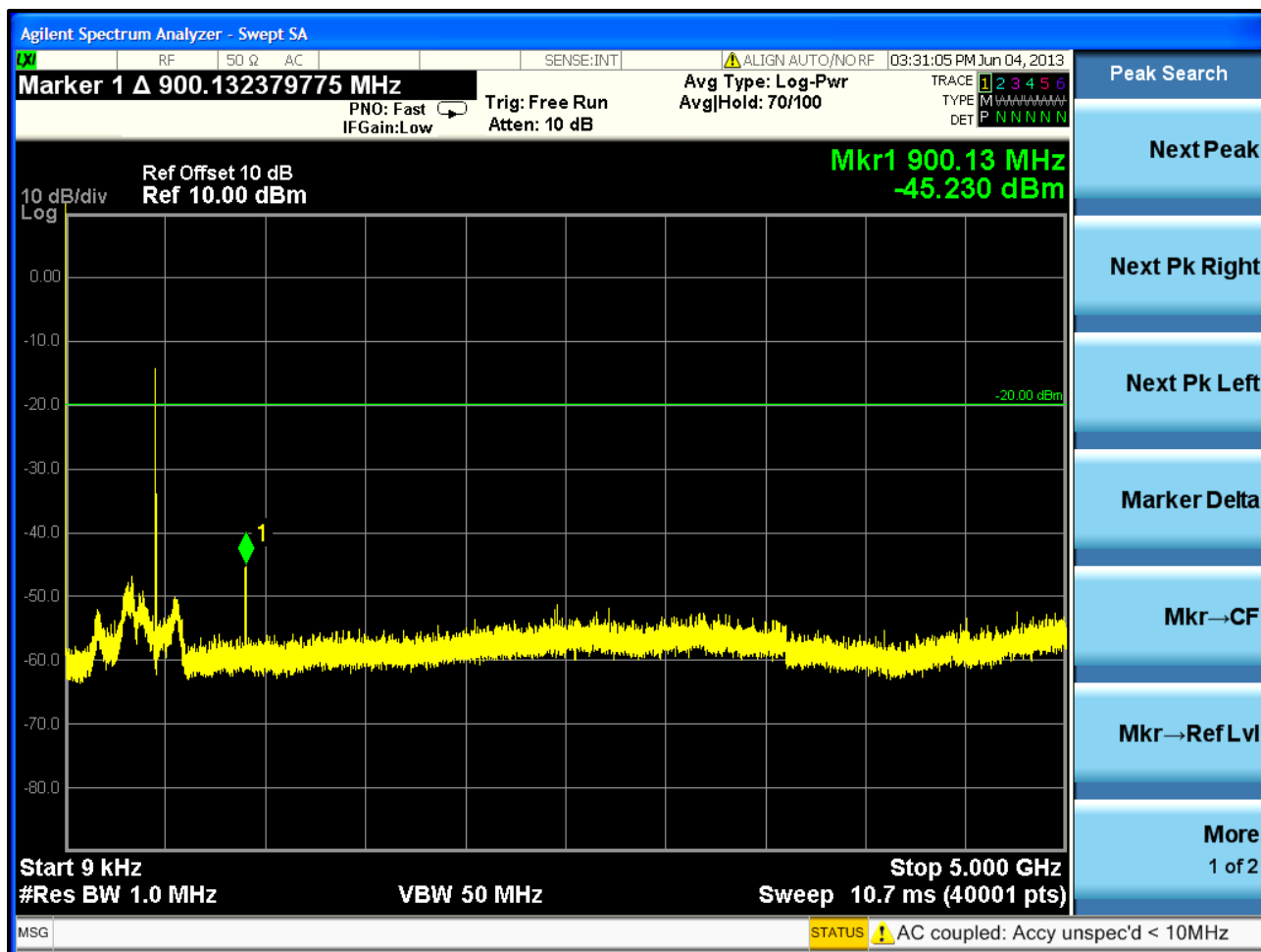
Plot 5-5: Spurious Emissions at Antenna Terminals – 450.0125 MHz
