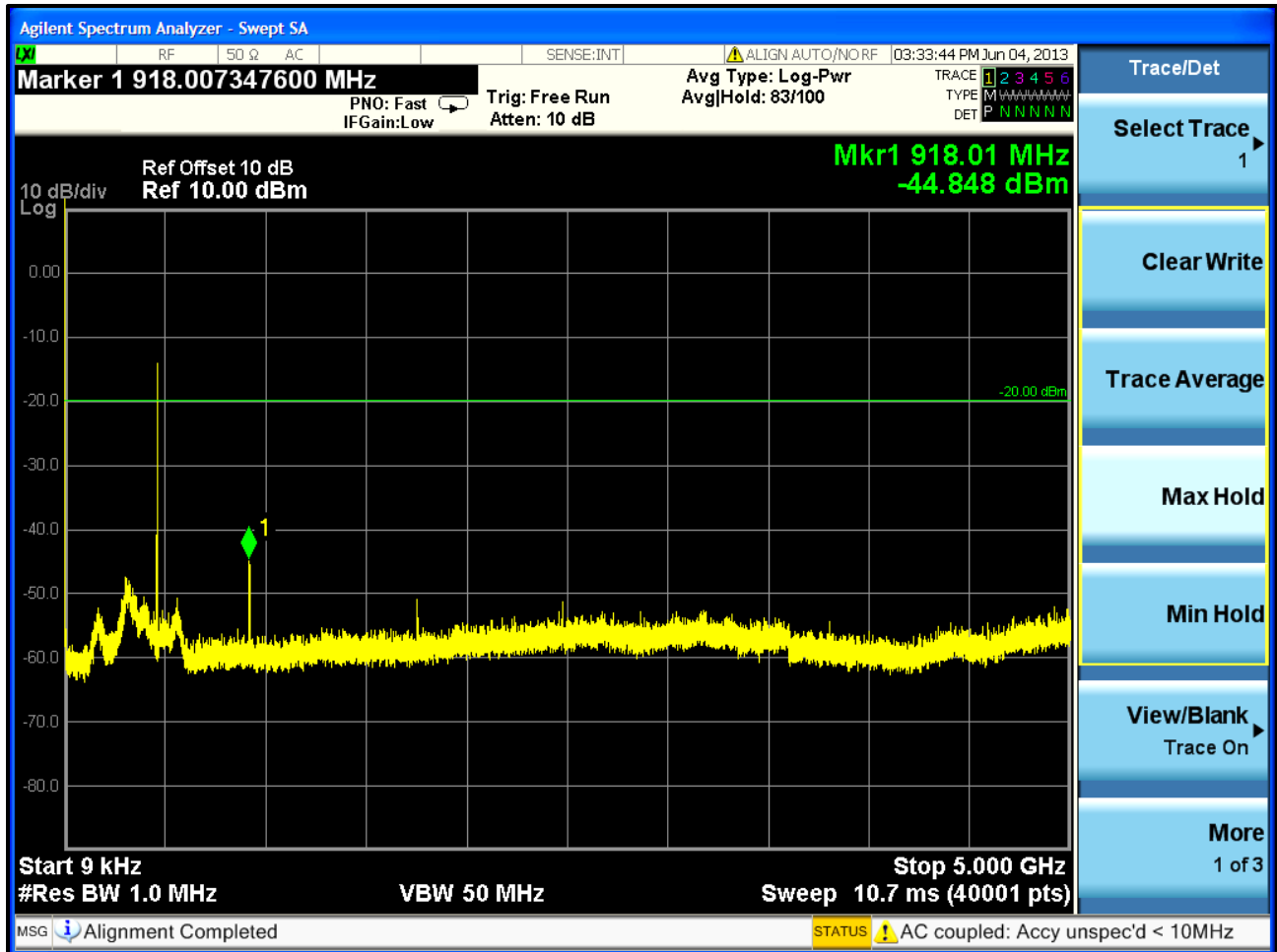
Plot 5-8: Spurious Emissions at Antenna Terminals – 458.9875 MHz
