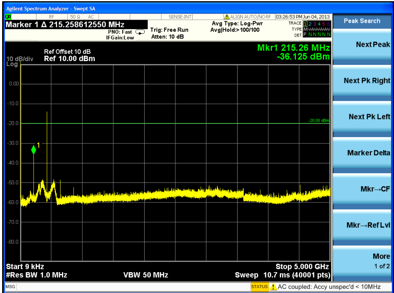
Plot 5-4: Spurious Emissions at Antenna Terminals – 429.9875 MHz
