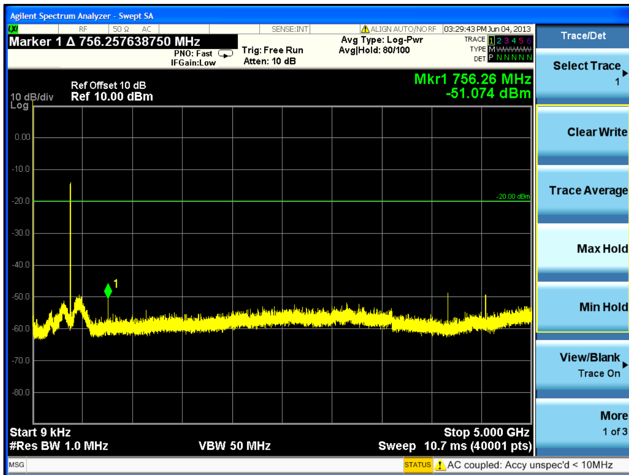
Plot 5-1: Spurious Emissions at Antenna Terminals – 378.0125 MHz
