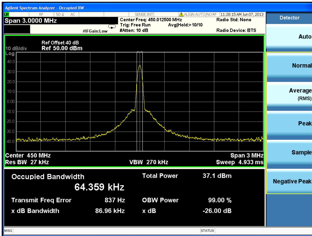
Plot 7-1: Occupied Bandwidth – 450.0125 MHz; Analog (FCC Part 22)
