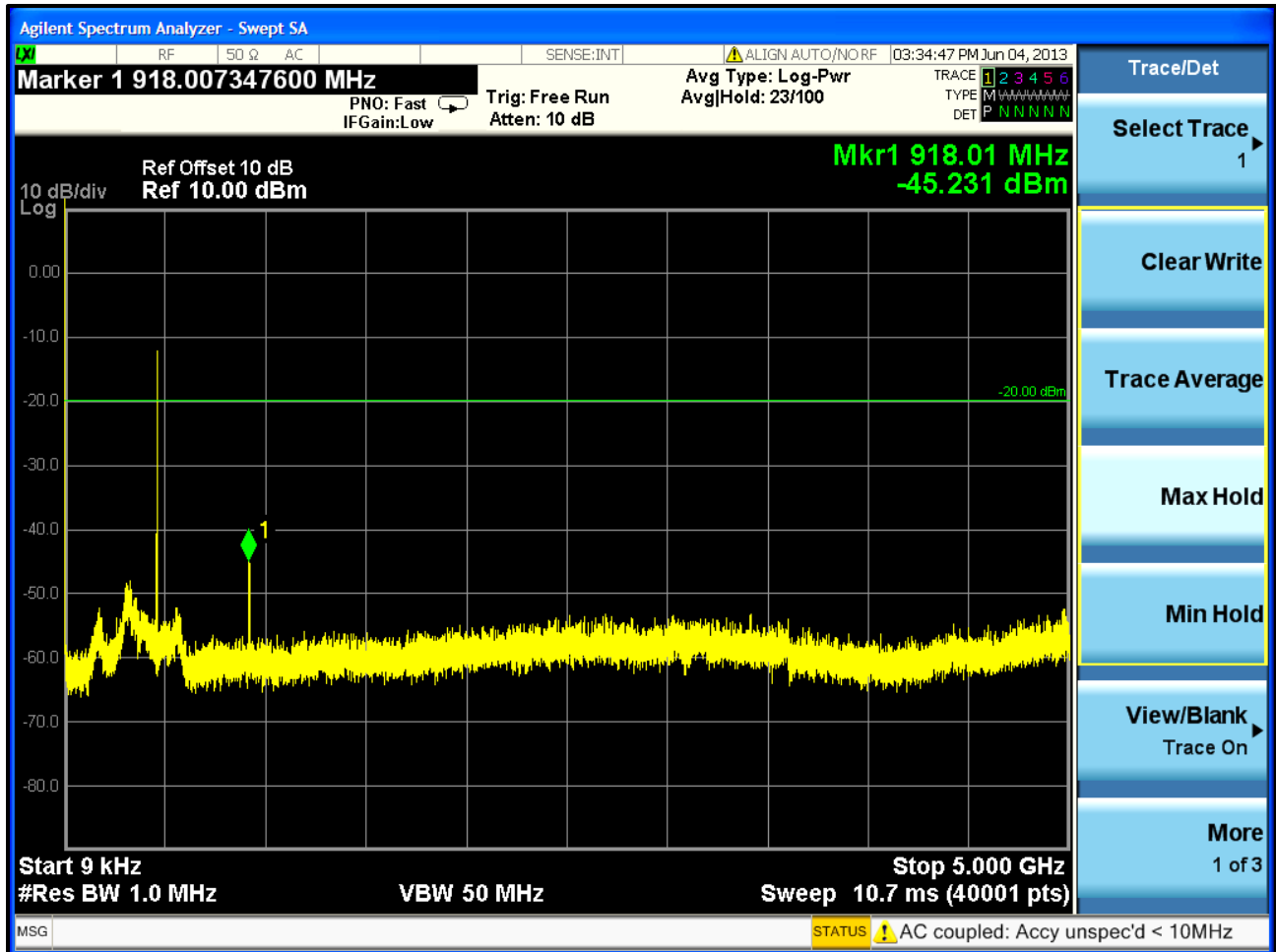
Plot 5-9: Spurious Emissions at Antenna Terminals – 459.0250 MHz
