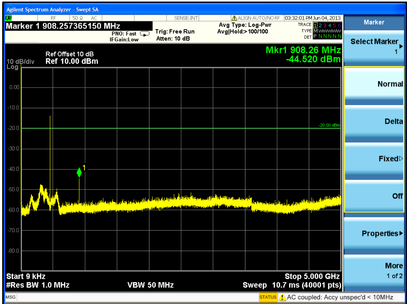
Plot 5-6: Spurious Emissions at Antenna Terminals – 454.0125 MHz
