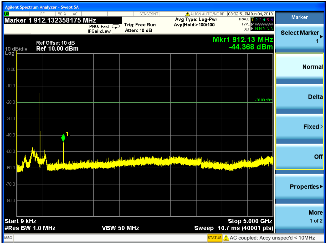
Plot 5-7: Spurious Emissions at Antenna Terminals – 456.0125 MHz
