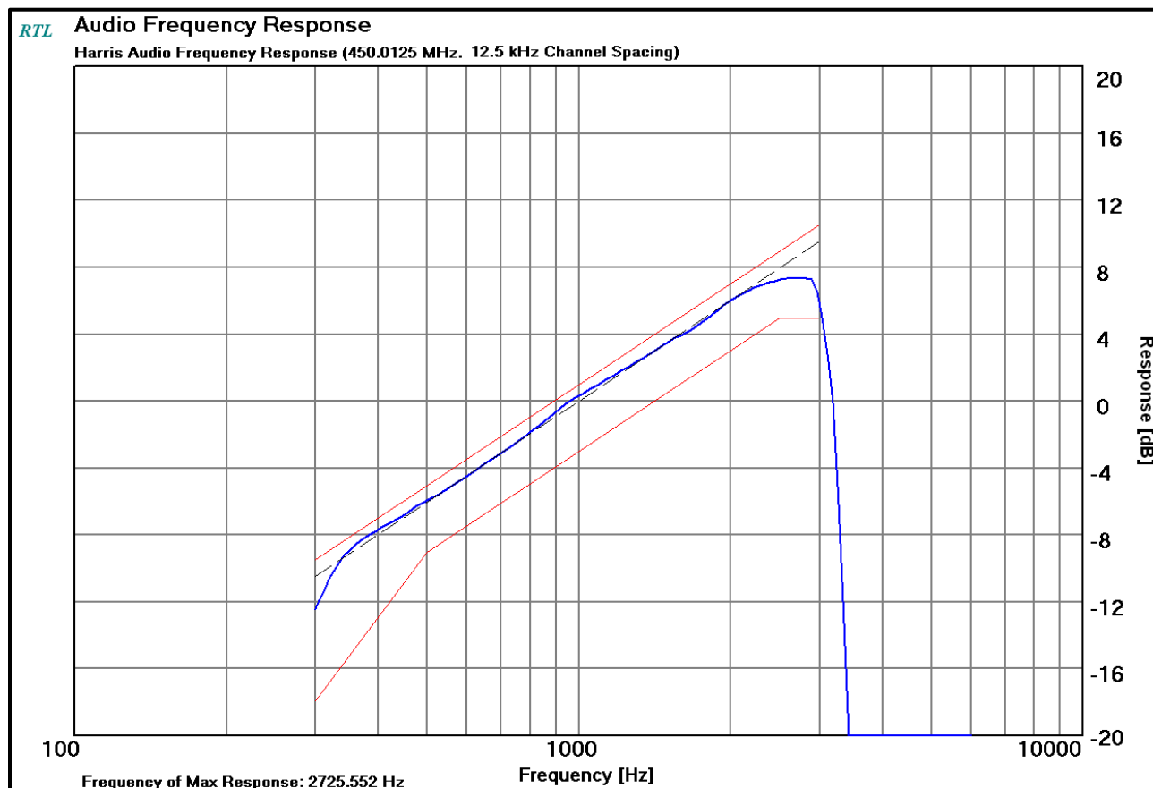
Plot 9-1: Modulation Characteristics - Audio Frequency Response – 450.0125 MHz
