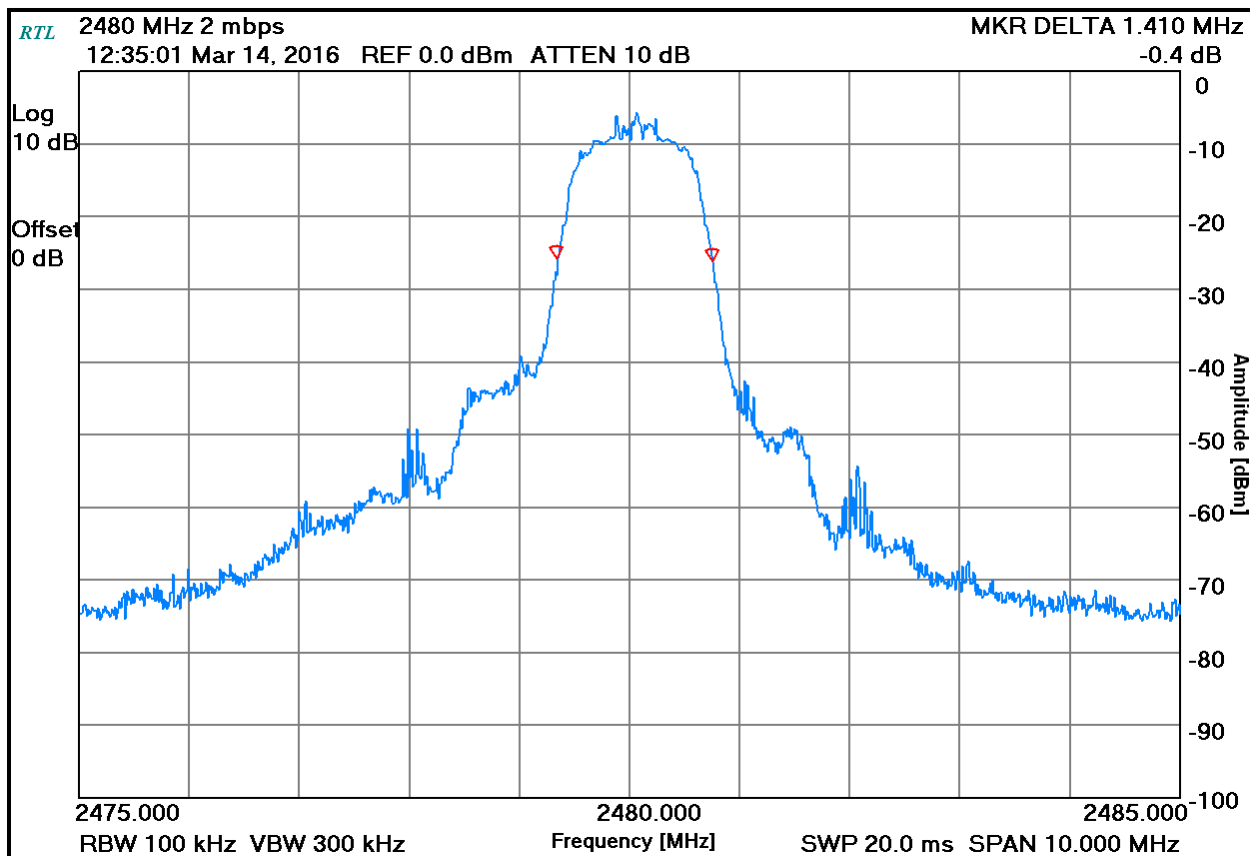
Plot 7-8: 20 dB Bandwidth - 2480 MHz; 2-EDR
