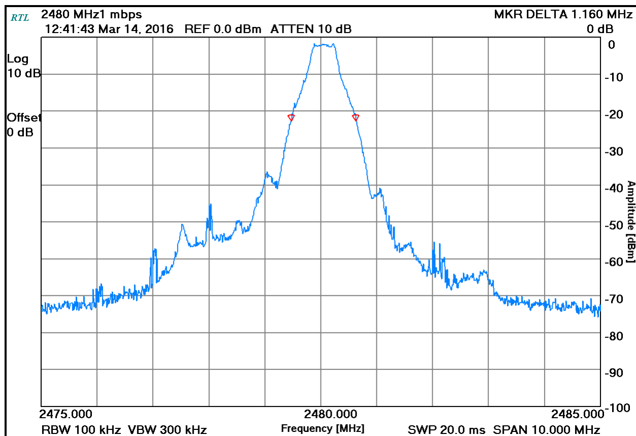
Plot 7-7: 20 dB Bandwidth - 2480 MHz; GFSK
