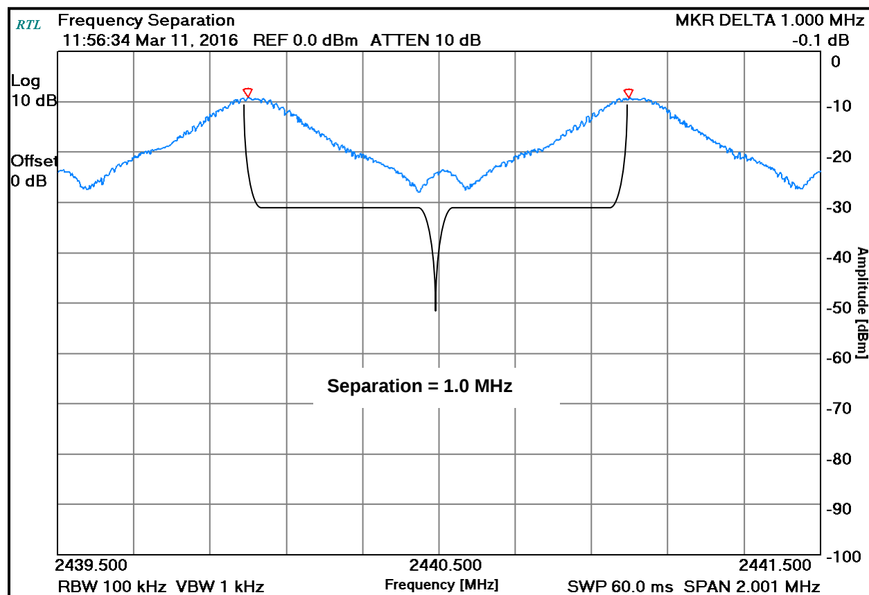
Plot 8-1: Carrier Frequency Separation
