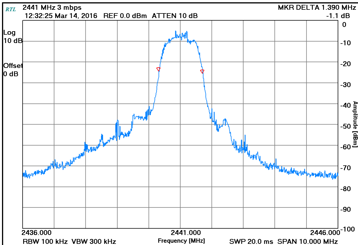
Plot 7-6: 20 dB Bandwidth - 2441 MHz; 3-EDR
