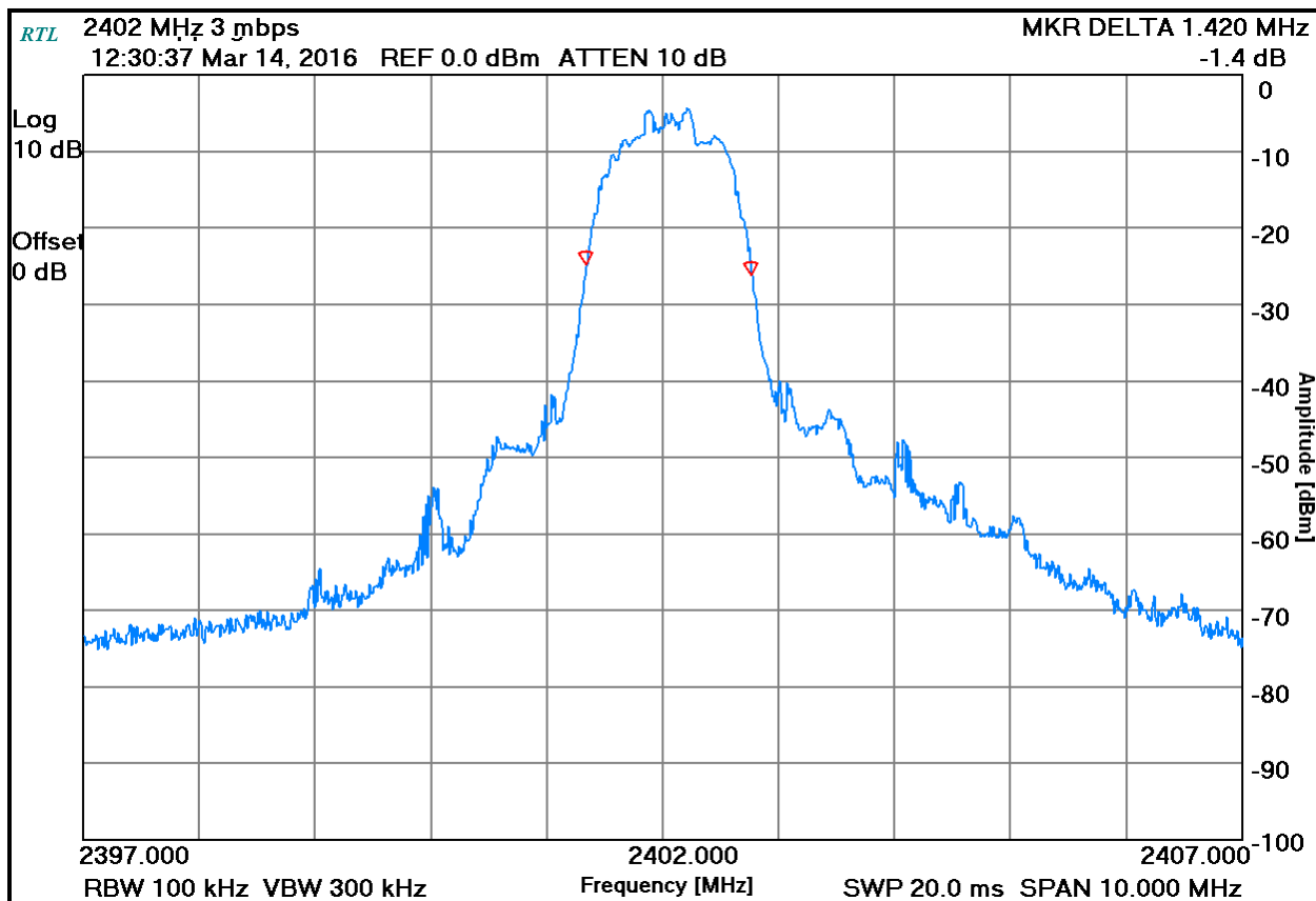
Plot 7-3: 20 dB Bandwidth - 2402 MHz; 3-EDR
