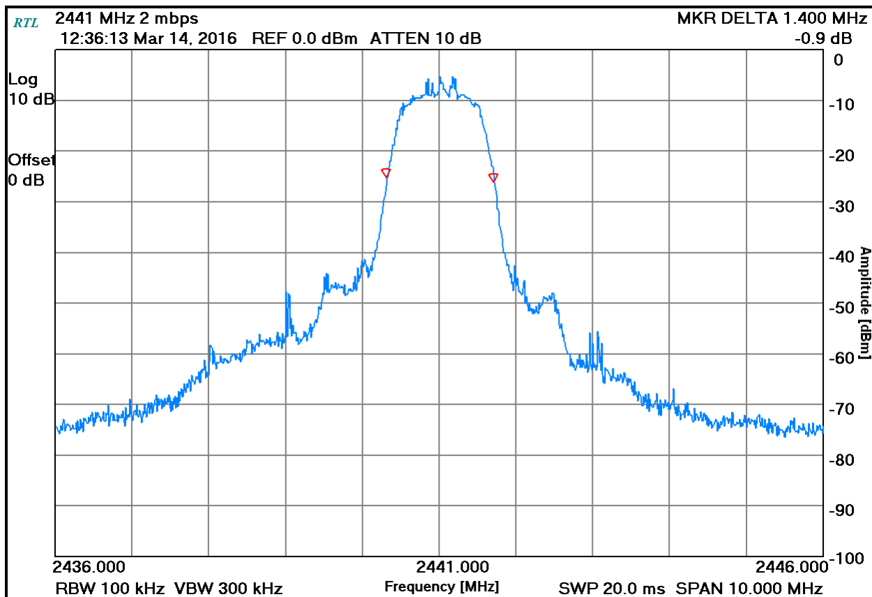
Plot 7-5: 20 dB Bandwidth - 2441 MHz; 2-EDR
