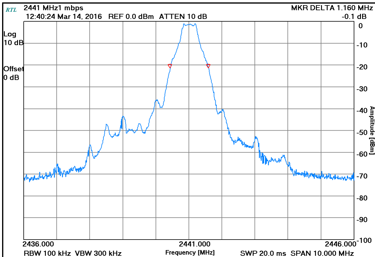
Plot 7-4: 20 dB Bandwidth - 2441 MHz; GFSK
