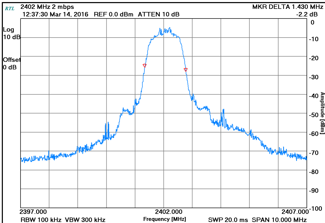
Plot 7-2: 20 dB Bandwidth - 2402 MHz; 2-EDR
