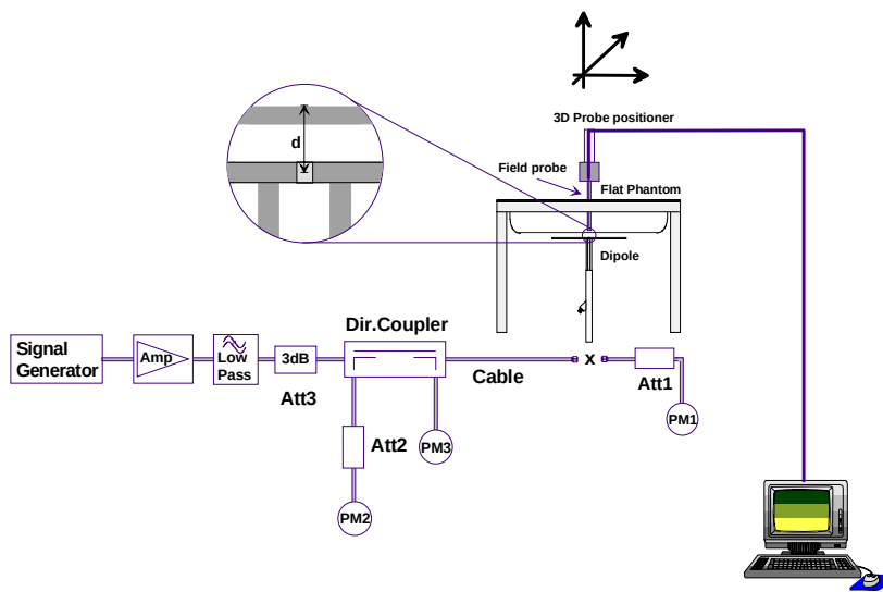
System Performance Check Measurement Setup Diagram (IEEE Standard 1528-2013)
