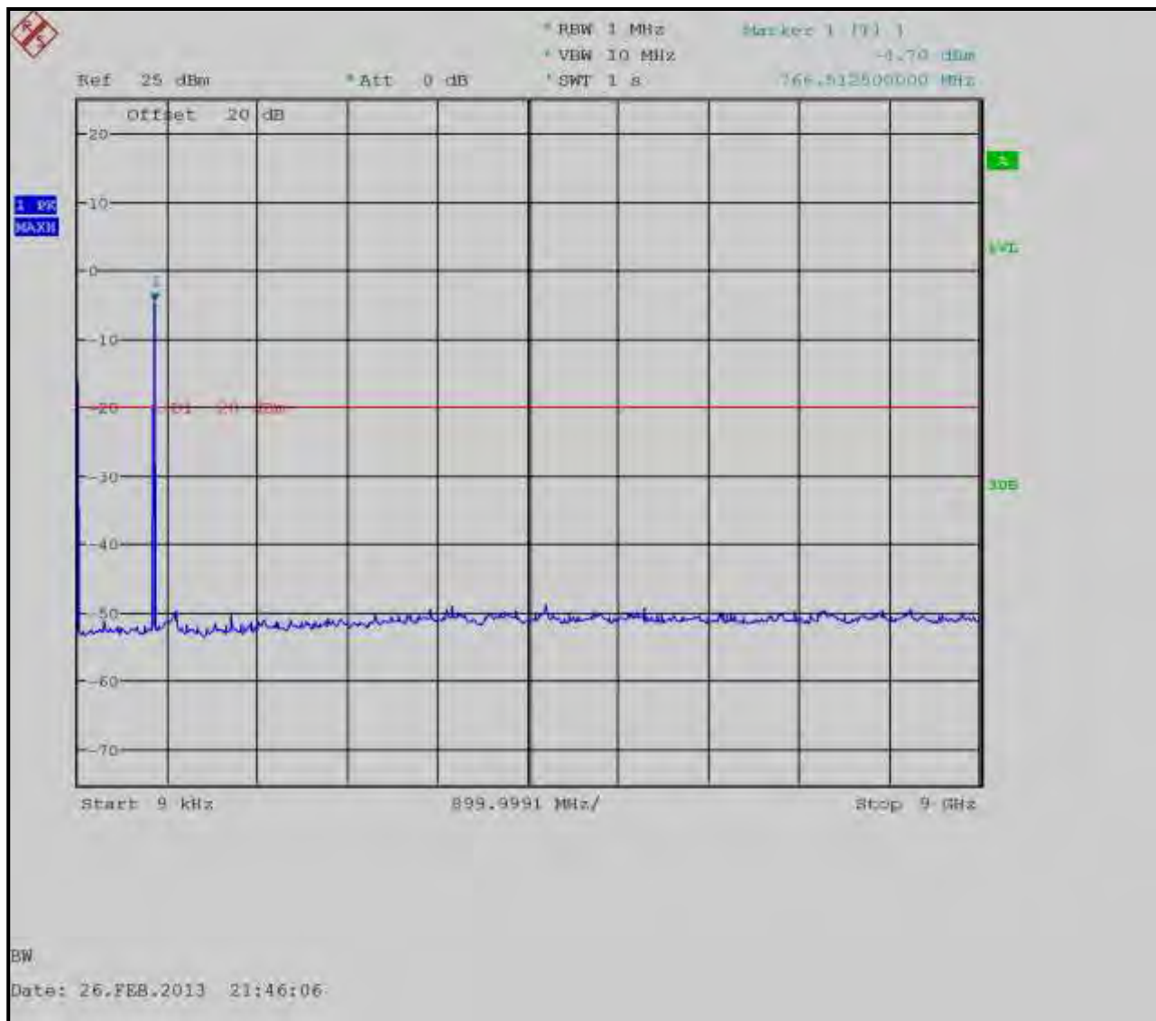
Plot 5-13: Conducted Spurious Emissions – H-CPM TDMA; 764.0125 MHz
