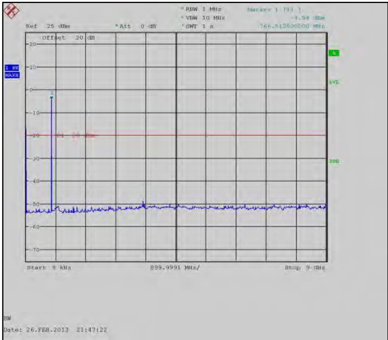
Plot 5-14: Conducted Spurious Emissions – H-CPM TDMA; 769.00625 MHz
