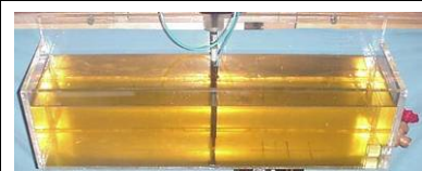
Plexiglas Side Planar Phantom
