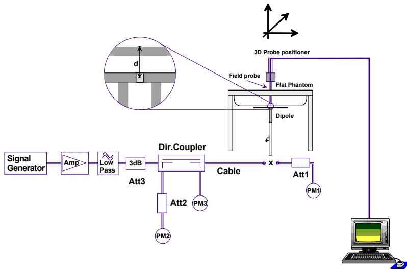
System Performance Check Measurement Setup Diagram (IEEE 1528-2013)
