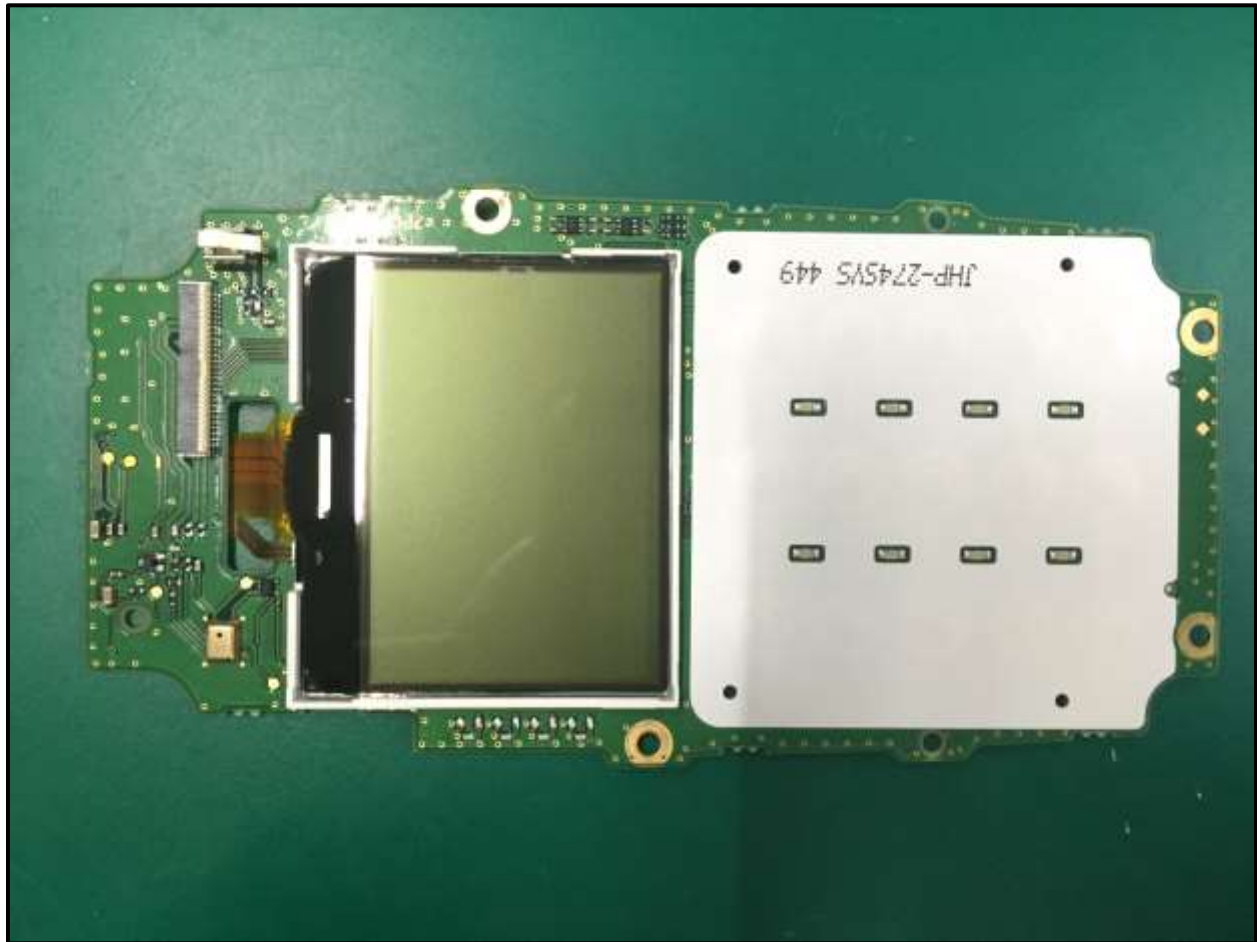
Photograph 14: Display Board with Display Front
