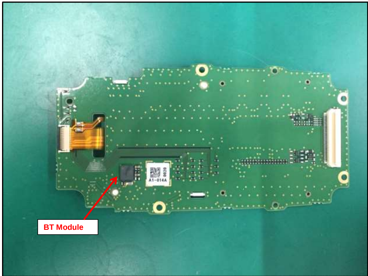
Photograph 16: Display Board Back with Bluetooth Module
