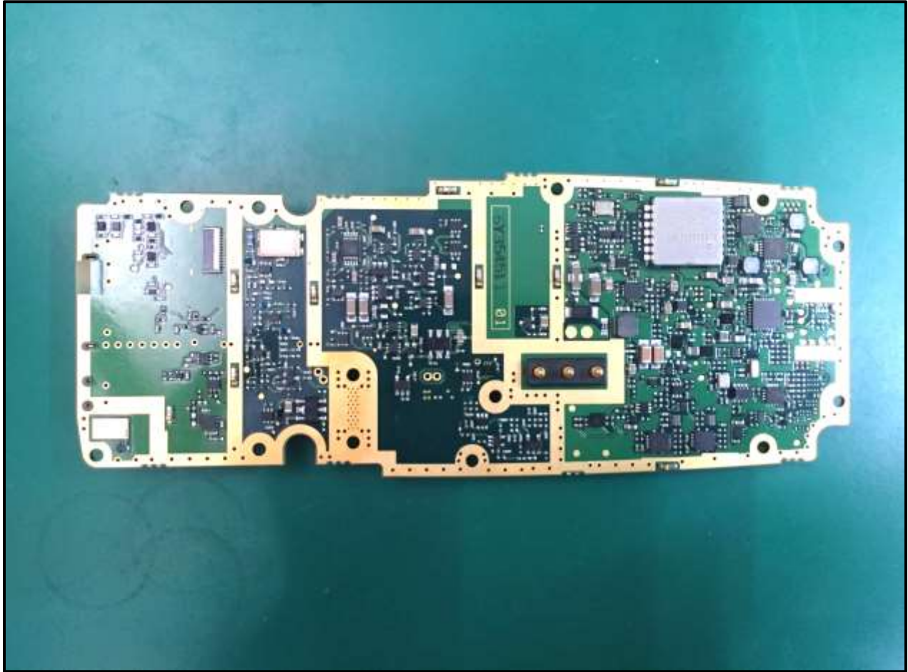
Photograph 18: Radio Board Back
