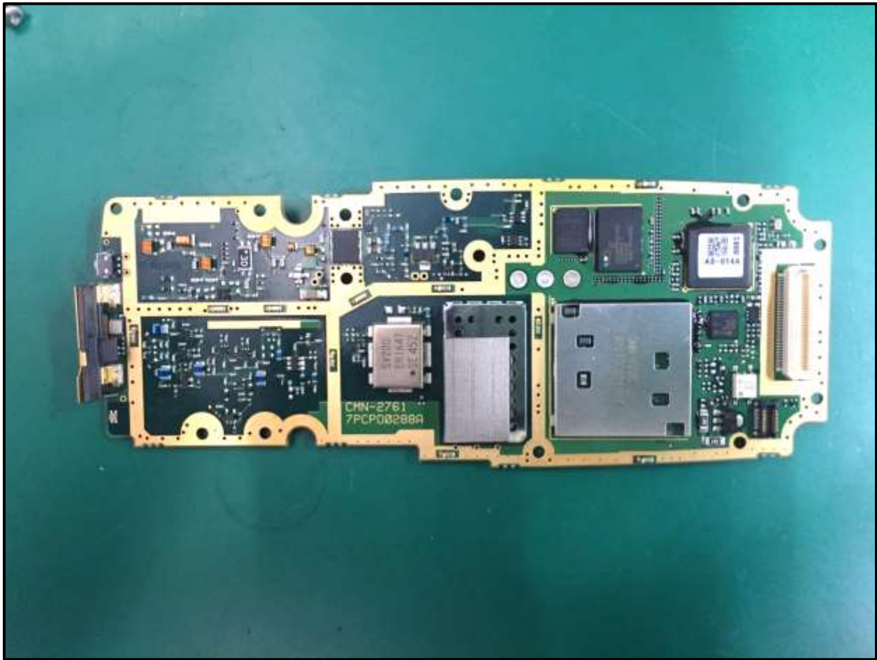
Photograph 17: Radio Board Front
