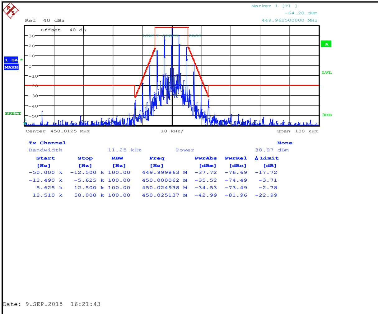
Plot 7-8: Occupied Bandwidth – 450.0125 MHz; Narrowband Analog; Mask D
