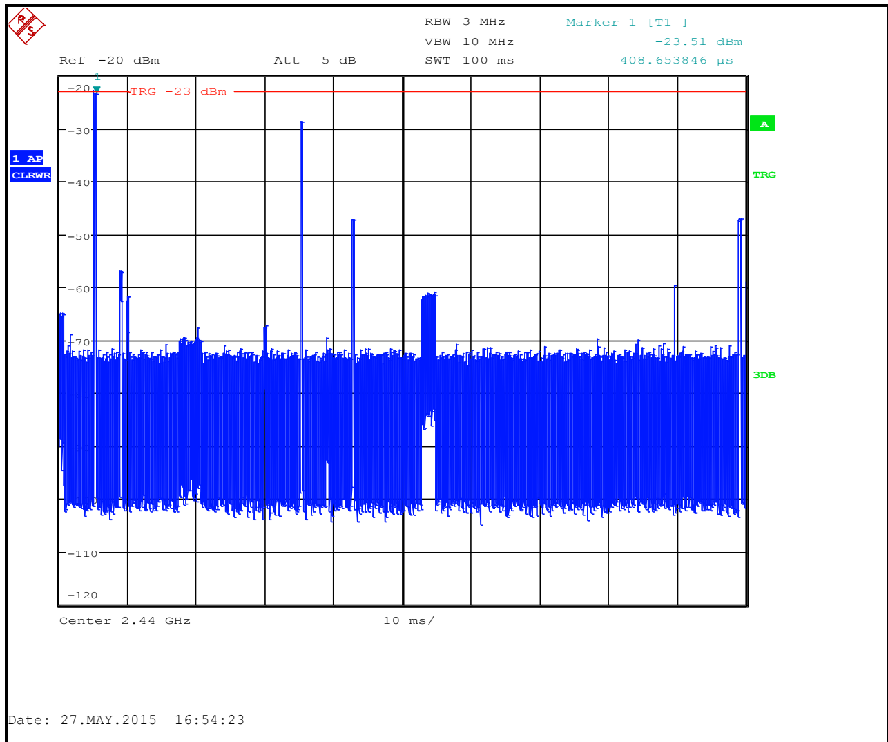
Plot 4-2: Single Pulse per 100ms
