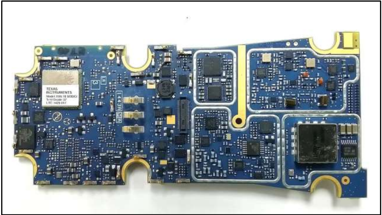
Photograph 12: Bottom without Shields
