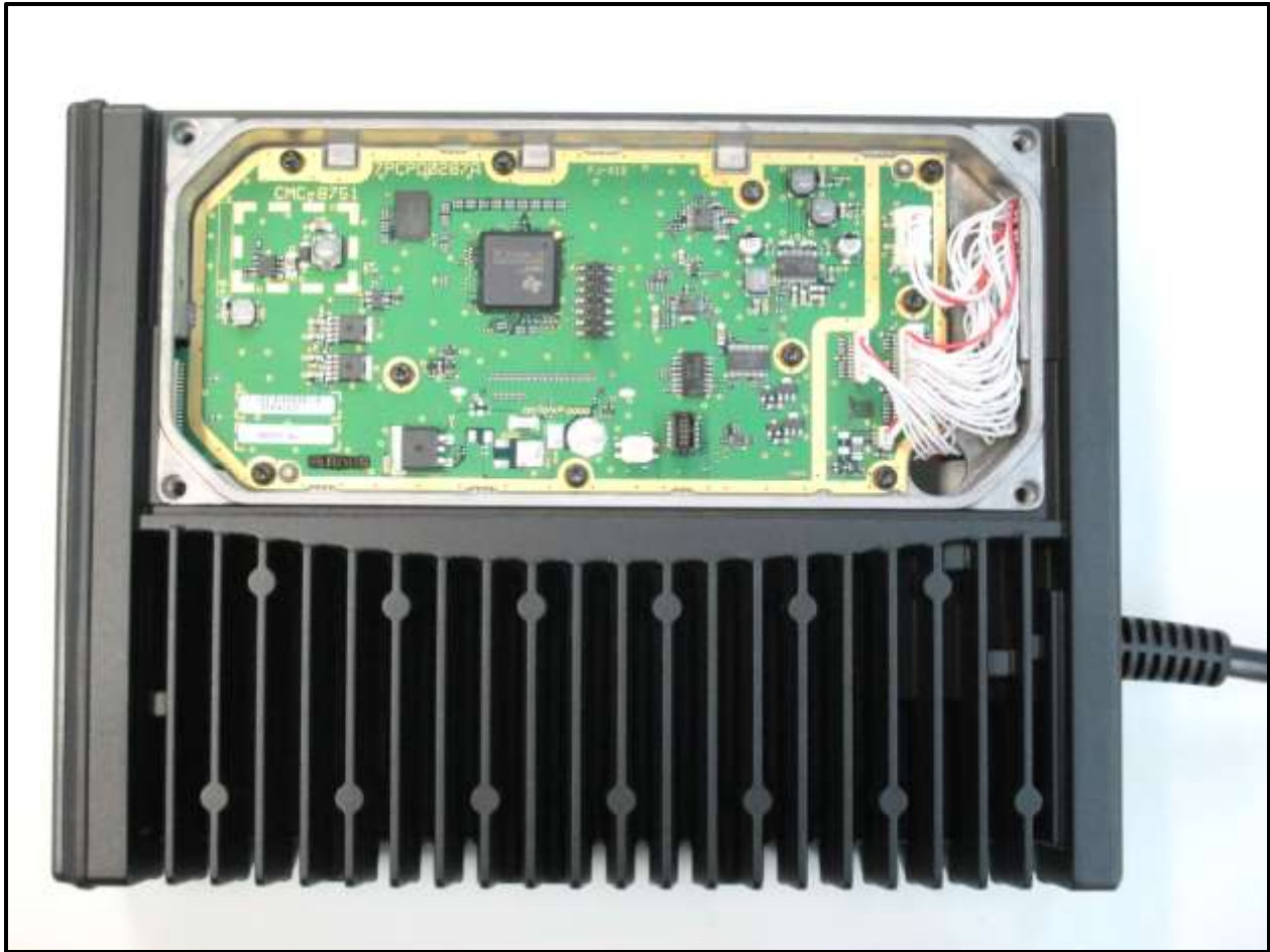
Photograph 18: Top Cover Removed
