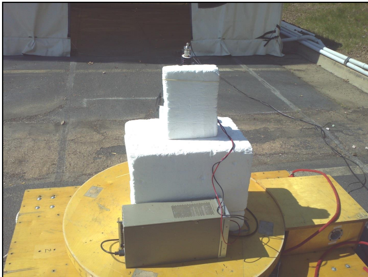
Photograph 6: Radiated Emissions (Spurious/Harmonics) – Back View
