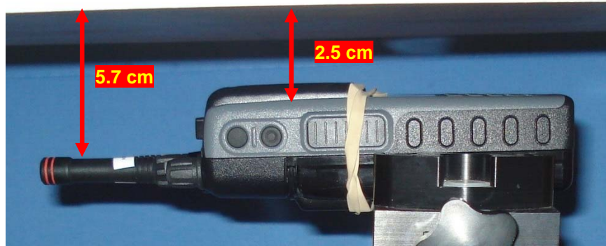
Face-Held Test Setup - Antenna 1 (1219/12)
