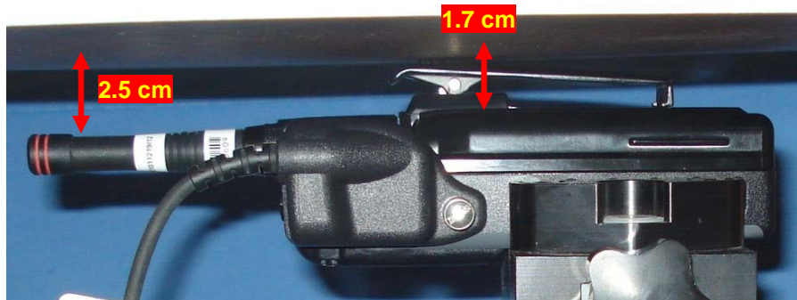
Body-worn Test Setup - Belt-Clip with Speaker-Microphone, Antenna 1 (1219/12)
