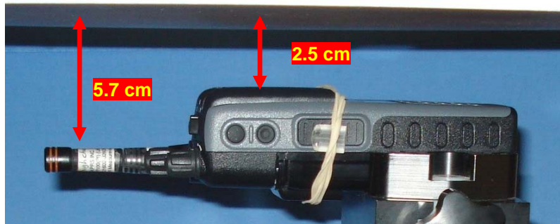
Face-Held Test Setup - Antenna 2 (1219/13)
