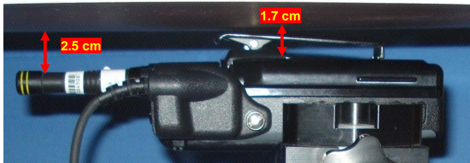
Body-worn Test Setup Belt-Clip with Speaker-Microphone, Antenna 3 (1219/14)
