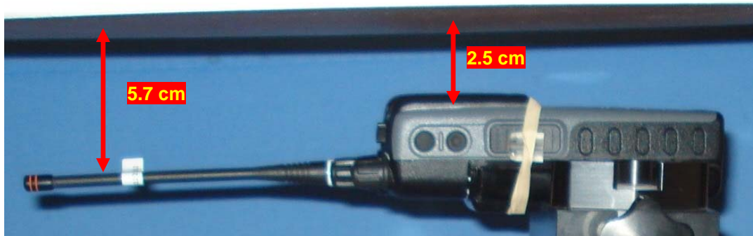
Face-Held Test Setup - Antenna 4 (1223/12)
