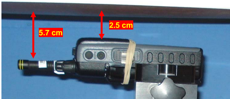
Face-Held Test Setup - Antenna 3 (1219/14)
