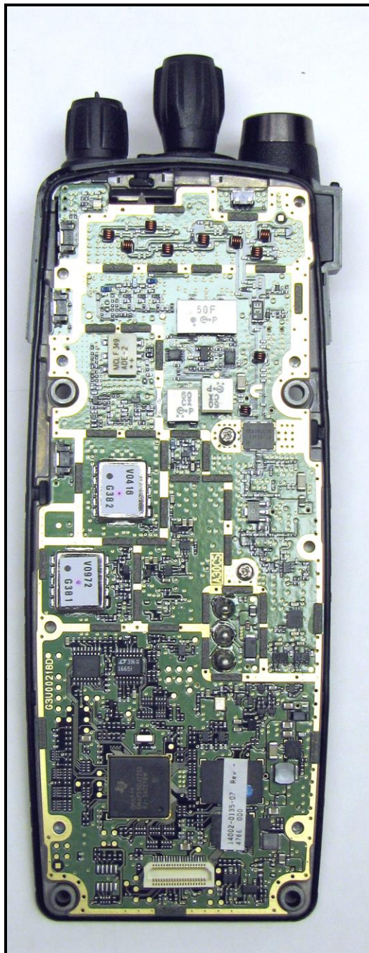
Photograph 22: Main Board in Radio
