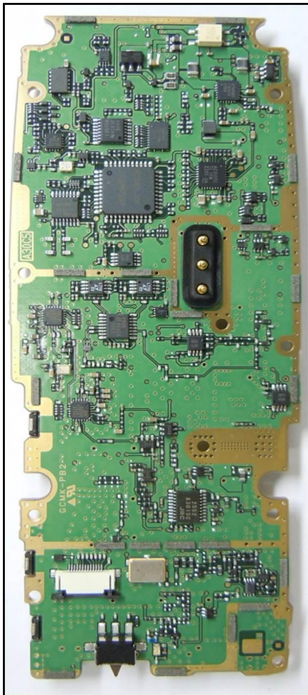
Photograph 24: Main Board – Bottom
