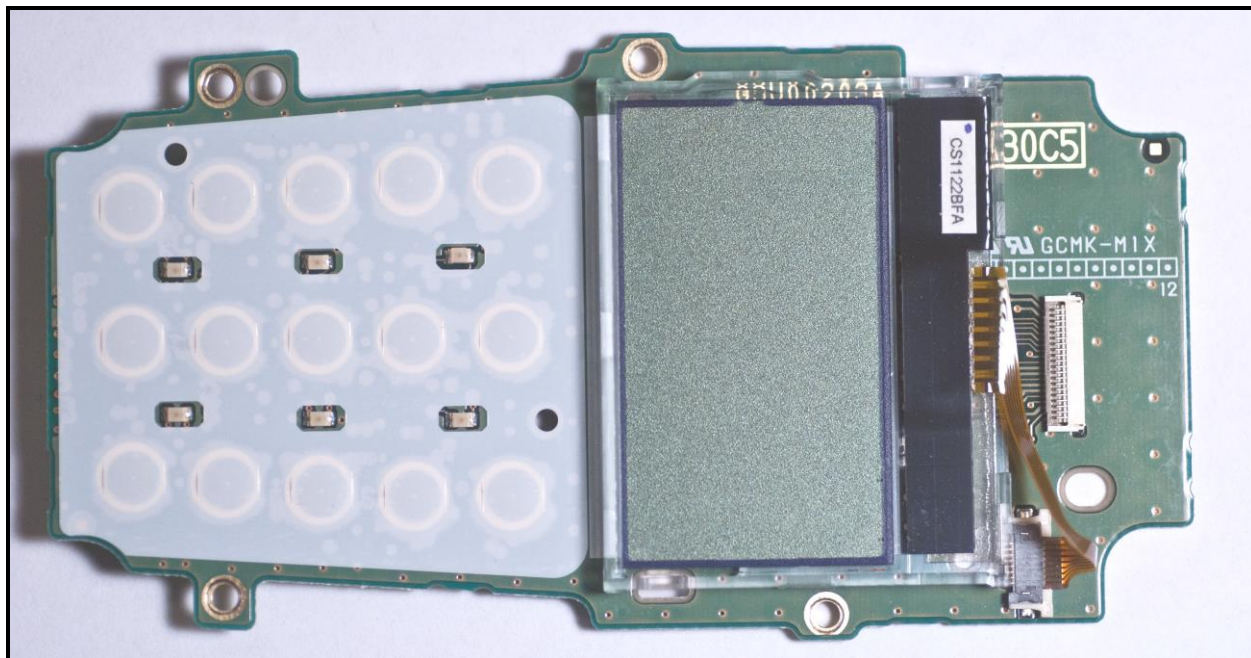
Photograph 26: Interface PWB LCD Side
