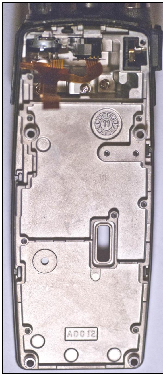
Photograph 29: Inside Rear Cover
