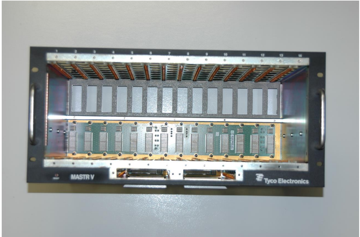
Photograph 3. Chassis – Front
