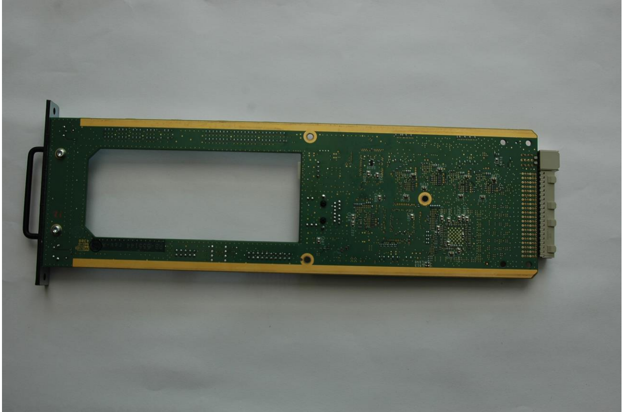
Photograph 5. E-Switch - Bottom Side
