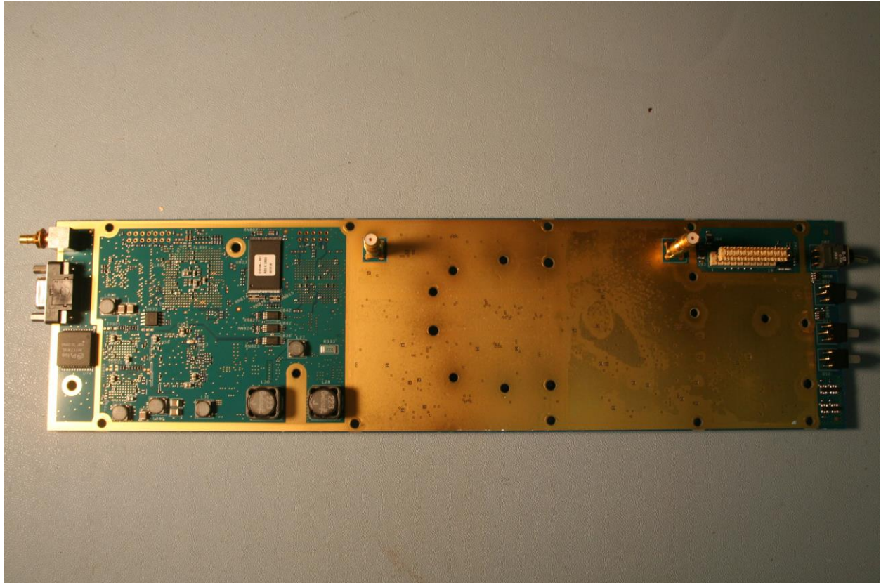
Photograph 7. Linearizer - Bottom Side
