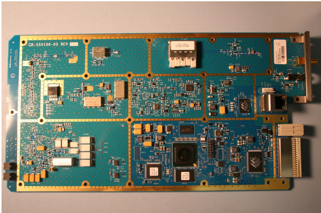
Photograph 21. Receiver - Top Side
