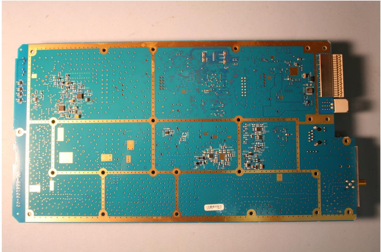
Photograph 20. Receiver - Bottom Side
