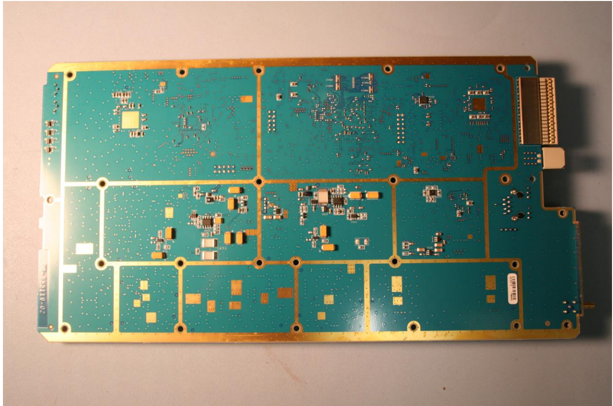
Photograph 24. Transmit Module - Bottom Side
