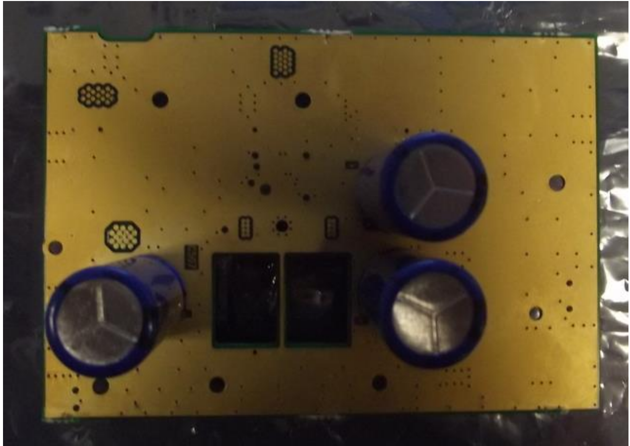
Photograph 16. Power Amplifier Switcher Assembly Bottom
