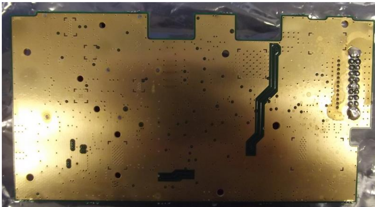
Photograph 10. Power Amplifier Driver Assembly Bottom Side
