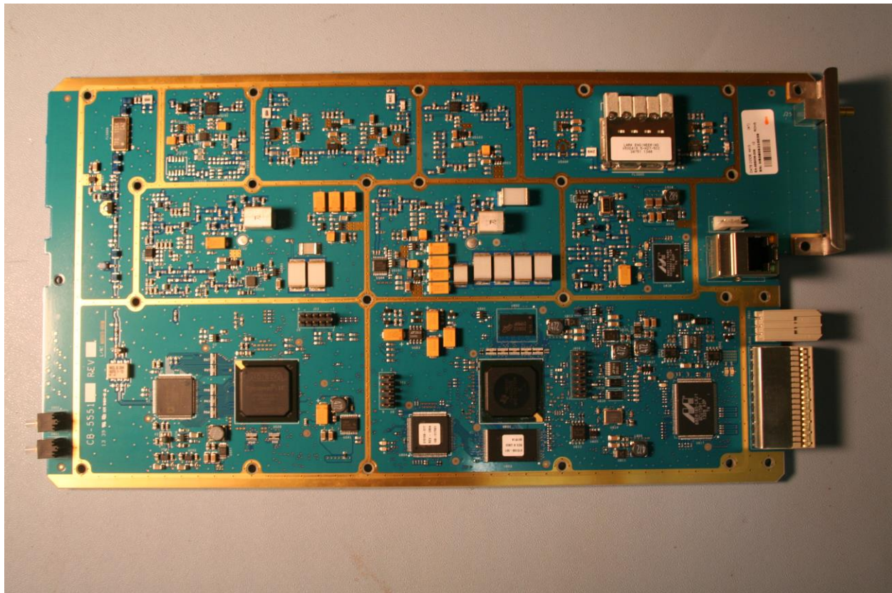
Photograph 25. Transmit Module - Top Side
