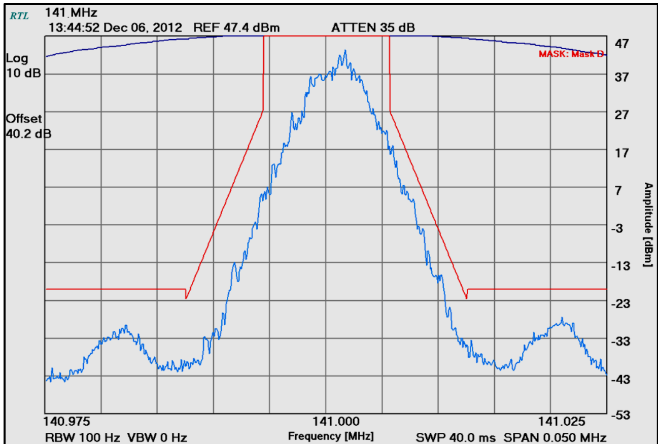
Plot 8-3: Occupied Bandwidth – 141.0000 MHz; Mask D
