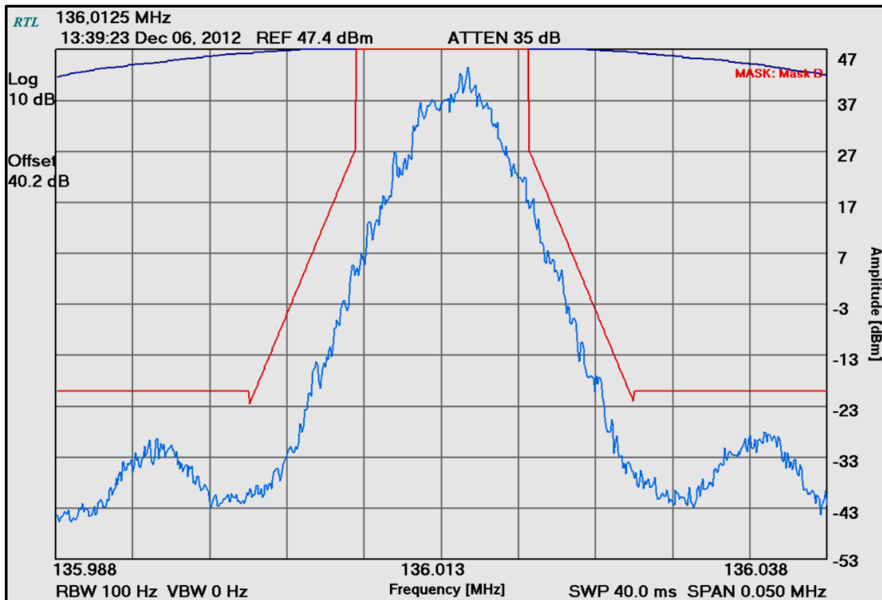
Plot 8-1: Occupied Bandwidth – 136.0125 MHz; Mask D
