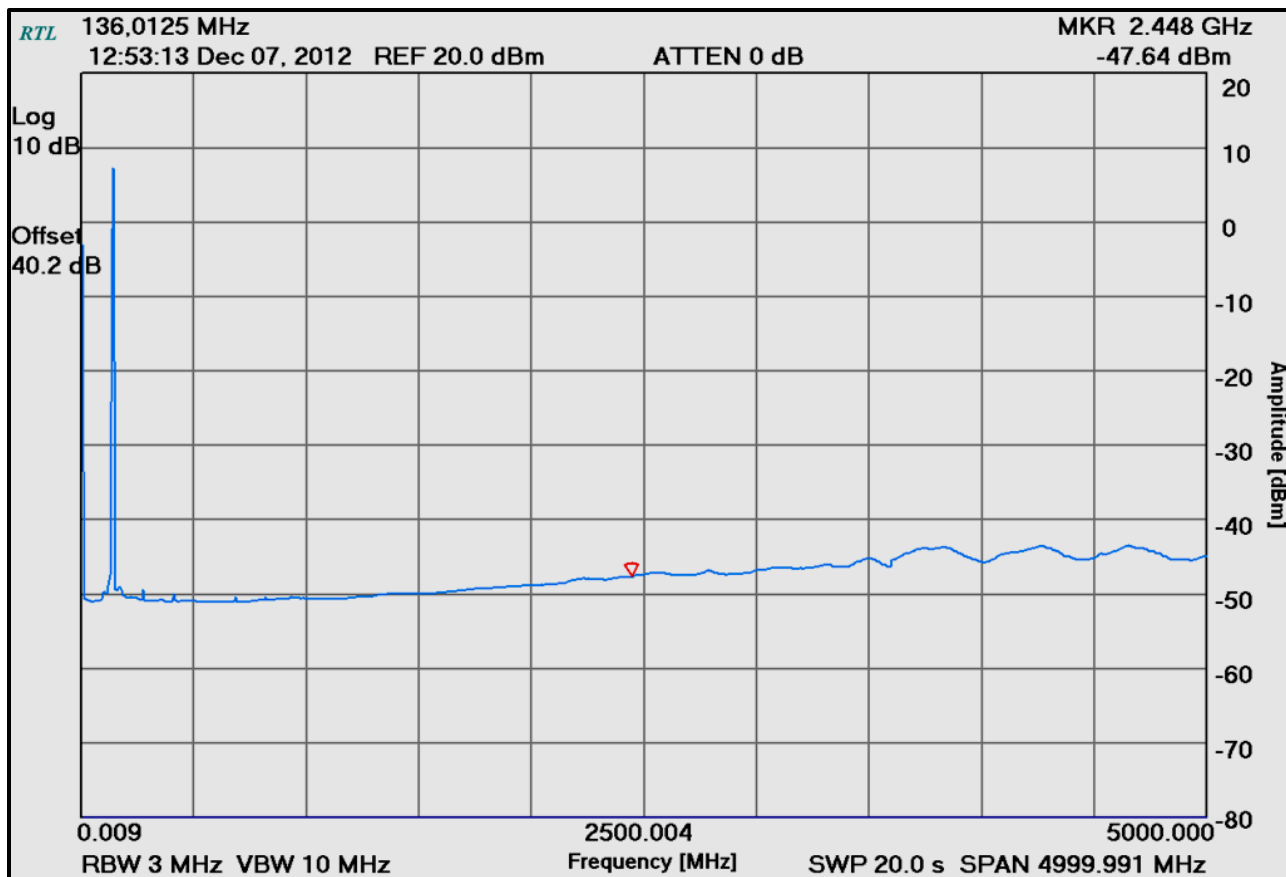
Plot 6-1: Spurious Emissions at Antenna Terminals – 136.0125MHz
