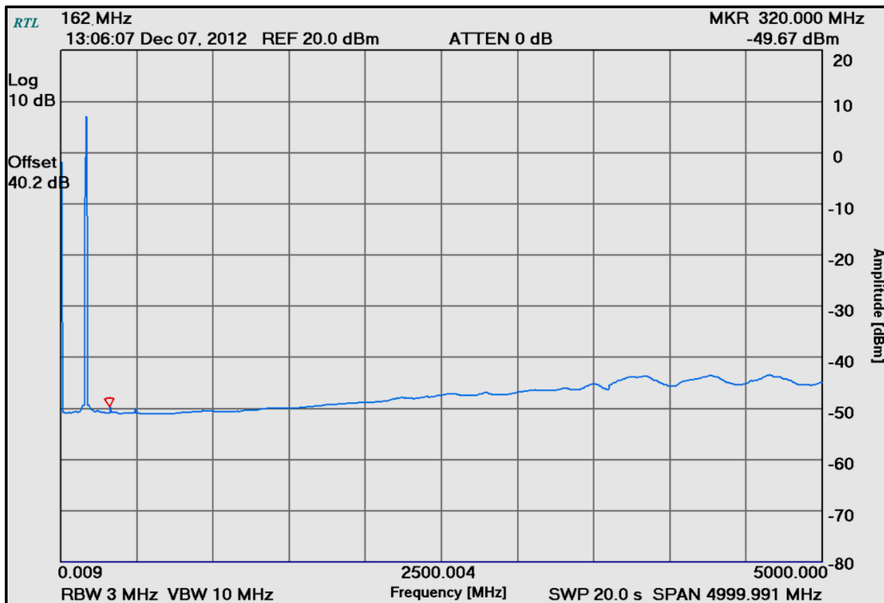
Plot 6-10: Spurious Emissions at Antenna Terminals – 162.0000 MHz
