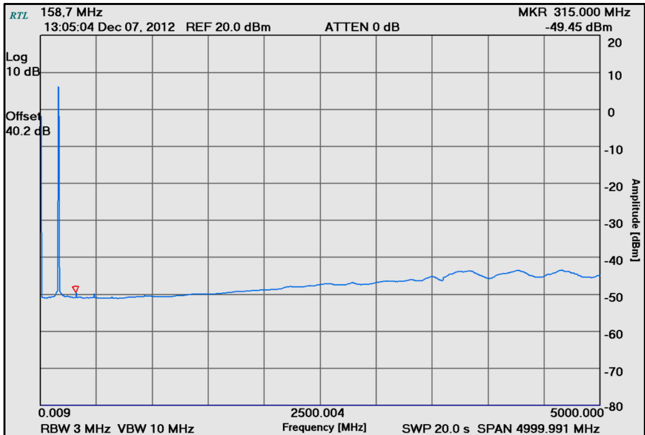
Plot 6-9: Spurious Emissions at Antenna Terminals – 158.7000 MHz
