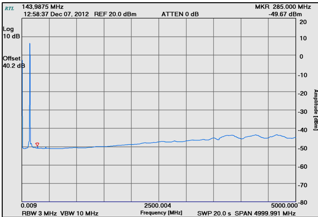
Plot 6-4: Spurious Emissions at Antenna Terminals – 143.9875 MHz
