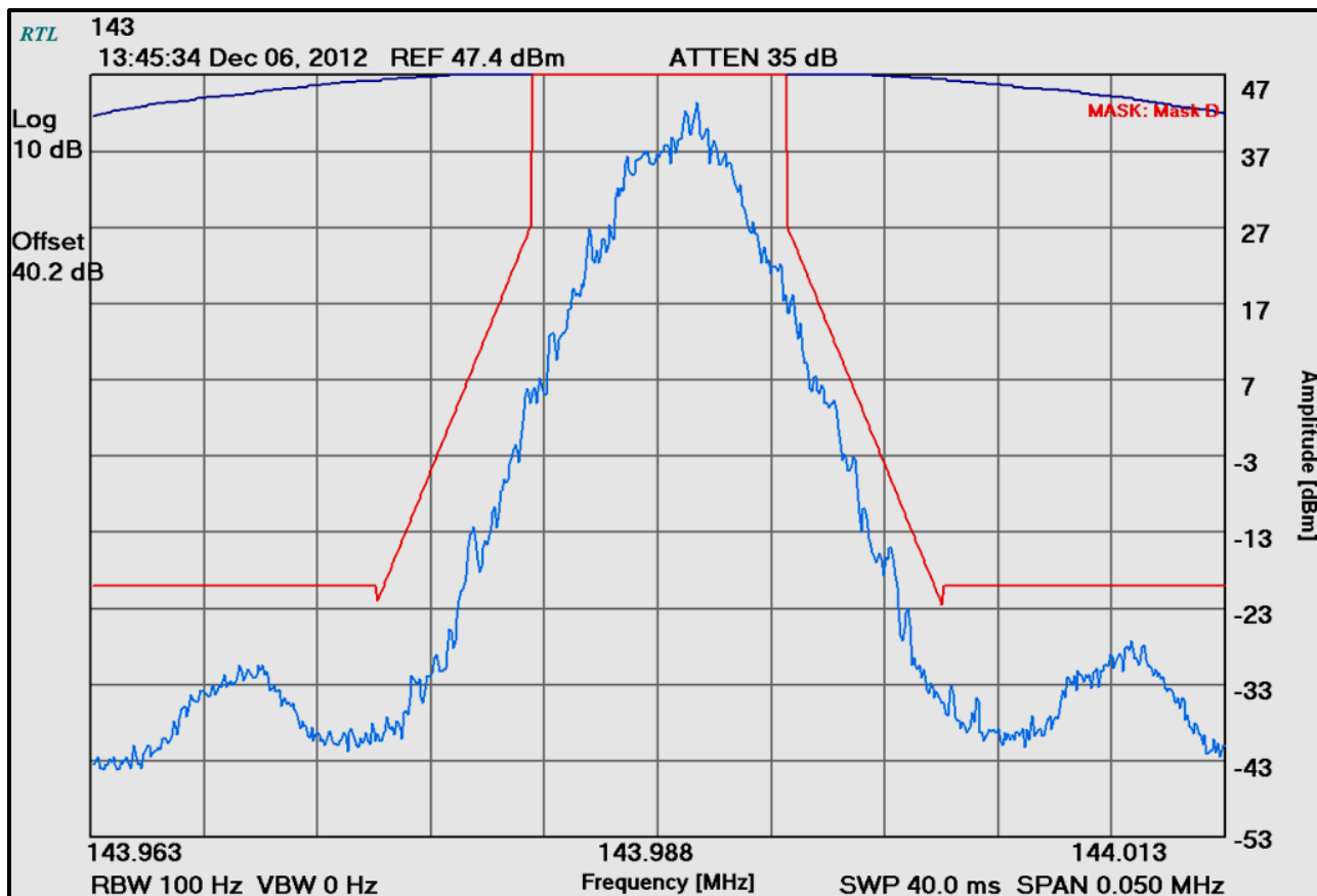
Plot 8-4: Occupied Bandwidth – 143.9875 MHz; Mask D
