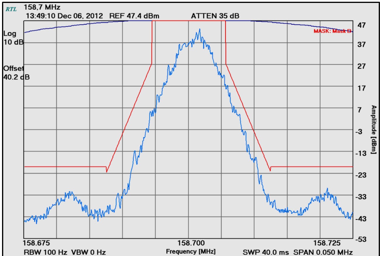
Plot 8-9: Occupied Bandwidth – 158.7000 MHz; Mask D
