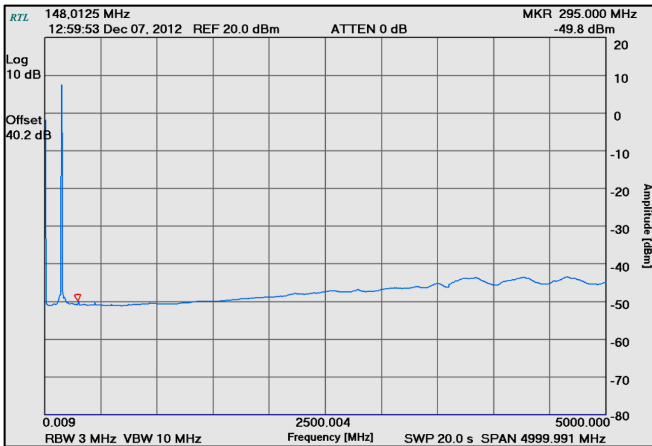
Plot 6-5: Spurious Emissions at Antenna Terminals – 148.0125 MHz
