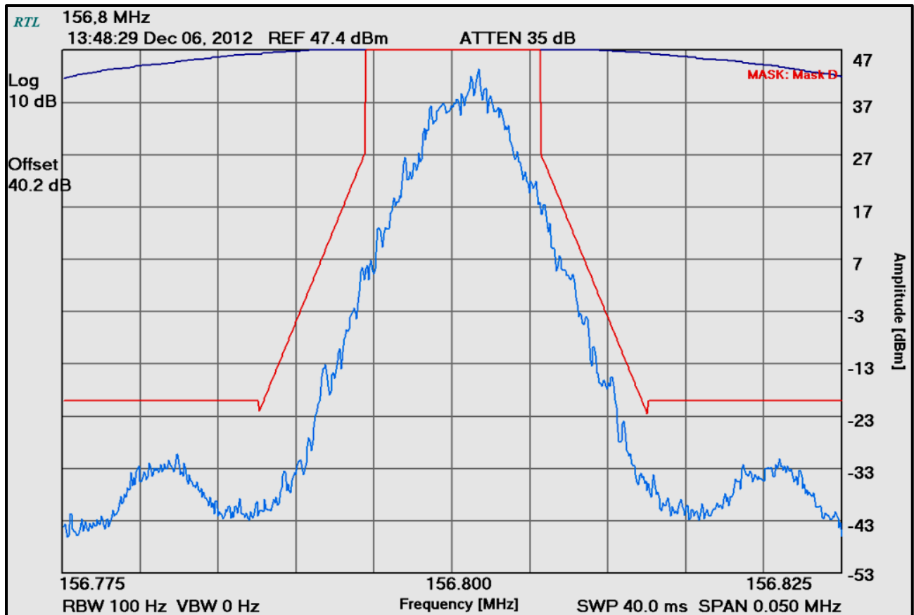
Plot 8-8: Occupied Bandwidth – 156.8000 MHz; Mask D
