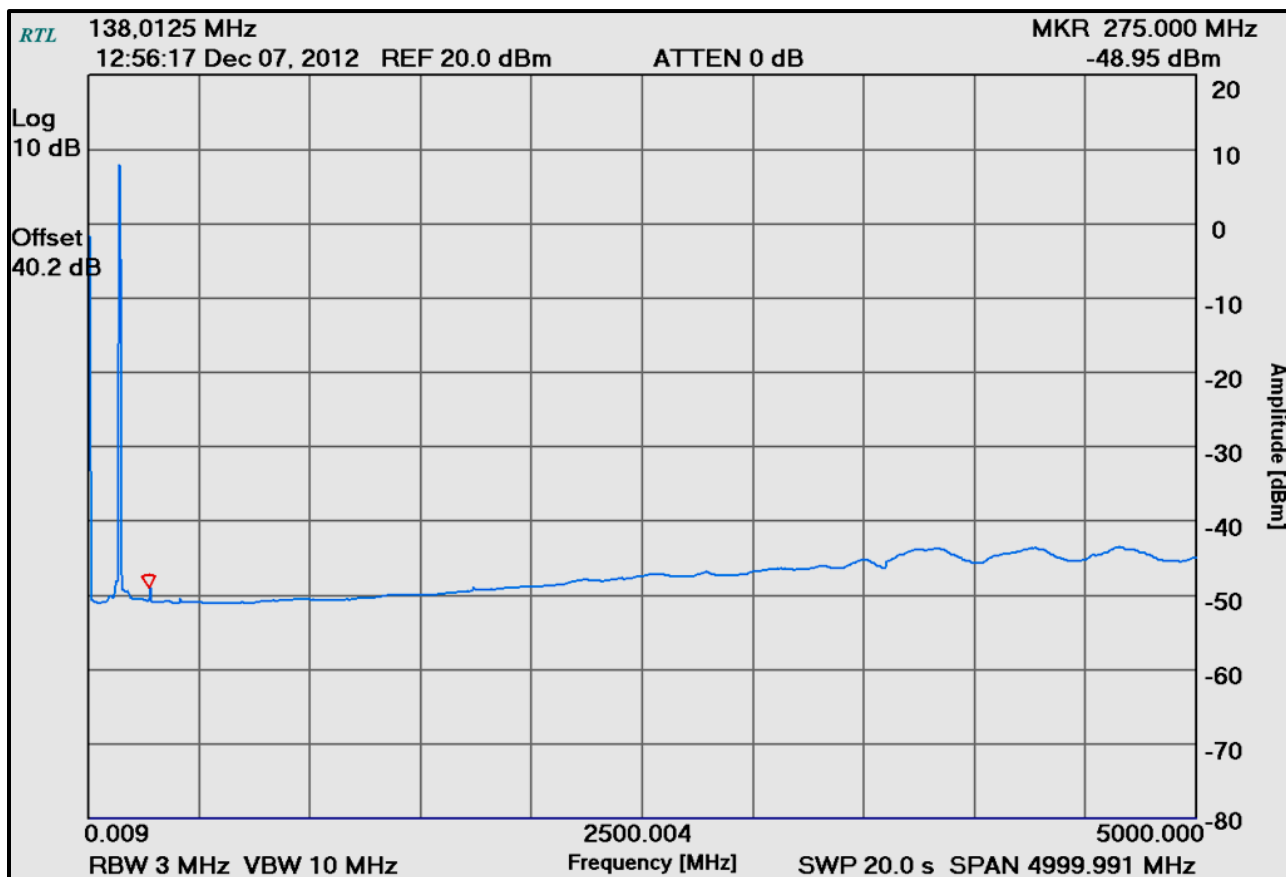
Plot 6-2: Spurious Emissions at Antenna Terminals – 138.0125 MHz
