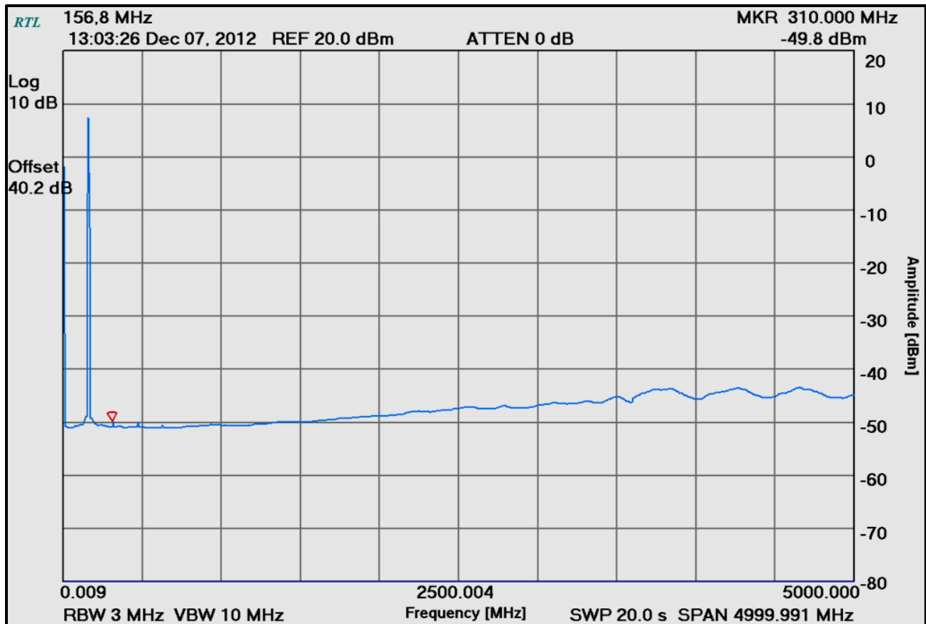
Plot 6-8: Spurious Emissions at Antenna Terminals – 156.8000 MHz
