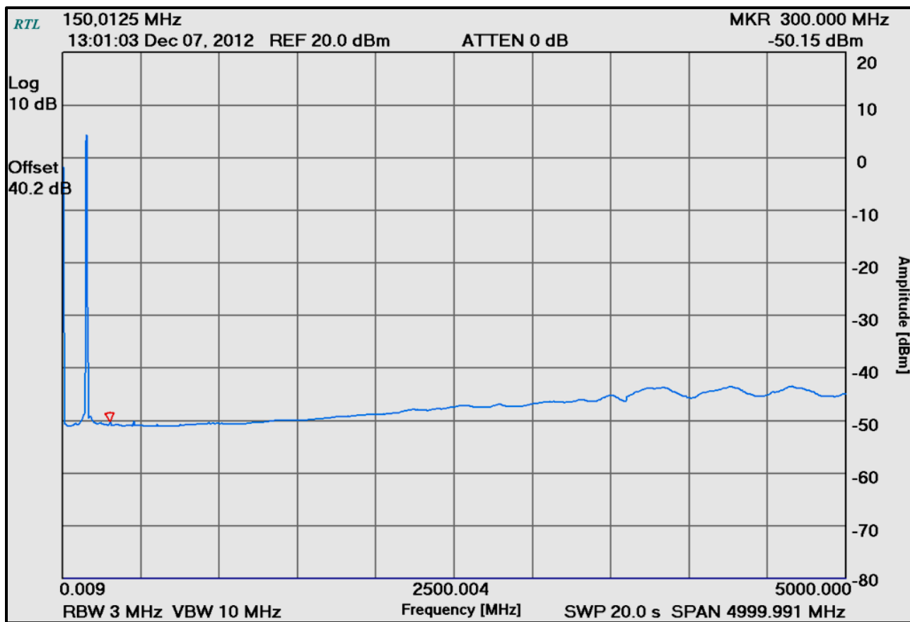
Plot 6-6: Spurious Emissions at Antenna Terminals – 150.0125 MHz
