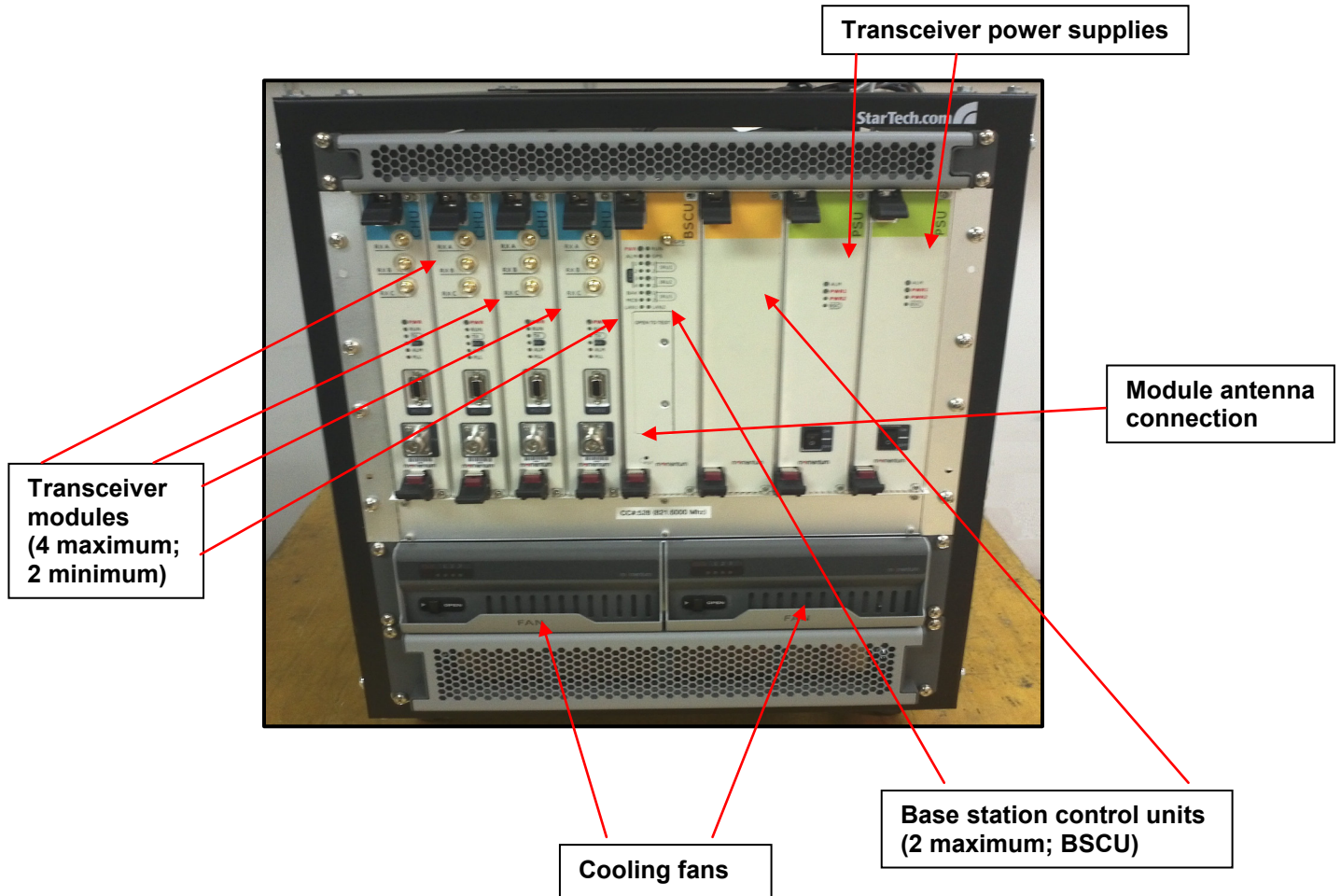
Photograph 1: EUT Configuration
