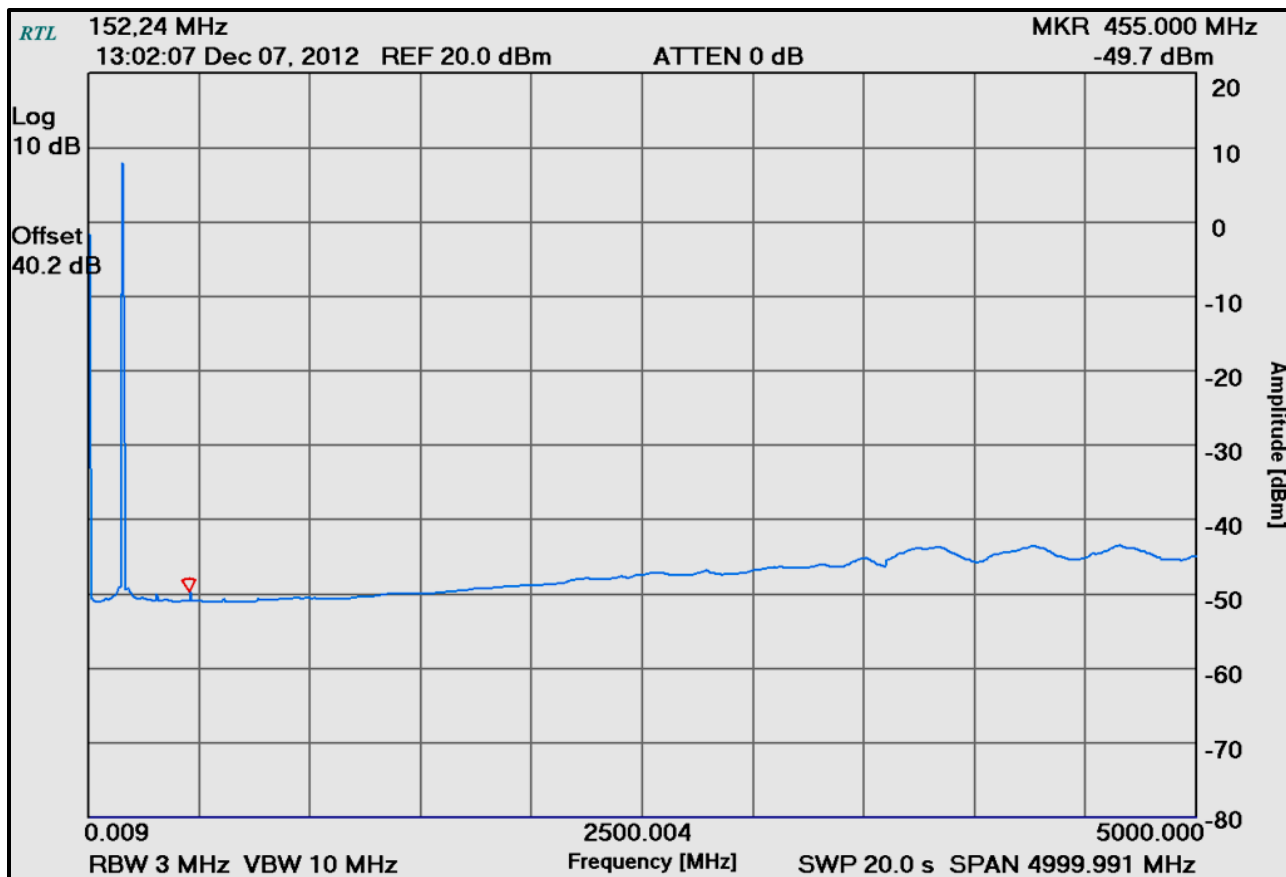
Plot 6-7: Spurious Emissions at Antenna Terminals – 152.2400 MHz
