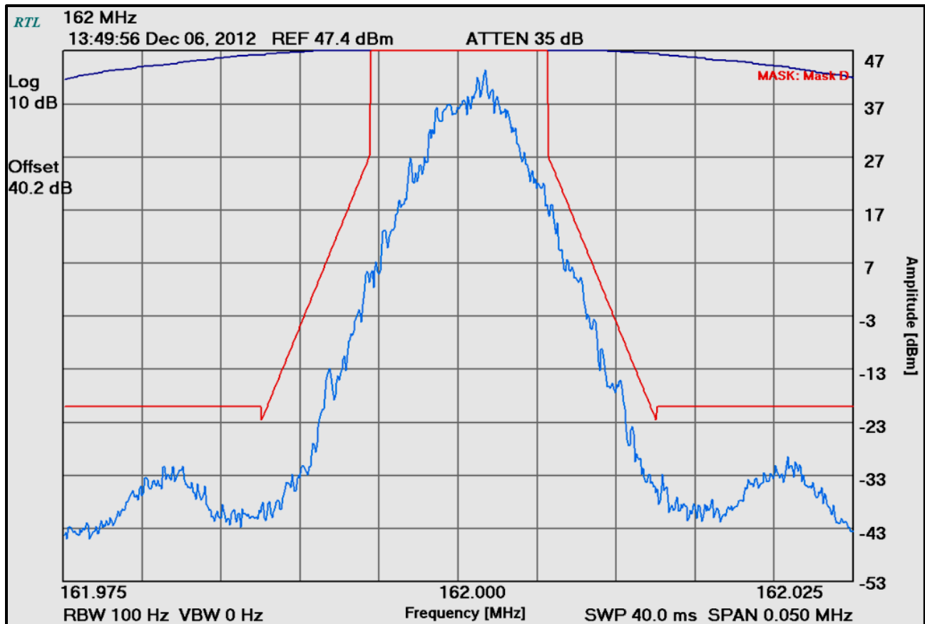
Plot 8-10: Occupied Bandwidth – 162.000 MHz; Mask D
