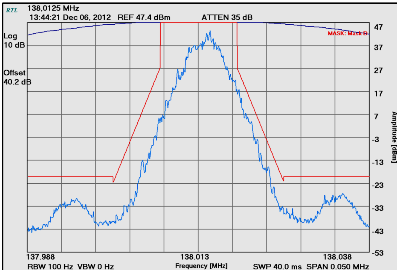
Plot 8-2: Occupied Bandwidth – 138.0125 MHz; Mask D
