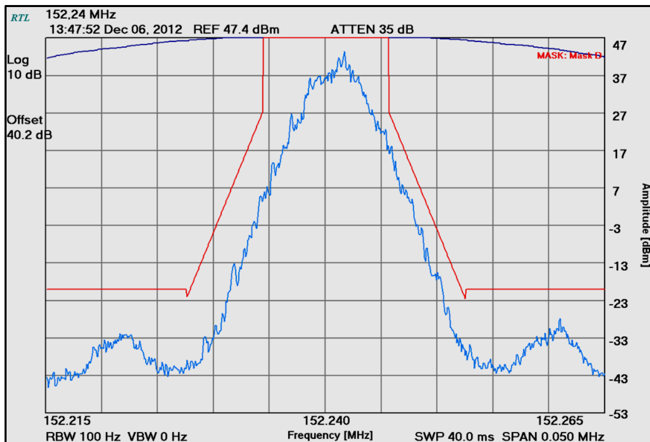
Plot 8-7: Occupied Bandwidth – 152.240 MHz; Mask D
