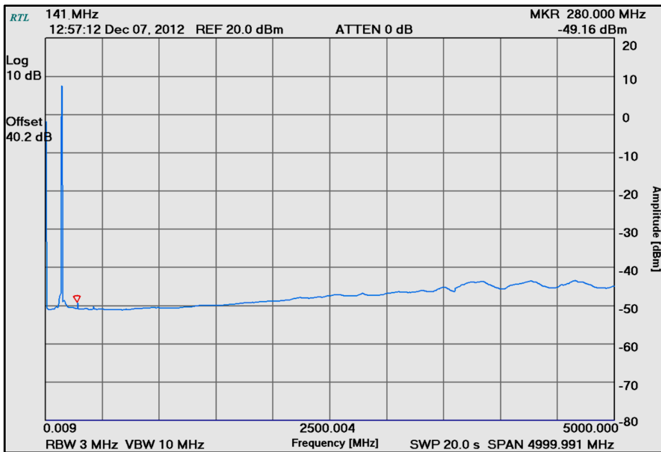
Plot 6-3: Spurious Emissions at Antenna Terminals – 141.0000 MHz
