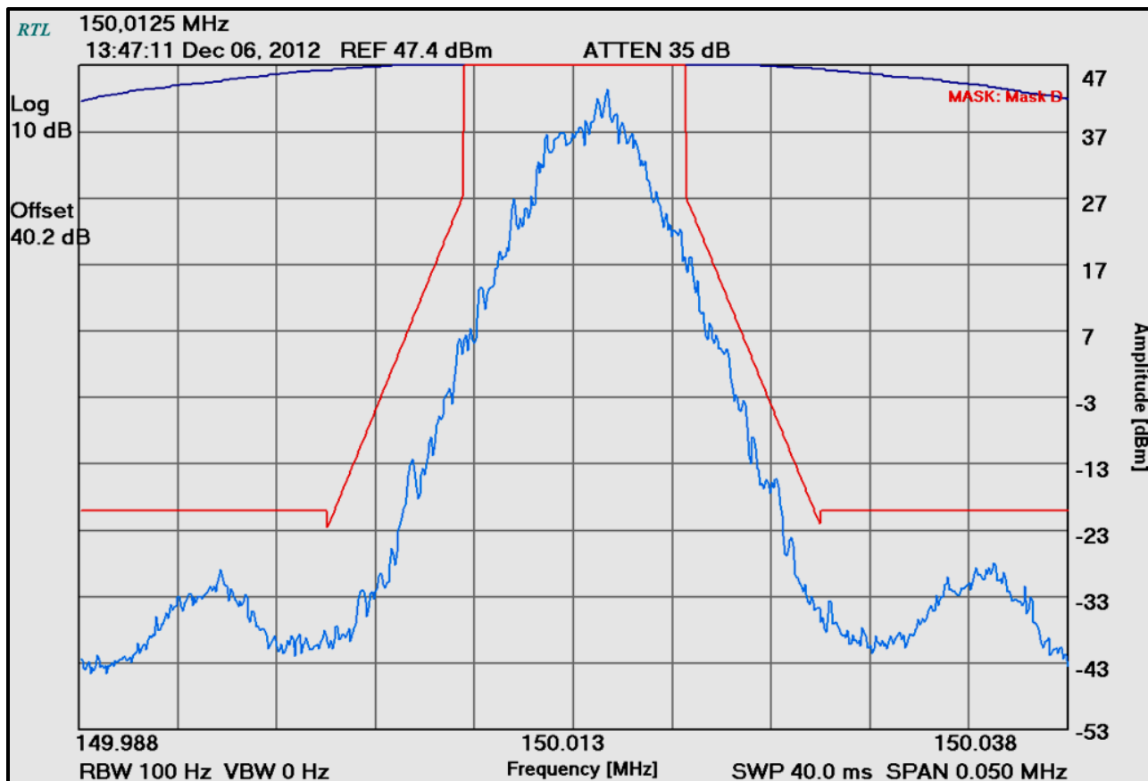
Plot 8-6: Occupied Bandwidth – 150.0125 MHz; Mask D
