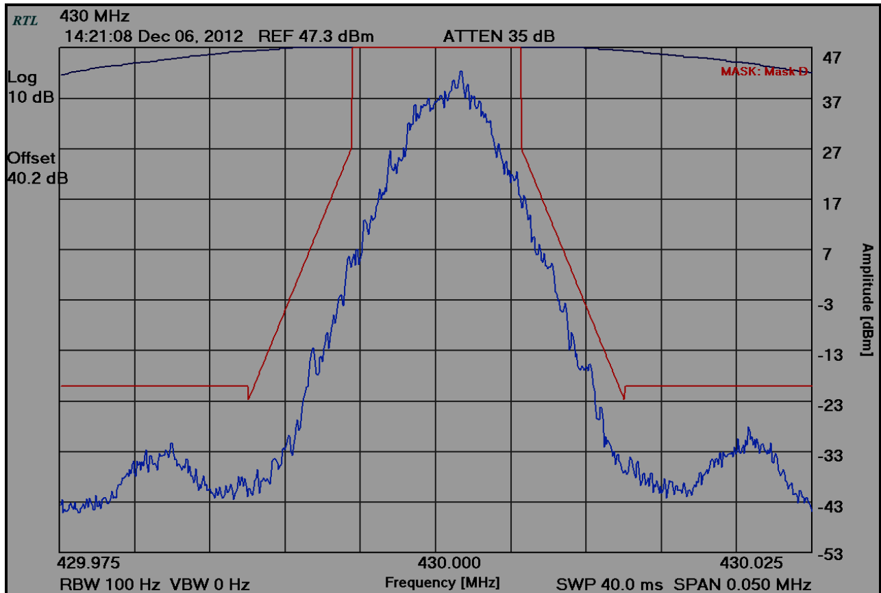
Plot 8-4: Occupied Bandwidth – 430.0000 MHz; Mask D
