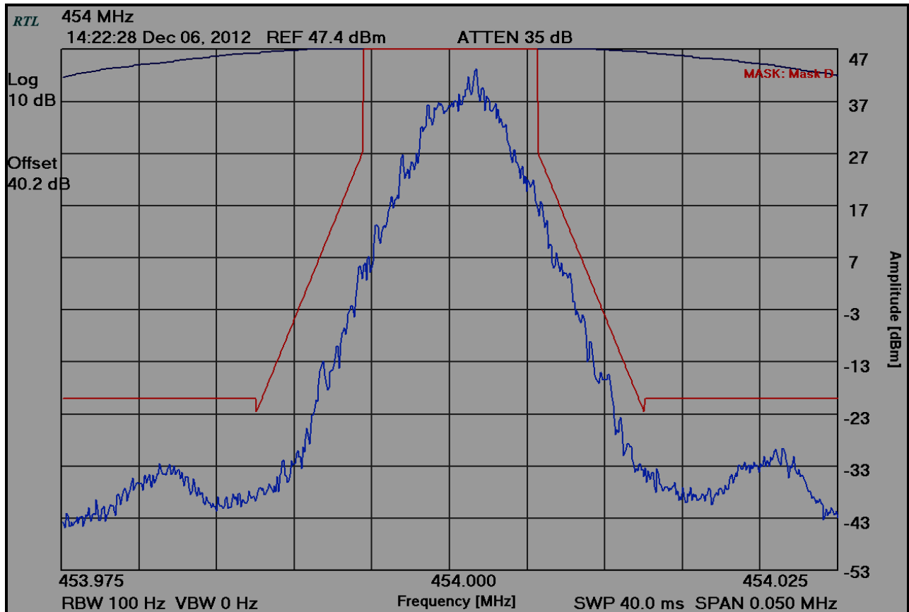
Plot 8-6: Occupied Bandwidth – 454.0000 MHz; Mask D
