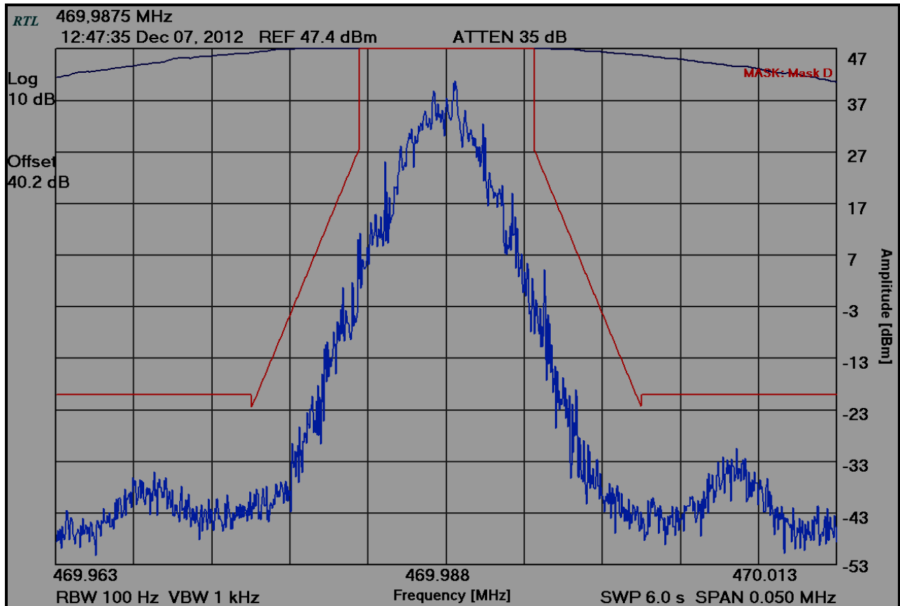
Plot 8-8: Occupied Bandwidth – 469.9875 MHz; Mask D
