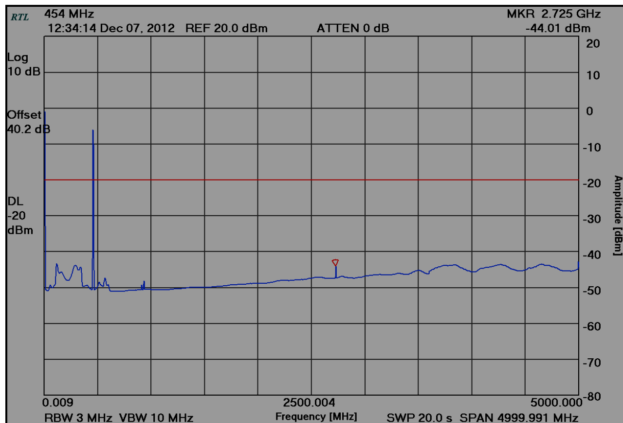
Plot 6-6: Spurious Emissions at Antenna Terminals – 454.0000 MHz
