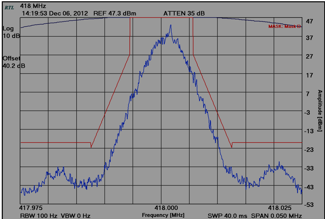
Plot 8-3: Occupied Bandwidth – 418.0000 MHz; Mask D
