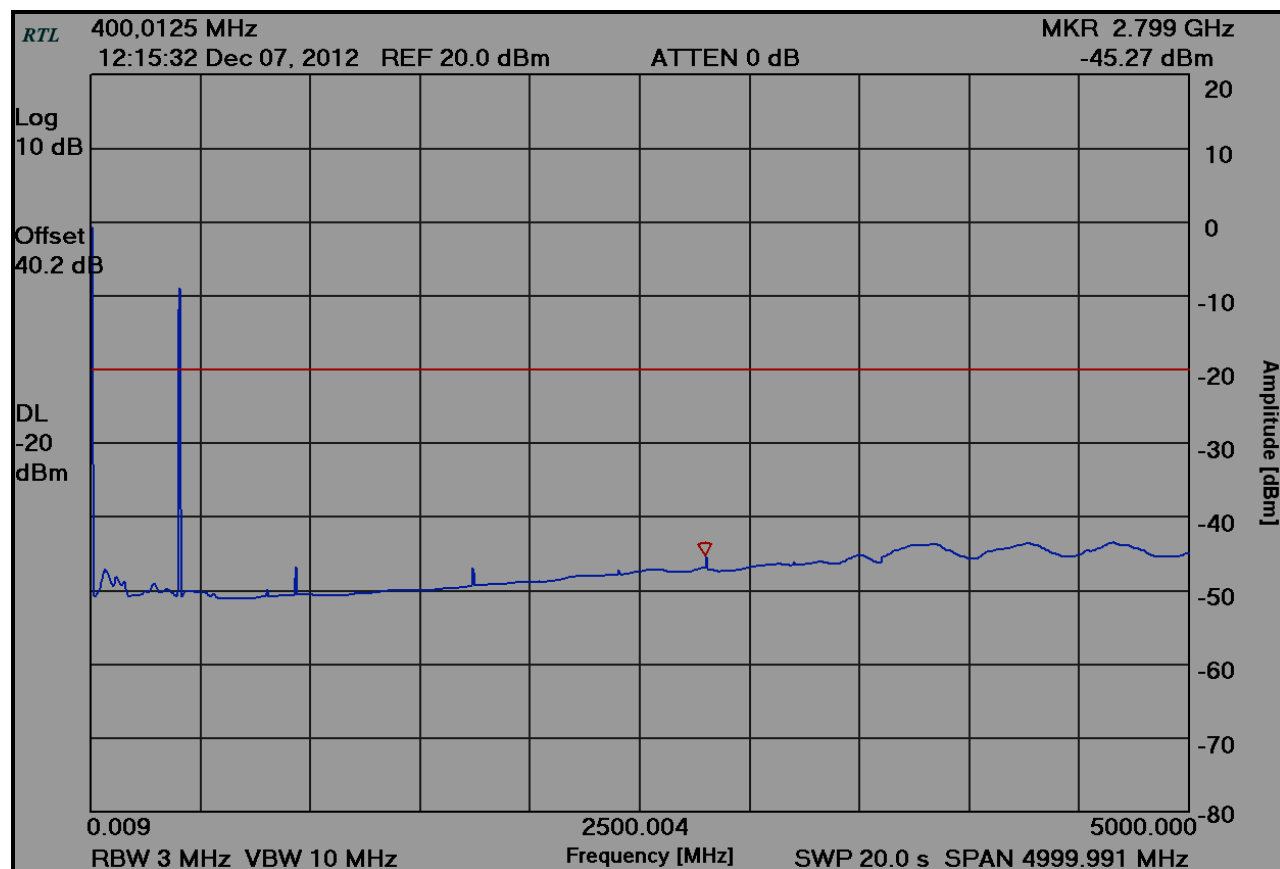
Plot 6-1: Spurious Emissions at Antenna Terminals – 400.0125 MHz
