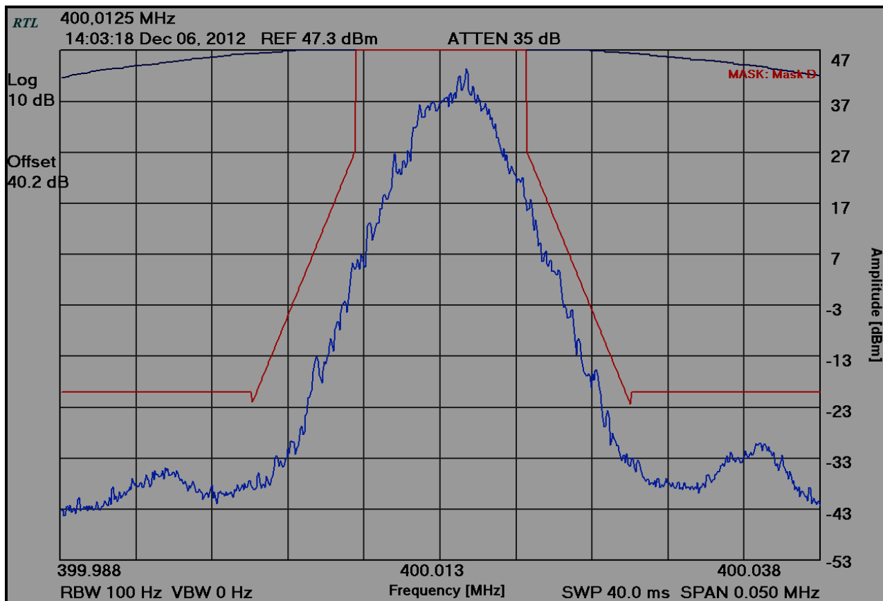
Plot 8-1: Occupied Bandwidth – 400.0125 MHz; Mask D
