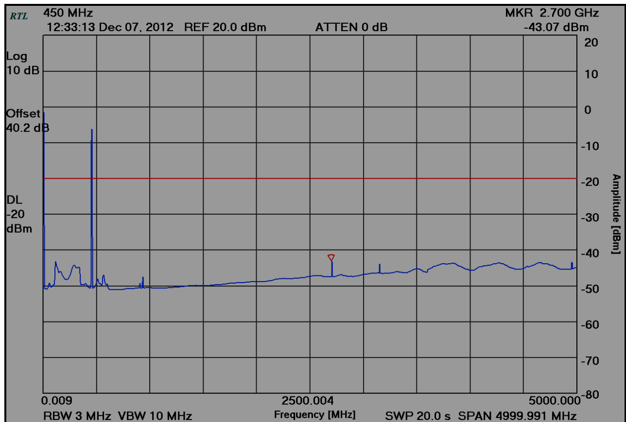
Plot 6-5: Spurious Emissions at Antenna Terminals – 450.0000 MHz
