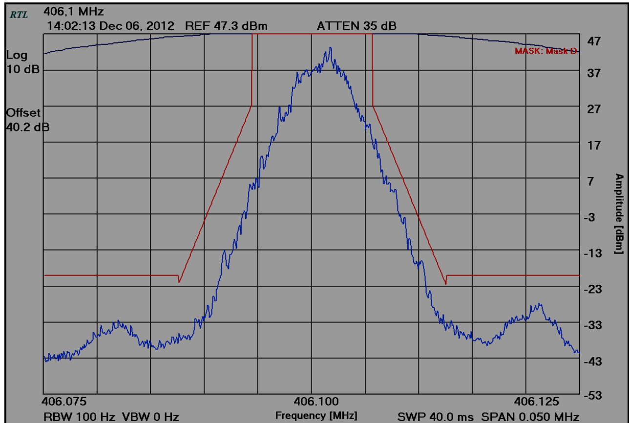
Plot 8-2: Occupied Bandwidth – 406.1000 MHz; Mask D
