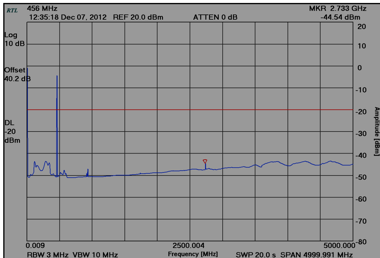
Plot 6-7: Spurious Emissions at Antenna Terminals – 456.0000 MHz
