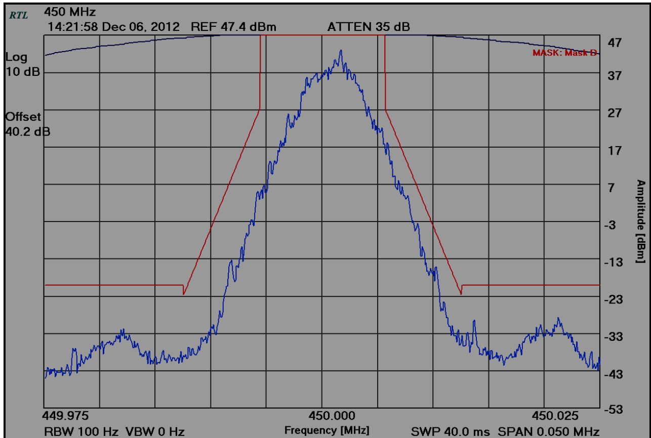
Plot 8-5: Occupied Bandwidth – 450.0000 MHz; Mask D
