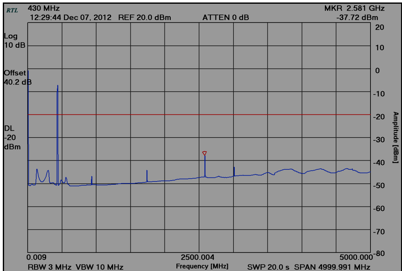
Plot 6-4: Spurious Emissions at Antenna Terminals – 430.0000 MHz
