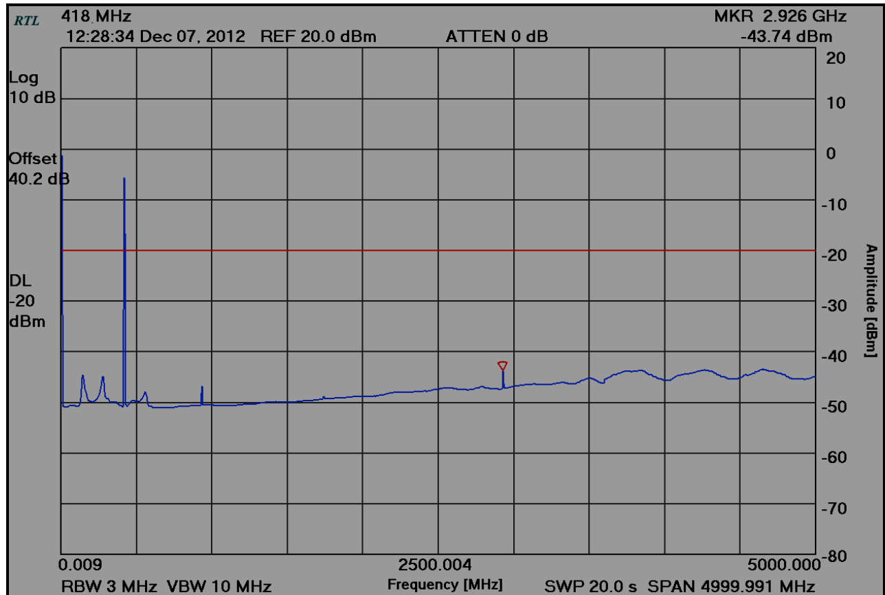
Plot 6-3: Spurious Emissions at Antenna Terminals – 418.0000 MHz
