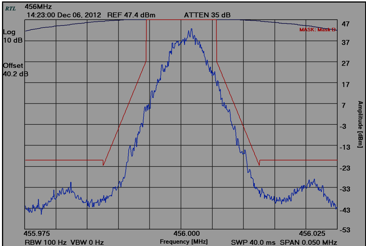
Plot 8-7: Occupied Bandwidth – 456.0000 MHz; Mask D
