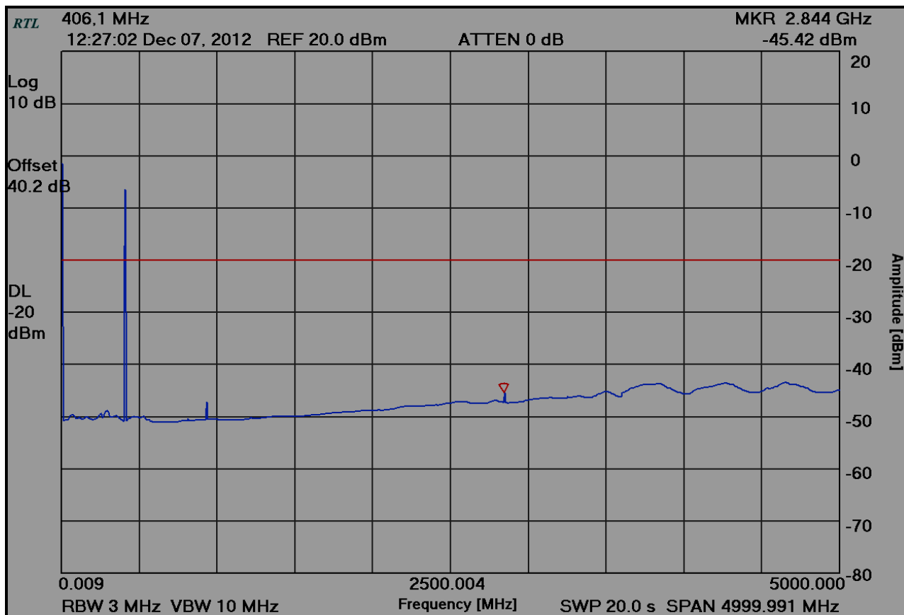
Plot 6-2: Spurious Emissions at Antenna Terminals – 406.1000 MHz
