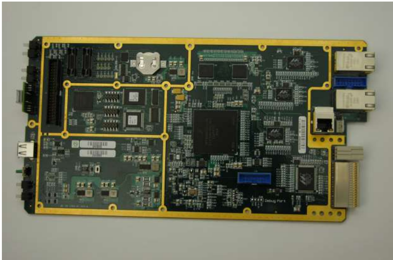
Photograph 16. Traffic Controller - Top Side
