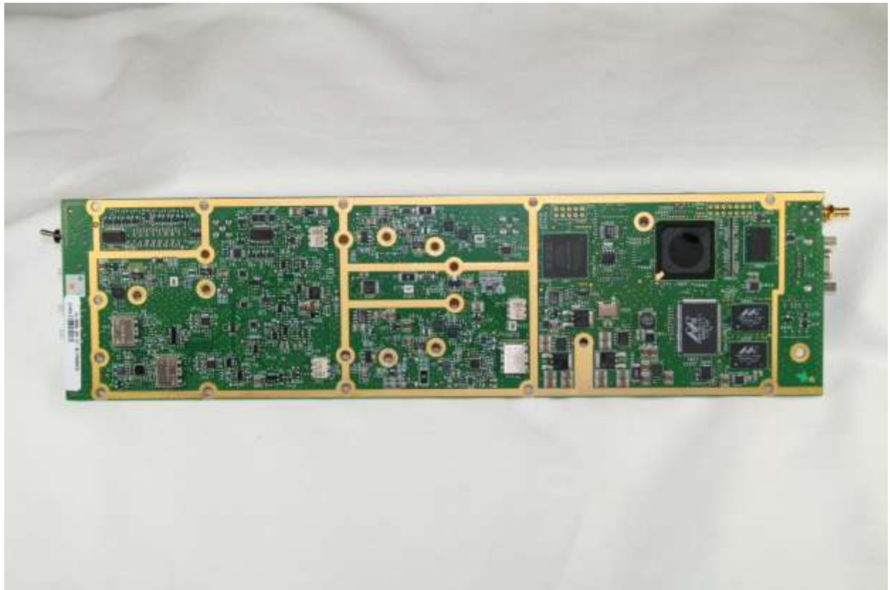
Photograph 4. Linearizer (470-520MHz) Top
