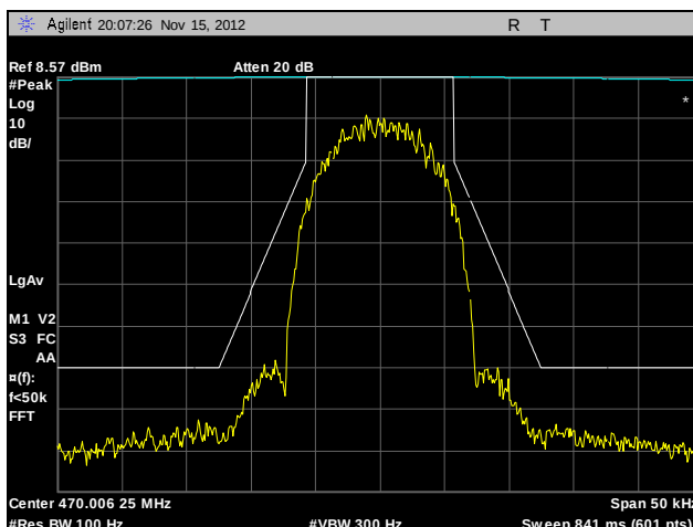
Plot 25. Emission Mask, 470.00625 MHz, HDQPSK, 10 W
