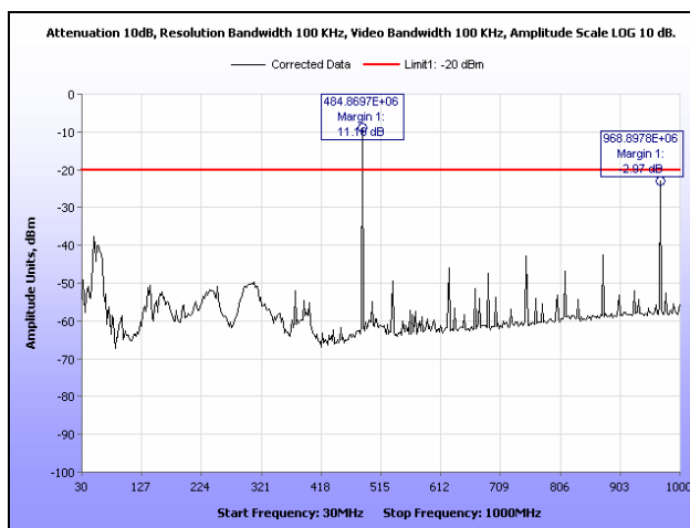
Plot 82. Radiated Spurious Emissions, Channel 2, C4FM, 30 MHz – 1 GHz, 100 W
