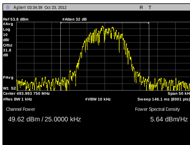
Plot 21. RF Power Output, 493.99375 MHz, 100W, CQPSK
