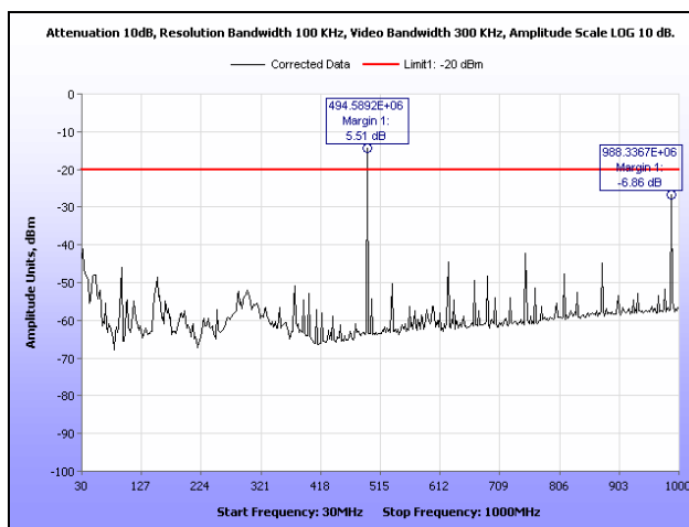
Plot 94. Radiated Spurious Emissions, 493.99375 MHz, C4FM, 30 MHz – 1 GHz, 100 W
