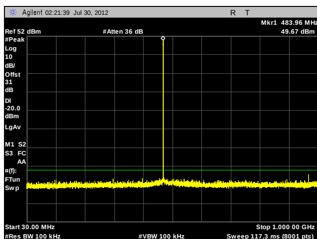
Plot 50. Conducted Spurious Emissions, 484.00625 MHz, C4FM, 30 MHz – 1 GHz
