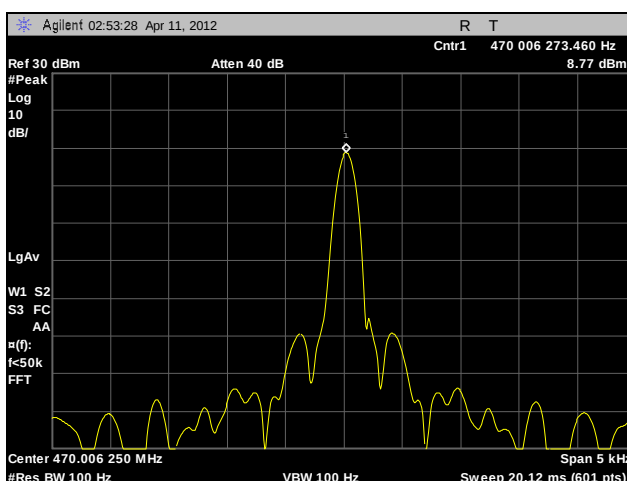
Plot 107. Frequency Stability, Channel 1, 0°C, 120 V
