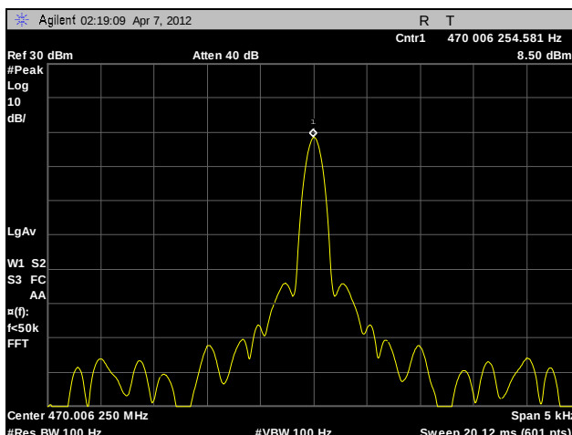
Plot 112. Frequency Stability, Channel 1, 30°C, 120 V
