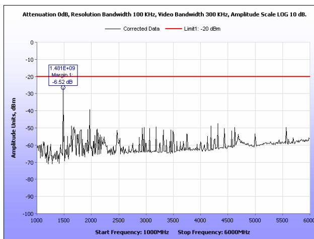
Plot 103. Radiated Spurious Emissions, 493.99375 MHz, HDQPSK, 1 GHz – 6 GHz, 100 W
