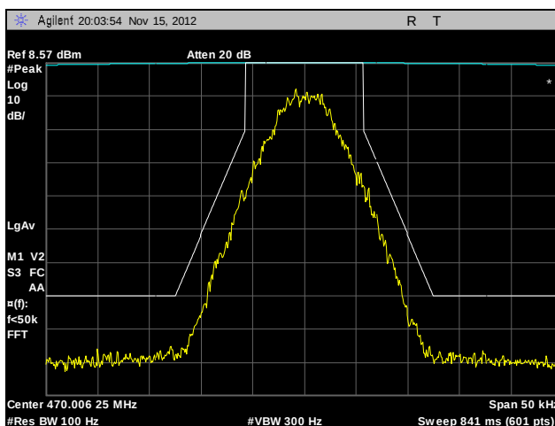
Plot 23. Emission Mask, 470.00625 MHz, C4FM, 10 W
