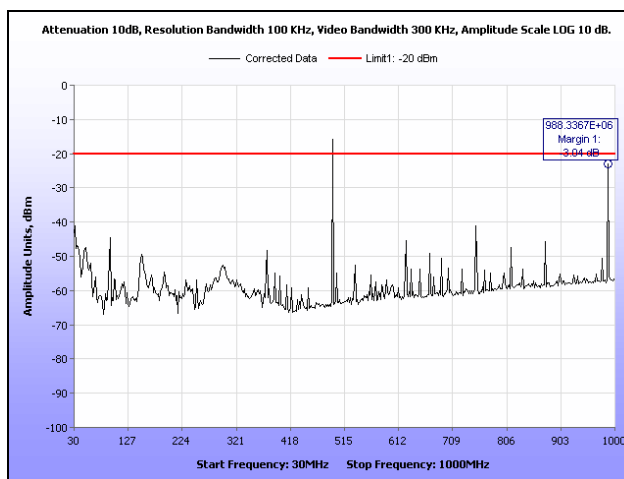
Plot 102. Radiated Spurious Emissions, 493.99375 MHz, HDQPSK, 30 MHz – 1 GHz, 100 W
