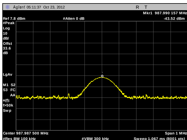
Plot 63. Conducted Spurious Emissions, 493.99375 MHz, CQPSK, 2 nd Harmonic
