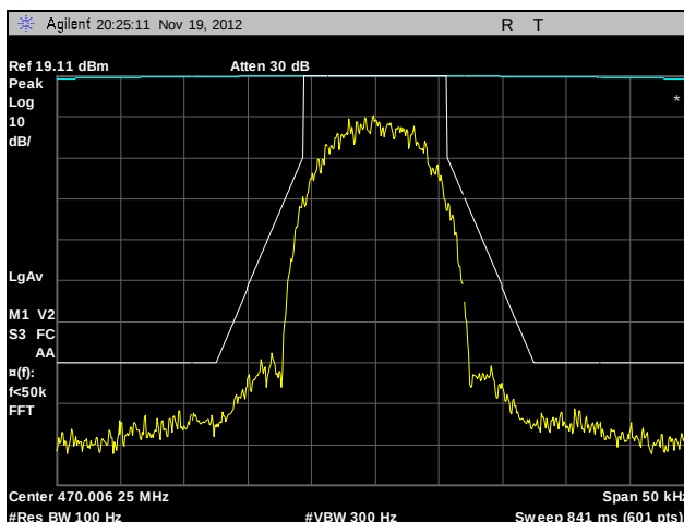
Plot 28. Emission Mask, 470.00625 MHz, HDQPSK, 100 W
