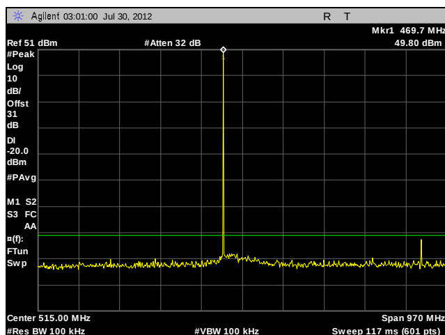
Plot 41. Conducted Spurious Emissions, 470.00625 MHz, C4FM, 30 MHz – 1 GHz
