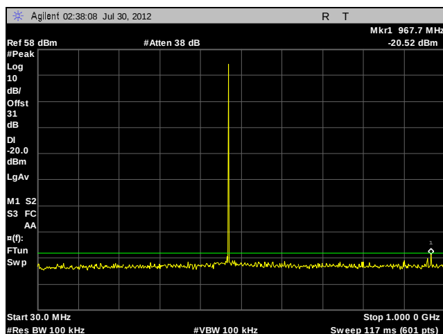
Plot 56. Conducted Spurious Emissions, 484.00625 MHz, HDQPSK, 30 MHz – 1 GHz
