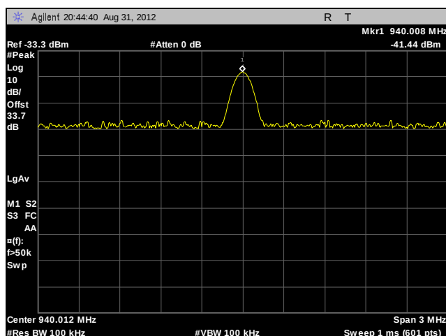
Plot 45. Conducted Spurious Emissions, 470.00625 MHz, CQPSK, 2 nd Harmonic
