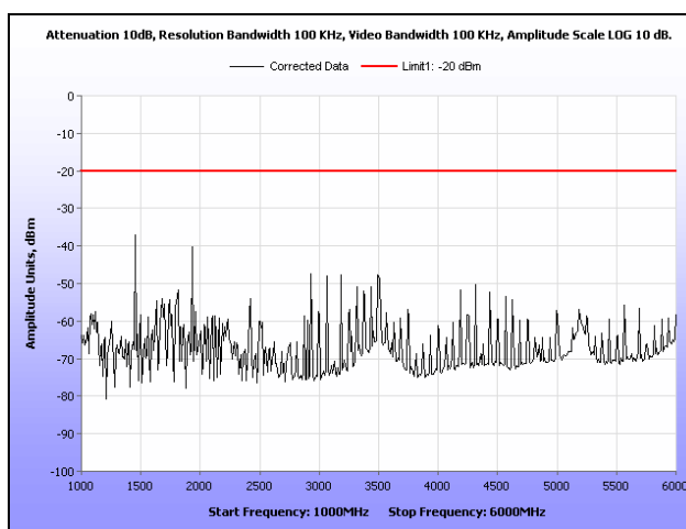
Plot 83. Radiated Spurious Emissions, Channel 2, C4FM, 1 GHz – 6 GHz, 100 W
