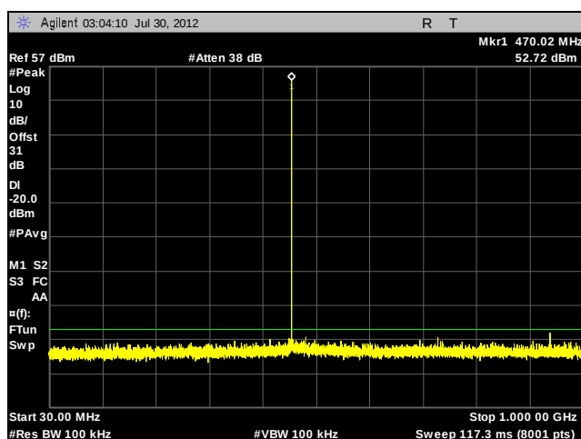
Plot 44. Conducted Spurious Emissions, 470.00625 MHz, CQPSK, 30 MHz – 1 GHz
