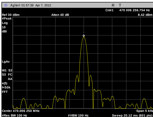
Plot 114. Frequency Stability, Channel 1, 50°C, 120 V
