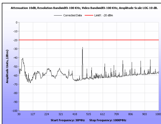
Plot 72. Radiated Spurious Emissions, Channel 1, CQPSK, 30 MHz – 1 GHz, 10 W
