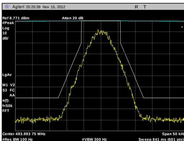
Plot 35. Emission Mask, 493.99375 MHz, C4FM, 10 W
