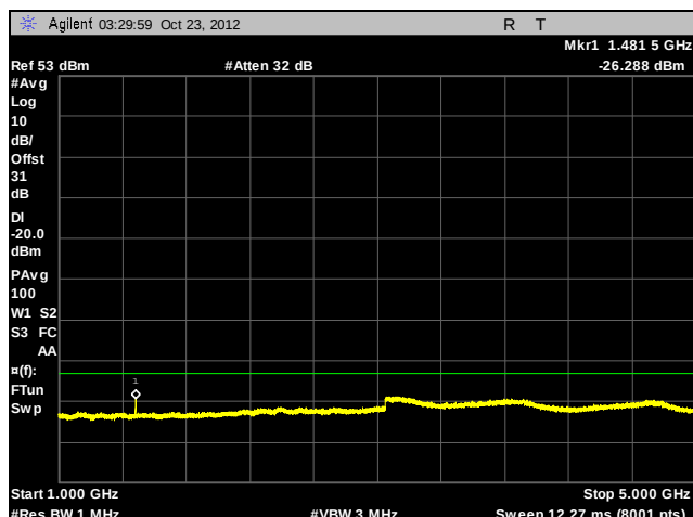
Plot 67. Conducted Spurious Emissions, 493.99375 MHz, HDQPSK, 1 GHz – 5 GHz
