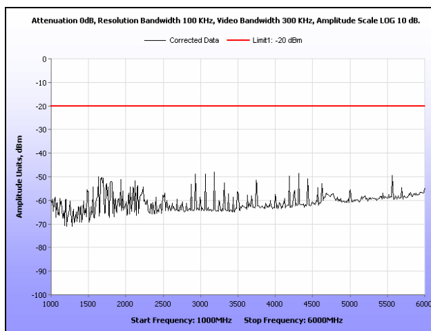
Plot 101. Radiated Spurious Emissions, 493.99375 MHz, HDQPSK, 1 GHz – 6 GHz, 10 W
