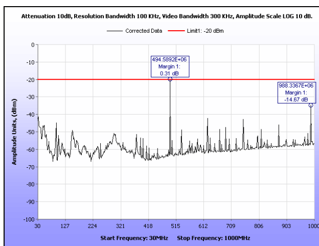
Plot 92. Radiated Spurious Emissions, 493.99375 MHz, C4FM, 30 MHz – 1 GHz, 10 W
