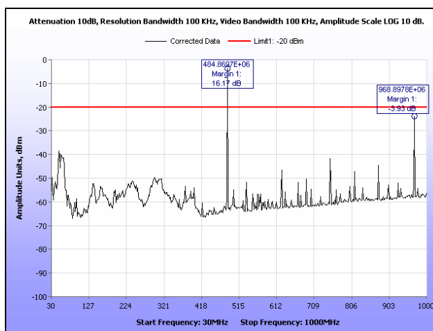
Plot 86. Radiated Spurious Emissions, Channel 2, CQPSK, 30 MHz – 1 GHz, 100 W
