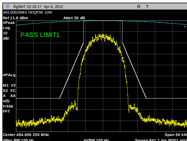
Plot 31. Emission Mask, 484.00625 MHz, HDQPSK, 10 W
