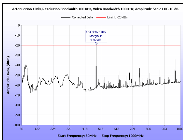
Plot 84. Radiated Spurious Emissions, Channel 2, CQPSK, 30 MHz – 1 GHz, 10 W
