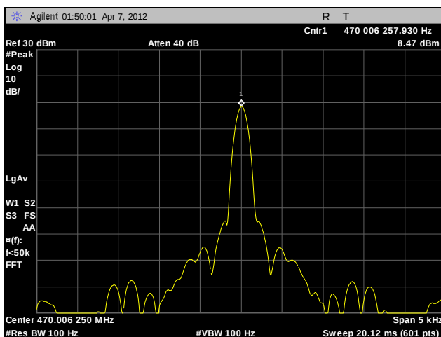
Plot 113. Frequency Stability, Channel 1, 40°C, 120 V
