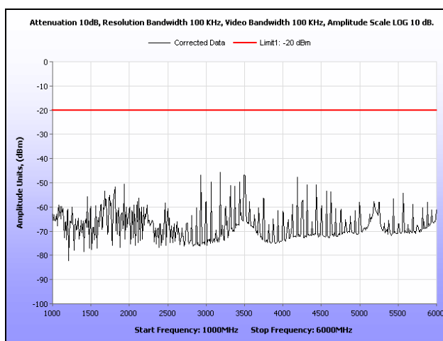
Plot 89. Radiated Spurious Emissions, Channel 2, HDQPSK, 1 GHz – 6 GHz, 10 W
