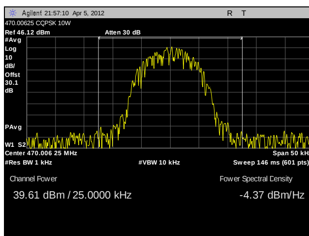
Plot 6. RF Power Output, 470.00625 MHz, 10W, CQPSK
