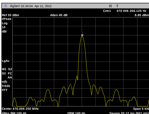
Plot 104. Frequency Stability, Channel 1, -30°C, 120 V
