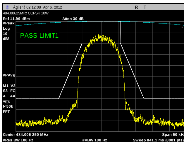
Plot 30. Emission Mask, 484.00625 MHz, CQPSK, 10 W
