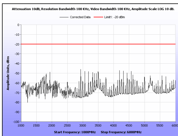
Plot 77. Radiated Spurious Emissions, Channel 1, HKQPSK, 1 GHz – 6 GHz, 10 W
