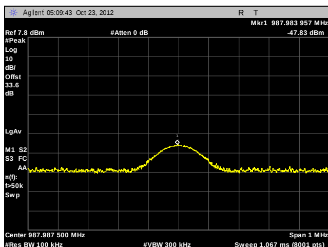
Plot 60. Conducted Spurious Emissions, 493.99375 MHz, C4FM, 2 nd Harmonic
