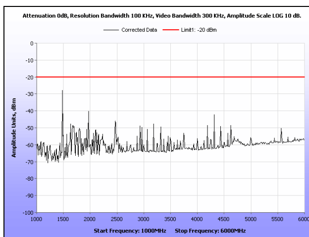
Plot 99. Radiated Spurious Emissions, 493.99375 MHz, CQPSK, 1 GHz – 6 GHz, 100 W
