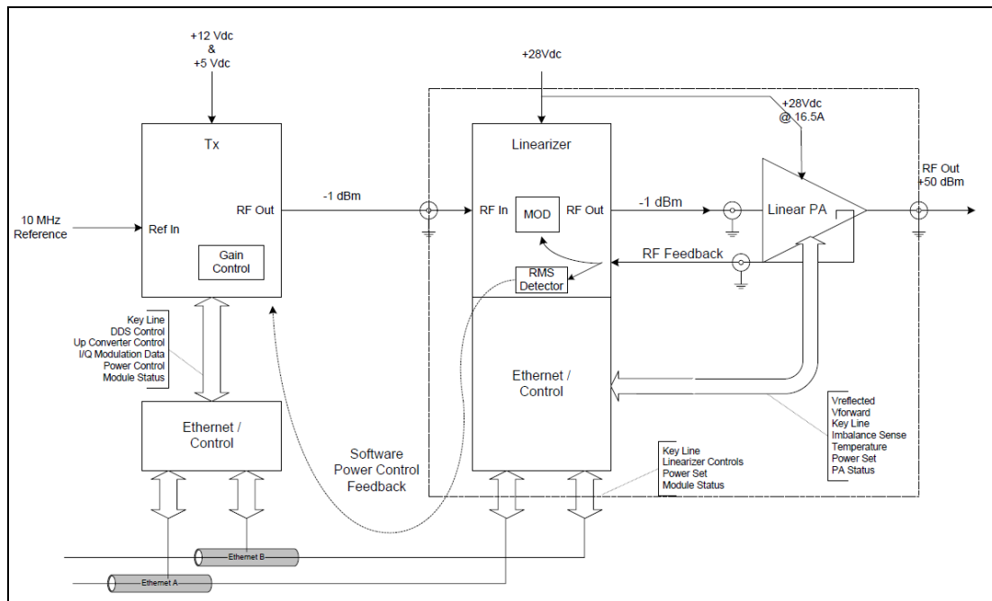
Figure 2. Transmitter Lineup Block Diagram
