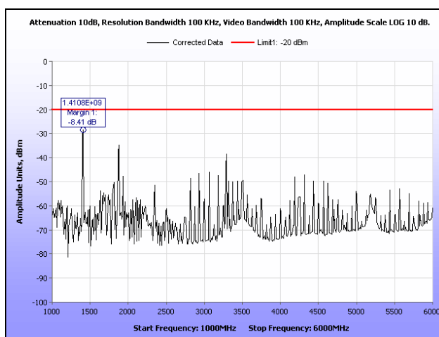
Plot 75. Radiated Spurious Emissions, Channel 1, CQPSK, 1 GHz – 6 GHz, 100 W
