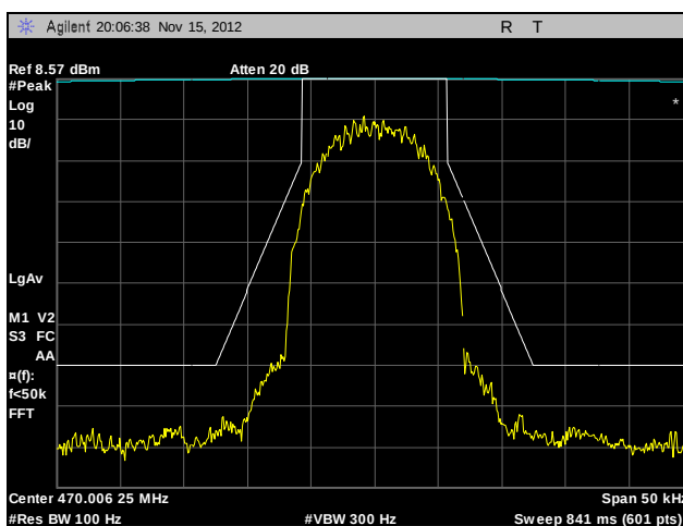
Plot 24. Emission Mask, 470.00625 MHz, CQPSK, 10 W
