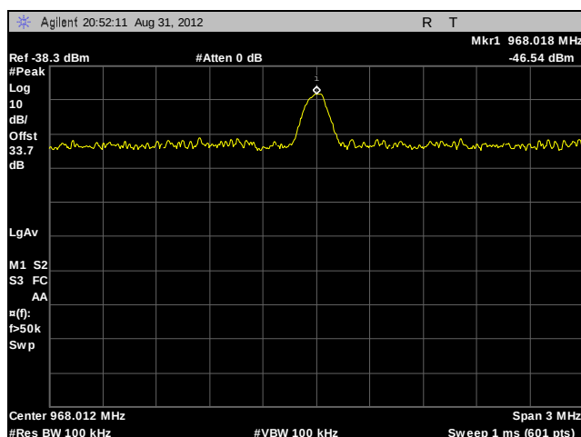
Plot 57. Conducted Spurious Emissions, 484.00625 MHz, HDQPSK, 2 nd Harmonic
