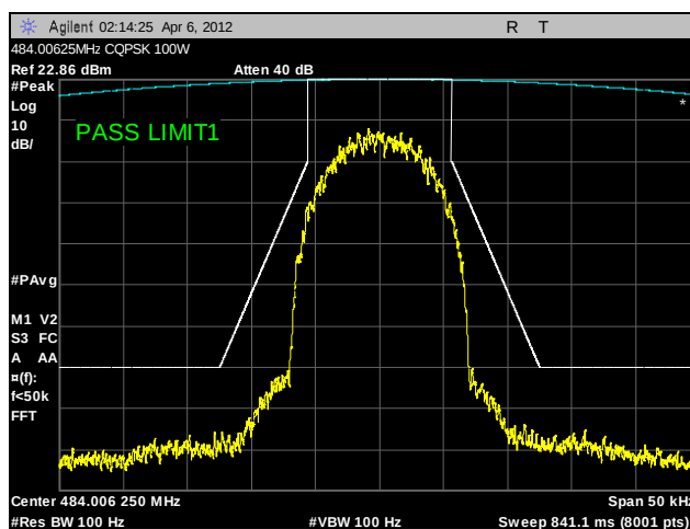
Plot 33. Emission Mask, 484.00625 MHz, CQPSK, 100 W
