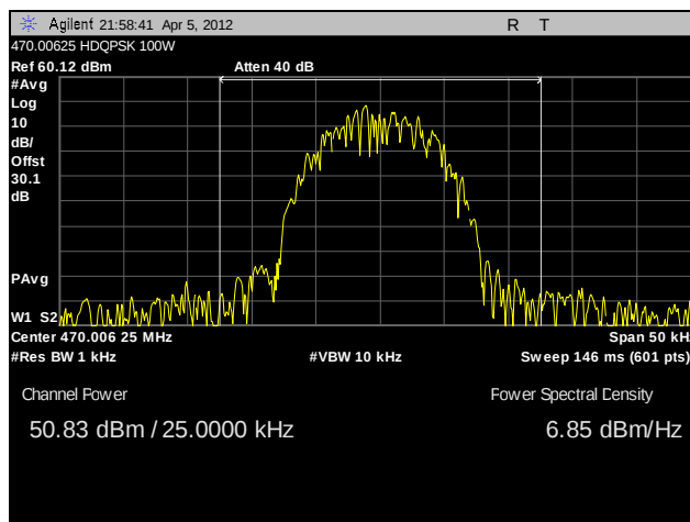
Plot 10. RF Power Output, 470.00625 MHz, 100W, HDQPSK
