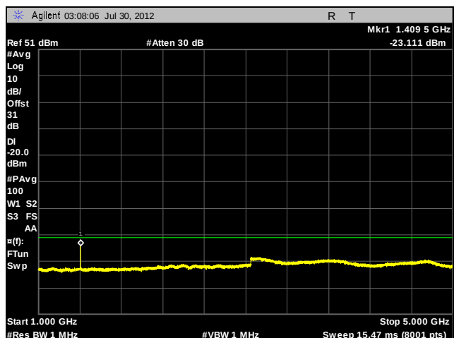
Plot 49. Conducted Spurious Emissions, 470.00625 MHz, HDQPSK, 1 GHz – 5 GHz
