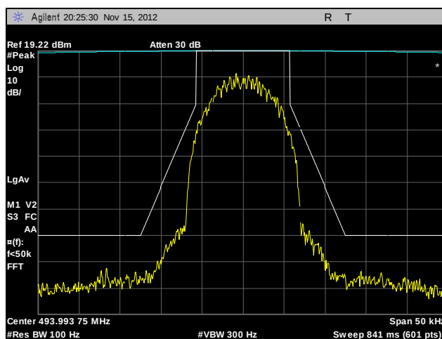
Plot 39. Emission Mask, 493.99375 MHz, CQPSK, 100 W
