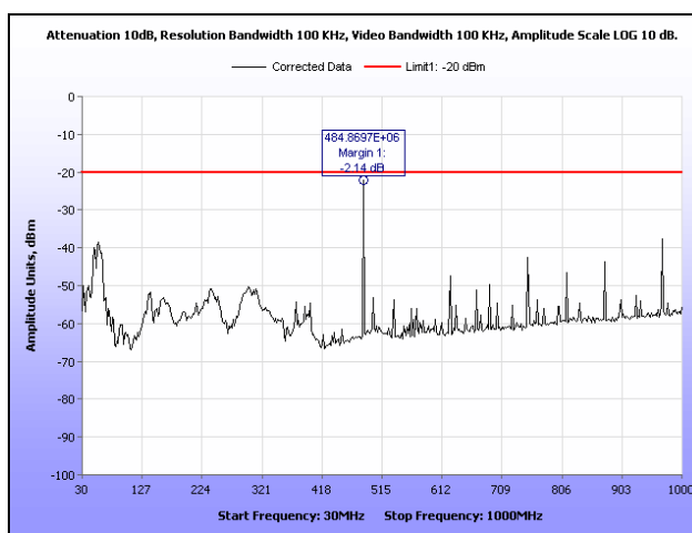
Plot 80. Radiated Spurious Emissions, Channel 2, C4FM, 30 MHz – 1 GHz, 10 W
