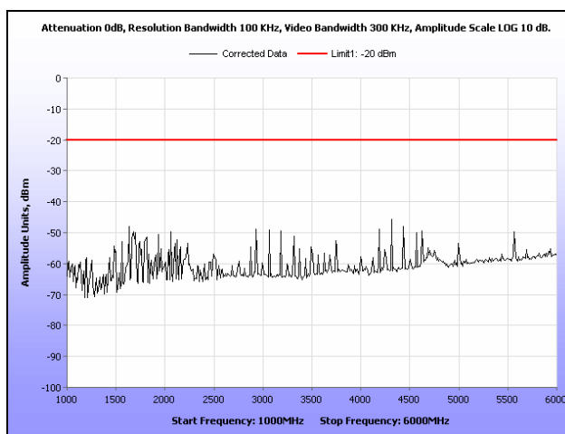
Plot 93. Radiated Spurious Emissions, 493.99375 MHz, C4FM, 1 GHz – 6 GHz, 10 W
