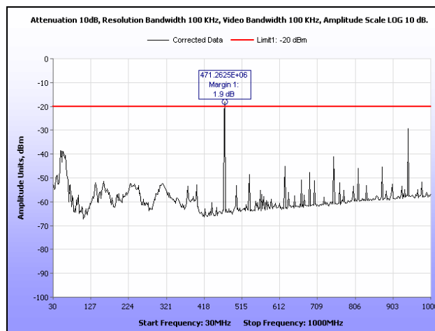
Plot 70. Radiated Spurious Emissions, Channel 1, C4FM, 30 MHz – 1 GHz, 100 W
