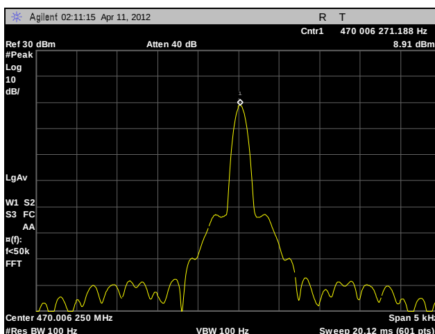
Plot 105. Frequency Stability, Channel 1, -20°C, 120 V
