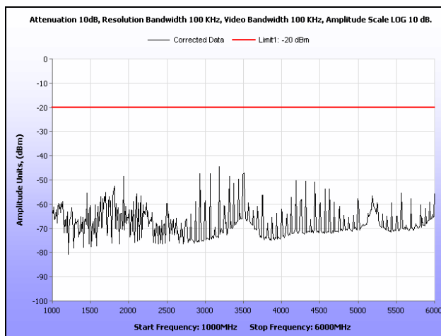
Plot 85. Radiated Spurious Emissions, Channel 2, CQPSK, 1 GHz – 6 GHz, 10 W
