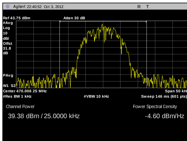
Plot 7. RF Power Output, 470.00625 MHz, 10W, HDQPSK
