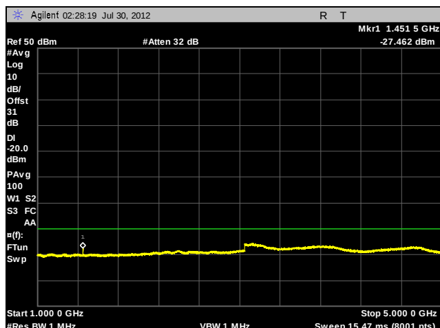
Plot 52. Conducted Spurious Emissions, 484.00625 MHz, C4FM, 1 GHz – 5 GHz
