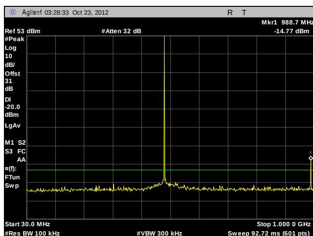
Plot 62. Conducted Spurious Emissions, 493.99375 MHz, CQPSK, 30 MHz – 1 GHz
