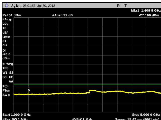
Plot 43. Conducted Spurious Emissions, 470.00625 MHz, C4FM, 1 GHz – 5 GHz
