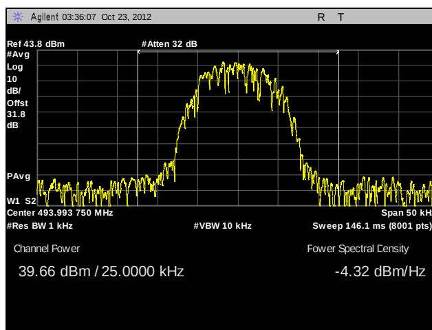
Plot 18. RF Power Output, 493.99375 MHz, 10W, CQPSK
