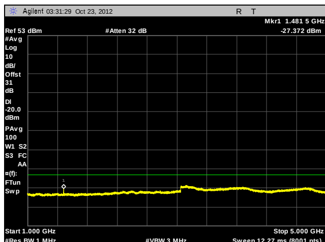
Plot 61. Conducted Spurious Emissions, 493.99375 MHz, C4FM, 1 GHz – 5 GHz
