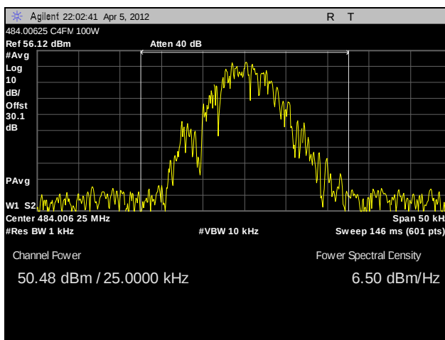
Plot 14. RF Power Output, 484.00625 MHz, 100W, C4FM
