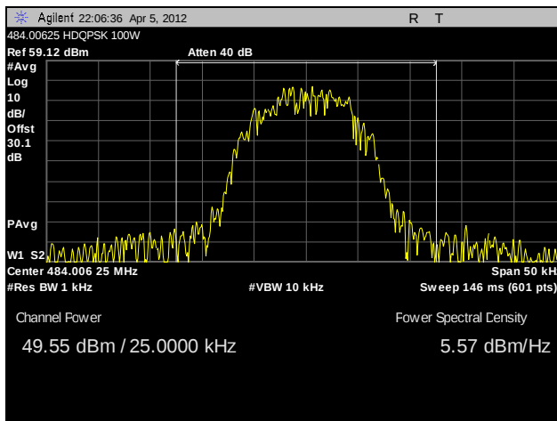
Plot 16. RF Power Output, 484.00625 MHz, 100W, HDQPSK
