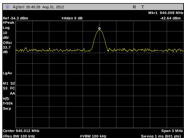
Plot 48. Conducted Spurious Emissions, 470.00625 MHz, HDQPSK, 2 nd Harmonic
