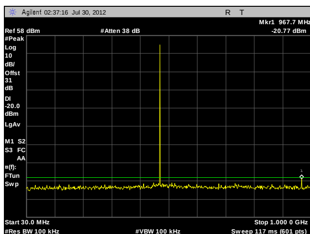
Plot 53. Conducted Spurious Emissions, 484.00625 MHz, CQPSK, 30 MHz – 1 GHz
