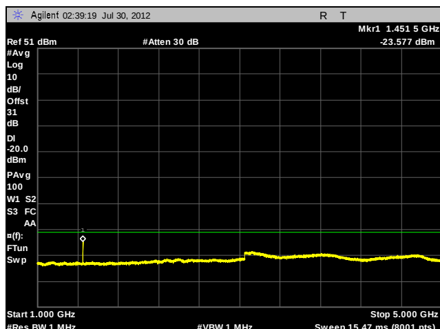
Plot 58. Conducted Spurious Emissions, 484.00625 MHz, HDQPSK, 1 GHz – 5 GHz
