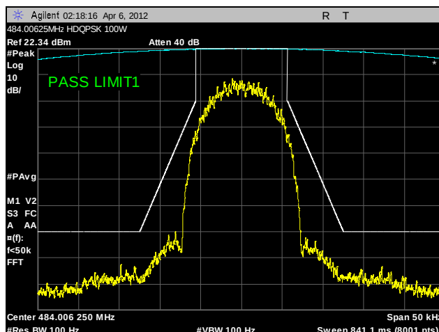
Plot 34. Emission Mask, 484.00625 MHz, HDQPSK, 100 W
