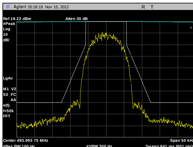
Plot 40. Emission Mask, 493.99375 MHz, HDQPSK, 100 W
