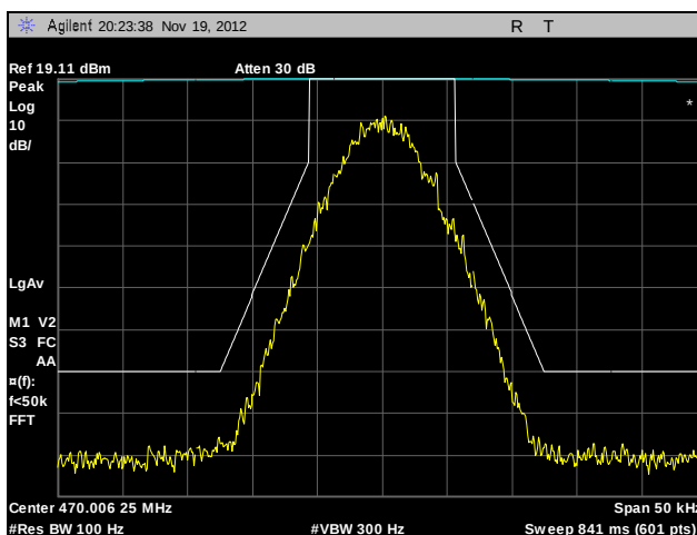
Plot 26. Emission Mask, 470.00625 MHz, C4FM, 100 W
