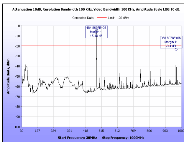
Plot 90. Radiated Spurious Emissions, Channel 2, HDQPSK, 30 MHz – 1 GHz, 100 W
