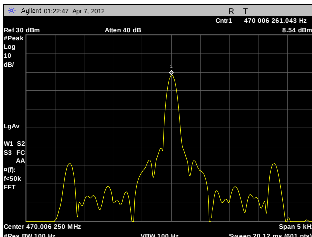
Plot 109. Frequency Stability, Channel 1, 20°C, 108 V
