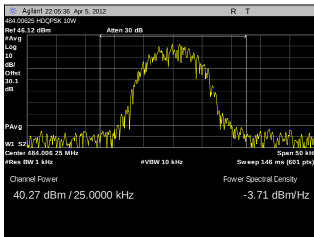
Plot 13. RF Power Output, 484.00625 MHz, 10W, HDQPSK
