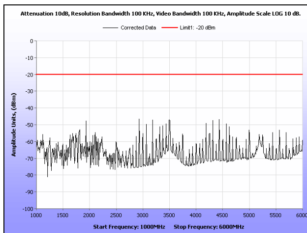
Plot 73. Radiated Spurious Emissions, Channel 1, CQPSK, 1 GHz – 6 GHz, 10 W
