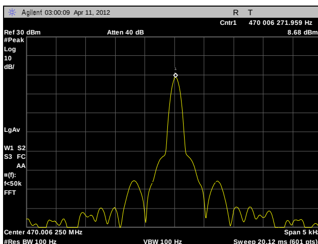
Plot 108. Frequency Stability, Channel 1, 10°C, 120 V
