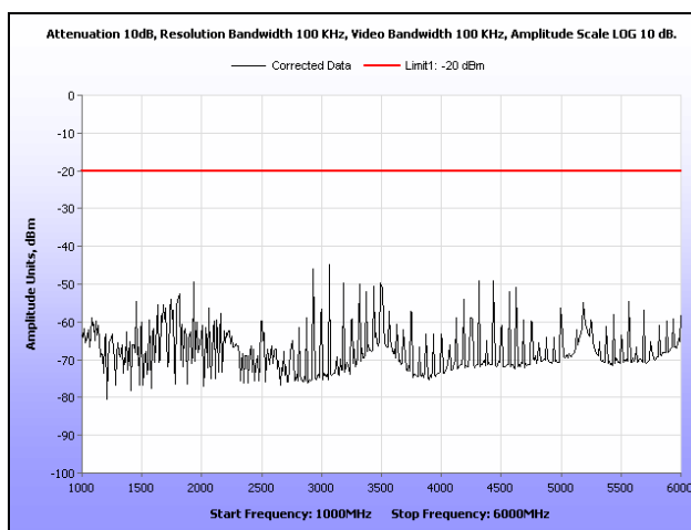
Plot 81. Radiated Spurious Emissions, Channel 2, C4FM, 1 GHz – 6 GHz, 10 W
