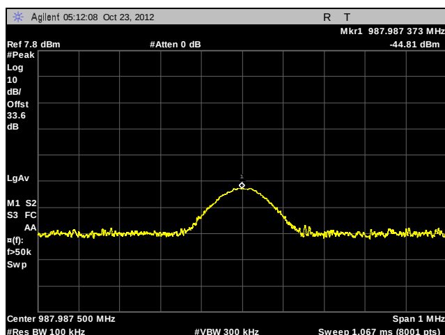
Plot 66. Conducted Spurious Emissions, 493.99375 MHz, HDQPSK, 2 nd Harmonic
