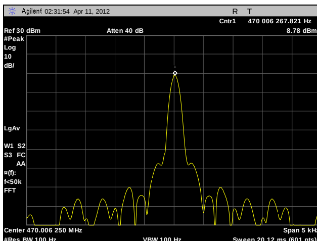
Plot 106. Frequency Stability, Channel 1, -10°C, 120 V
