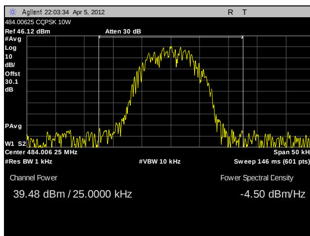
Plot 12. RF Power Output, 484.00625 MHz, 10W, CQPSK
