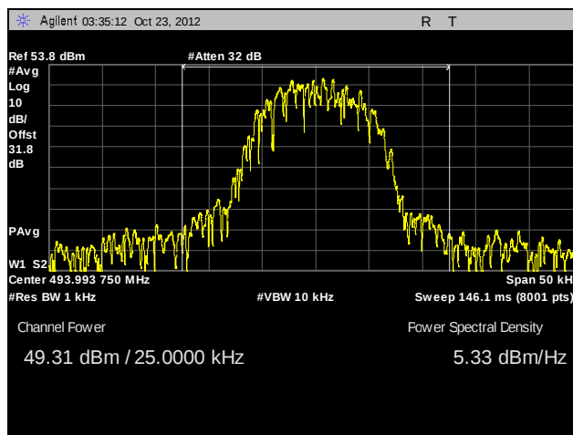
Plot 22. RF Power Output, 493.99375 MHz, 100W, HDQPSK
