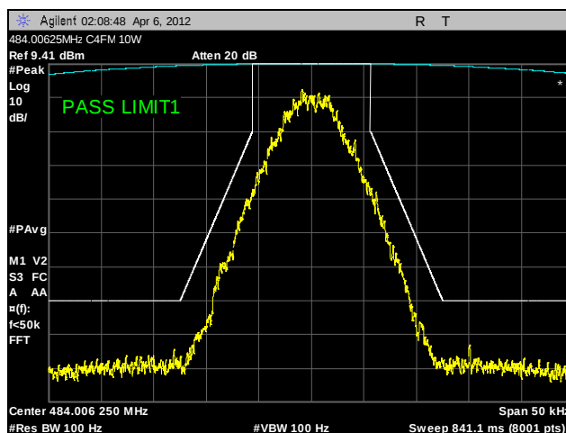
Plot 29. Emission Mask, 484.00625 MHz, C4FM, 10 W
