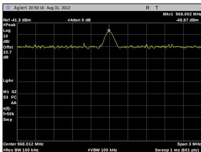
Plot 51. Conducted Spurious Emissions, 484.00625 MHz, C4FM, 2 nd Harmonic
