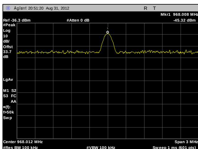
Plot 54. Conducted Spurious Emissions, 484.00625 MHz, CQPSK, 2 nd Harmonic
