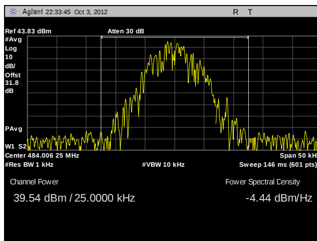
Plot 11. RF Power Output, 484.00625 MHz, 10W, C4FM
