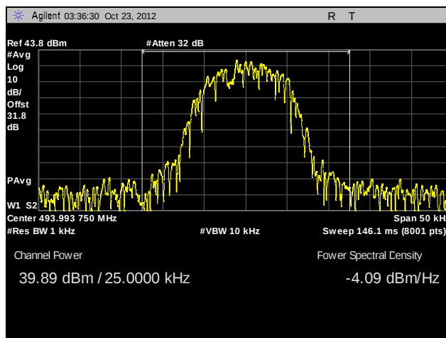
Plot 19. RF Power Output, 493.99375 MHz, 10W, HDQPSK
