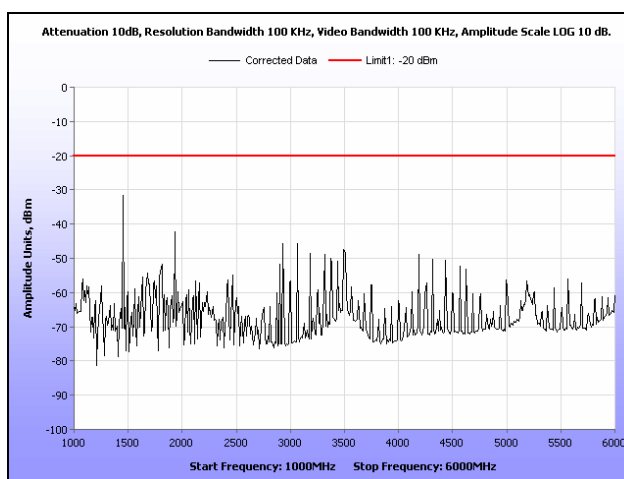
Plot 87. Radiated Spurious Emissions, Channel 2, CQPSK, 1 GHz – 6 GHz, 100 W
