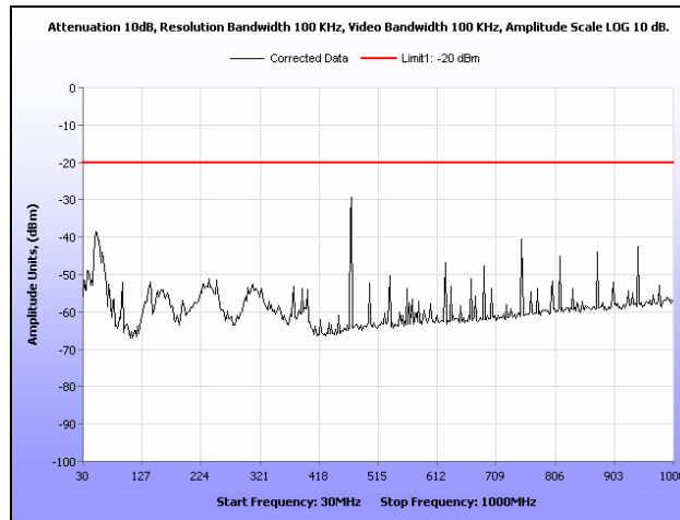
Plot 68. Radiated Spurious Emissions, Channel 1, C4FM, 30 MHz – 1 GHz, 10 W
