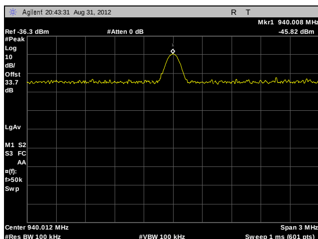
Plot 42. Conducted Spurious Emissions, 470.00625 MHz, C4FM, 2 nd Harmonic
