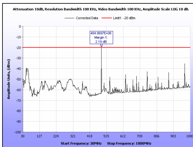
Plot 88. Radiated Spurious Emissions, Channel 2, HDQPSK, 30 MHz – 1 GHz, 10 W
