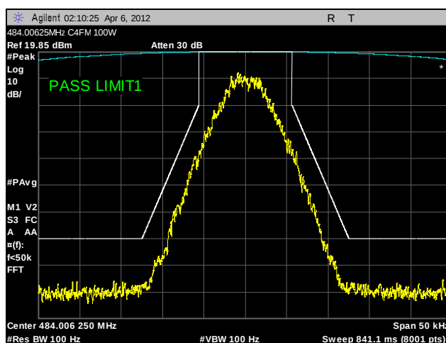
Plot 32. Emission Mask, 484.00625 MHz, C4FM, 100 W
