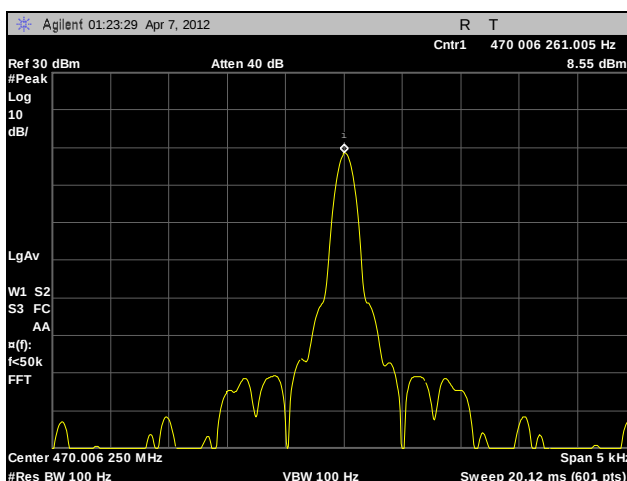
Plot 111. Frequency Stability, Channel 1, 20°C, 132 V
