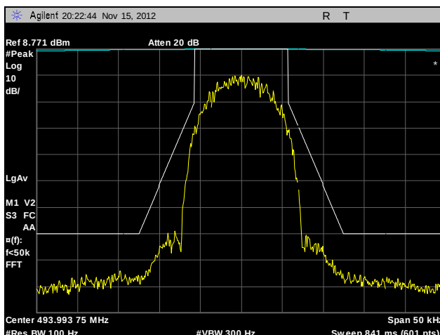
Plot 37. Emission Mask, 493.99375 MHz, HDQPSK, 10 W
