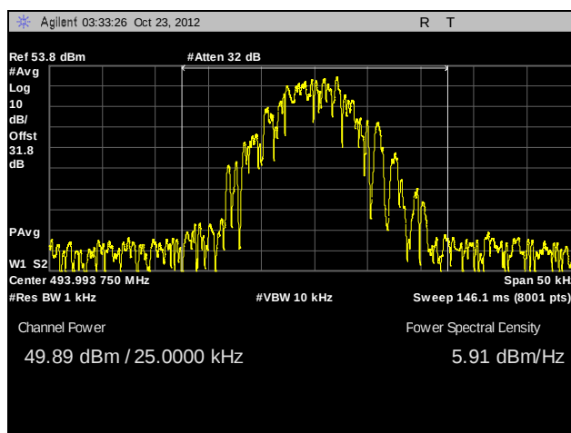
Plot 20. RF Power Output, 493.99375 MHz, 100W, C4FM
