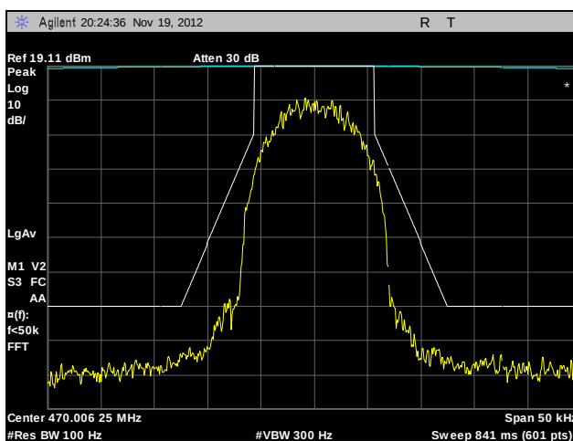
Plot 27. Emission Mask, 470.00625 MHz, CQPSK, 100 W
