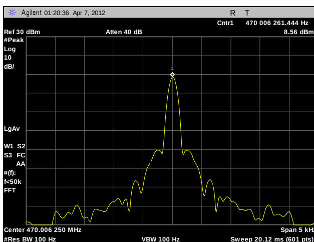
Plot 110. Frequency Stability, Channel 1, 20°C, 120 V
