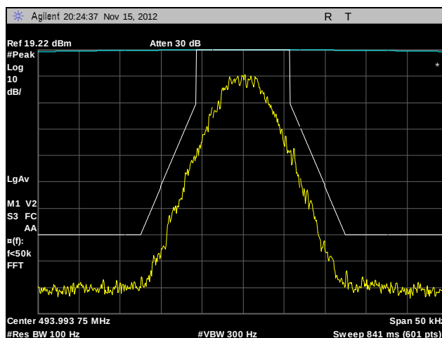
Plot 38. Emission Mask, 493.99375 MHz, C4FM, 100 W
