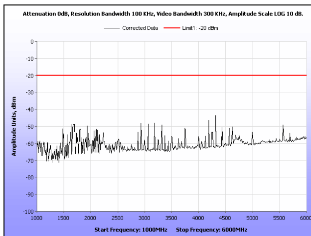
Plot 97. Radiated Spurious Emissions, 493.99375 MHz, CQPSK, 1 GHz – 6 GHz, 10 W
