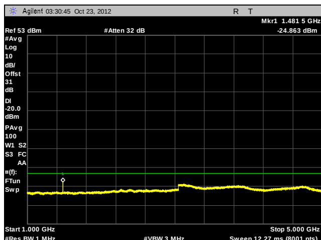
Plot 64. Conducted Spurious Emissions, 493.99375 MHz, CQPSK, 1 GHz – 5 GHz
