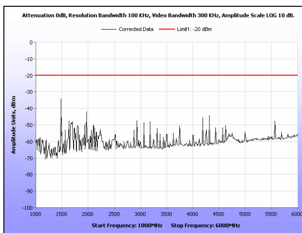
Plot 95. Radiated Spurious Emissions, 493.99375 MHz, C4FM, 1 GHz – 6 GHz, 100 W
