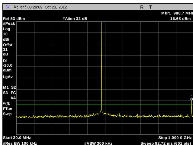
Plot 65. Conducted Spurious Emissions, 493.99375 MHz, HDQPSK, 30 MHz – 1 GHz
