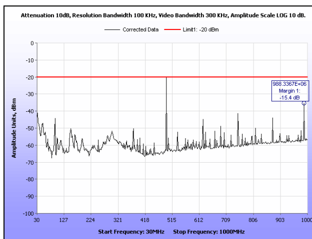
Plot 96. Radiated Spurious Emissions, 493.99375 MHz, CQPSK, 30 MHz – 1 GHz, 10 W
