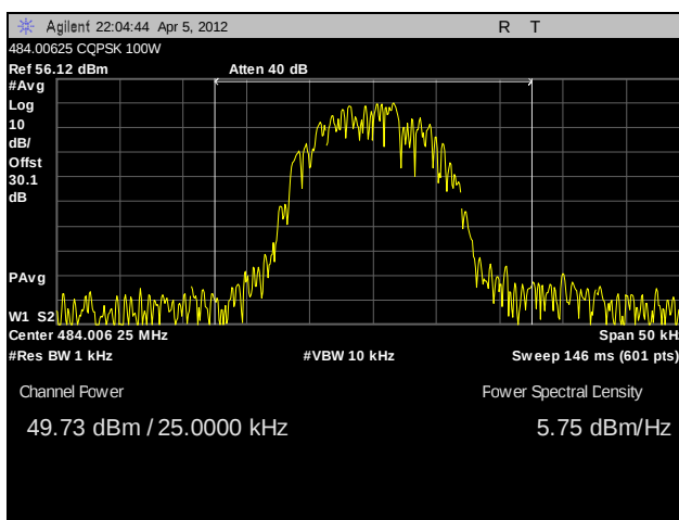
Plot 15. RF Power Output, 484.00625 MHz, 100W, CQPSK
