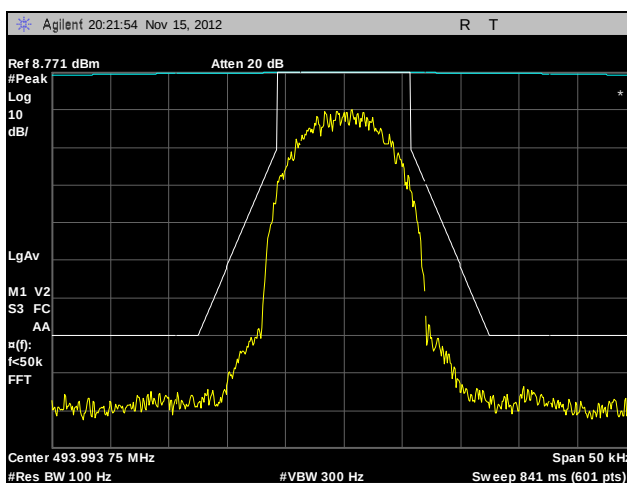
Plot 36. Emission Mask, 493.99375 MHz, CQPSK, 10 W
