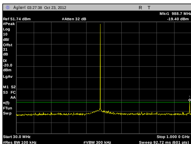
Plot 59. Conducted Spurious Emissions, 493.99375 MHz, C4FM, 30 MHz – 1 GHz
