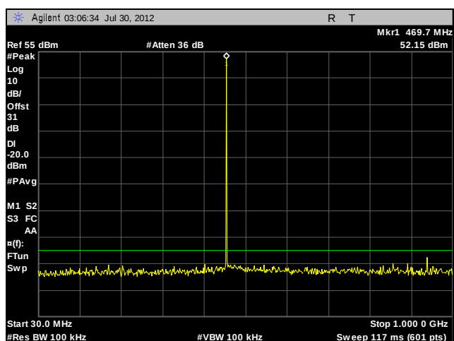
Plot 47. Conducted Spurious Emissions, 470.00625 MHz, HDQPSK, 30 MHz – 1 GHz
