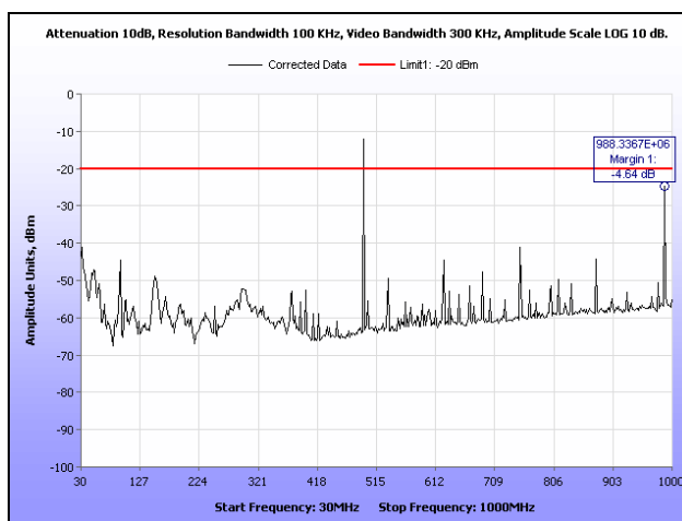
Plot 98. Radiated Spurious Emissions, 493.99375 MHz, CQPSK, 30 MHz – 1 GHz, 100 W
