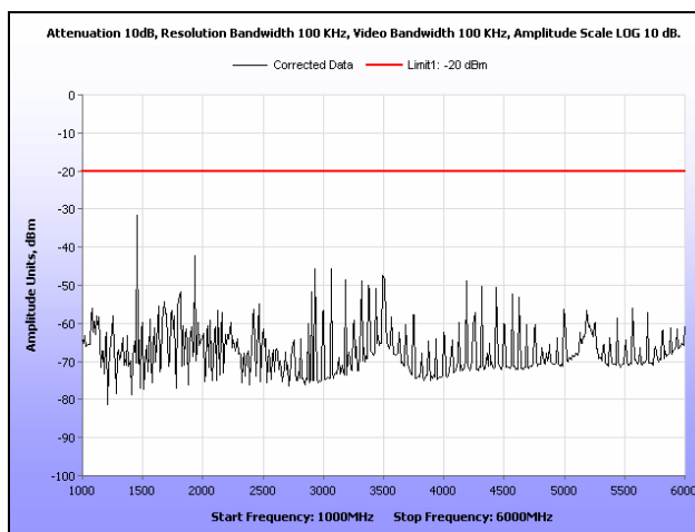
Plot 91. Radiated Spurious Emissions, Channel 2, HDQPSK, 1 GHz – 6 GHz, 100 W
