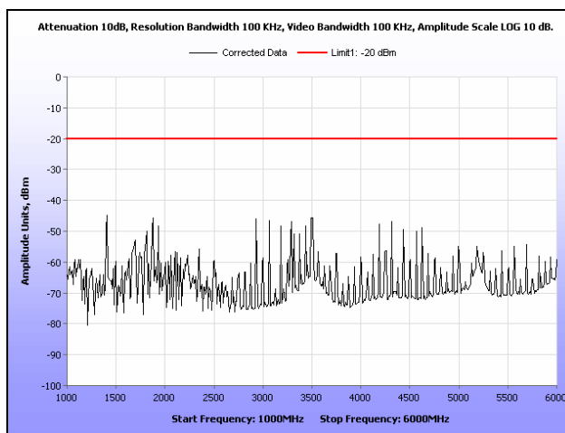
Plot 71. Radiated Spurious Emissions, Channel 1, C4FM, 1 GHz – 6 GHz, 100 W
