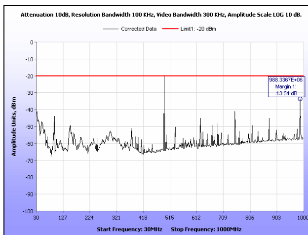
Plot 100. Radiated Spurious Emissions, 493.99375 MHz, HDQPSK, 30 MHz – 1 GHz, 10 W
