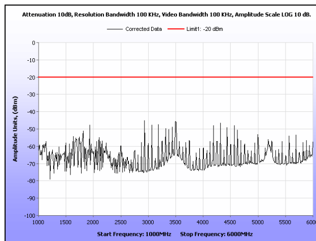
Plot 69. Radiated Spurious Emissions, Channel 1, C4FM, 1 GHz – 6 GHz, 10 W
