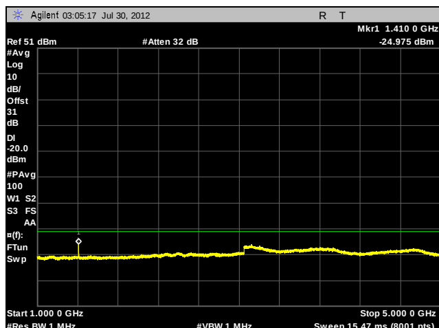
Plot 46. Conducted Spurious Emissions, 470.00625 MHz, CQPSK, 1 GHz – 5 GHz
