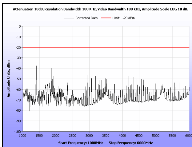
Plot 79. Radiated Spurious Emissions, Channel 1, HDQPSK, 1 GHz – 6 GHz, 100 W
