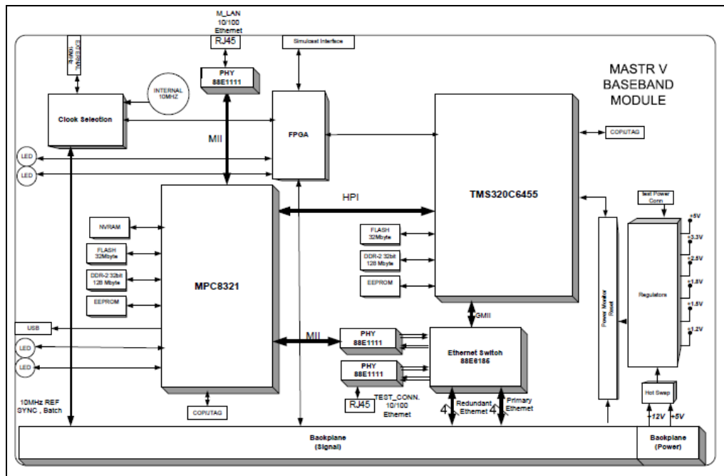
Figure 11. Baseband Module Block Diagram
