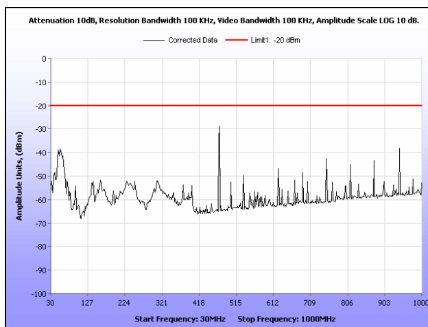
Plot 76. Radiated Spurious Emissions, Channel 1, HKQPSK, 30 MHz – 1 GHz, 10 W
