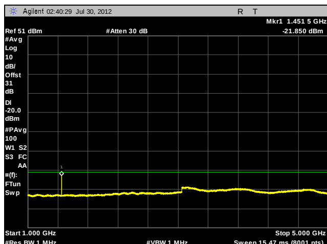
Plot 55. Conducted Spurious Emissions, 484.00625 MHz, CQPSK, 1 GHz – 5 GHz
