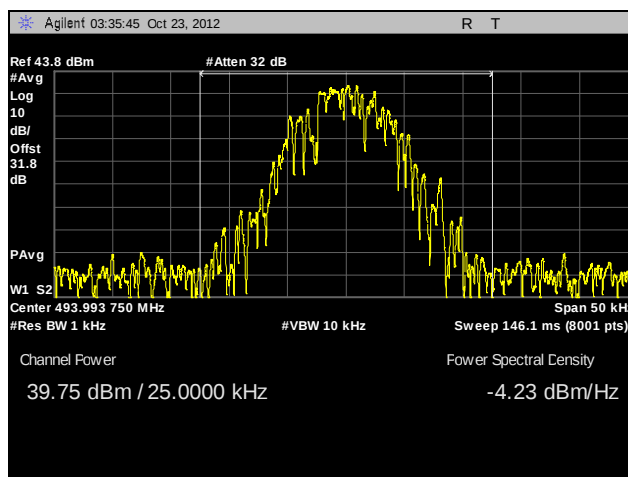
Plot 17. RF Power Output, 493.99375 MHz, 10W, C4FM
