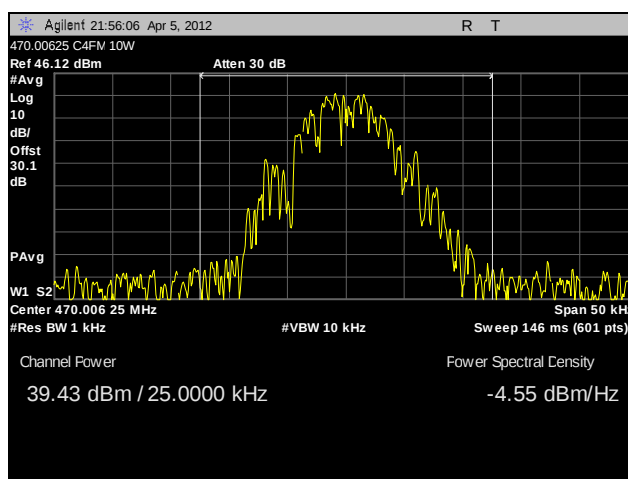
Plot 5. RF Power Output, 470.00625 MHz, 10W, C4FM
