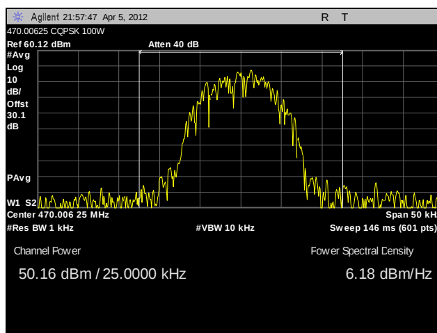
Plot 9. RF Power Output, 470.00625 MHz, 100W, CQPSK
