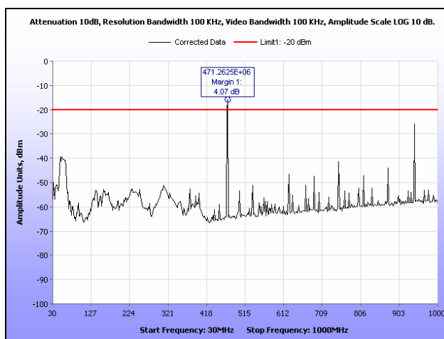
Plot 74. Radiated Spurious Emissions, Channel 1, CQPSK, 30 MHz – 1 GHz, 100 W
