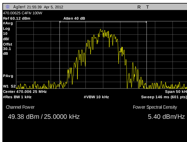
Plot 8. RF Power Output, 470.00625 MHz, 100W, C4FM
