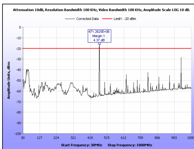
Plot 78. Radiated Spurious Emissions, Channel 1, HKQPSK, 30 MHz – 1 GHz, 100 W
