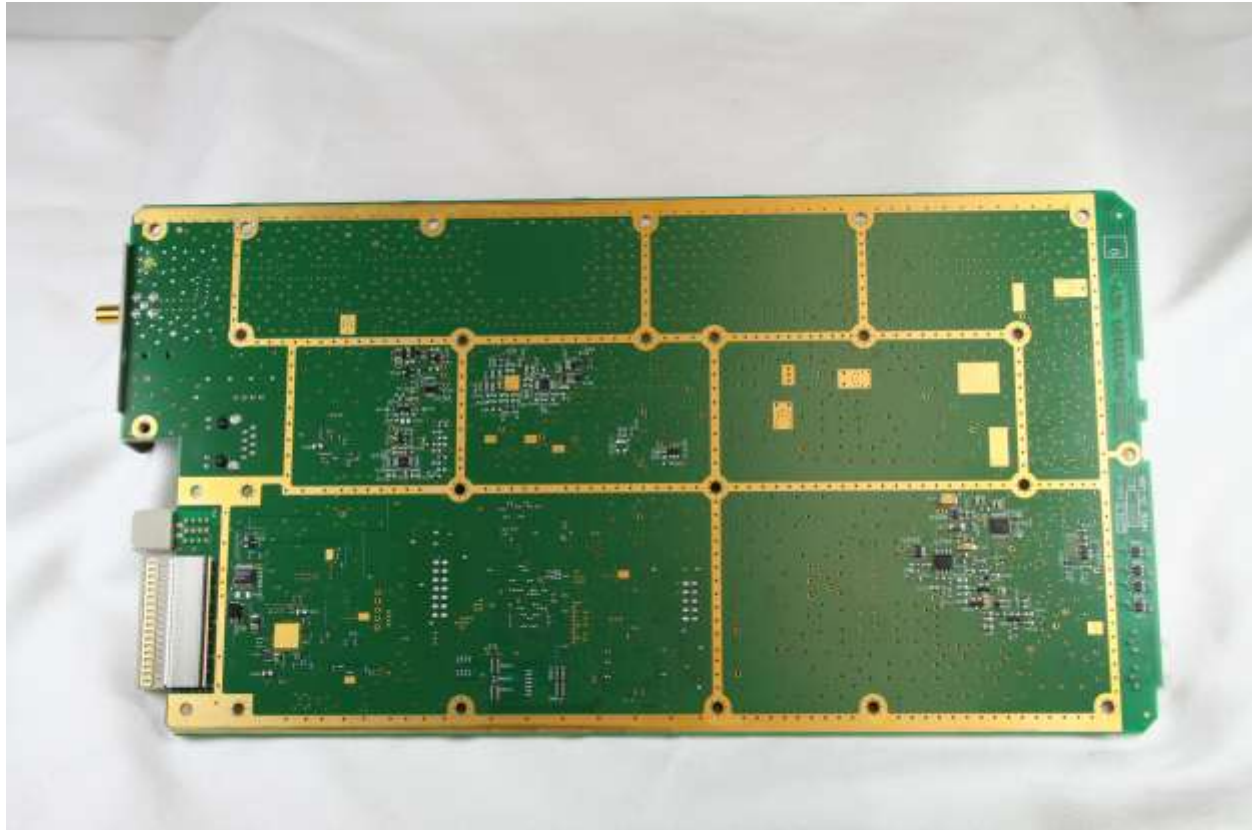
Photograph 5. RX Module (470-494MHz) Bottom
