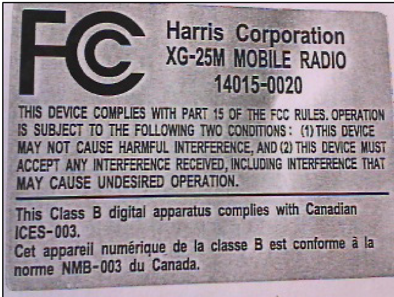
Photograph 2: Part 15 Label Sample
