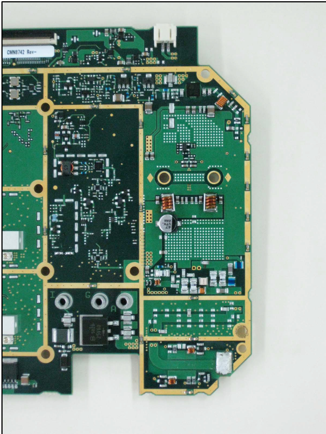
Photograph 18: Parts Side – Right Side
