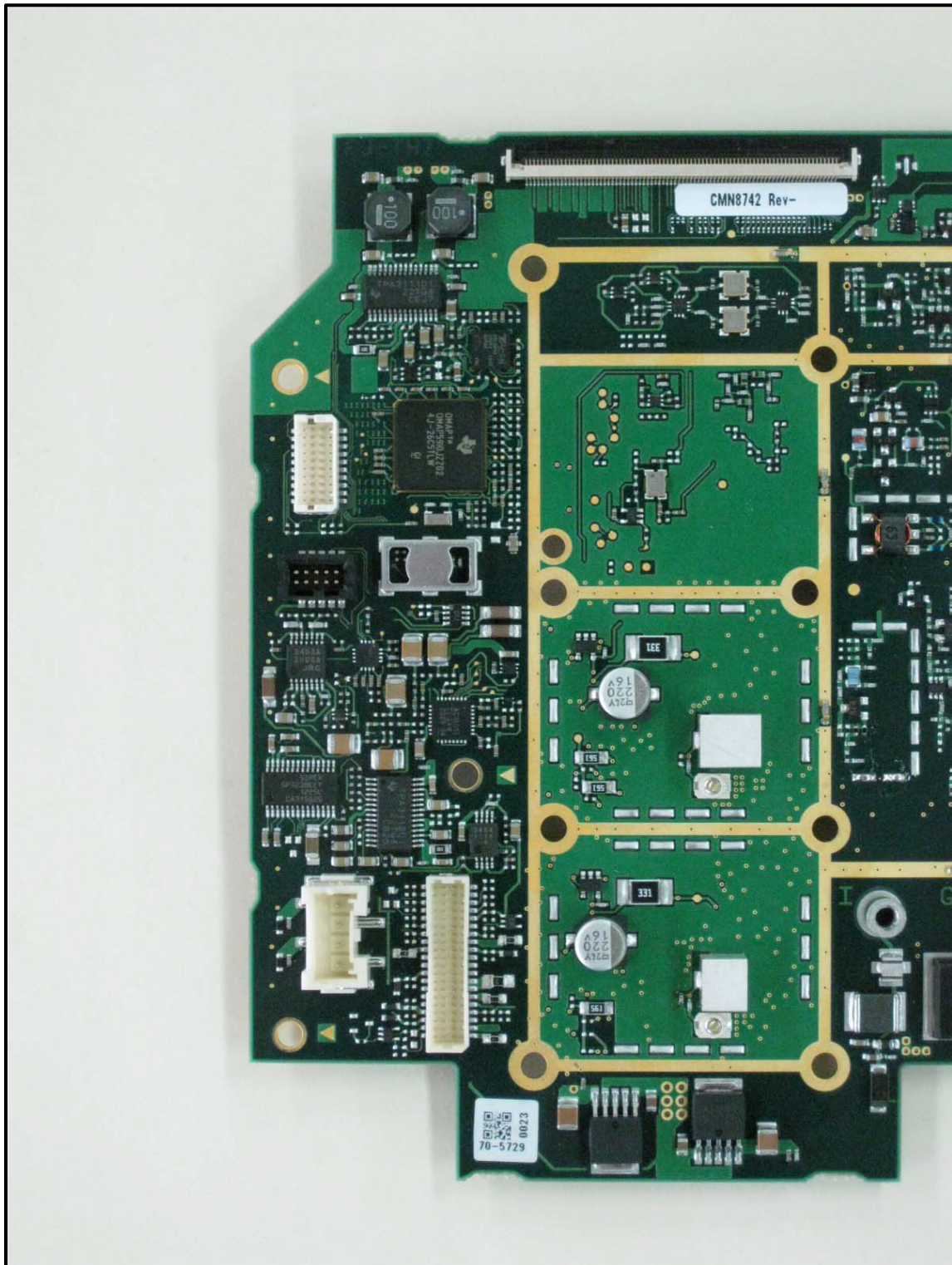
Photograph 17: Parts Side – Left Side
