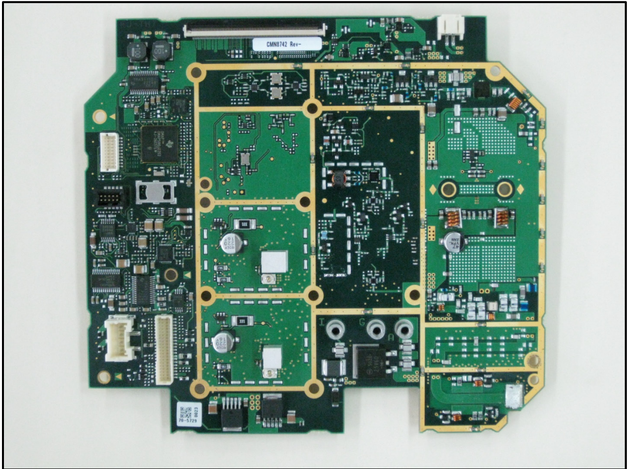
Photograph 15: PCB - Parts Side
