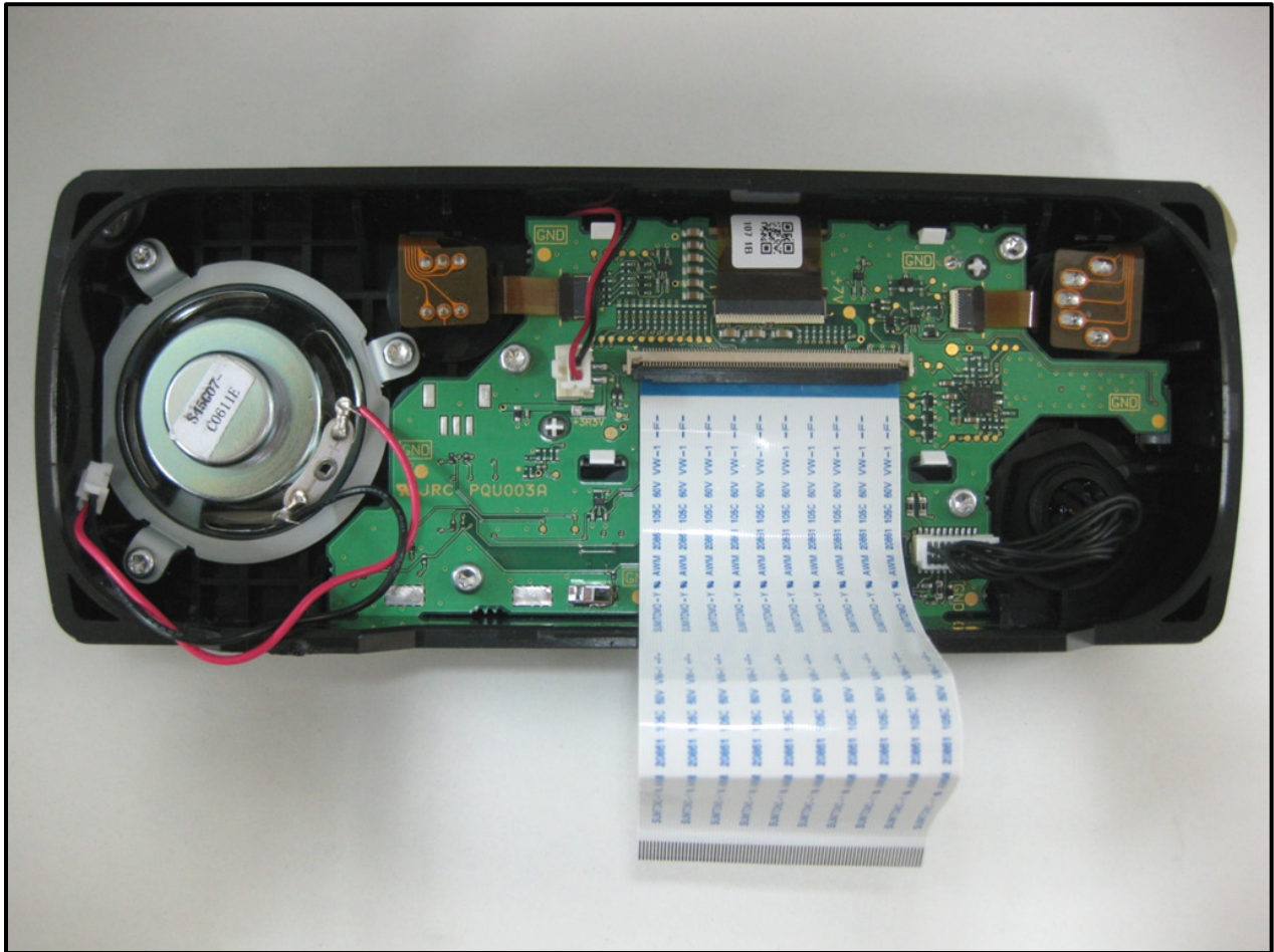
Photograph 21: Separated from Main Unit
