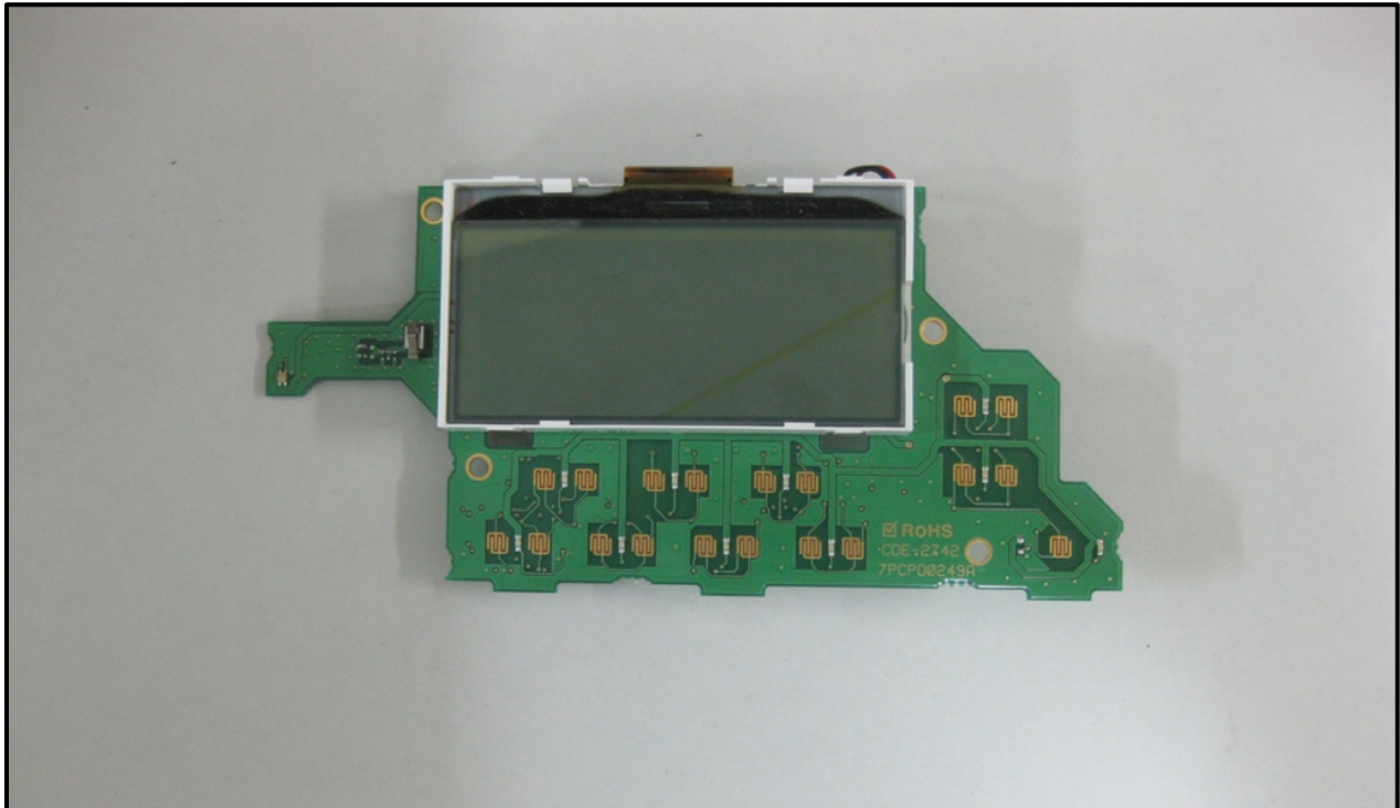
Photograph 22: Parts Side
