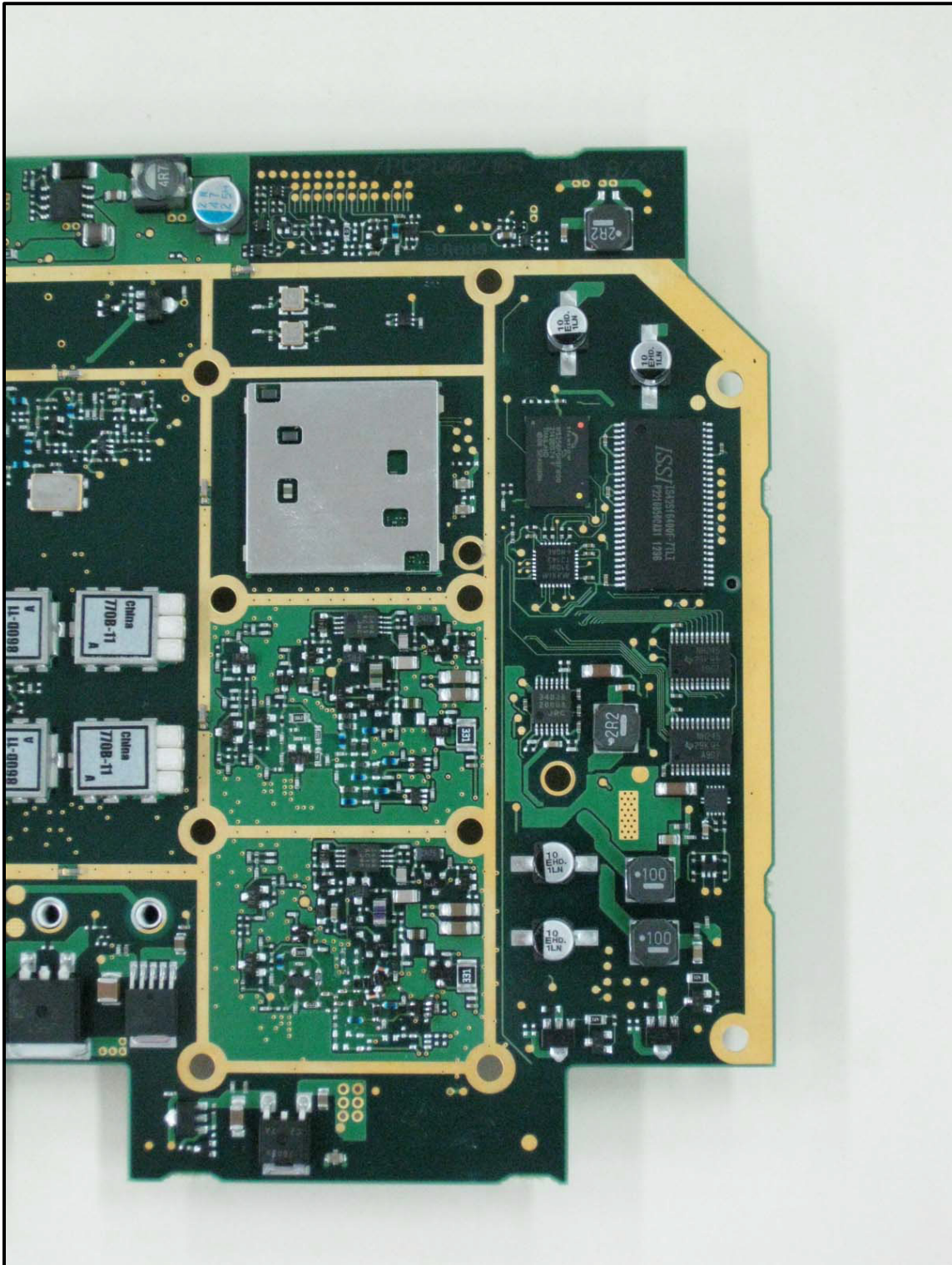
Photograph 20: Solder Side – Right Side
