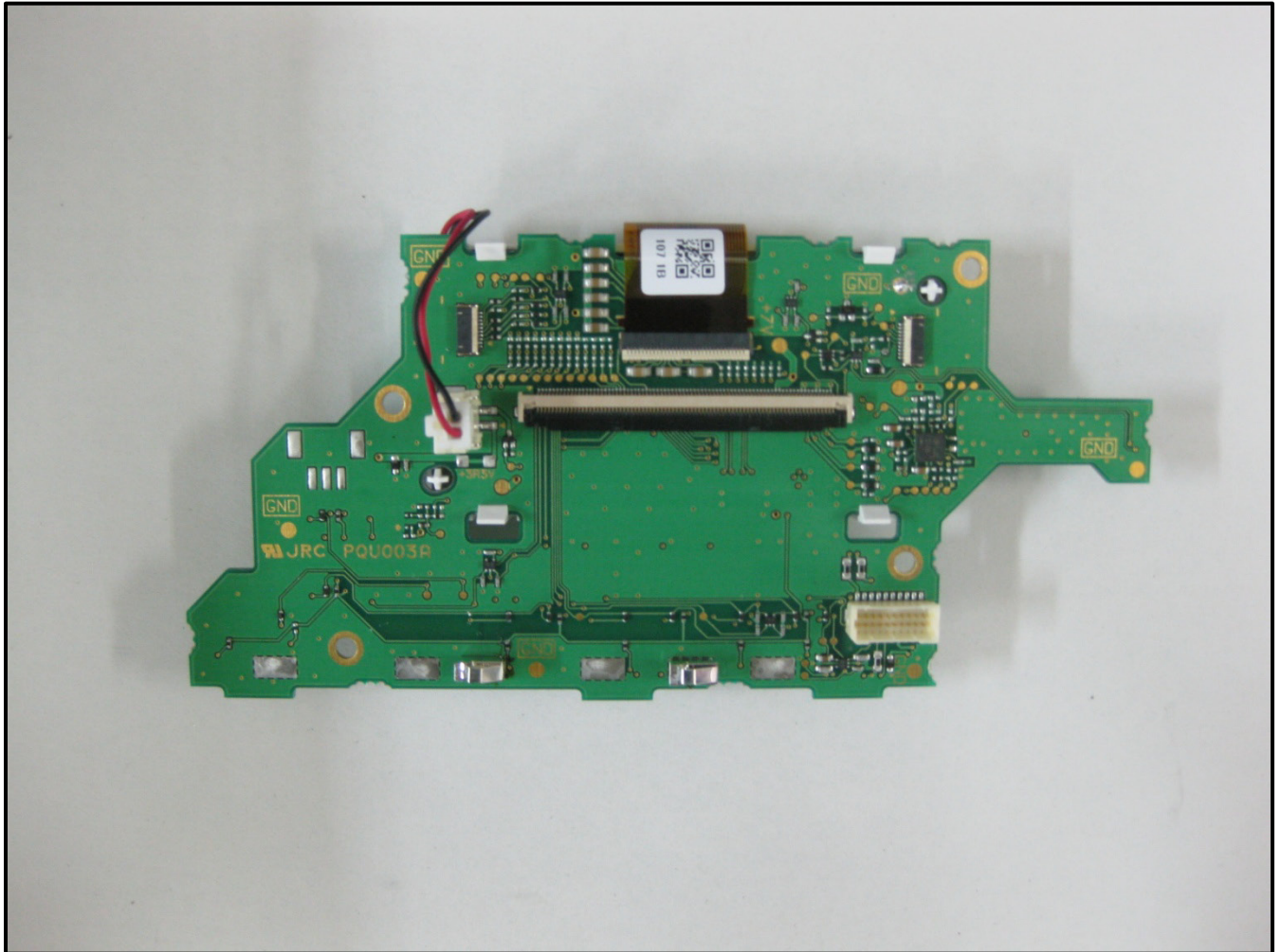
Photograph 19: Solder Side
