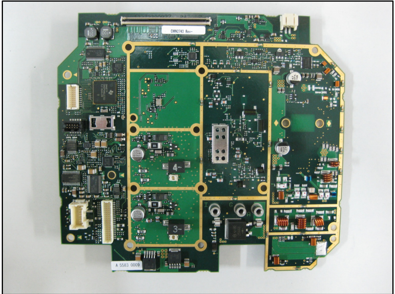
Photograph 16: Part Side
