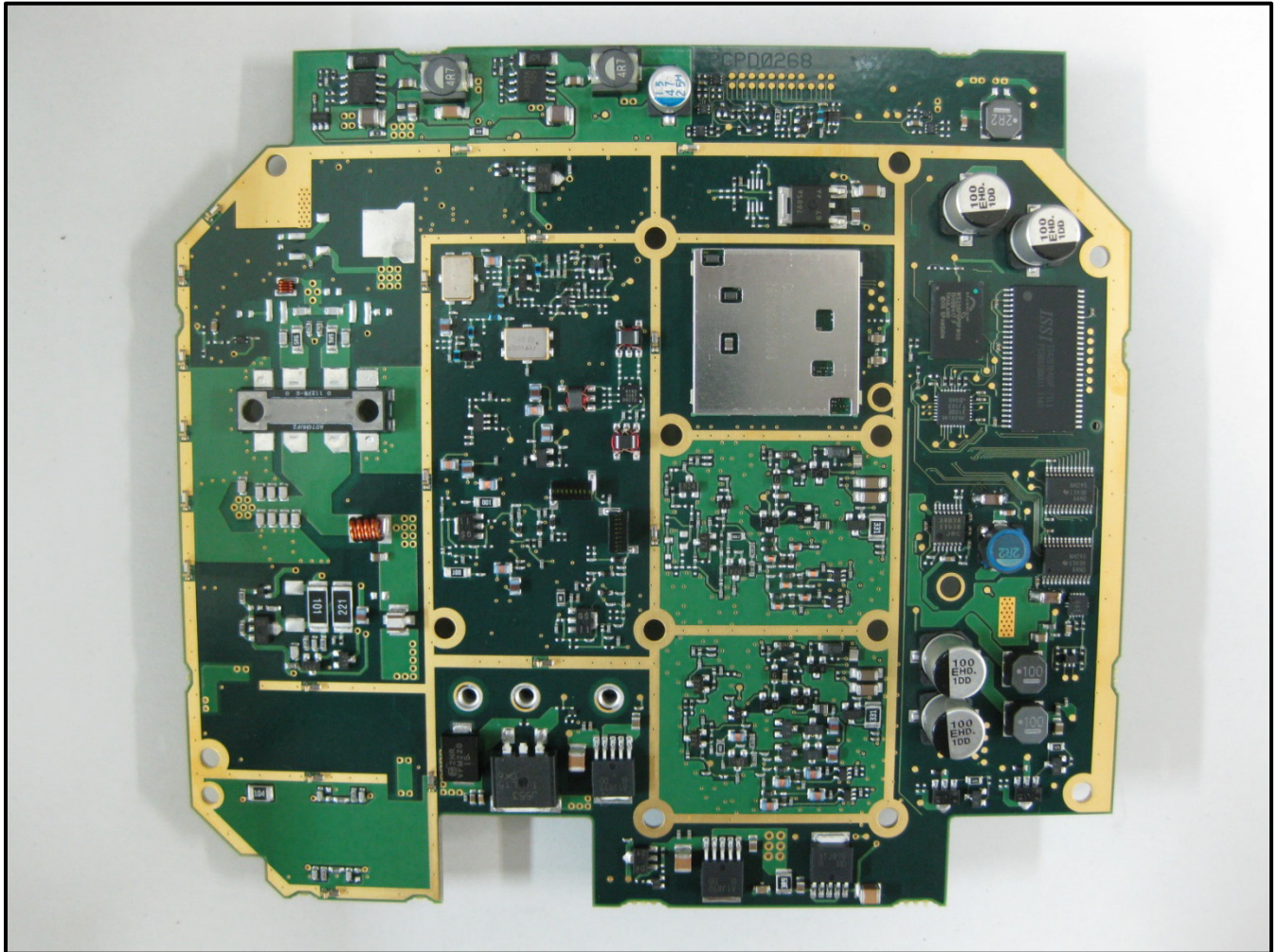
Photograph 17: Solder Side
