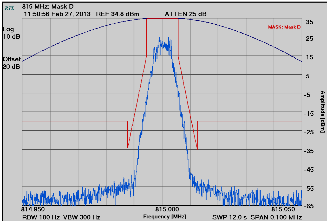
Plot 6-2: Occupied Bandwidth – H-CPM TDMA; 815.0000 MHz; Mask D
