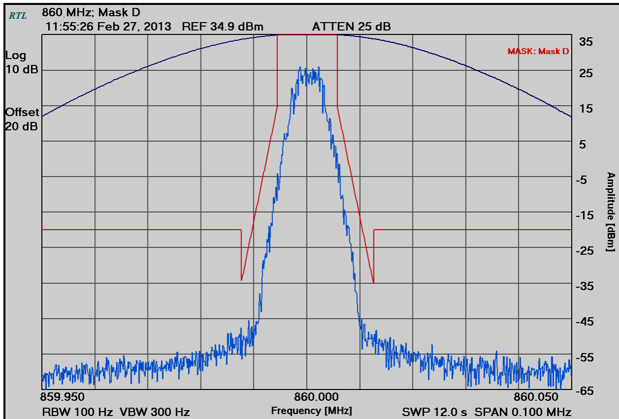
Plot 6-5: Occupied Bandwidth – H-CPM TDMA; 860.0000 MHz; Mask D
