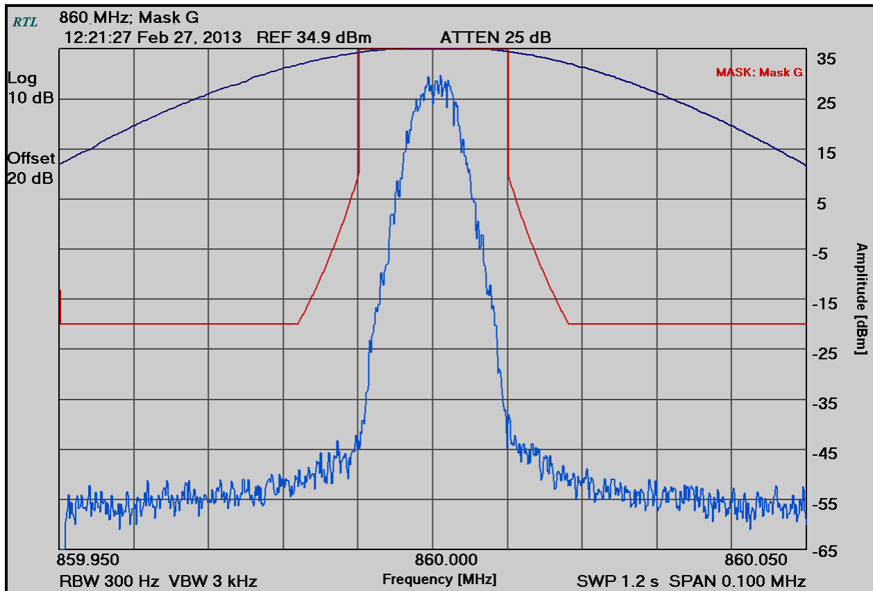
Plot 6-11: Occupied Bandwidth – H-CPM TDMA; 860.0000 MHz; Mask G
