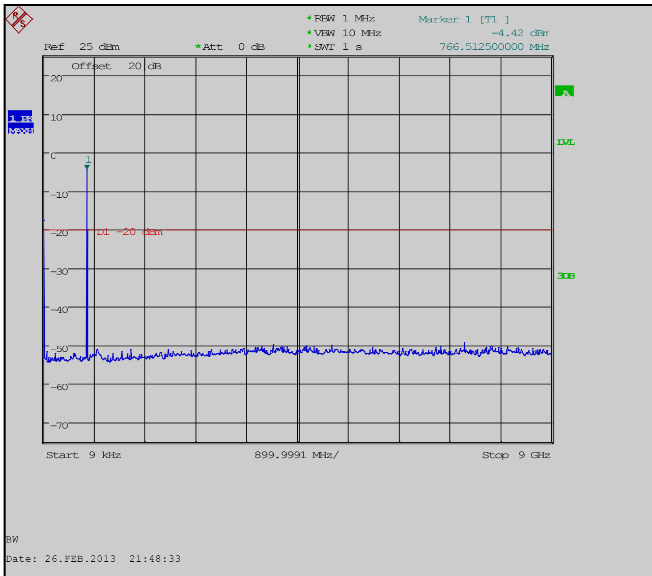
Plot 5-4: Conducted Spurious Emissions – H-CPM TDMA; 775.9875 MHz
