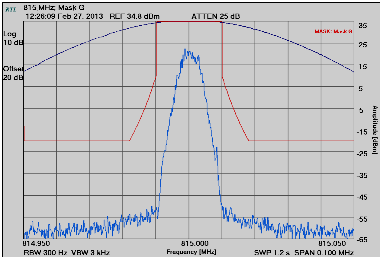
Plot 6-8: Occupied Bandwidth – H-CPM TDMA; 815.0000 MHz; Mask G
