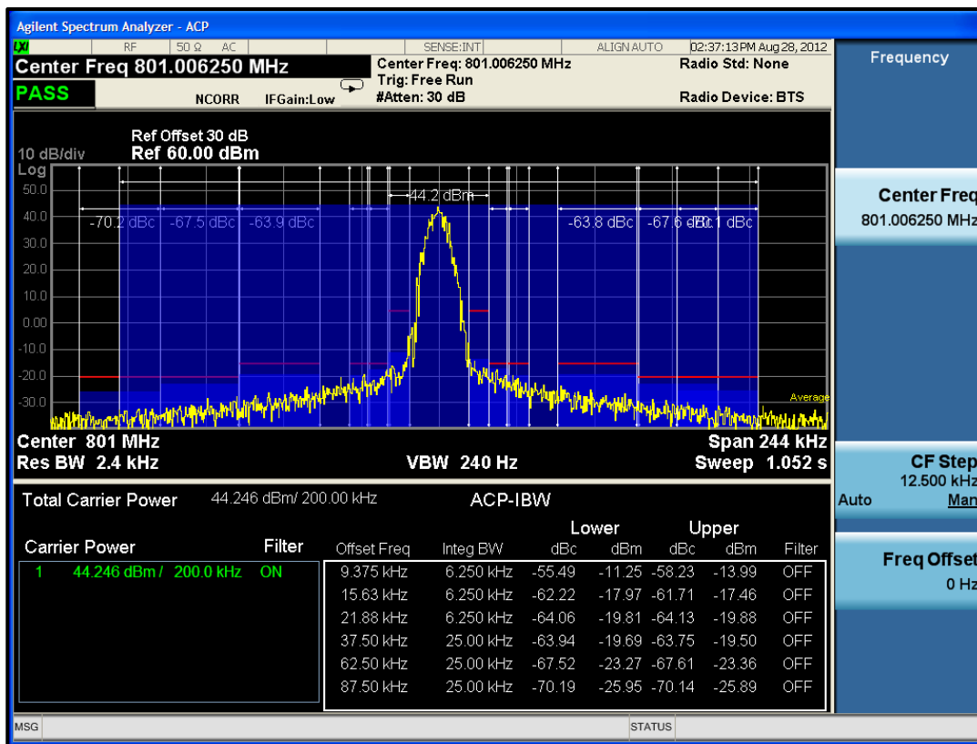
Plot 7-23: Adjacent Channel Power – 801.00625 MHz; P25 (9.375 kHz - 87.5 kHz)
