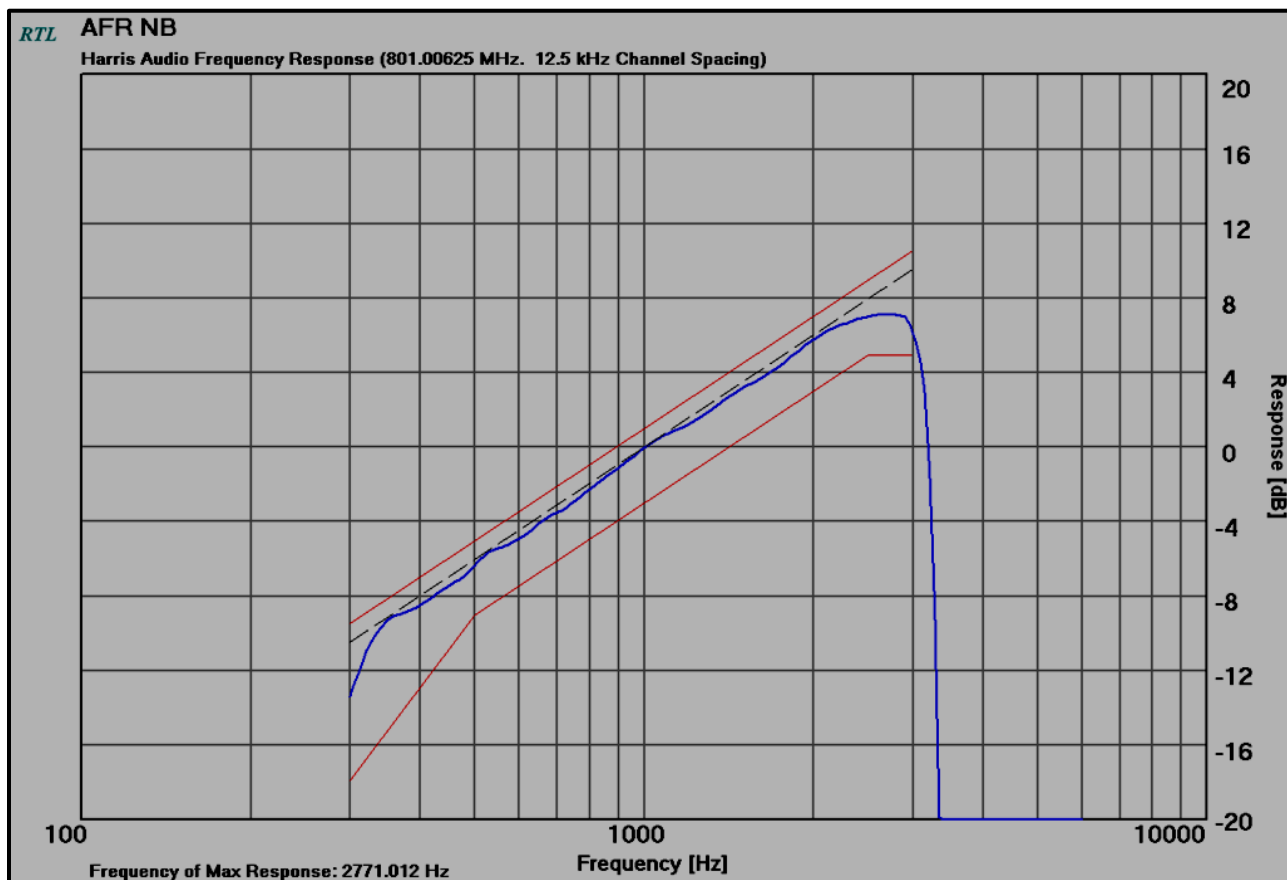
Plot 11-1: Modulation Characteristics - Audio Frequency Response – 801.00625 MHz; NB
