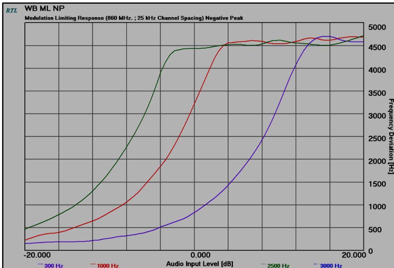
Plot 11-6: Modulation Characteristics – Modulation Limiting – 860.0000 MHz; WB, Negative Peak
