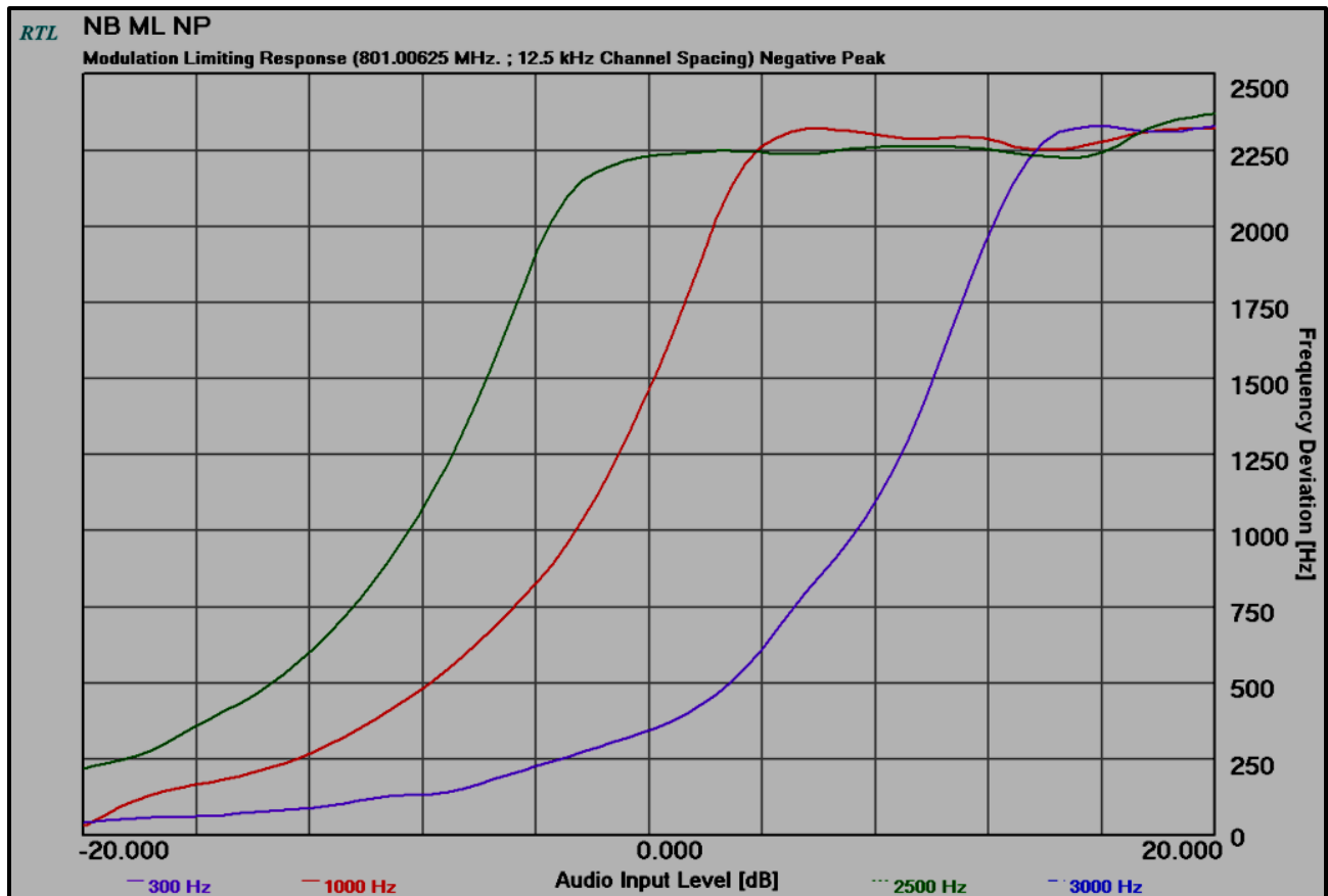
Plot 11-4: Modulation Characteristics – Modulation Limiting - 801.00625 MHz; NB, Negative Peak
