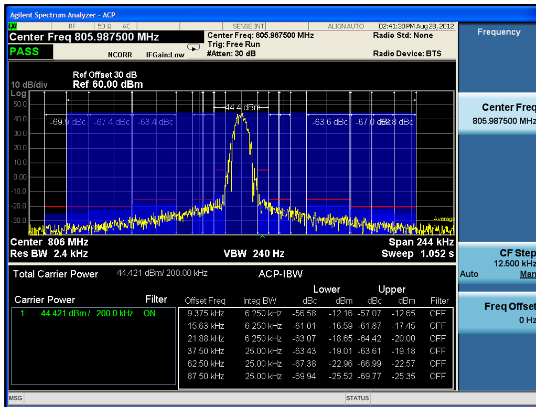
Plot 7-35: Adjacent Channel Power - 805.9875 MHz; OTP NB Mode (9.375 kHz - 87.5 kHz)
