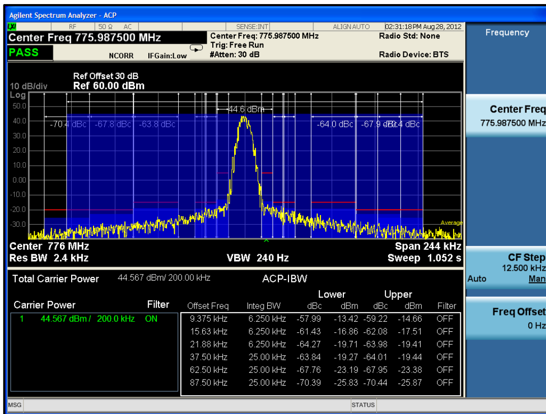
Plot 7-11: Adjacent Channel Power - 775.9875 MHz; P25 Mode (9.375 kHz - 87.5 kHz)
