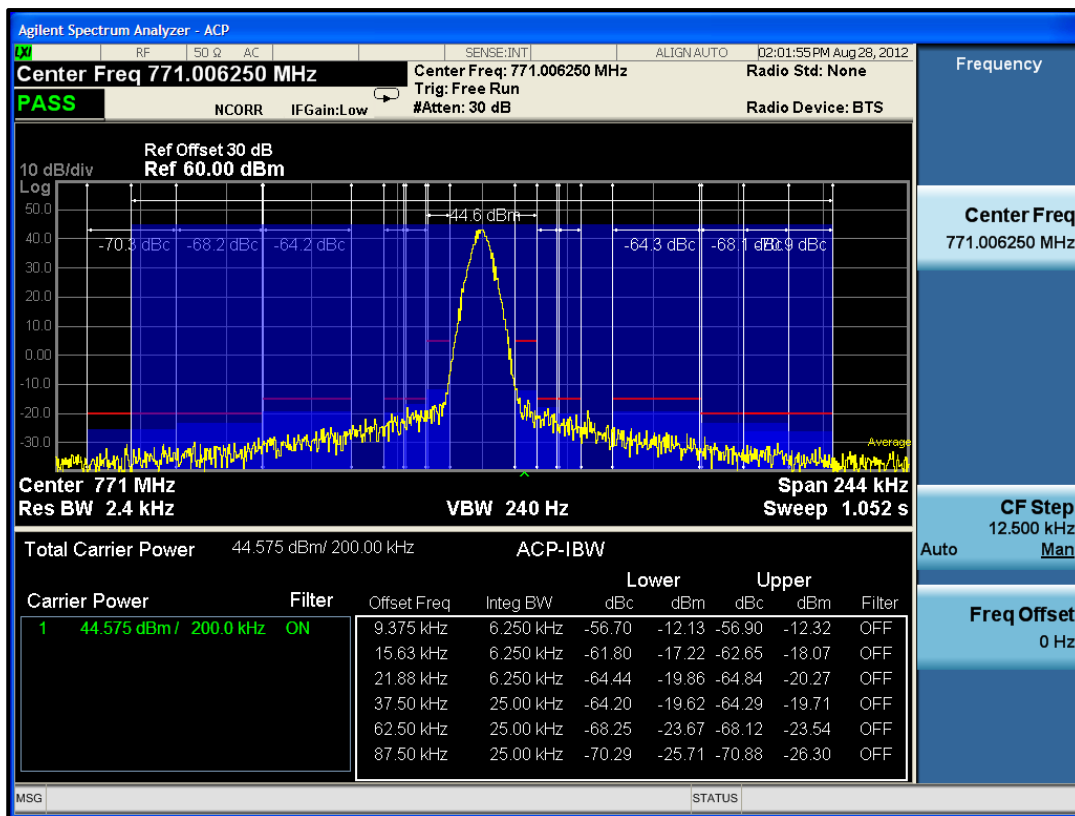
Plot 7-5: Adjacent Channel Power - 771.00625 MHz; Analog Mode (9.375 kHz - 87.5 kHz)
