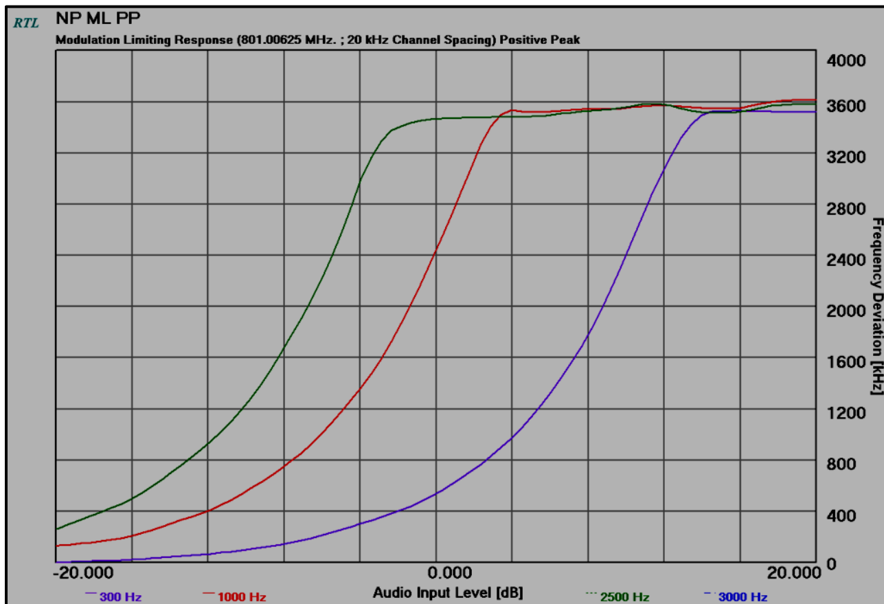
Plot 11-7: Modulation Characteristics – Modulation Limiting – 801.00625 MHz; WB (NPSPAC), Positive Peak
