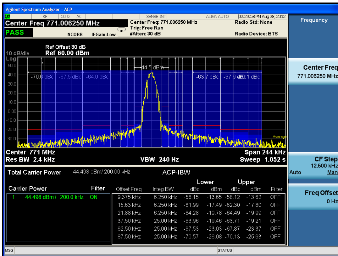
Plot 7-7: Adjacent Channel Power - 771.00625 MHz; P25 Mode (9.375 kHz - 87.5 kHz)
