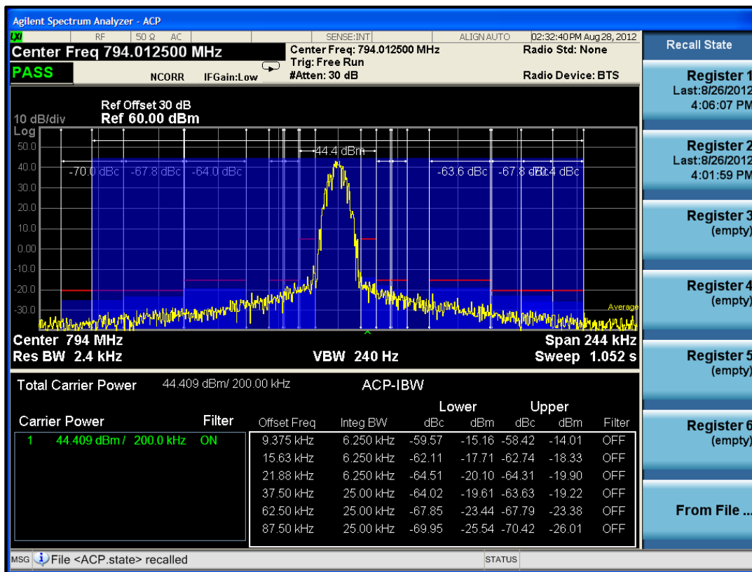
Plot 7-15: Adjacent Channel Power – 794.0125 MHz; P25 (9.375 kHz - 87.5 kHz)
