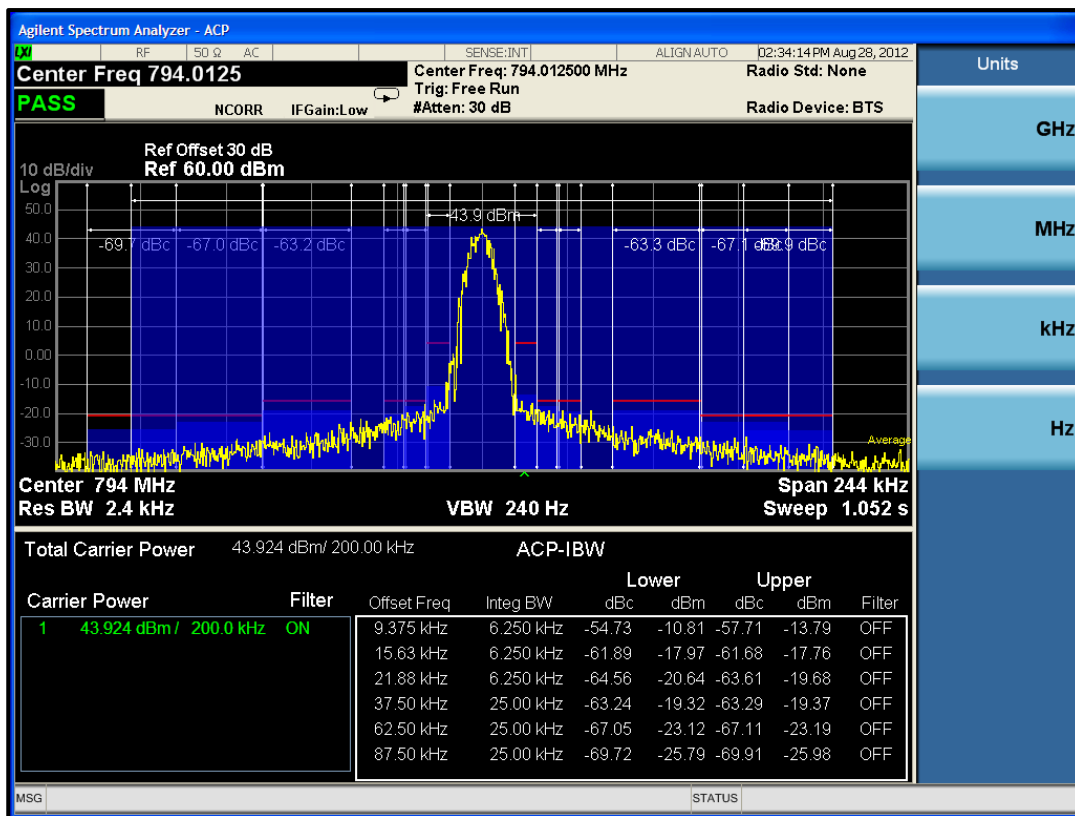
Plot 7-19: Adjacent Channel Power – 794.0125 MHz; OTP NB Mode; (9.375 kHz - 87.5 kHz)
