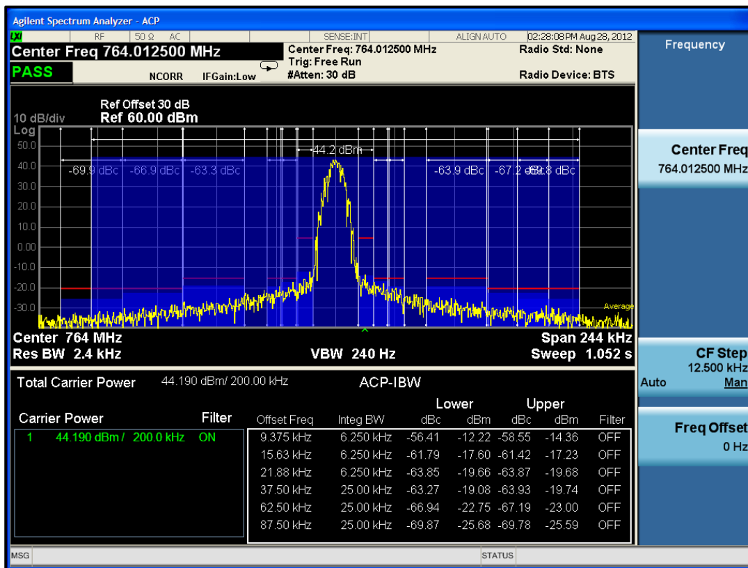
Plot 7-3: Adjacent Channel Power - 764.0125 MHz; P25 Mode (9.375 kHz - 87.5 kHz)
