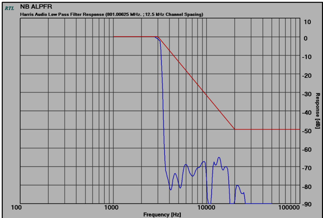
Plot 11-2: Modulation Characteristics – Audio Low Pass Filter – 801.00625 MHz; NB
