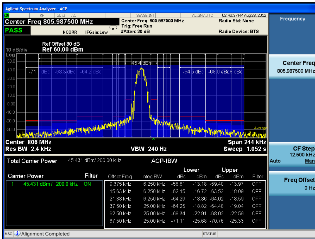
Plot 7-31: Adjacent Channel Power – 805.9875 MHz; P25 (9.375 kHz - 87.5 kHz)
