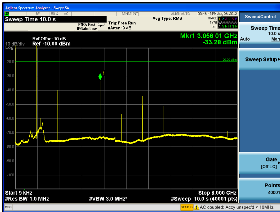
Plot 6-2: Spurious Emissions at Antenna Terminals – 771.00625 MHz
