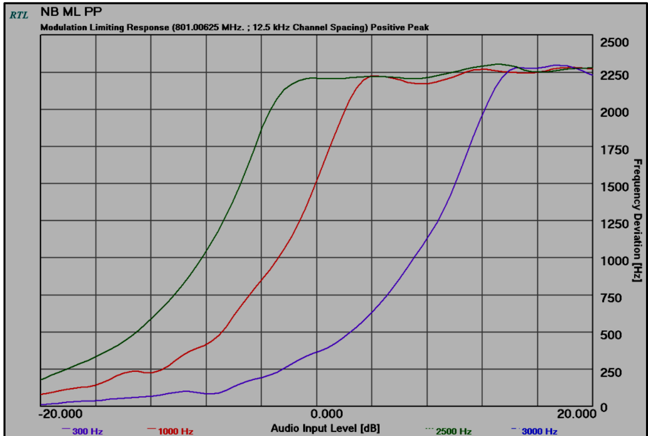
Plot 11-3: Modulation Characteristics – Modulation Limiting – 801.00625 MHz; NB, Positive Peak
