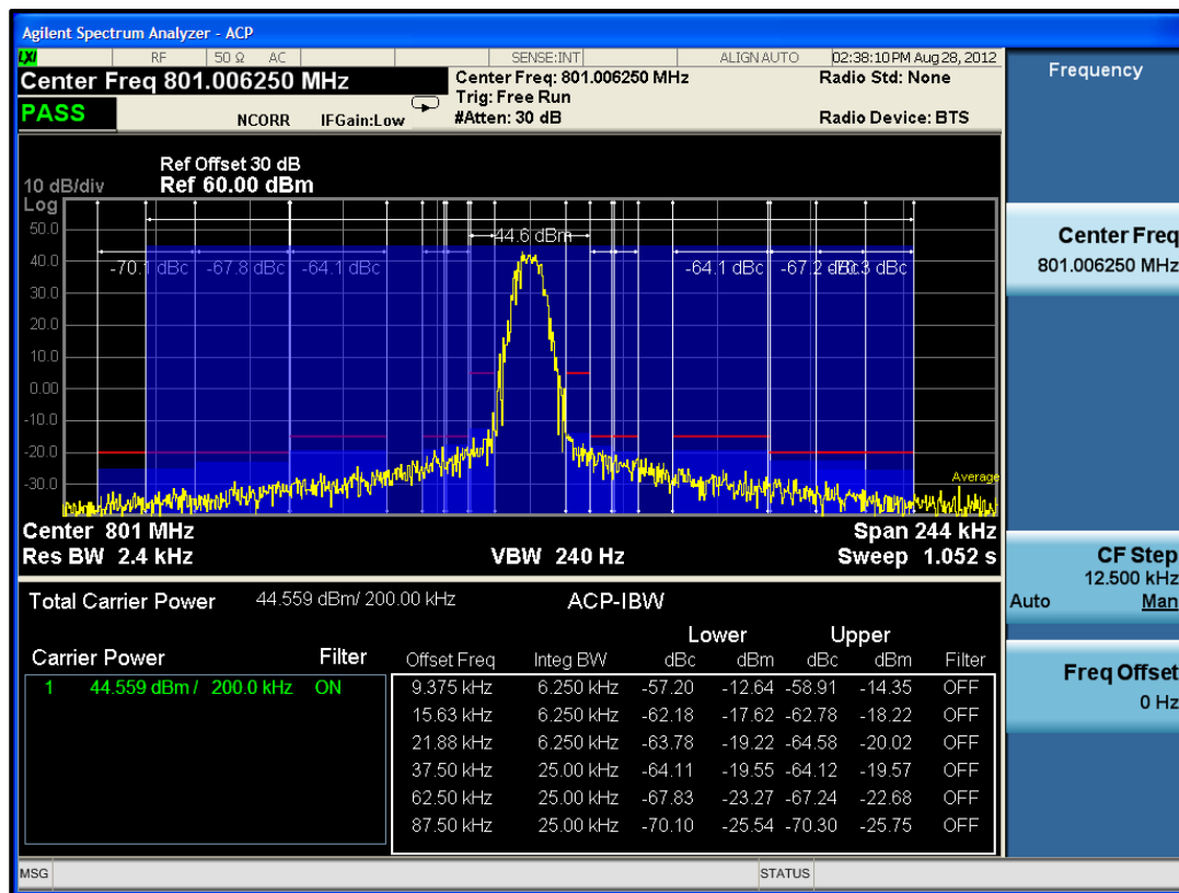
Plot 7-27: Adjacent Channel Power – 801.00625 MHz; OTP NB Mode (9.375 kHz - 87.5 kHz)
