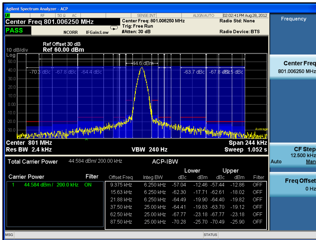
Plot 7-21: Adjacent Channel Power – 801.00625 MHz; Analog Mode; (9.375 kHz - 87.5 kHz)
