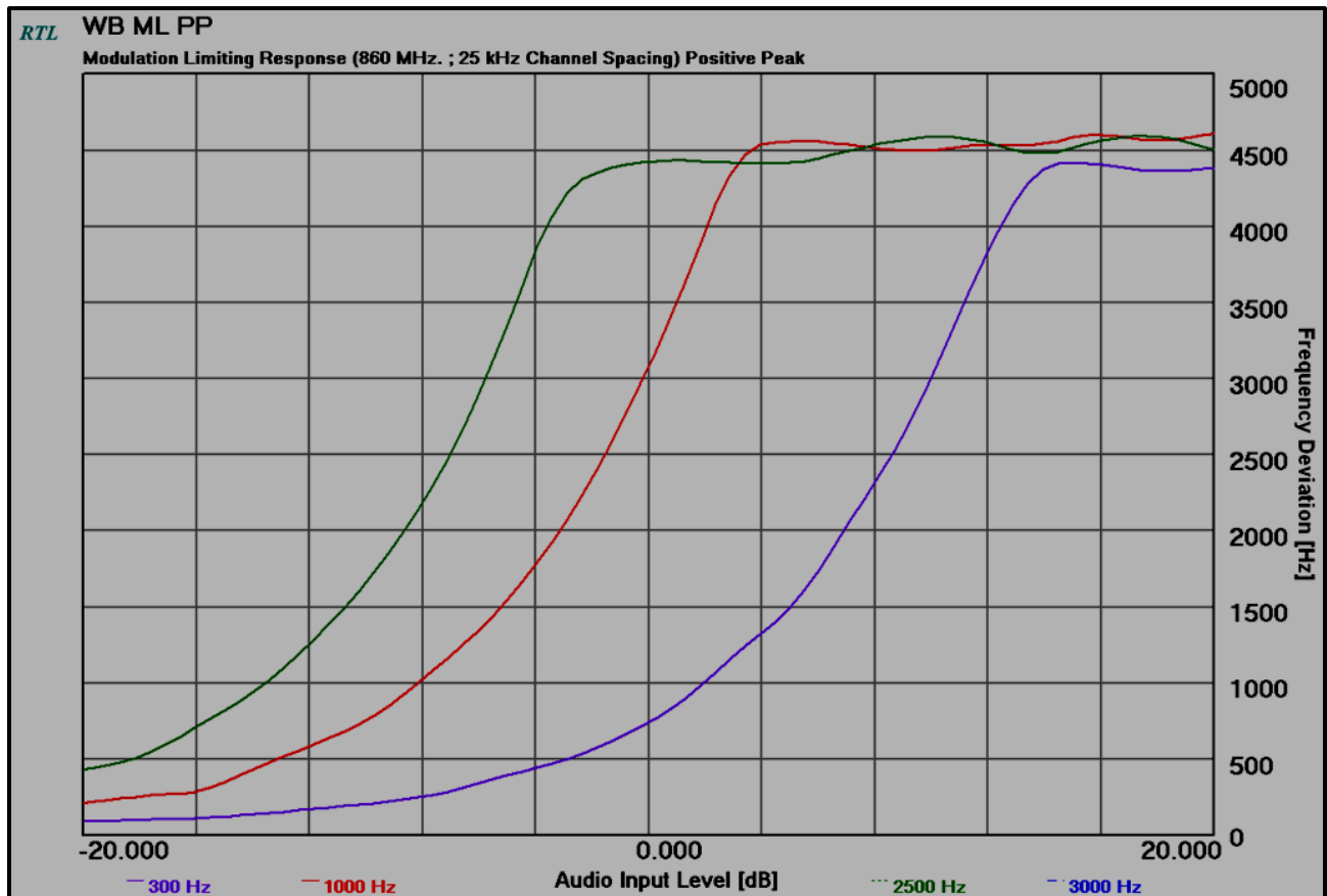
Plot 11-5: Modulation Characteristics – Modulation Limiting – 860.0000 MHz; WB, Positive Peak
