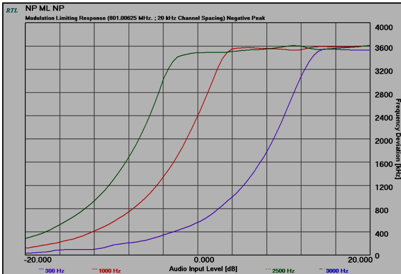
Plot 11-8: Modulation Characteristics – Modulation Limiting – 801.00625 MHz; WB (NPSPAC), Negative Peak
