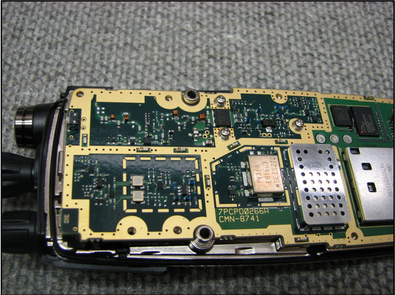
Photograph 20: Main Board View 2
