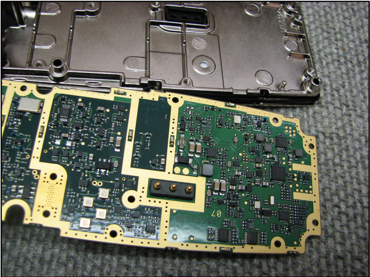
Photograph 23: Main Board Back View 2
