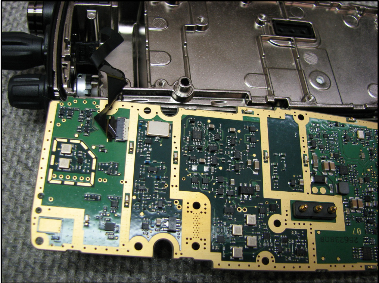
Photograph 24: Main Board Back View 3
