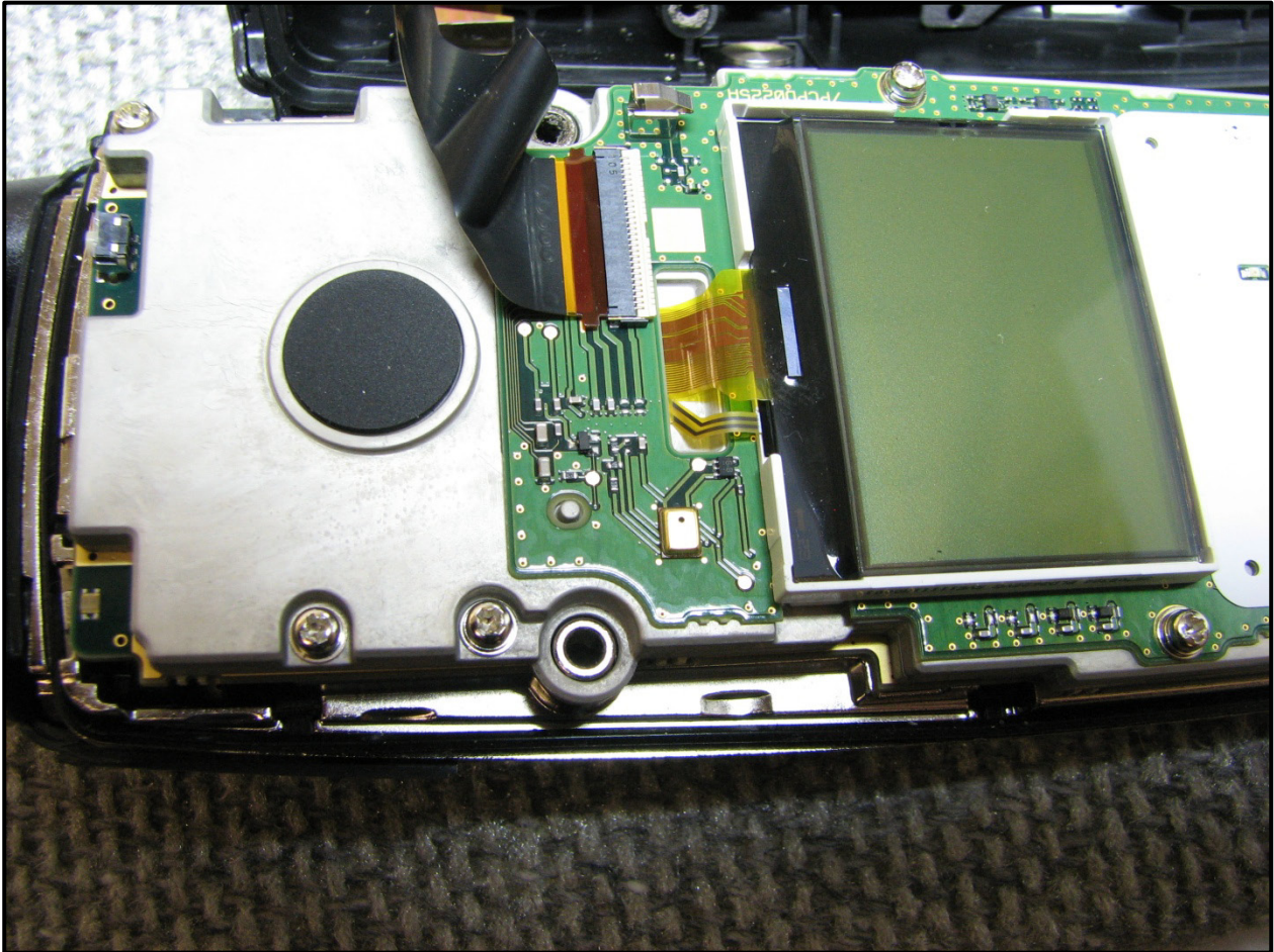
Photograph 13: IF Board View 1
