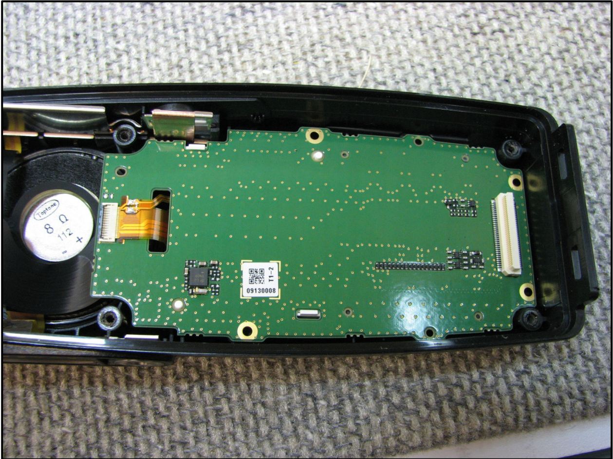
Photograph 18: IF Board View 6
