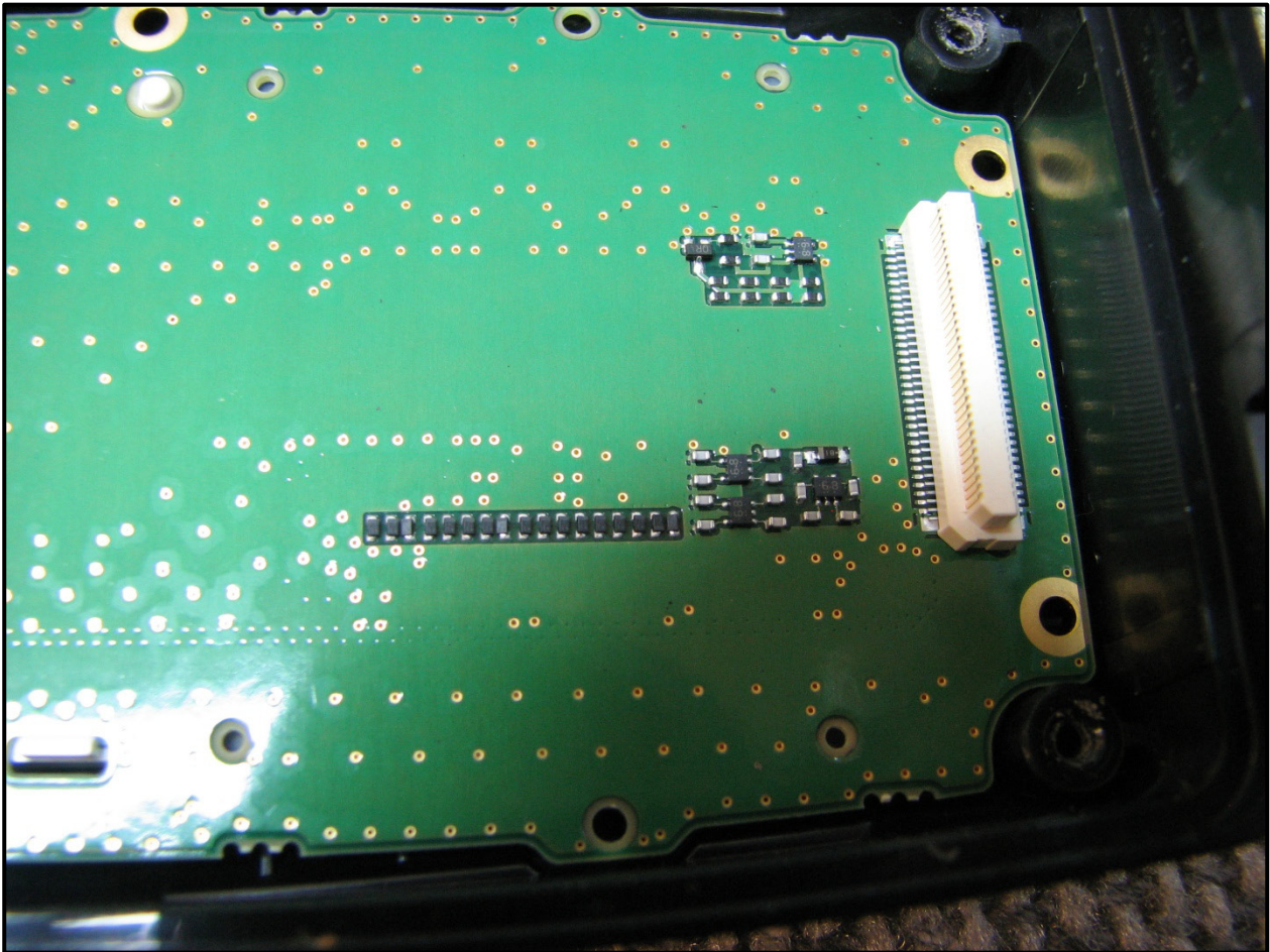
Photograph 17: IF Board View 5
