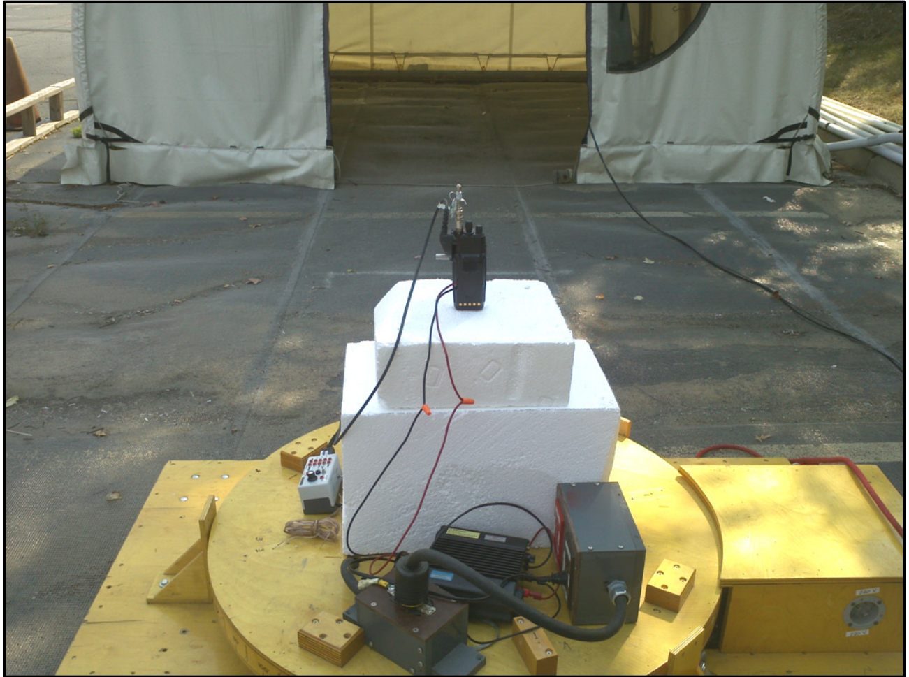
Photograph 6: Radiated Emissions (Spurious/Harmonics) – Back View
