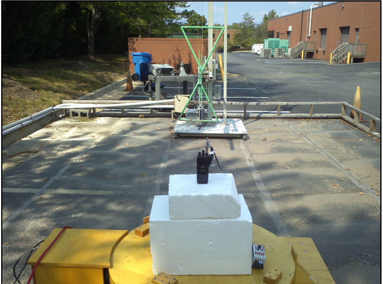
Photograph 5: Radiated Emissions (Spurious/Harmonics) – Front View
