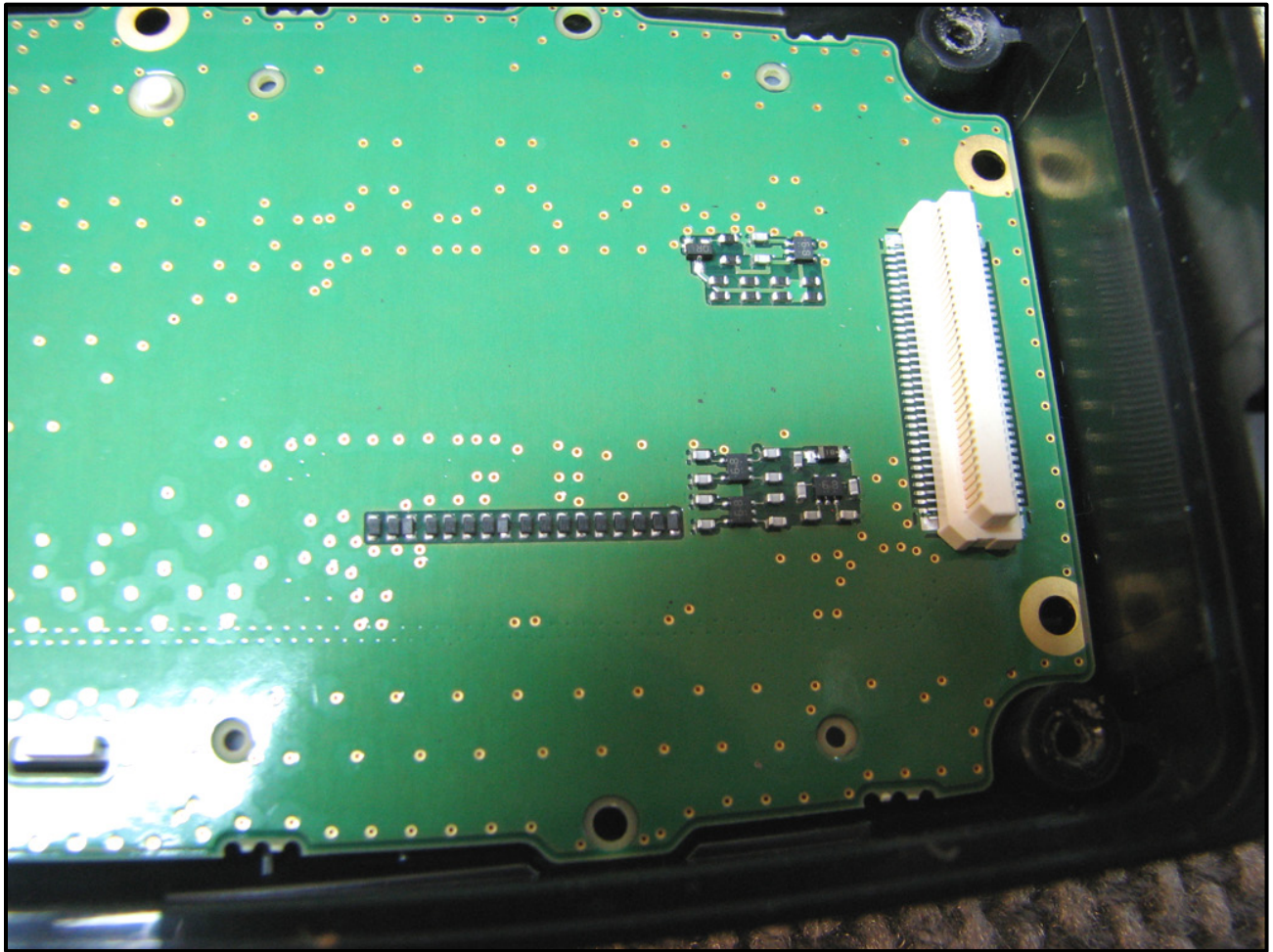
Photograph 27: IF Board 5
