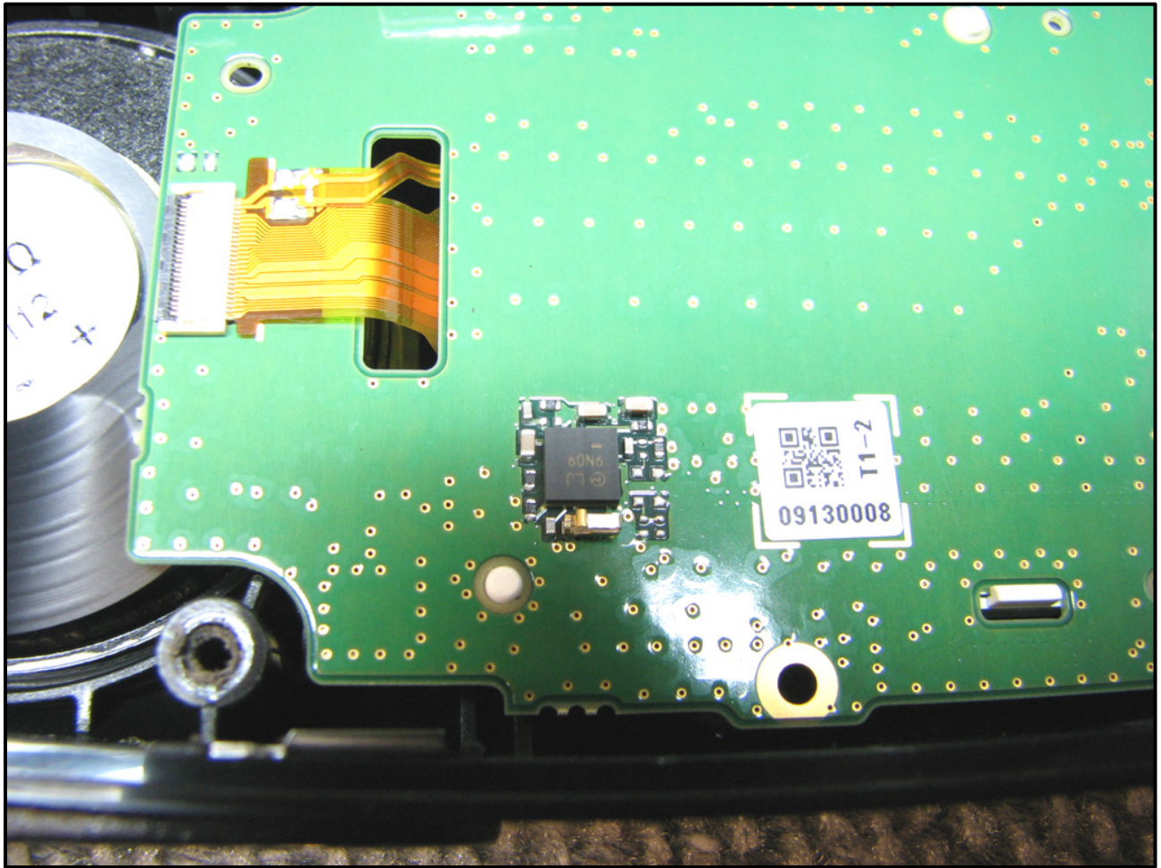
Photograph 26: IF Board 4
