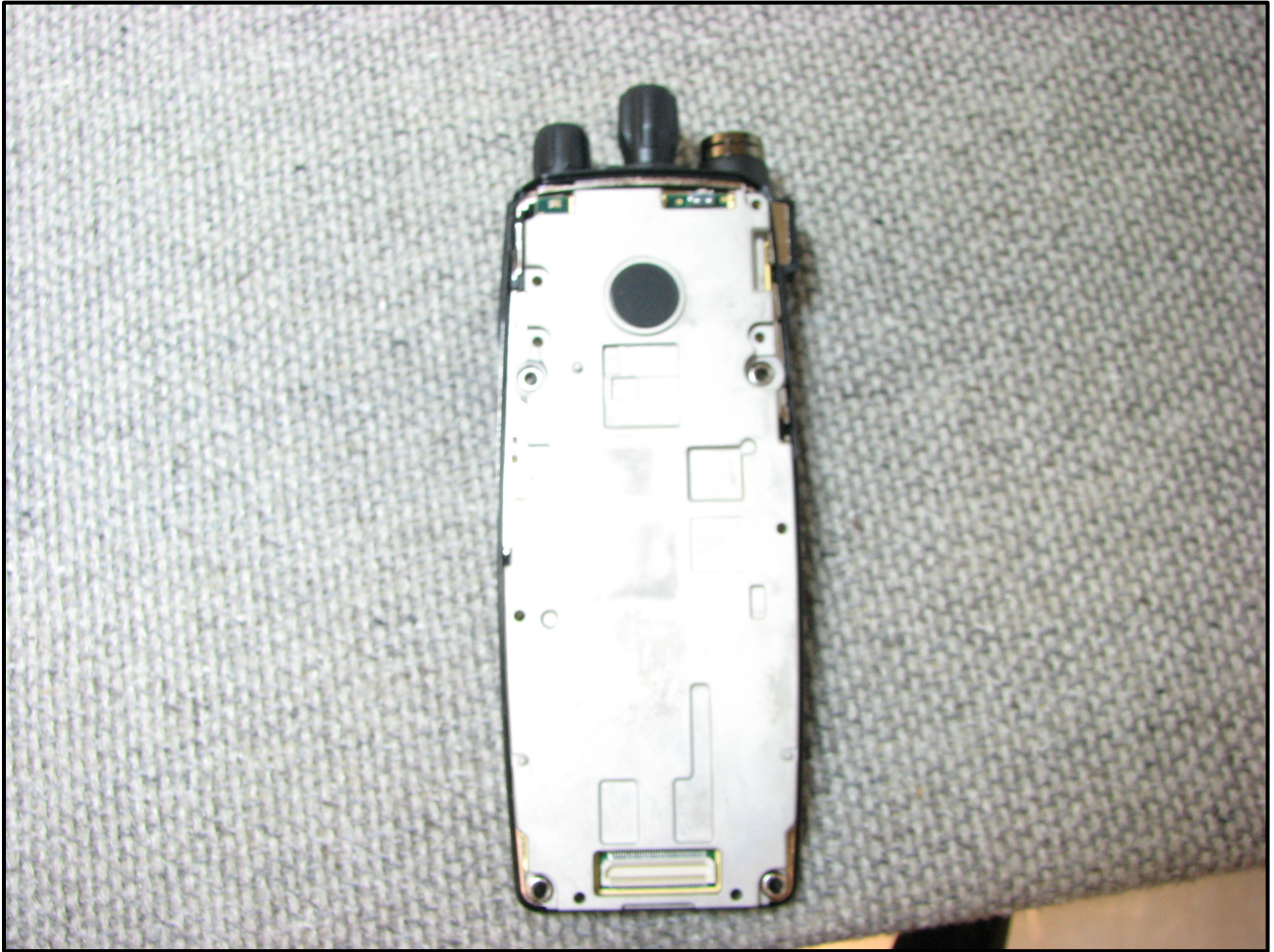
Photograph 29: Radio Shield
