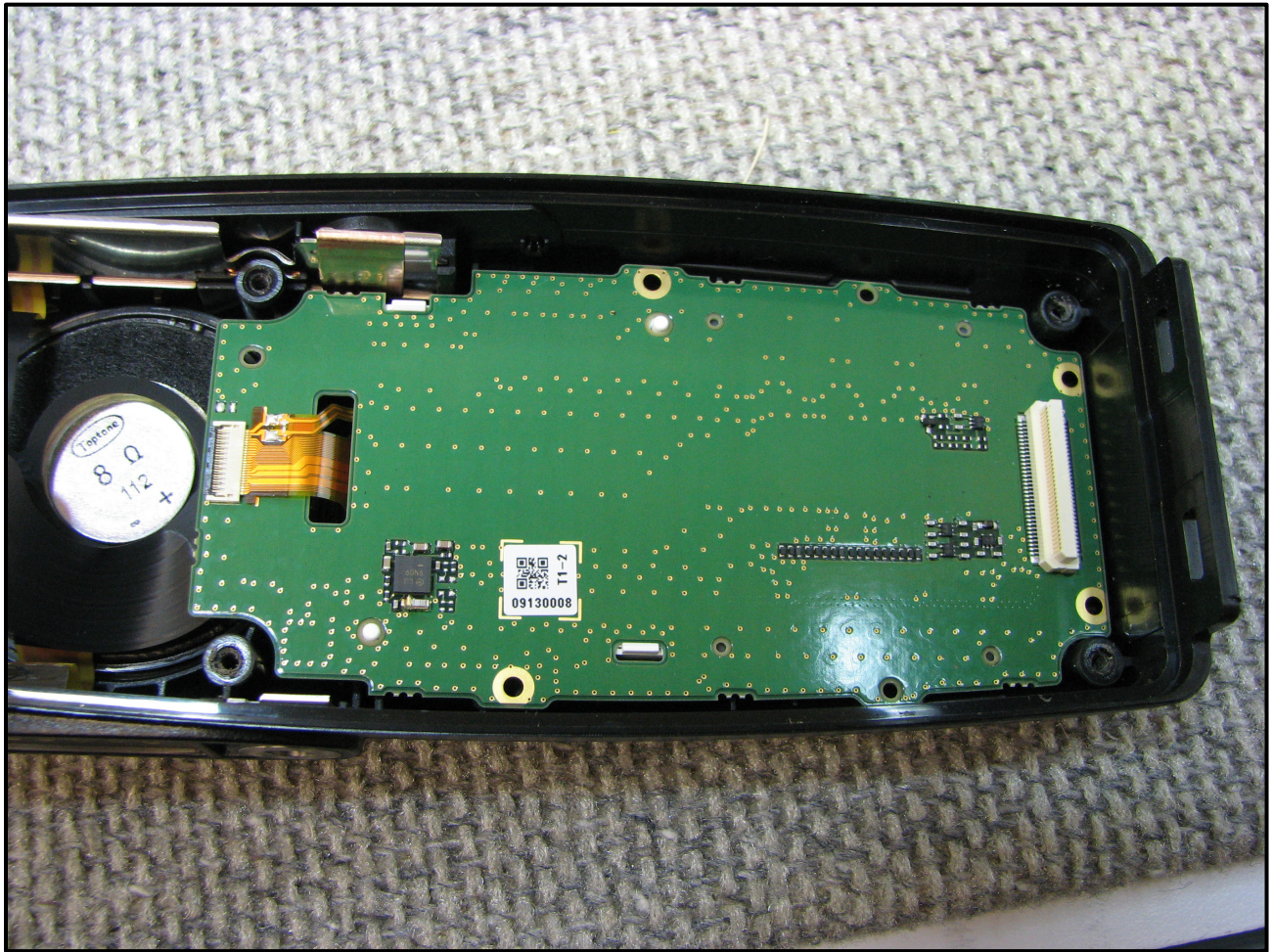
Photograph 28: IF Board 6
