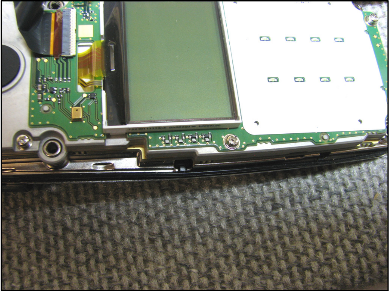
Photograph 24: IF Board 2
