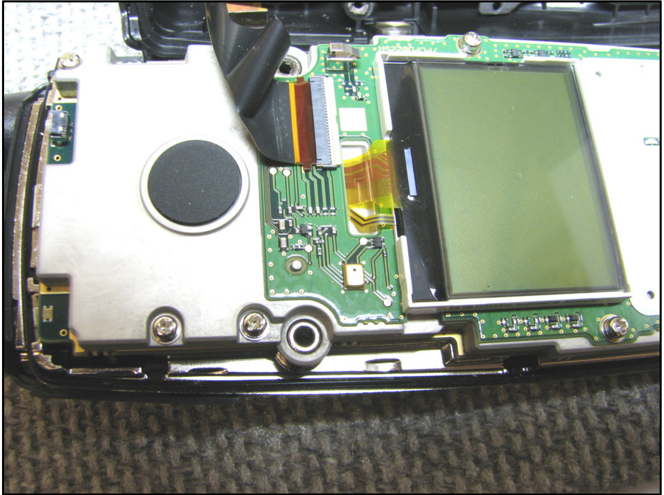
Photograph 23: IF Board 1
