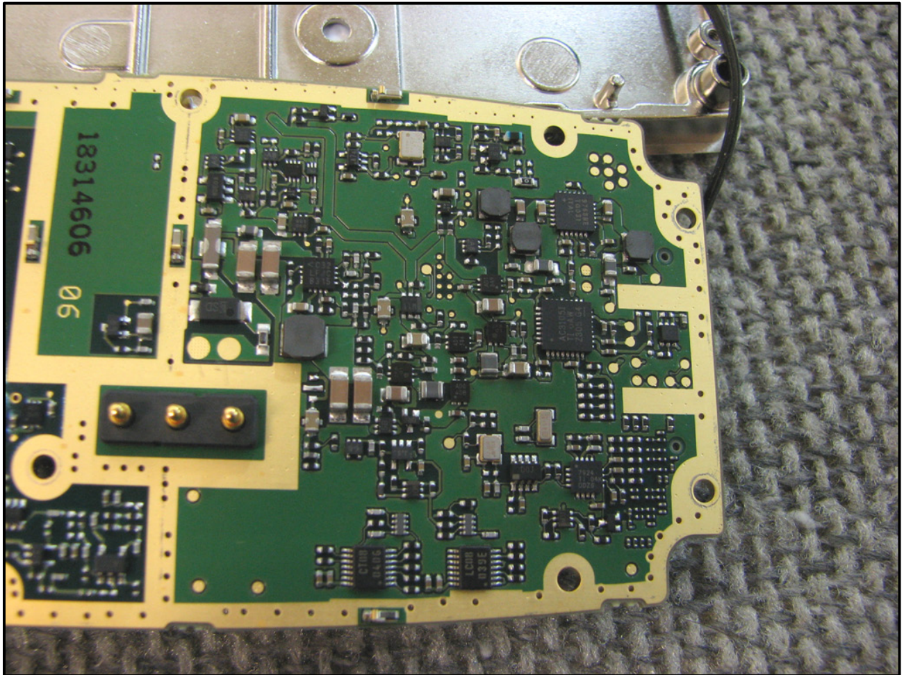
Photograph 22: Main Board 8
