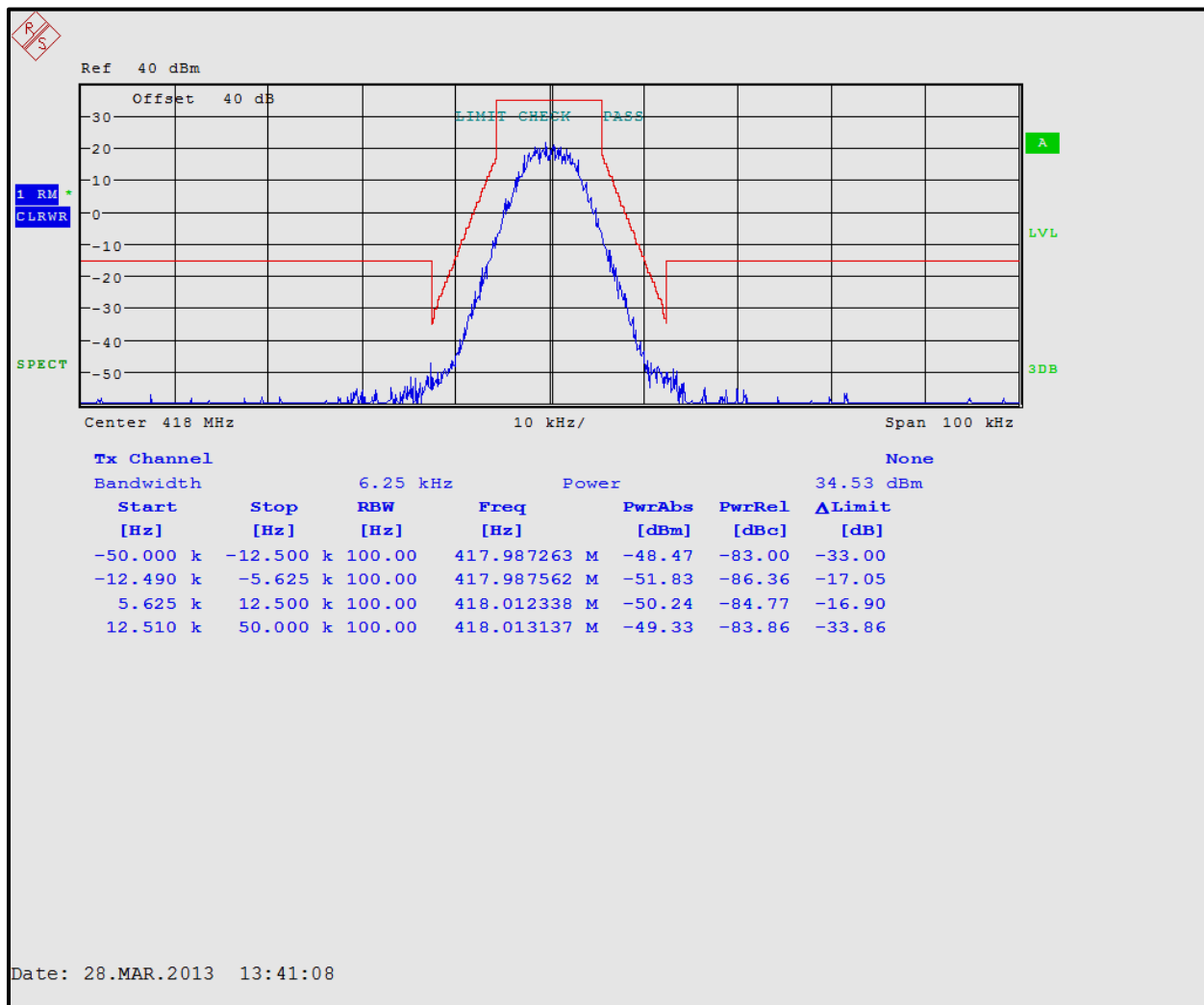
Plot 5-2: Occupied Bandwidth – 418.0 MHz; H-CPM TDMA (Mask D)
