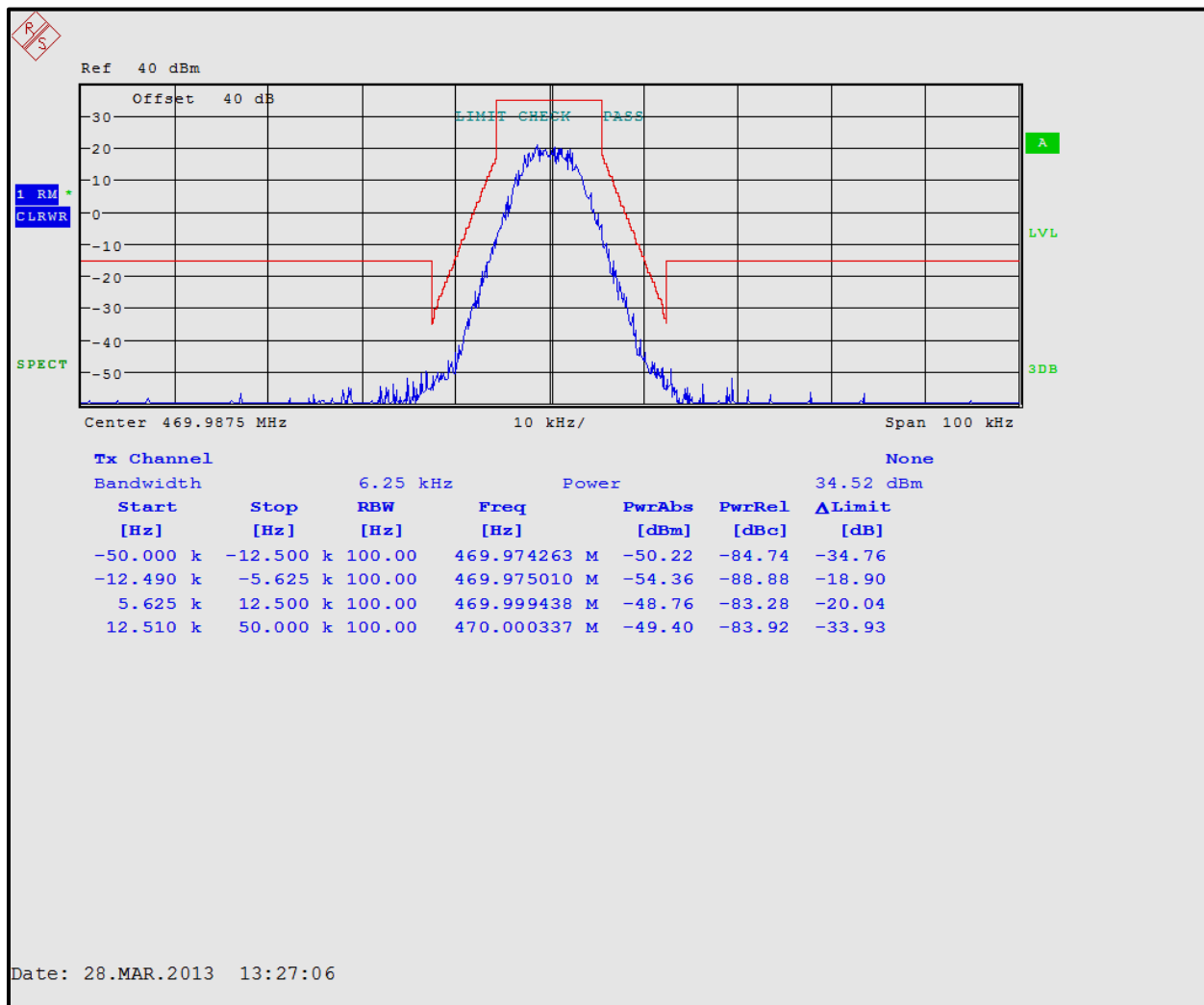
Plot 5-7: Occupied Bandwidth – 469.9875 MHz; H-CPM TDMA (Mask D)
