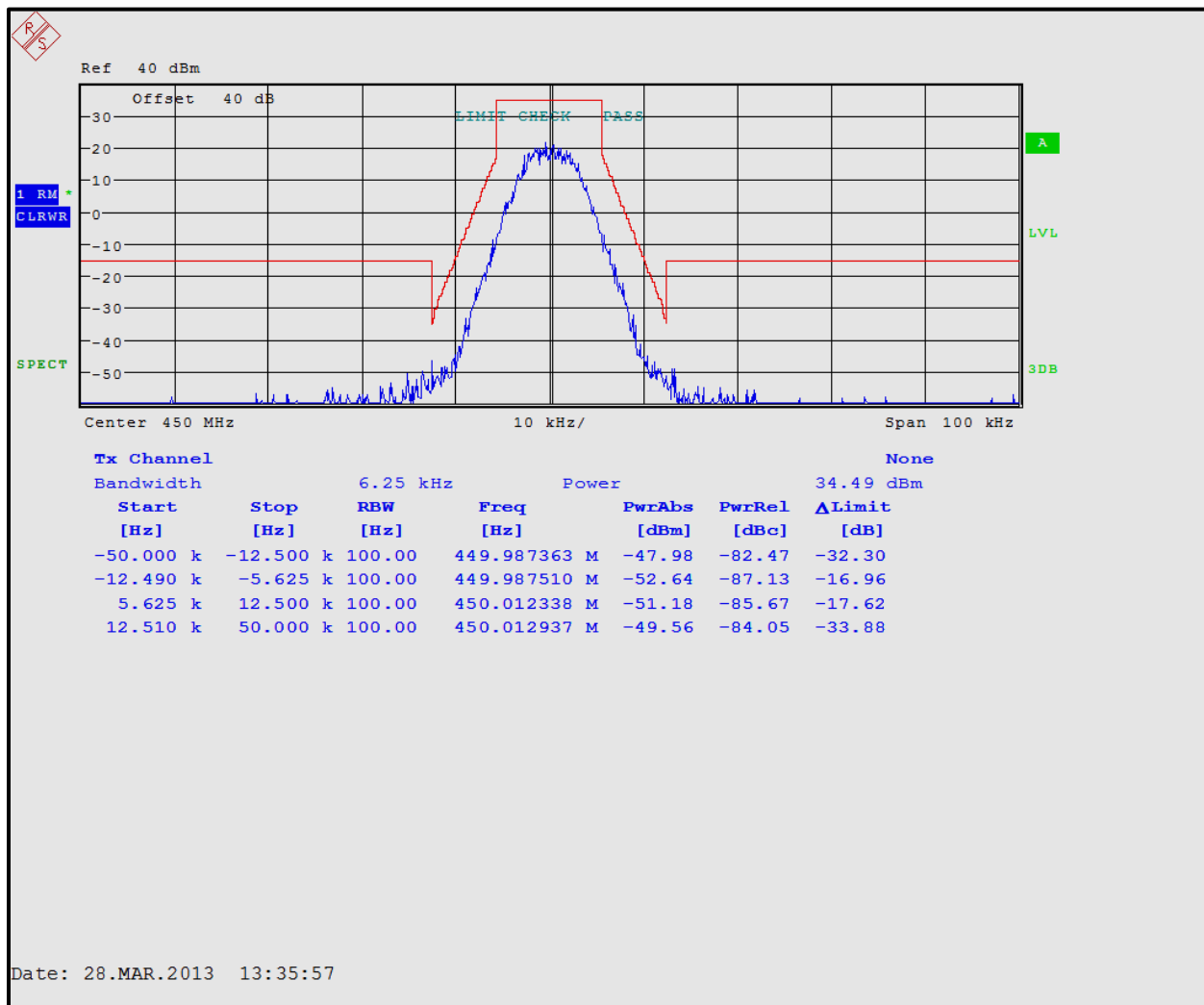
Plot 5-4: Occupied Bandwidth – 450.0 MHz; H-CPM TDMA (Mask D)
