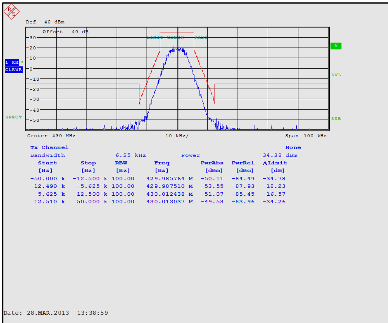
Plot 5-3: Occupied Bandwidth – 430.0 MHz; H-CPM TDMA (Mask D)
