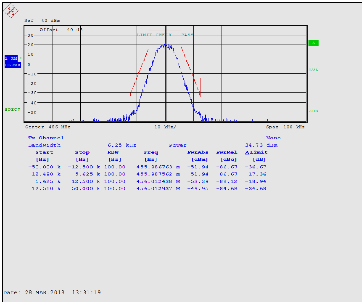
Plot 5-6: Occupied Bandwidth – 456.0 MHz; H-CPM TDMA (Mask D)
