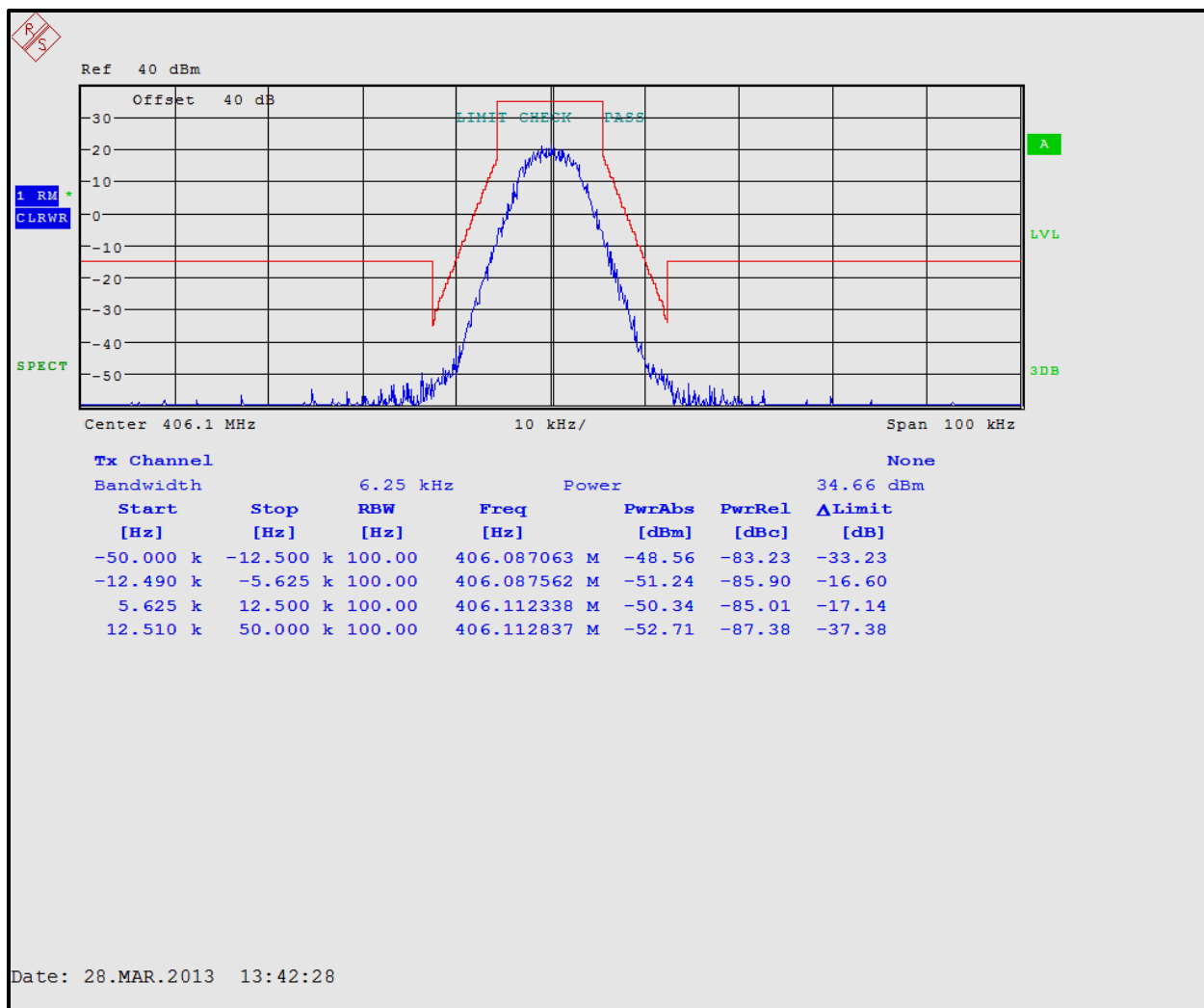
Plot 5-1: Occupied Bandwidth – 406.1 MHz; H-CPM TDMA (Mask D)
