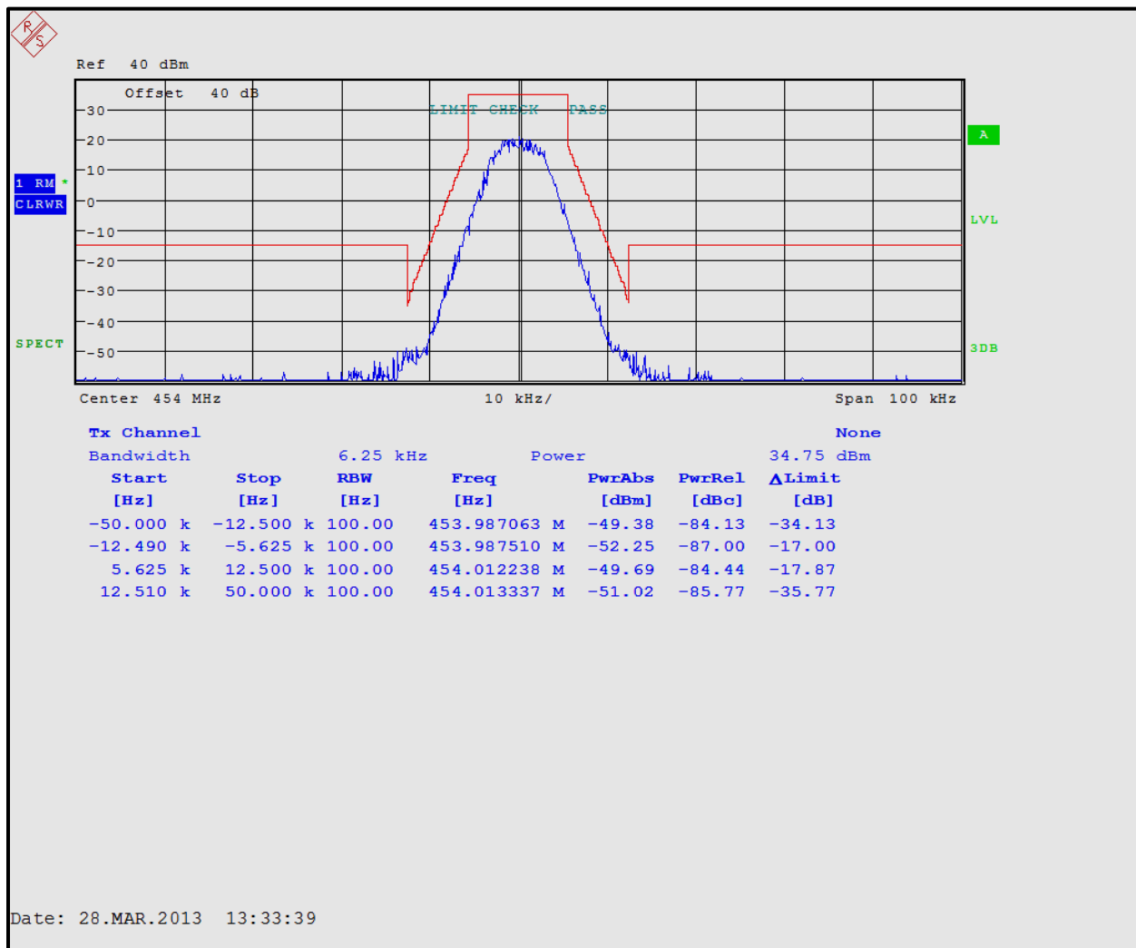
Plot 5-5: Occupied Bandwidth – 454.0 MHz; H-CPM TDMA (Mask D)
