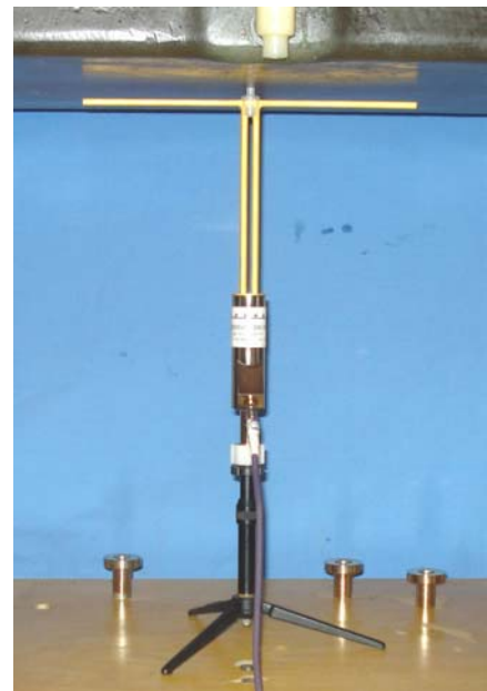
450 MHz SPEAG Validation Dipole Setup
