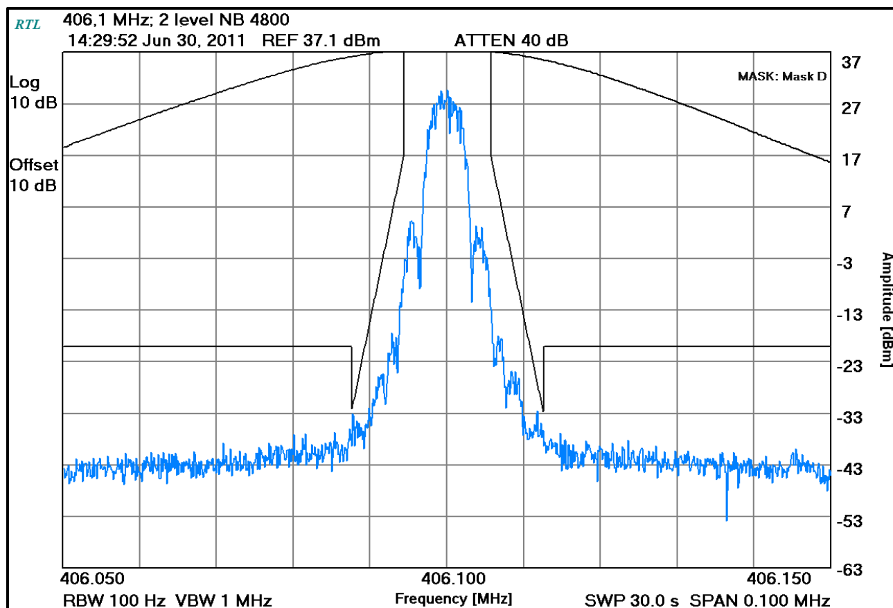
Plot 7-10: Occupied Bandwidth – 406.1 MHz; 2 level NB 4800 (Mask D)
