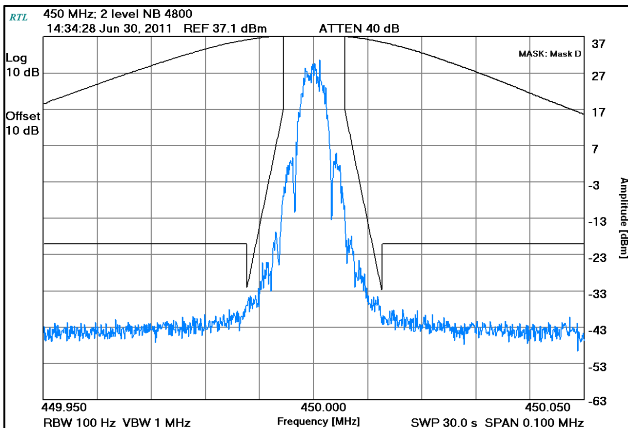
Plot 7-13: Occupied Bandwidth – 450 MHz; 2 level NB 4800 (Mask D)
