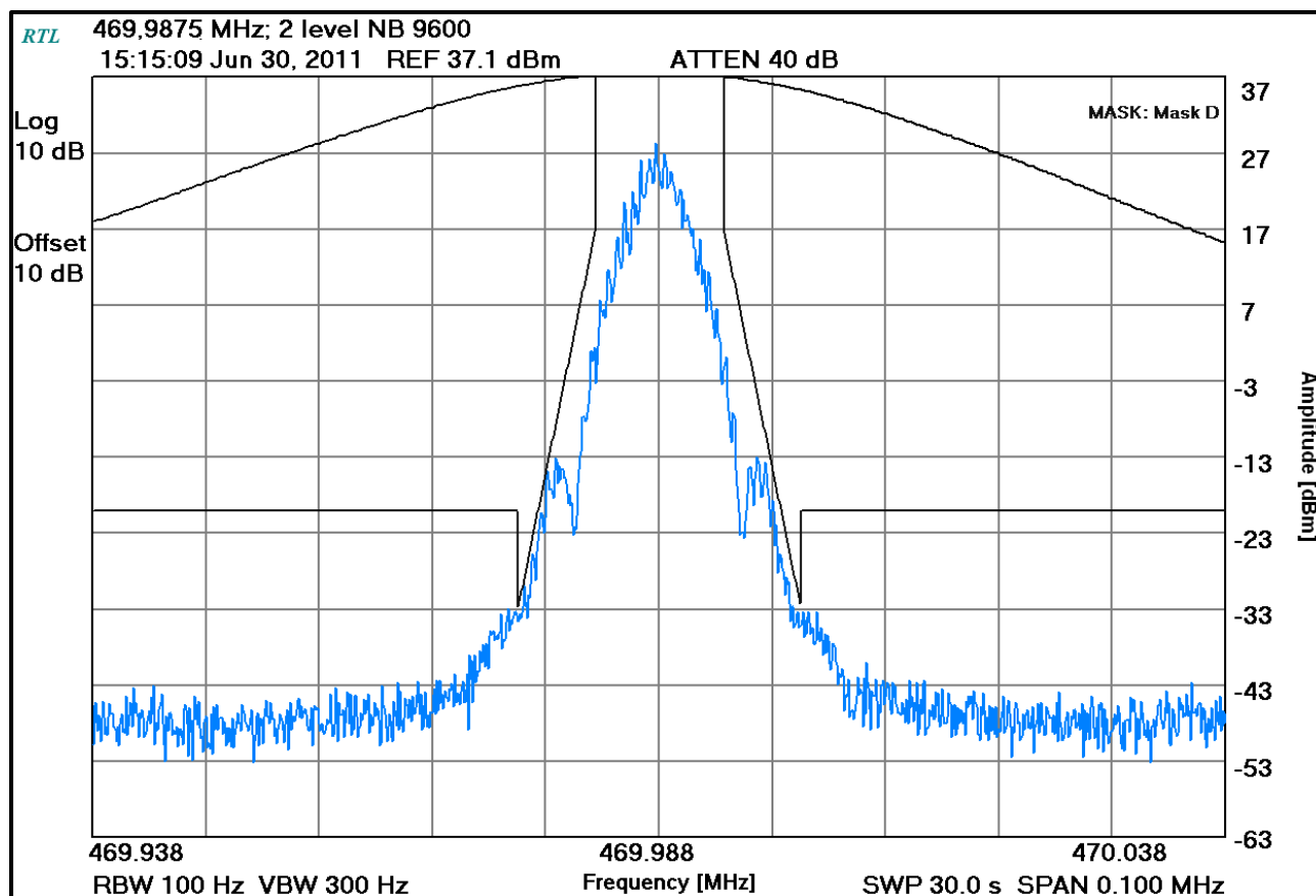
Plot 7-24: Occupied Bandwidth – 469.9875 MHz; 2 level NB 9600 (Mask D)
