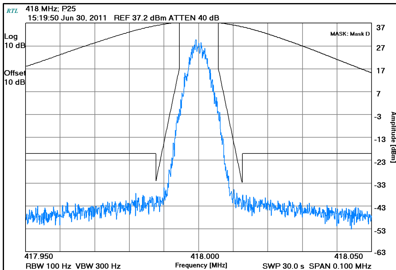
Plot 7-27: Occupied Bandwidth – 418 MHz; P25 (Mask D)
