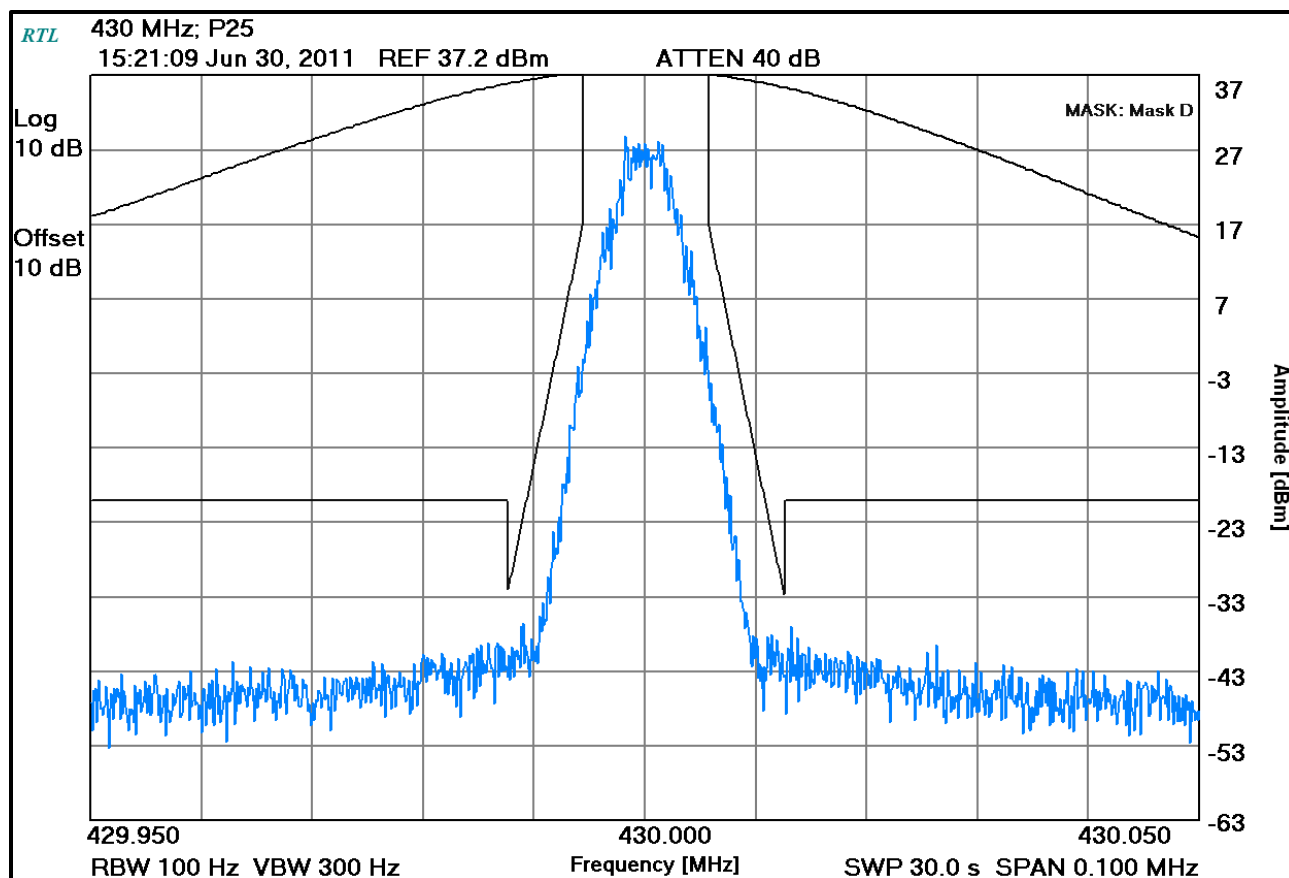
Plot 7-28: Occupied Bandwidth – 430 MHz; P25 (Mask D)
