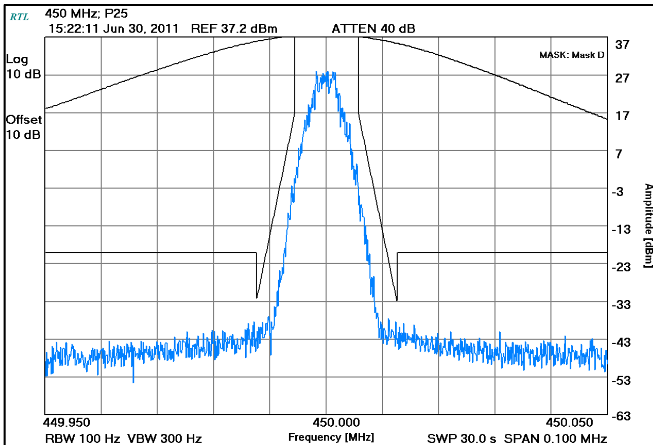
Plot 7-29: Occupied Bandwidth – 450 MHz; P25 (Mask D)
