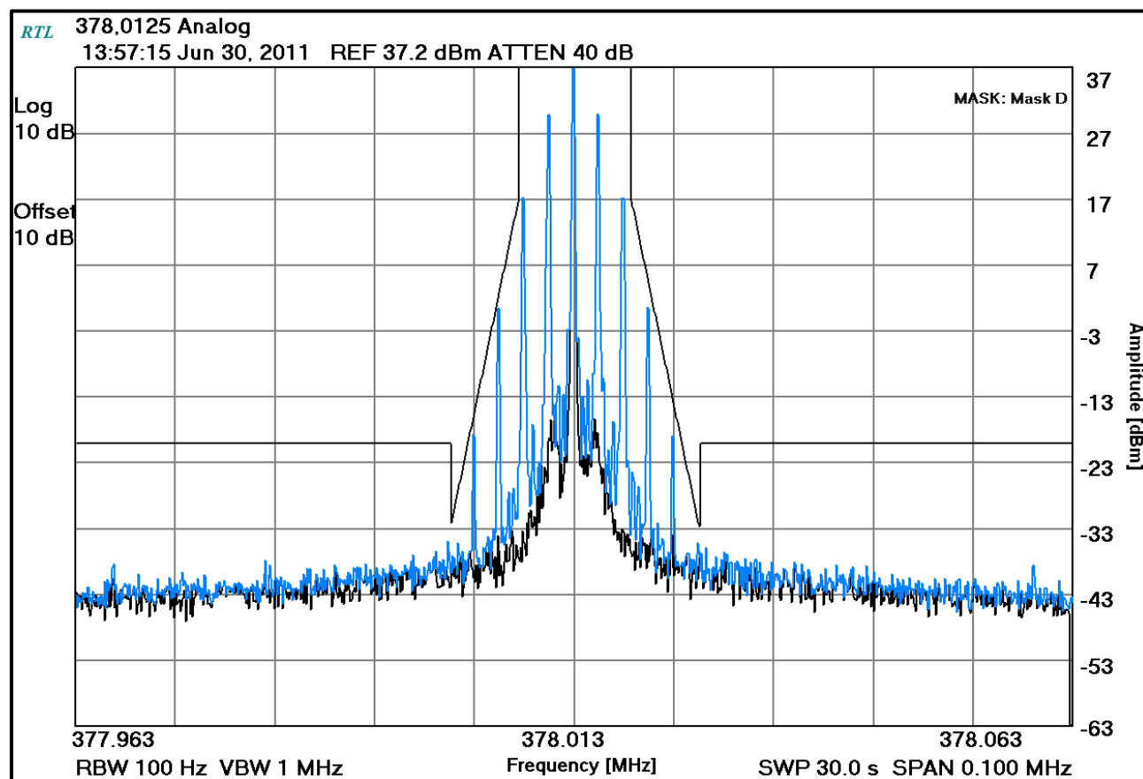
Plot 7-1: Occupied Bandwidth – 378.0125 MHz; Analog (Mask D)
