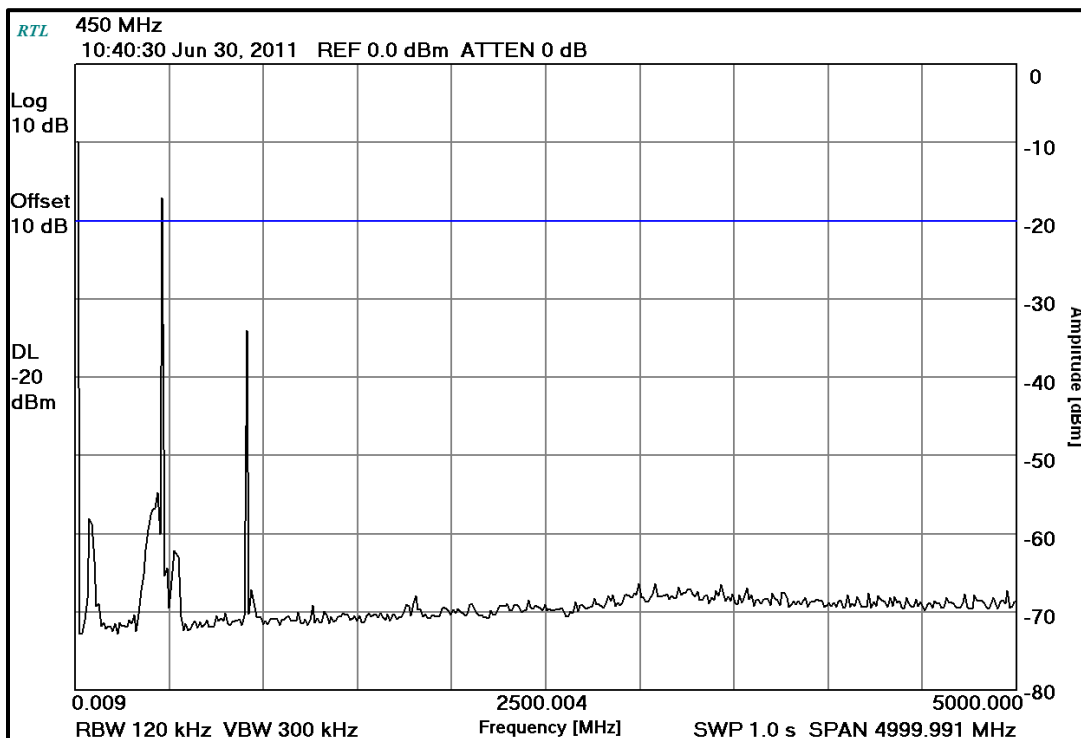
Plot 5-5: Conducted Spurious - 450 MHz - Analog High Power
