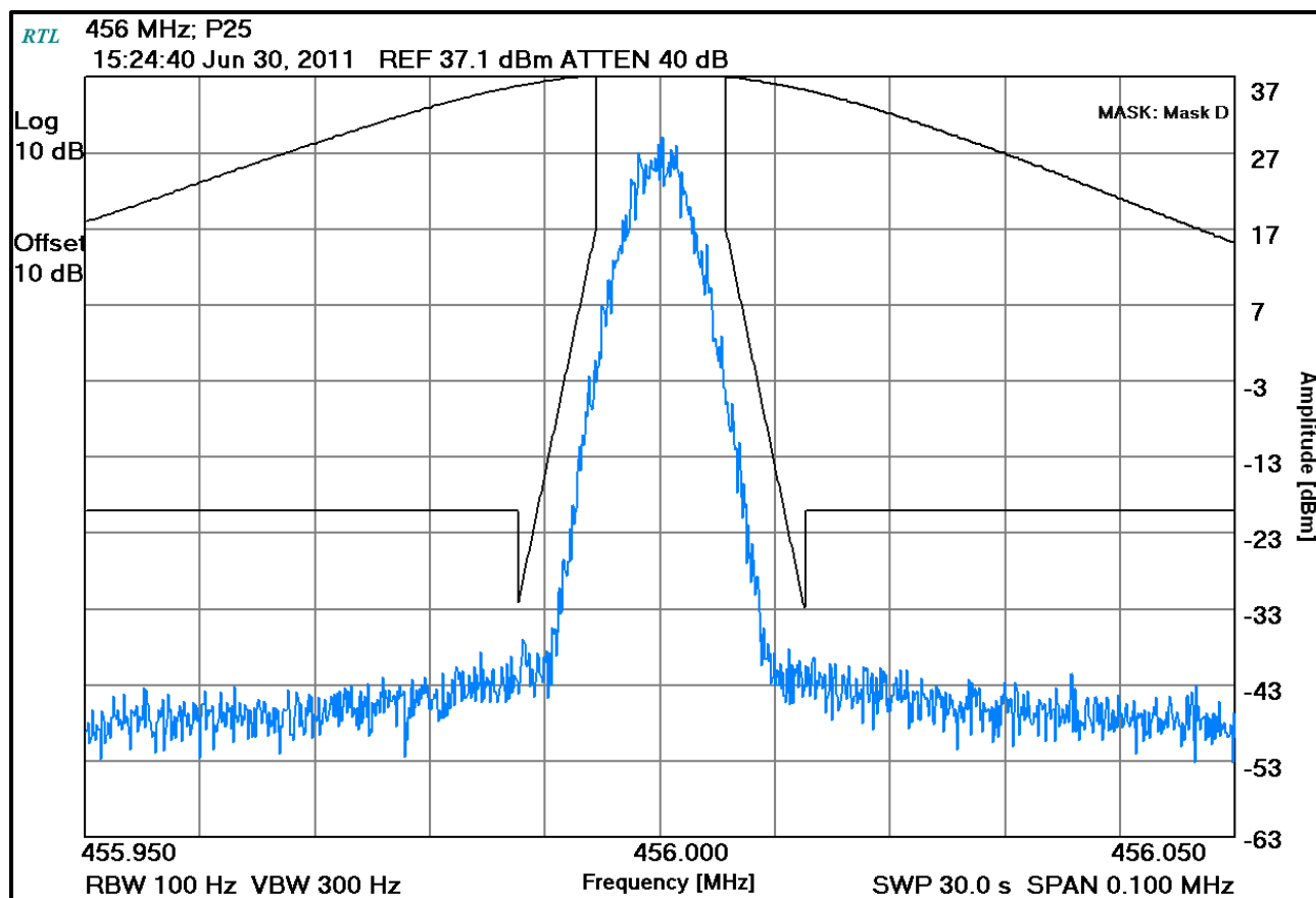
Plot 7-31: Occupied Bandwidth – 456 MHz; P25 (Mask D)
