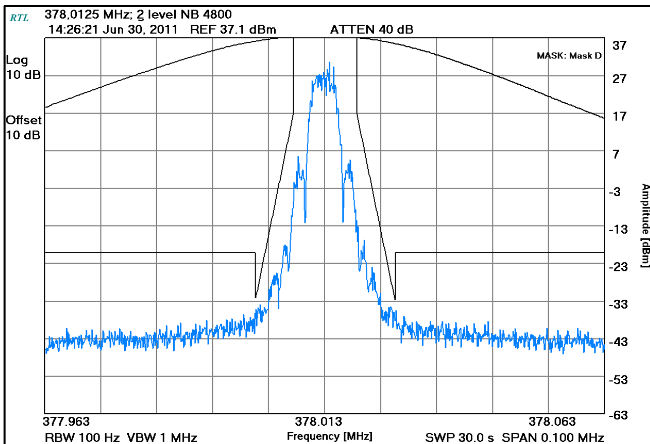
Plot 7-9: Occupied Bandwidth – 378.0125 MHz; 2 level NB 4800 (Mask D)
