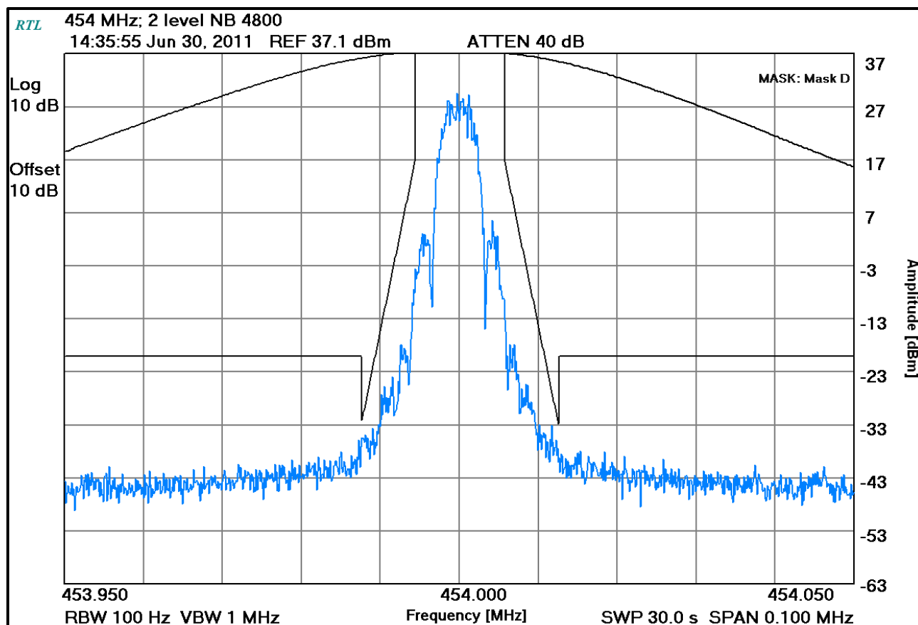
Plot 7-14: Occupied Bandwidth – 454 MHz; 2 level NB 4800 (Mask D)
