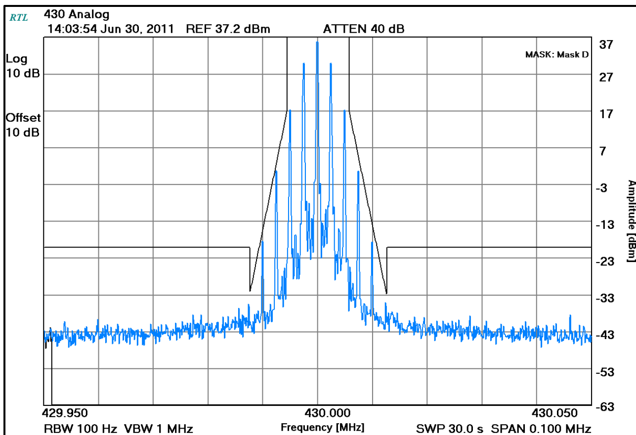
Plot 7-4: Occupied Bandwidth – 430 MHz; Analog (Mask D)
