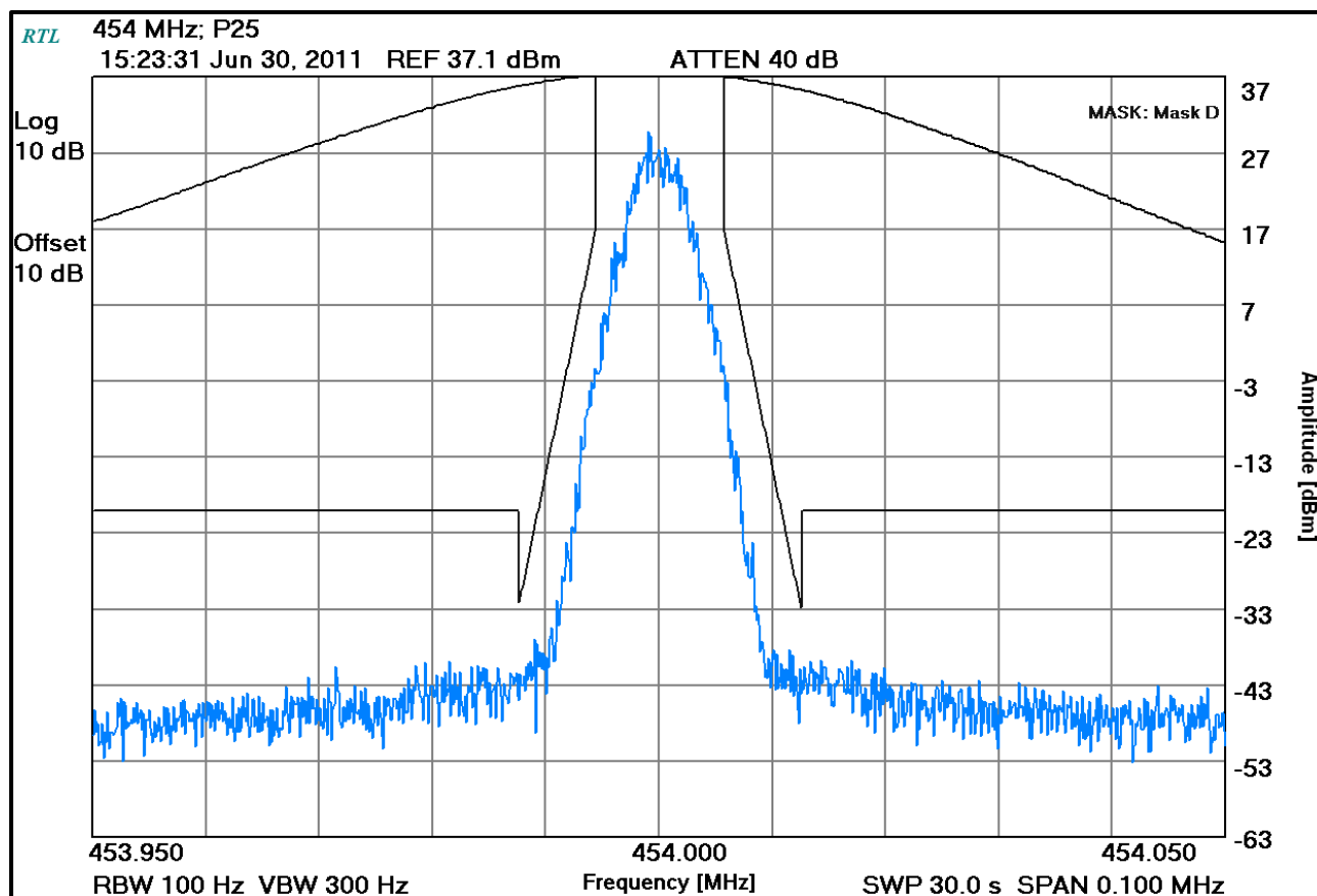
Plot 7-30: Occupied Bandwidth – 454 MHz; P25 (Mask D)
