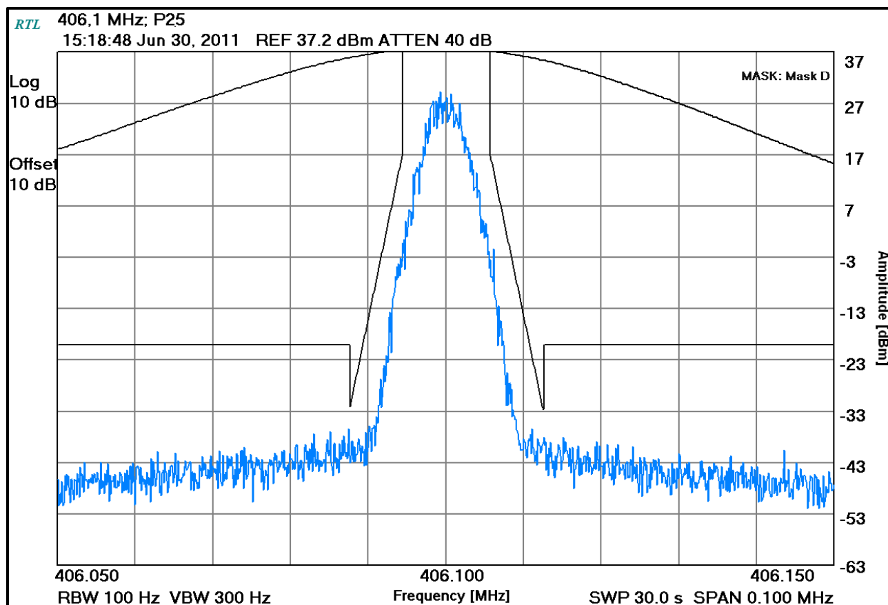
Plot 7-26: Occupied Bandwidth – 406.1 MHz; P25 (Mask D)
