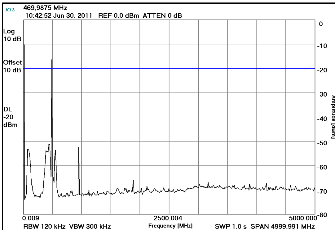
Plot 5-8: Conducted Spurious – 469.9875 MHz – Analog High Power
