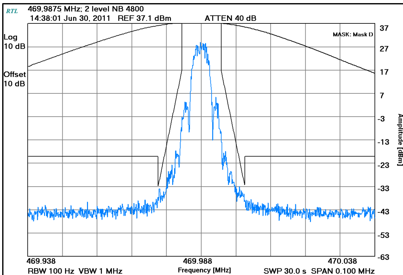
Plot 7-16: Occupied Bandwidth – 469.9875 MHz; 2 level NB 4800 (Mask D)
