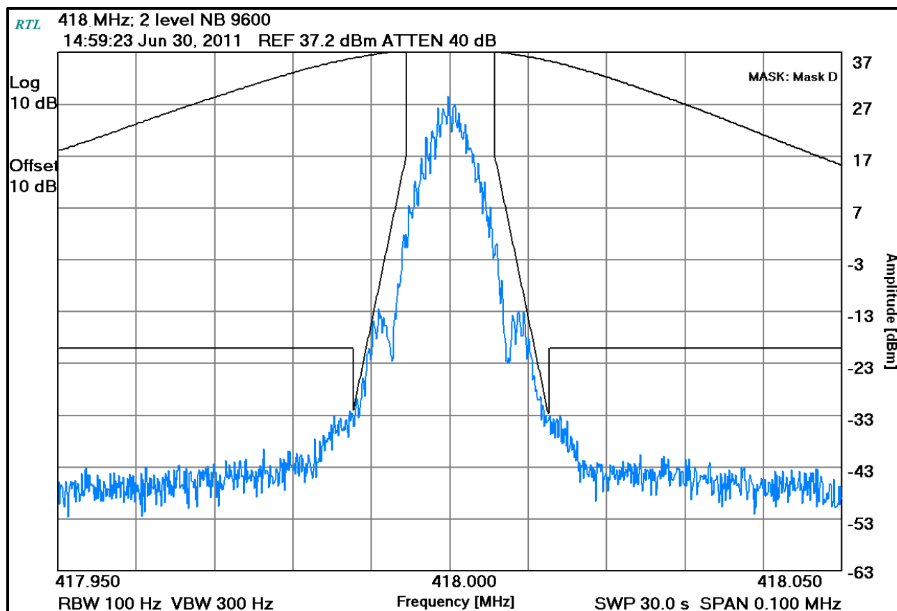
Plot 7-19: Occupied Bandwidth – 418 MHz; 2 level NB 9600 (Mask D)
