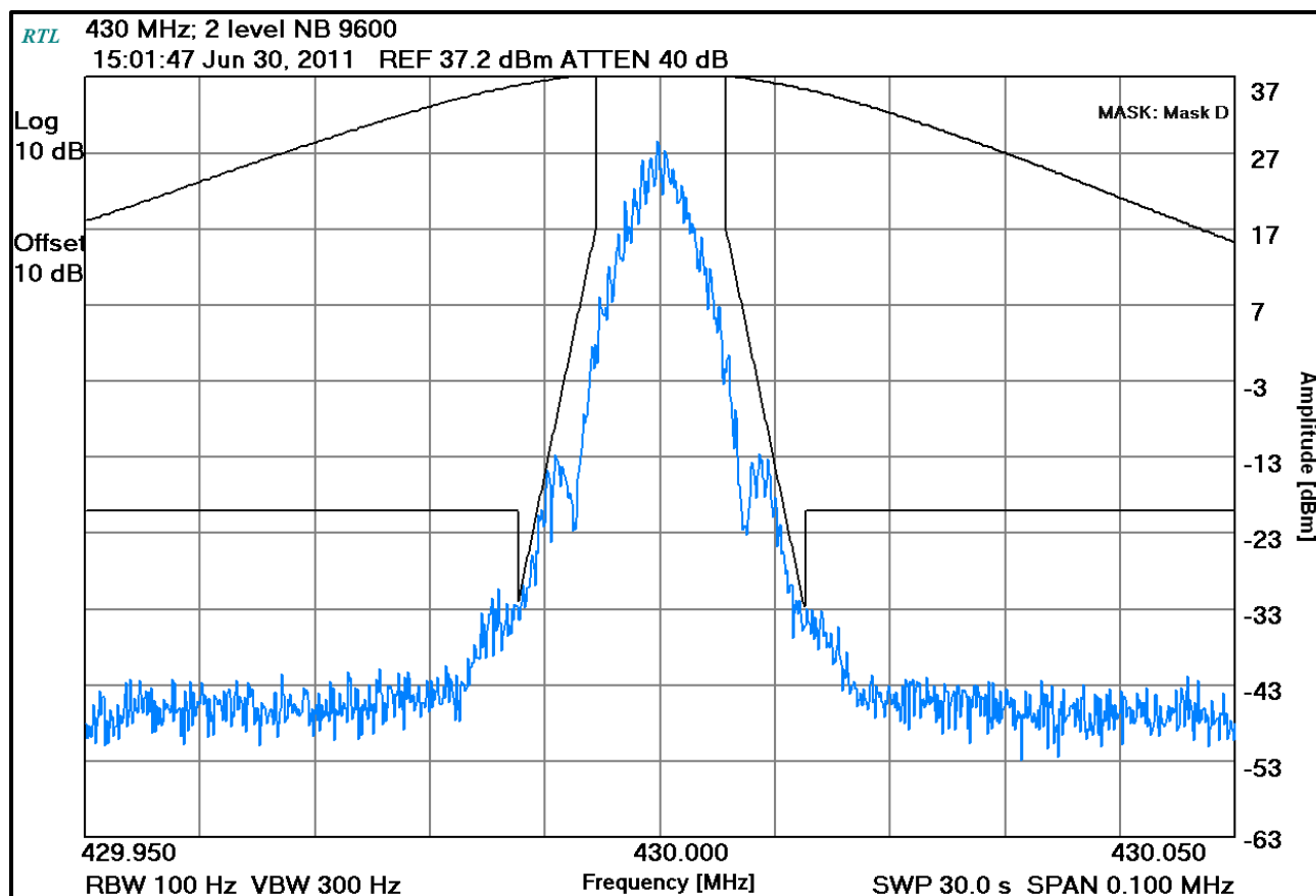
Plot 7-20: Occupied Bandwidth – 430 MHz; 2 level NB 9600 (Mask D)
