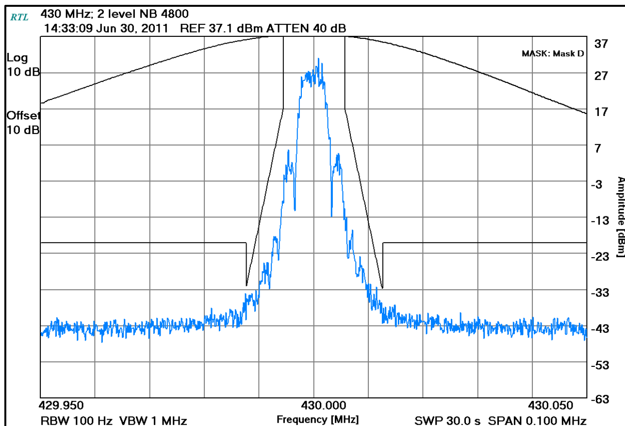
Plot 7-12: Occupied Bandwidth – 430 MHz; 2 level NB 4800 (Mask D)
