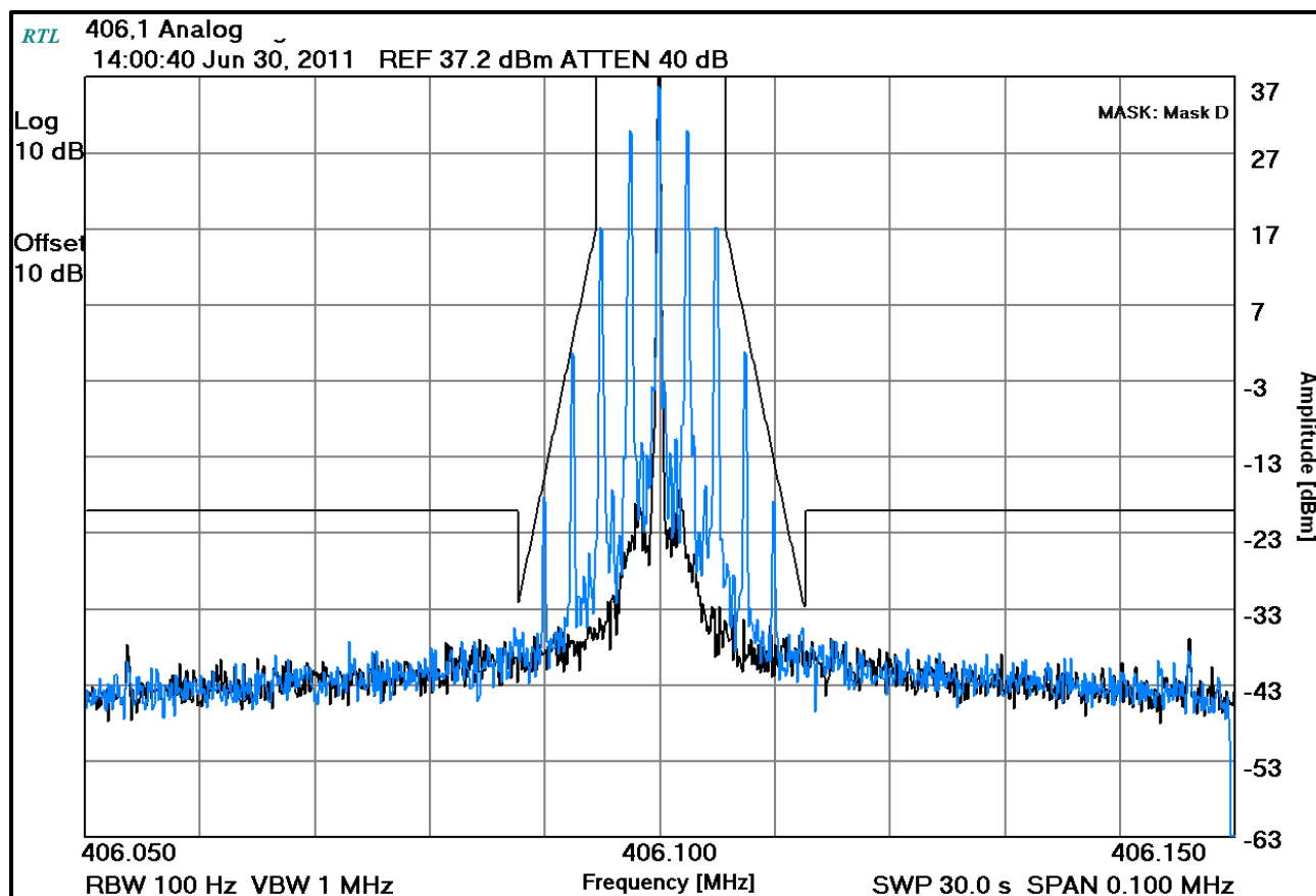
Plot 7-2: Occupied Bandwidth – 406.1 MHz; Analog (Mask D)
