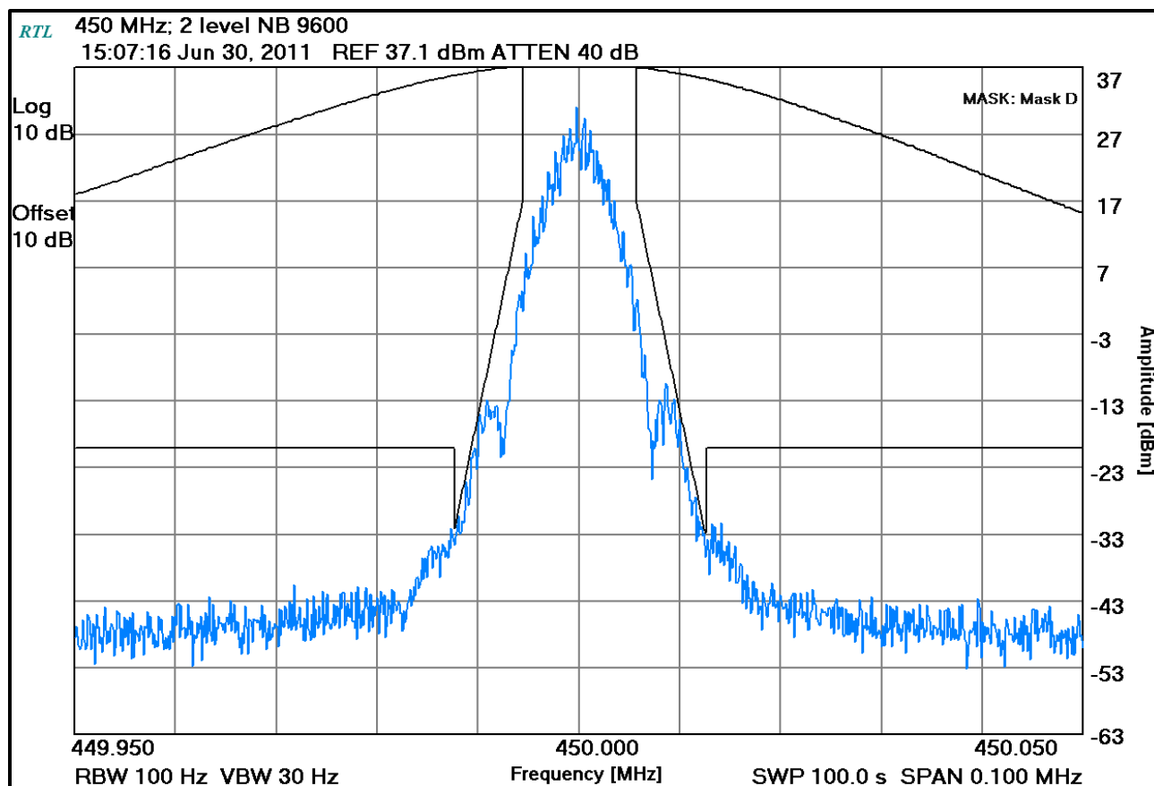
Plot 7-21: Occupied Bandwidth – 450 MHz; 2 level NB 9600 (Mask D)
