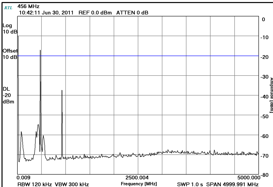
Plot 5-7: Conducted Spurious – 456 MHz – Analog High Power
