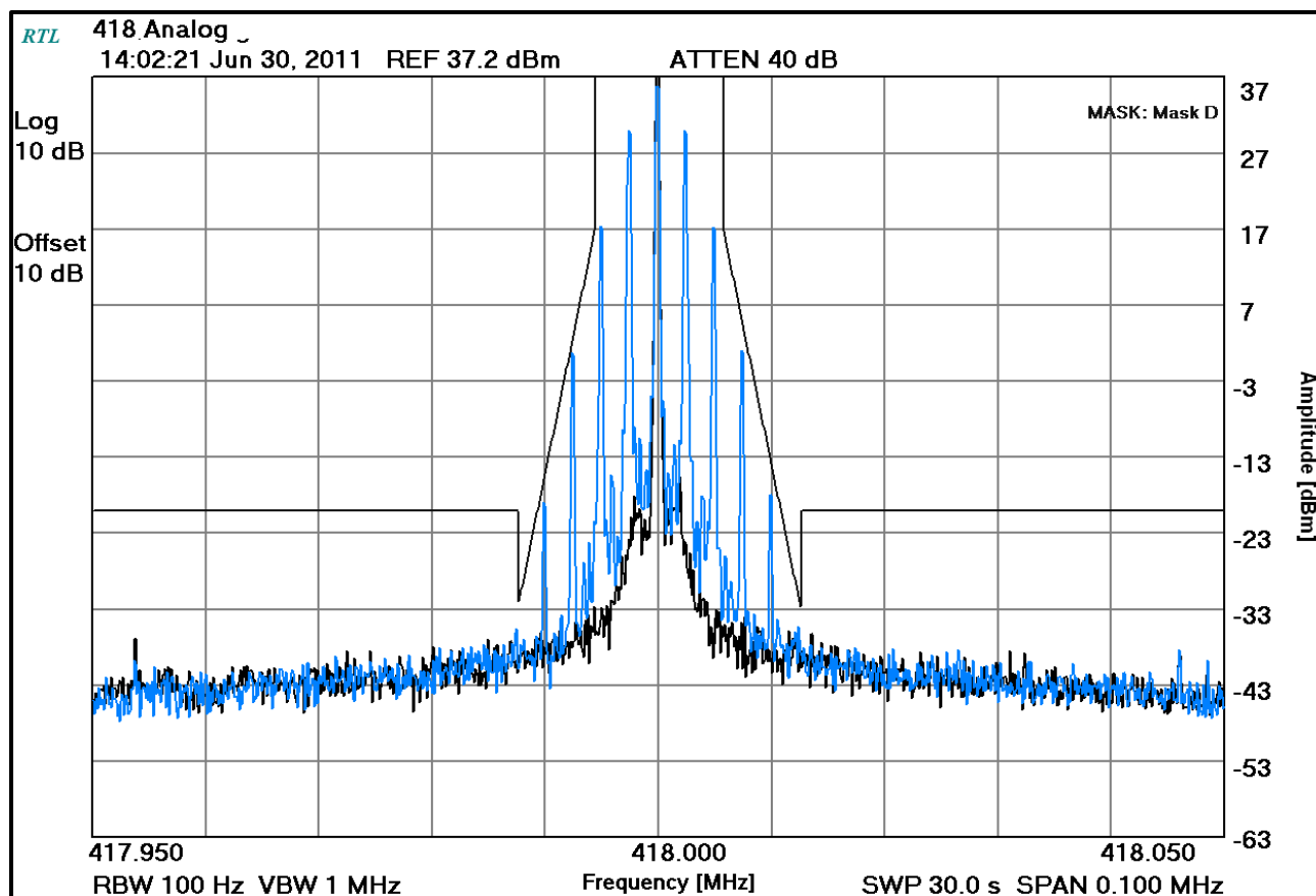
Plot 7-3: Occupied Bandwidth – 418 MHz; Analog (Mask D)
