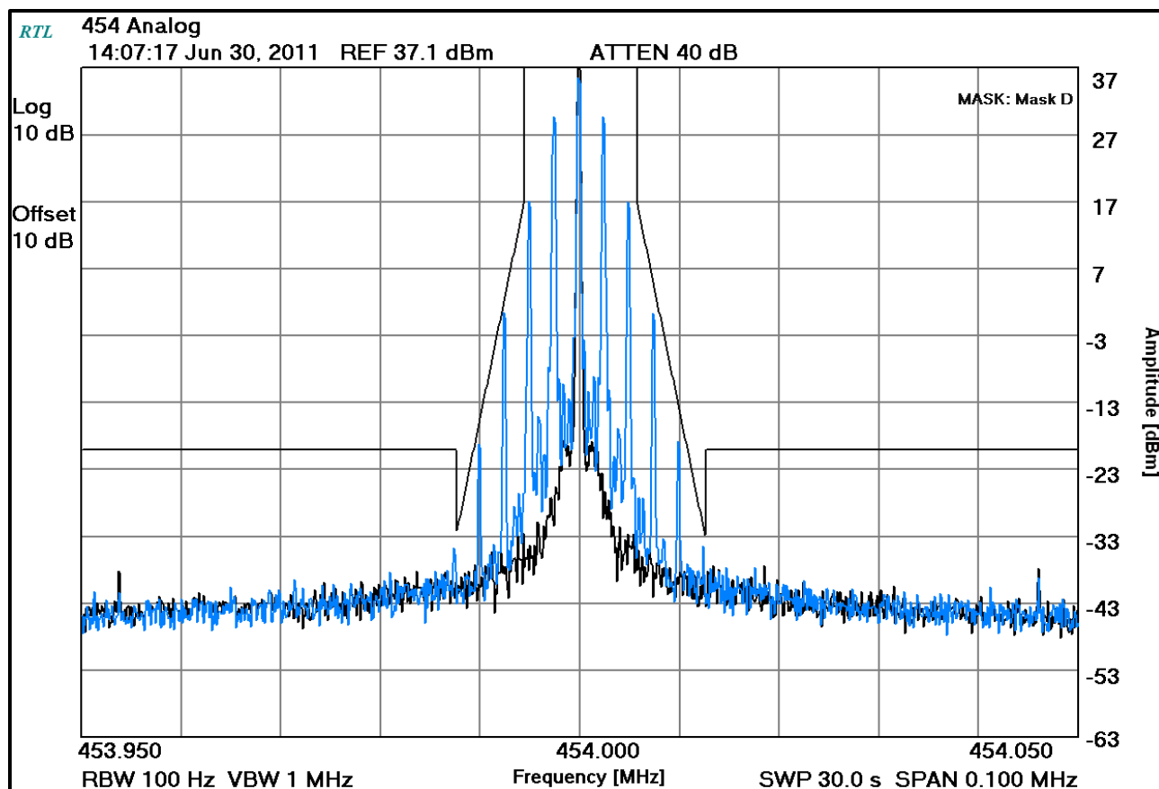
Plot 7-6: Occupied Bandwidth – 454 MHz; Analog (Mask D)
