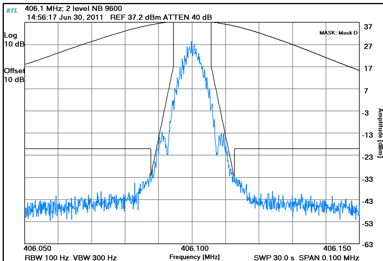
Plot 7-18: Occupied Bandwidth – 406.1 MHz; 2 level NB 9600 (Mask D)
