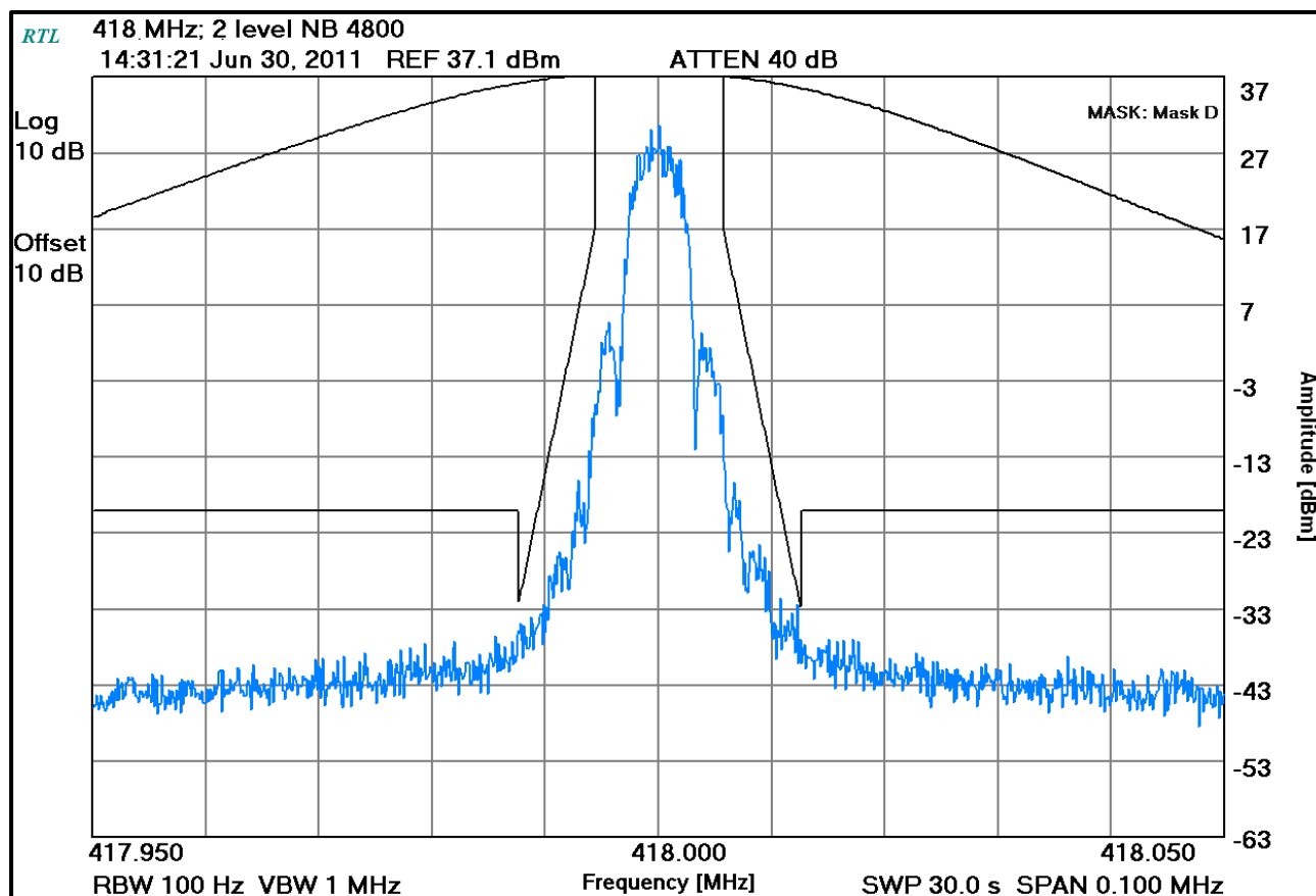
Plot 7-11: Occupied Bandwidth – 418 MHz; 2 level NB 4800 (Mask D)
