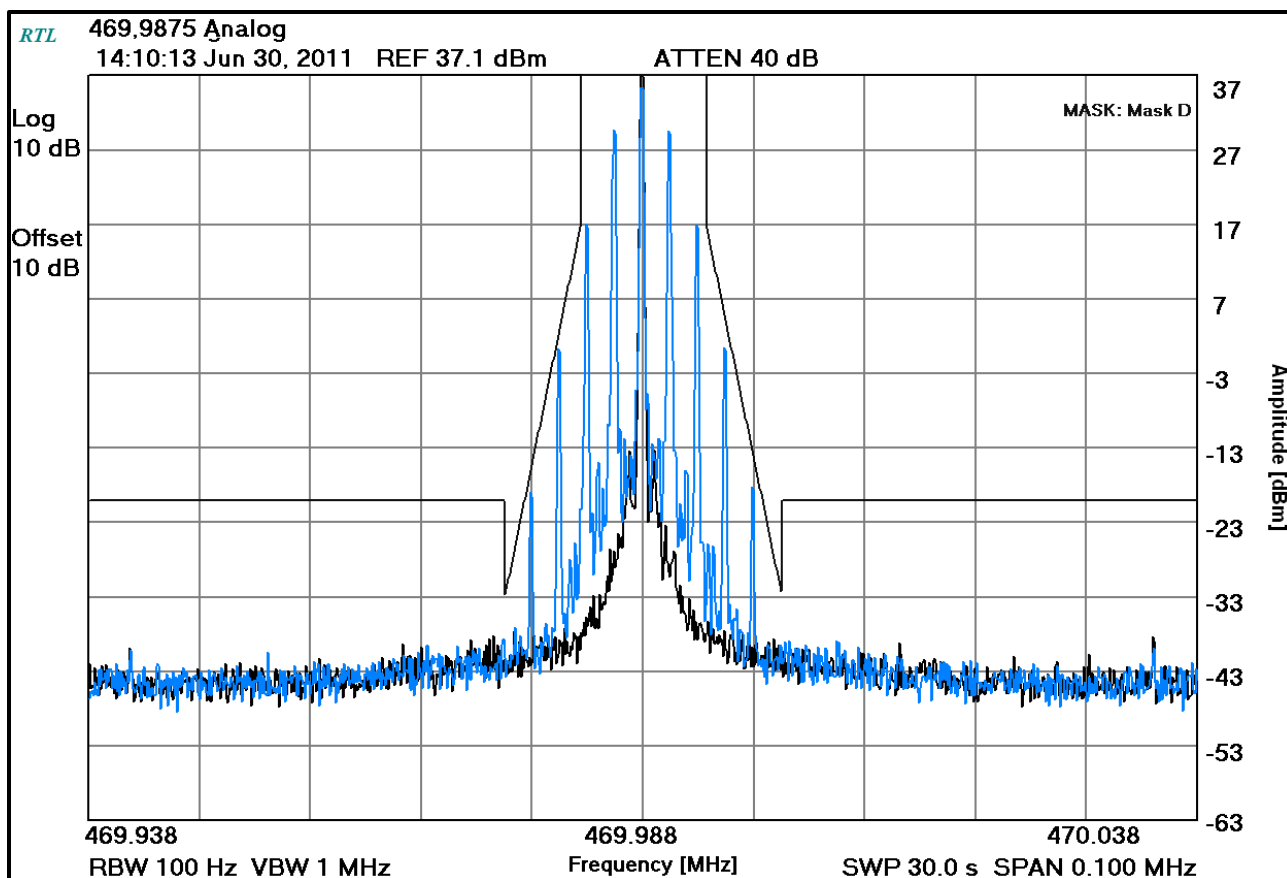
Plot 7-8: Occupied Bandwidth – 469.9875 MHz; Analog (Mask D)
