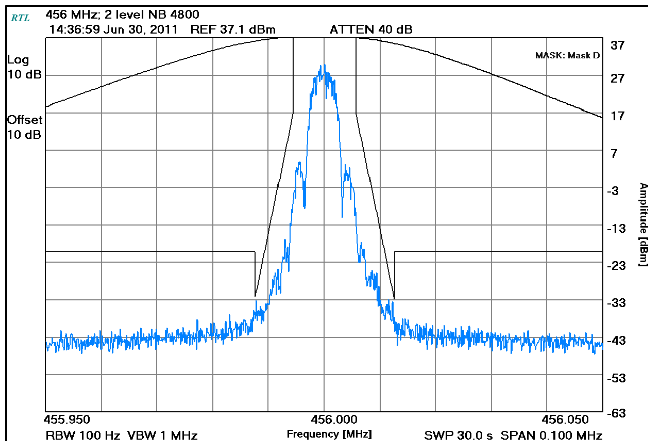
Plot 7-15: Occupied Bandwidth – 456 MHz; 2 level NB 4800 (Mask D)
