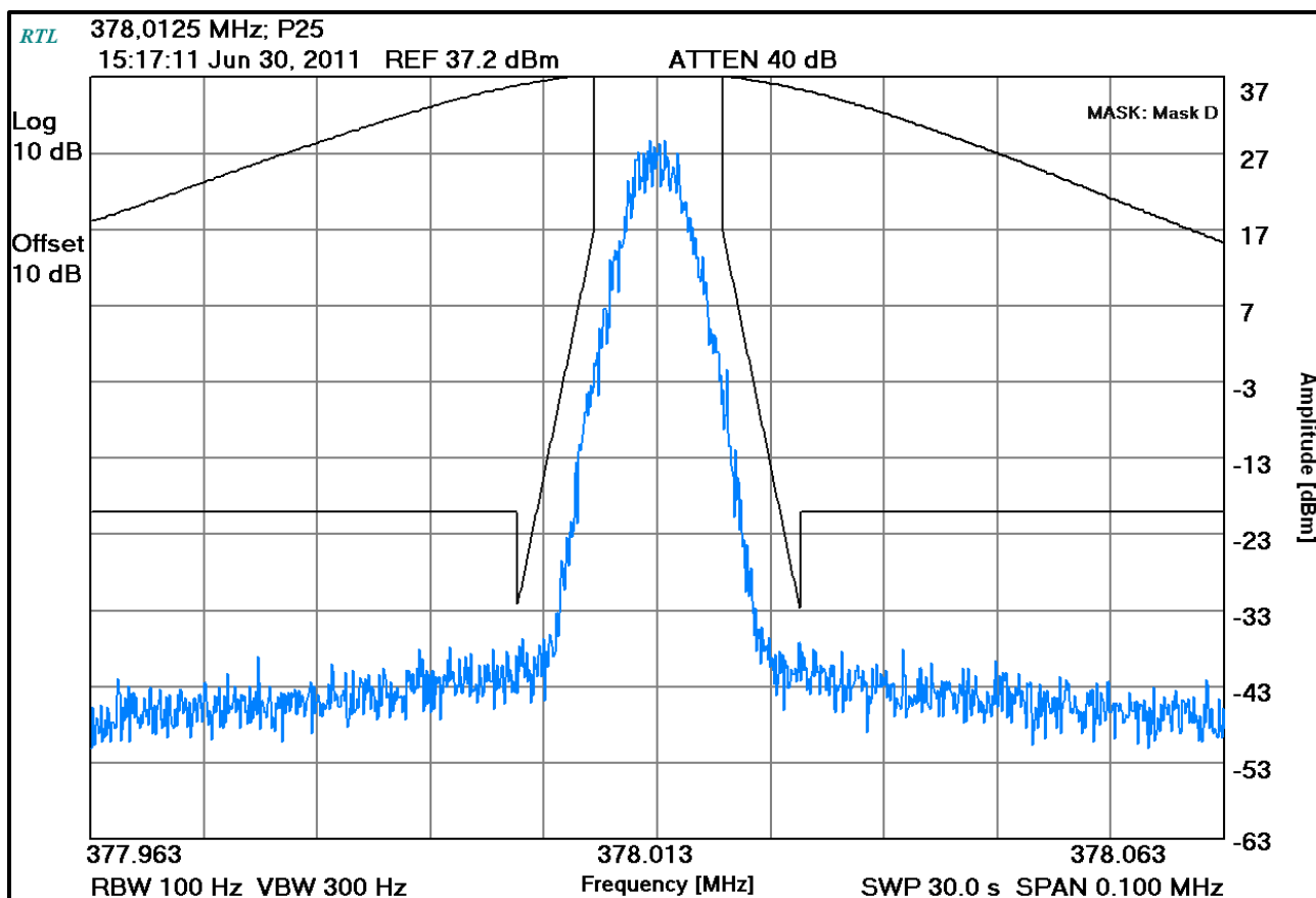
Plot 7-25: Occupied Bandwidth – 378.0125 MHz; P25 (Mask D)
