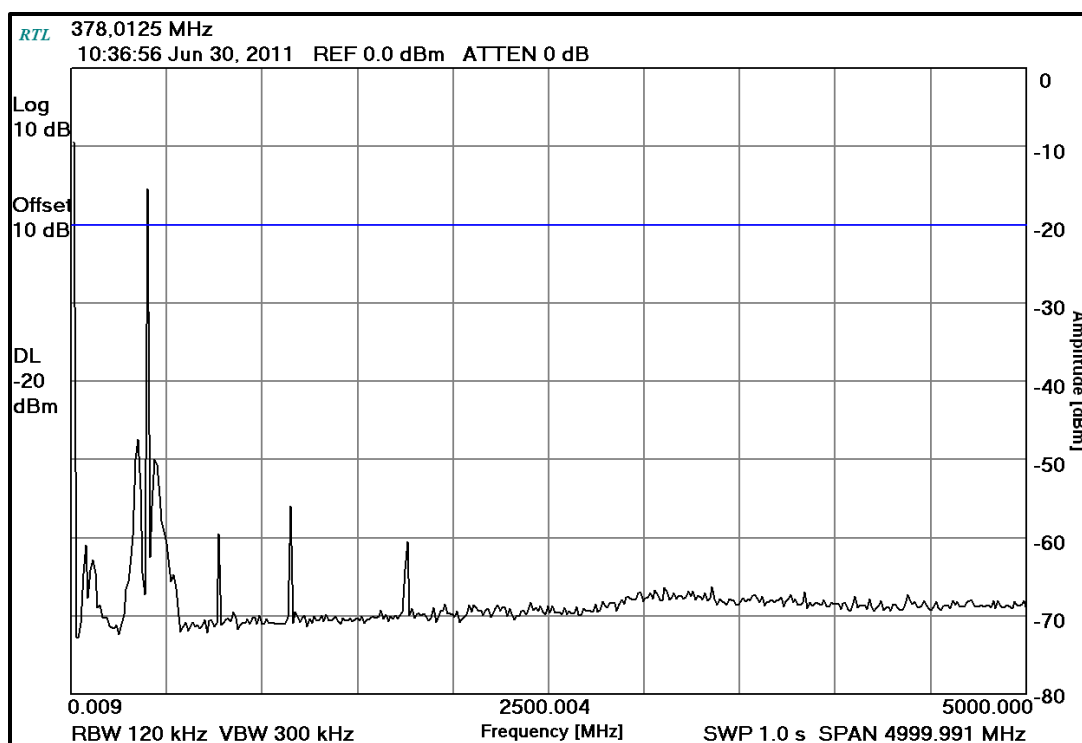
Plot 5-1: Conducted Spurious - 378.0125 MHz - Analog High Power
