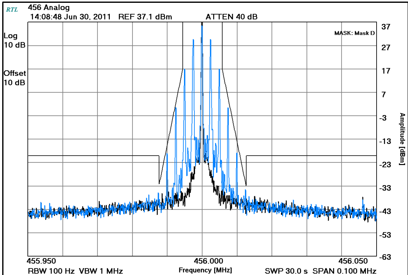
Plot 7-7: Occupied Bandwidth – 456 MHz; Analog (Mask D)
