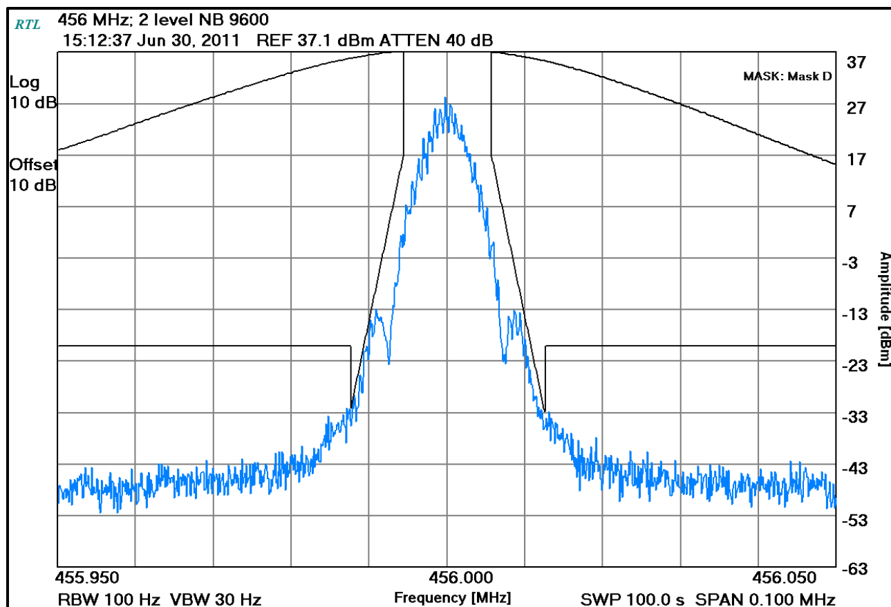
Plot 7-23: Occupied Bandwidth – 456 MHz; 2 level NB 9600 (Mask D)
