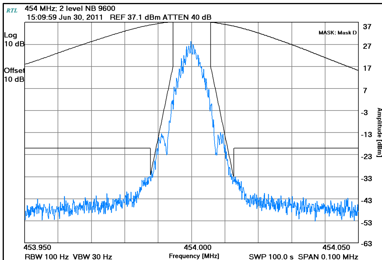
Plot 7-22: Occupied Bandwidth – 454 MHz; 2 level NB 9600 (Mask D)
