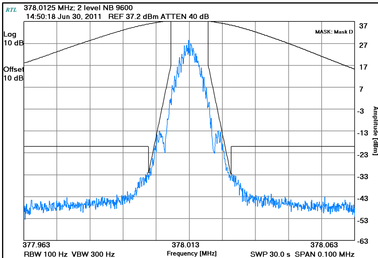
Plot 7-17: Occupied Bandwidth – 378.0125 MHz; 2 level NB 9600 (Mask D)
