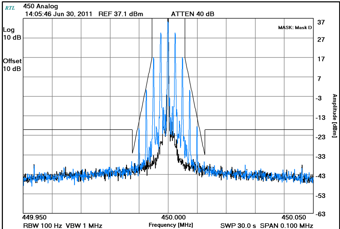
Plot 7-5: Occupied Bandwidth – 450 MHz; Analog (Mask D)
