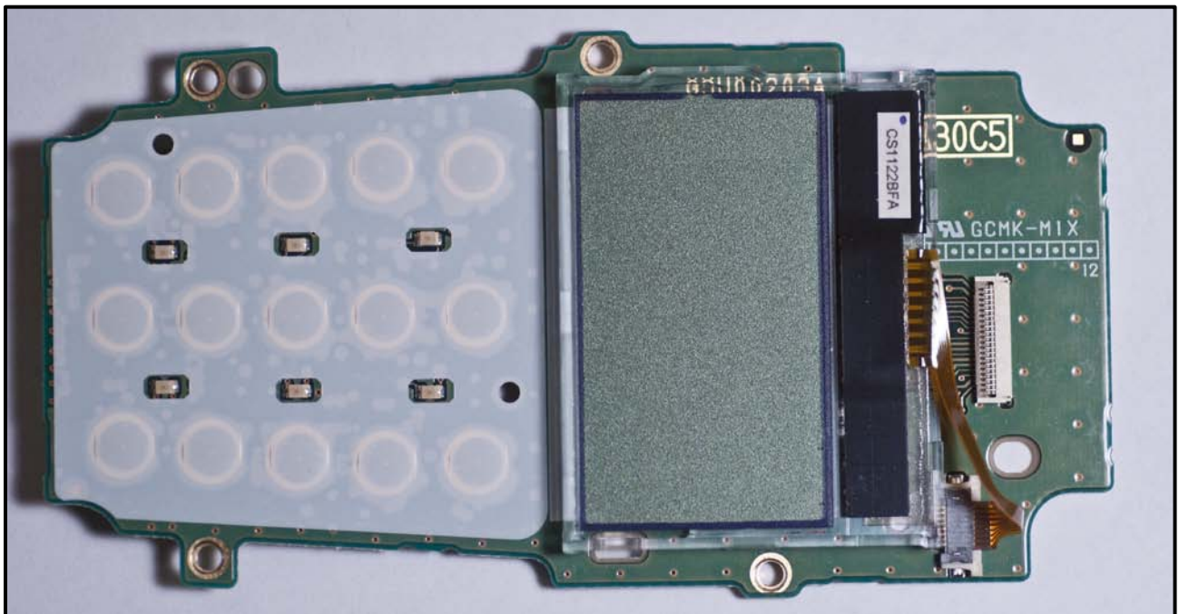
Photograph 20: Interface PWB – LCD Side
