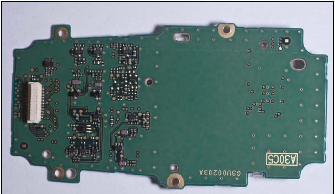
Photograph 19: Interface PWB – Component Side
