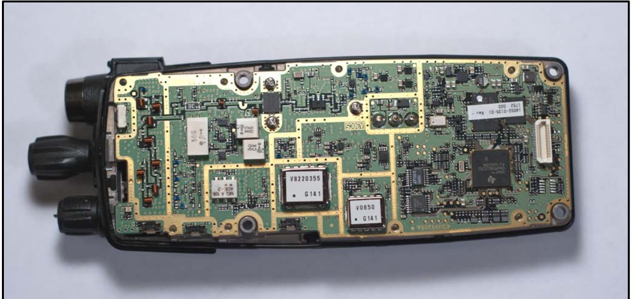
Photograph 15: Main PWB in Unit
