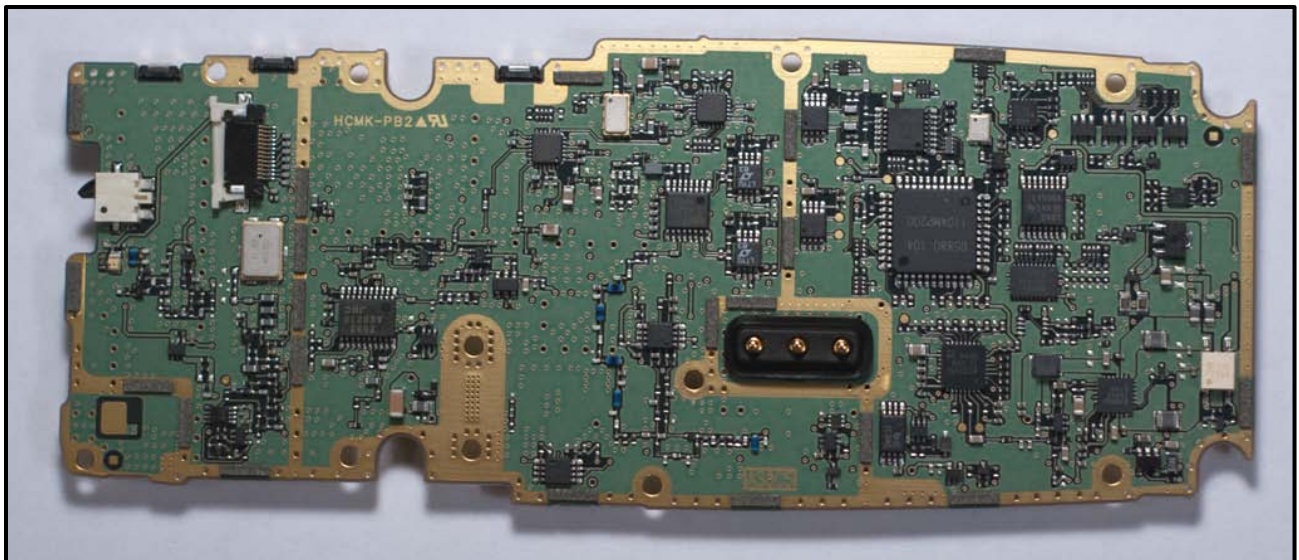
Photograph 16: Main PWB - Side 1
