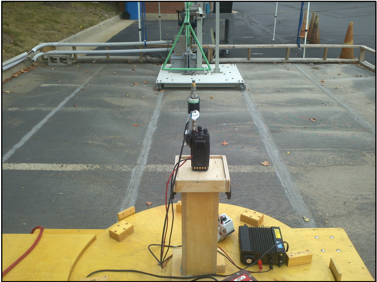
Photograph 6: Radiated Emissions – Back View
