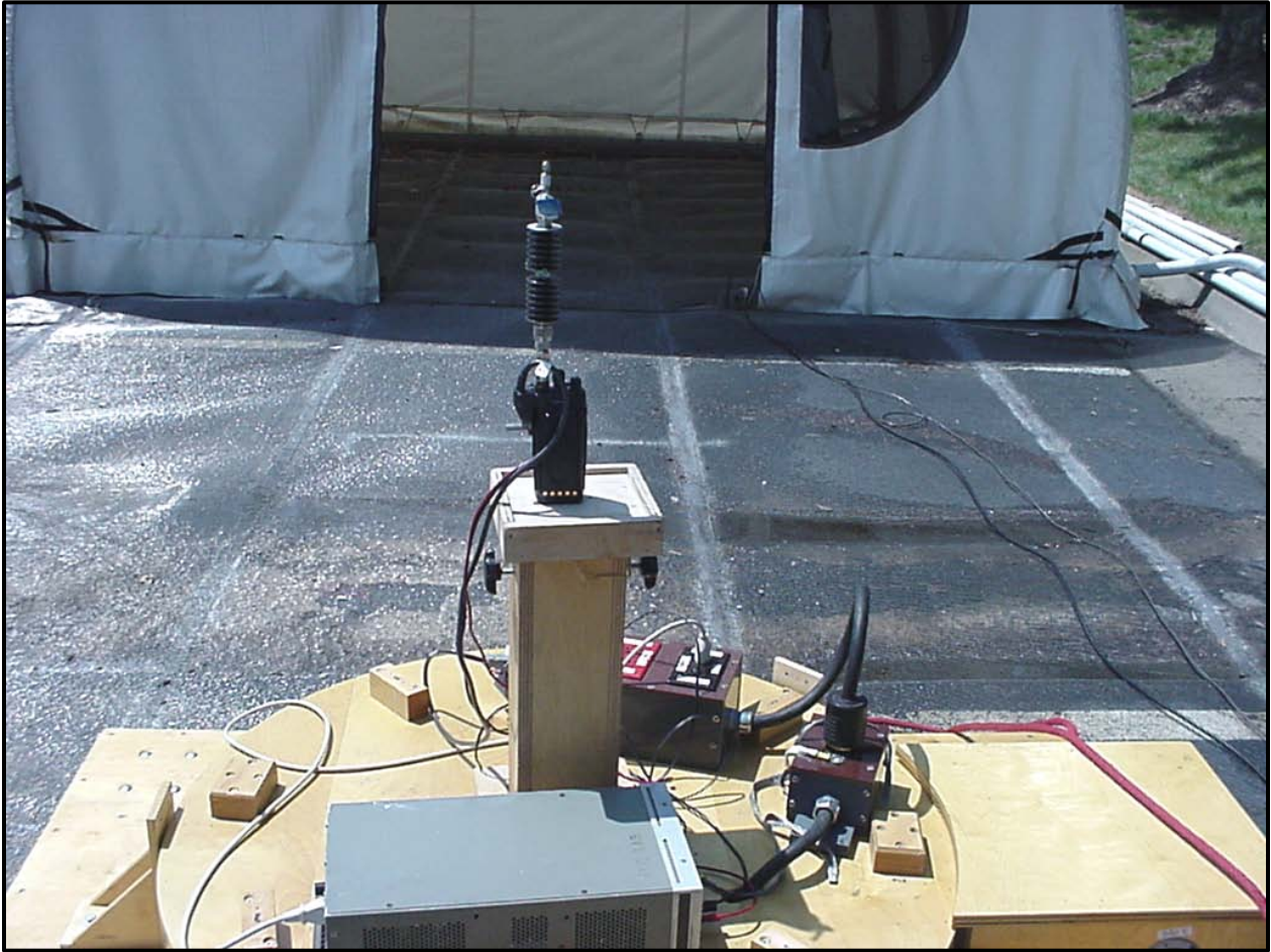
Photograph 5: Radiated Emissions – Back View
