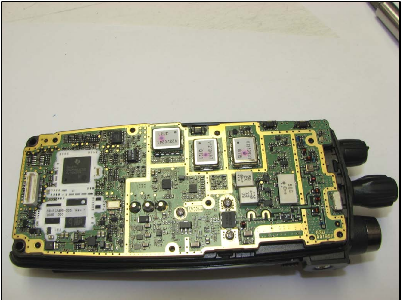
Photograph 15: Main PWB in Unit
