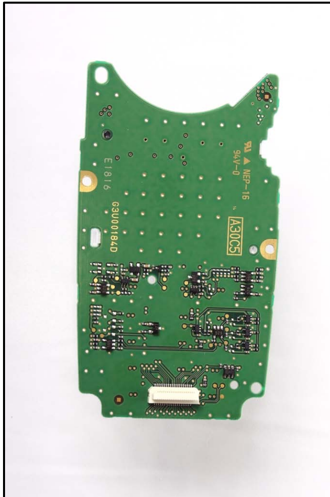
Photograph 19: Interface PWB Component Side
