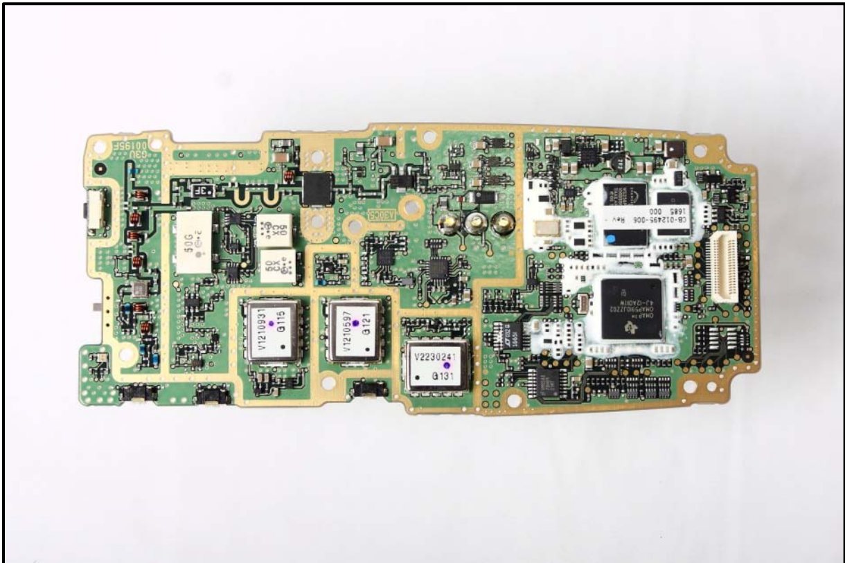
Photograph 16: Main PWB Side 1
