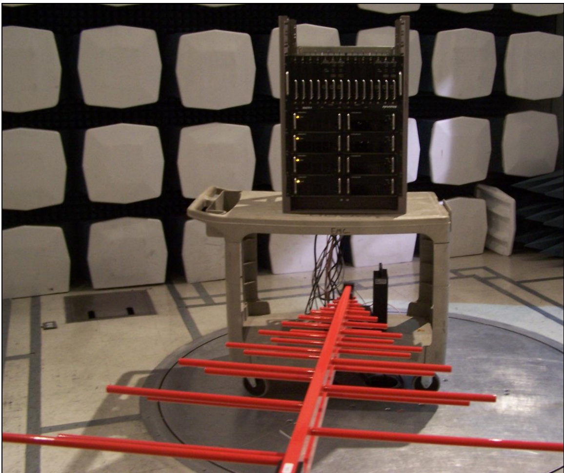
Photograph 2. Radiated Emission, Test Setup
