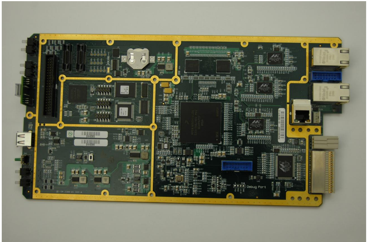
Photograph 10. Traffic Controller - Top Side
