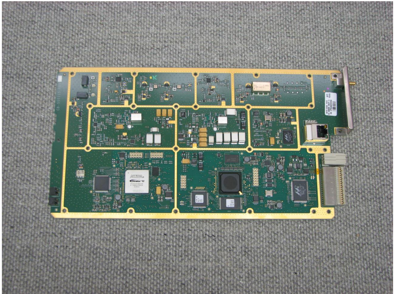
Photograph 14. VHF TX Exciter Module
