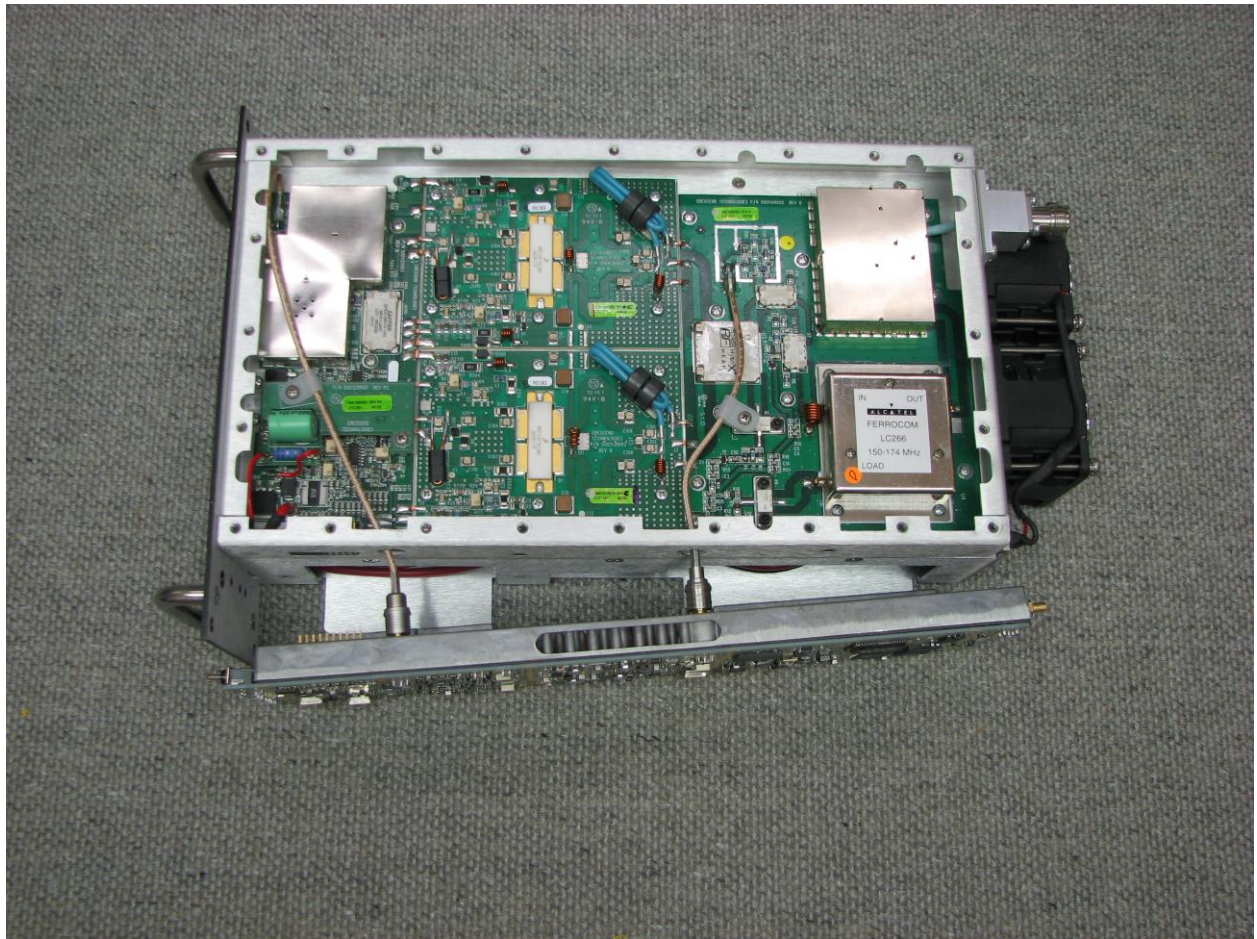
Photograph 11. VHF PA & Linearizer Paired
