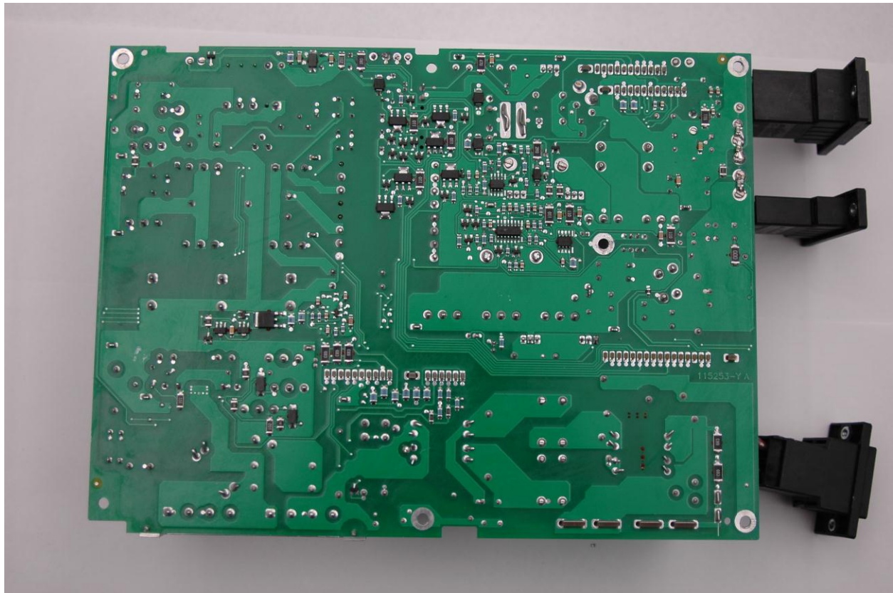
Photograph 7. Power Supply - Bottom Side
