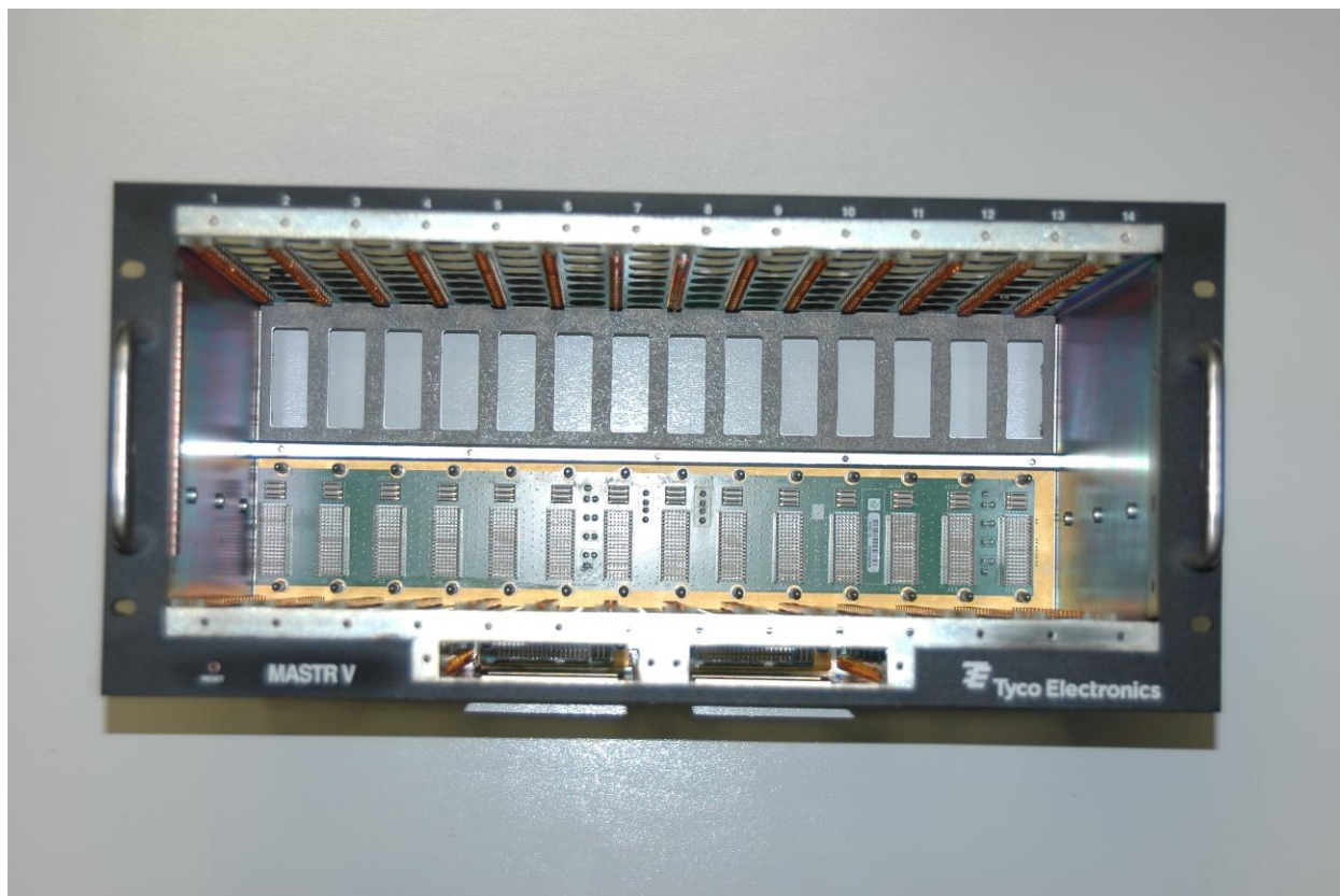
Photograph 3. Chassis – Front
