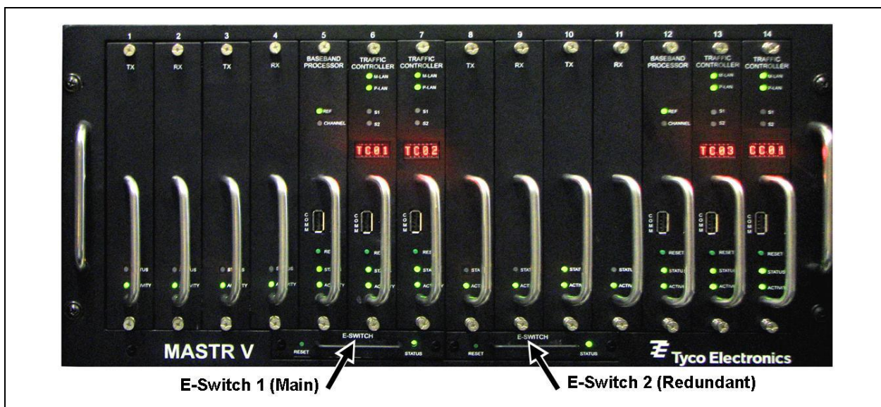
Figure 4-1: MASTR V 150-174 MHz Base Station Shelf equipped with Four (4) RF Channels
