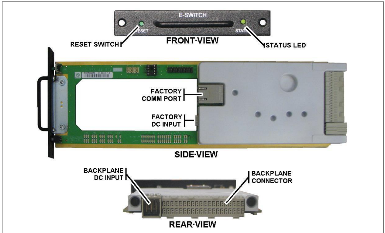
Figure 4-4: Ethernet Switch Module
