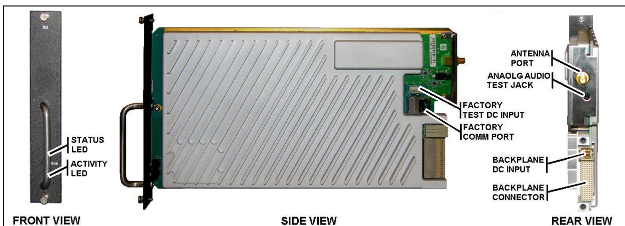
Figure 4-6: RX Module
