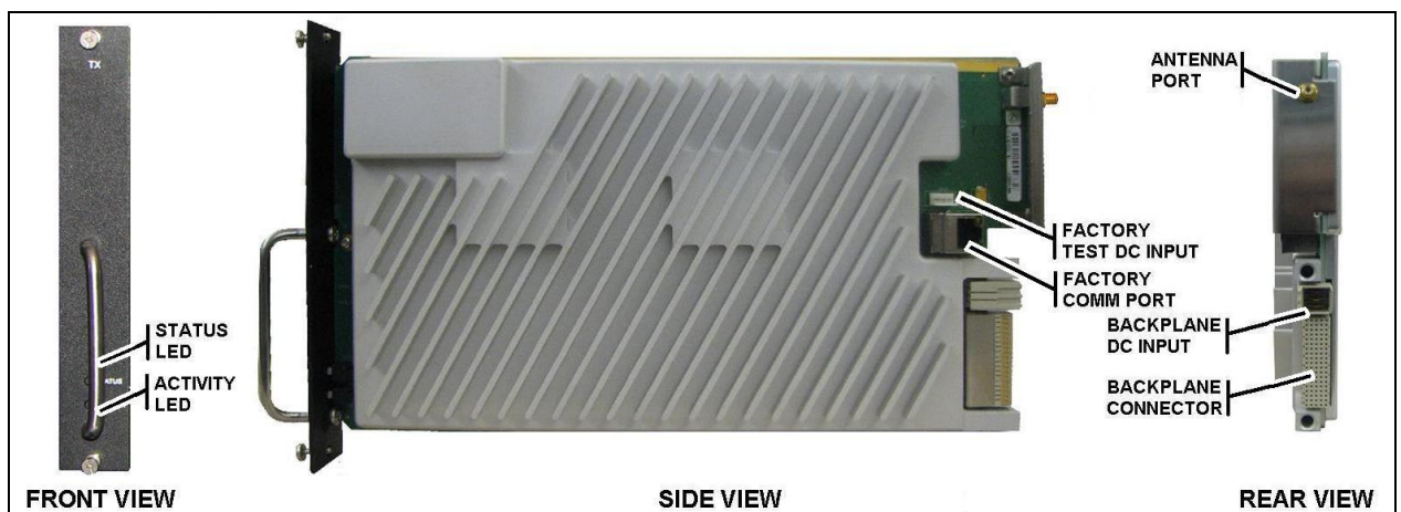
Figure 4-5: TX Module
