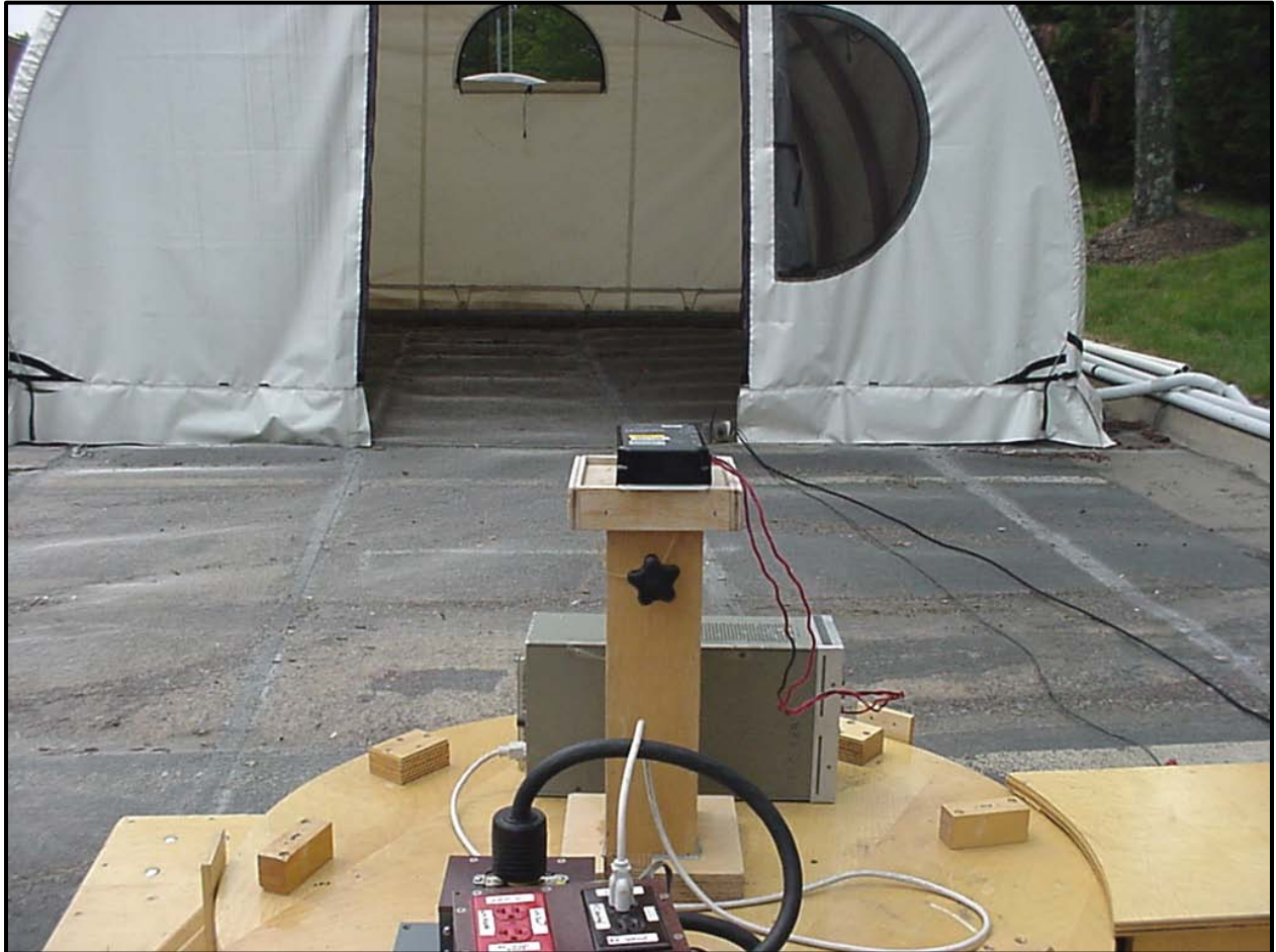
Photograph 3: Radiated Emissions – Front View
