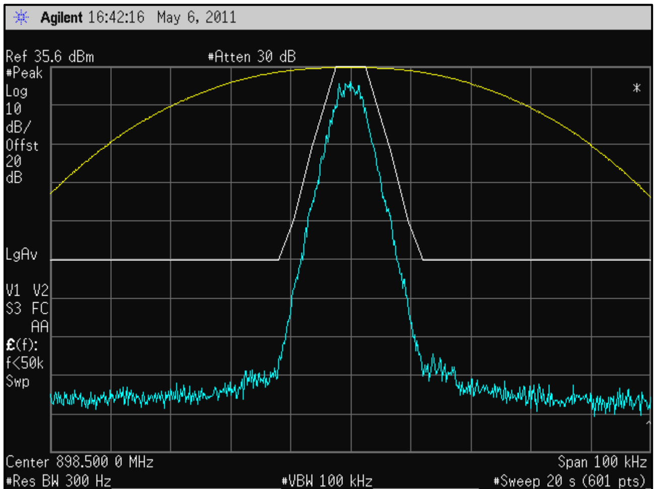
Plot 6-2: Occupied Bandwidth – 898.5000 MHz Mask J
