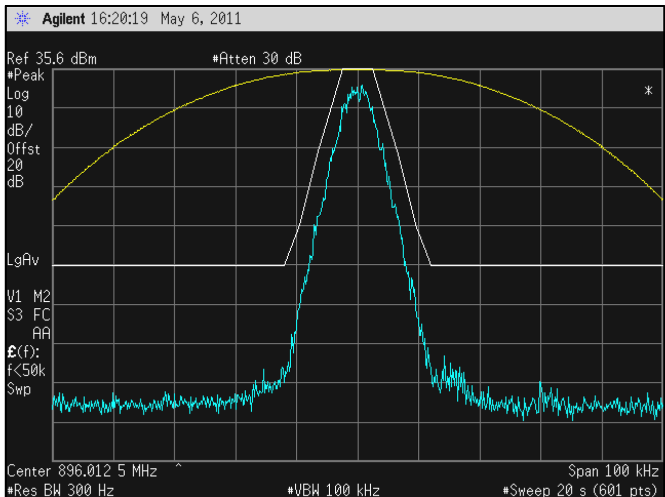
Plot 6-1: Occupied Bandwidth – 896.0125 MHz Mask J
