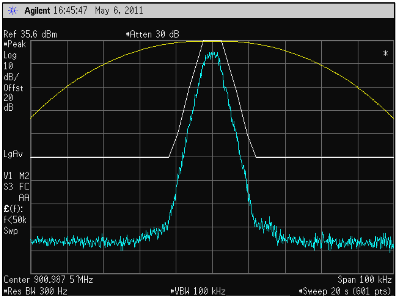
Plot 6-3: Occupied Bandwidth – 900.9875 MHz Mask J
