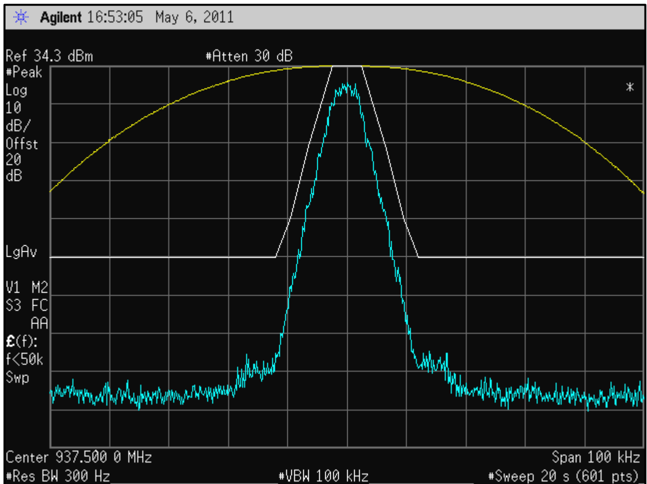
Plot 6-5: Occupied Bandwidth – 937.5000 MHz Mask J
