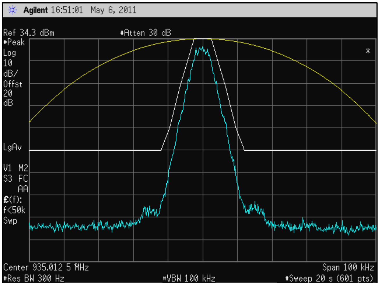
Plot 6-4: Occupied Bandwidth – 935.0125 MHz Mask J
